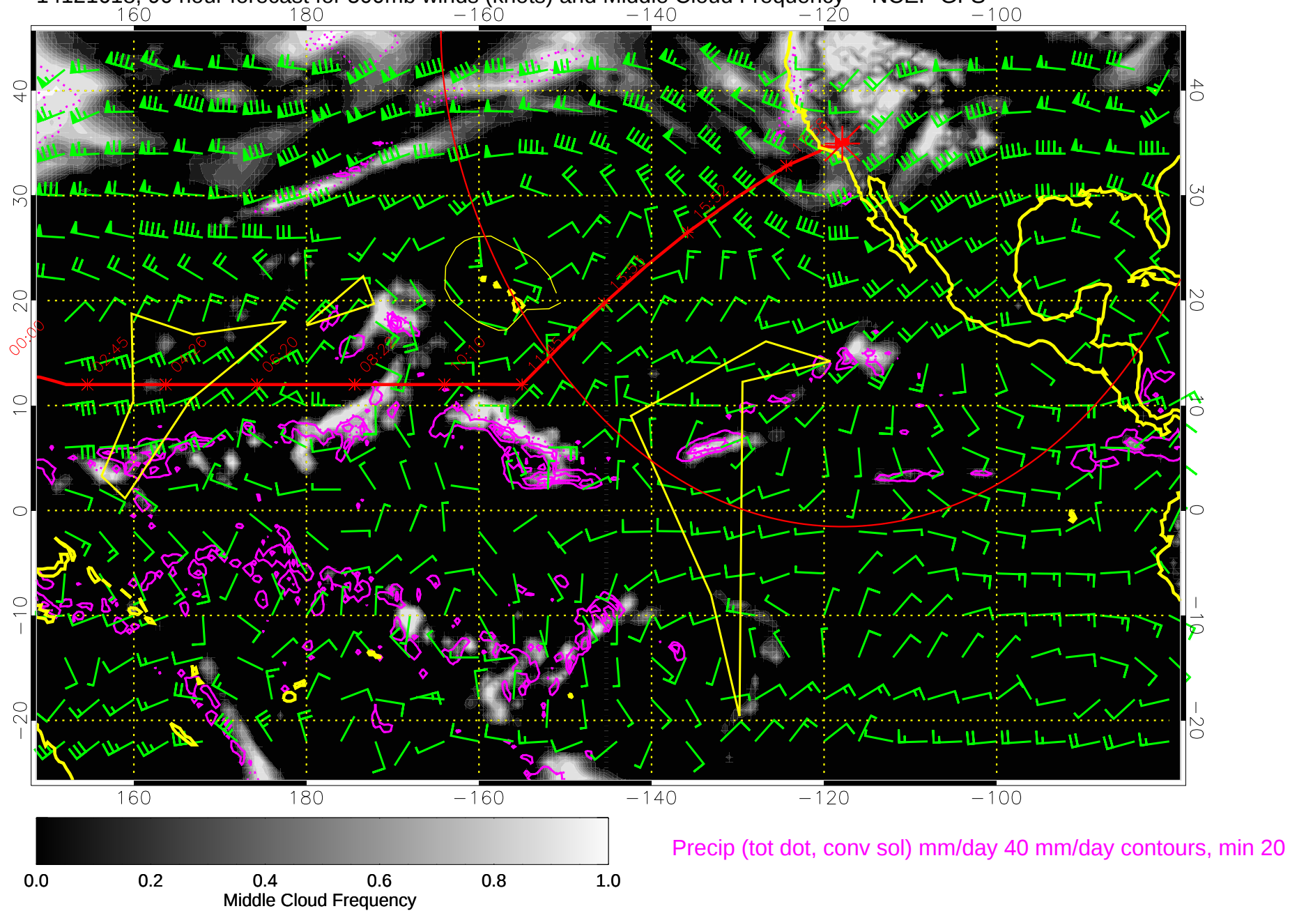
14121618, 90 hour forecast for 500mb winds (knots) and Middle Cloud Frequency -- NCEP GFS
