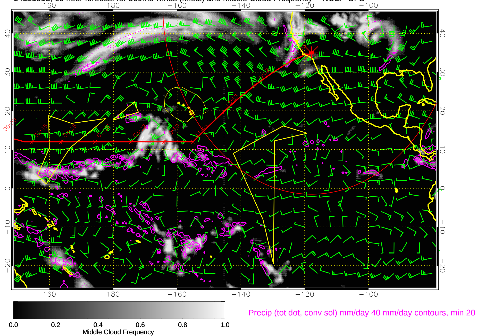
14121512, 60 hour forecast for 500mb winds (knots) and Middle Cloud Frequency -- NCEP GFS
