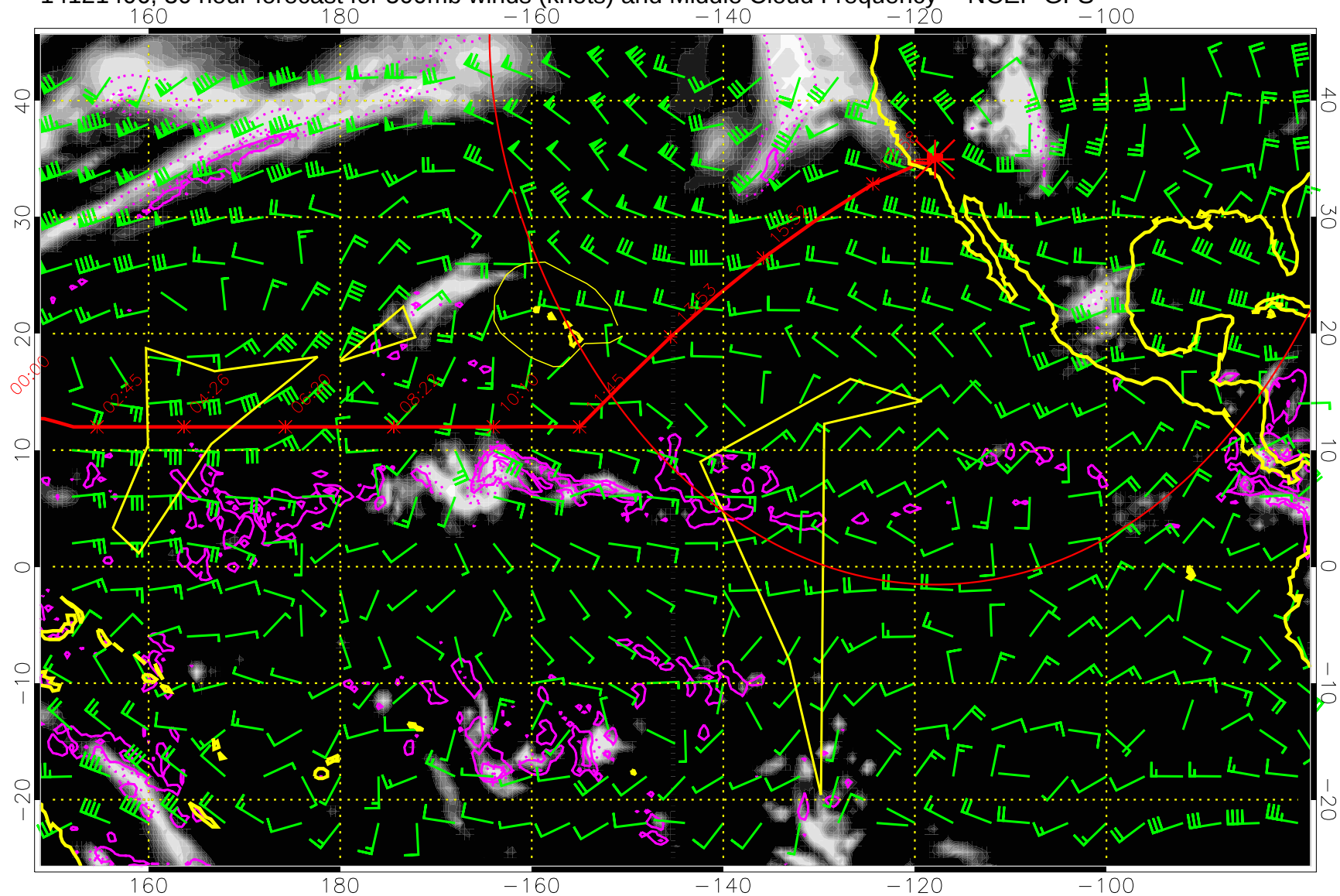
14121406, 30 hour forecast for 500mb winds (knots) and Middle Cloud Frequency -- NCEP GFS
