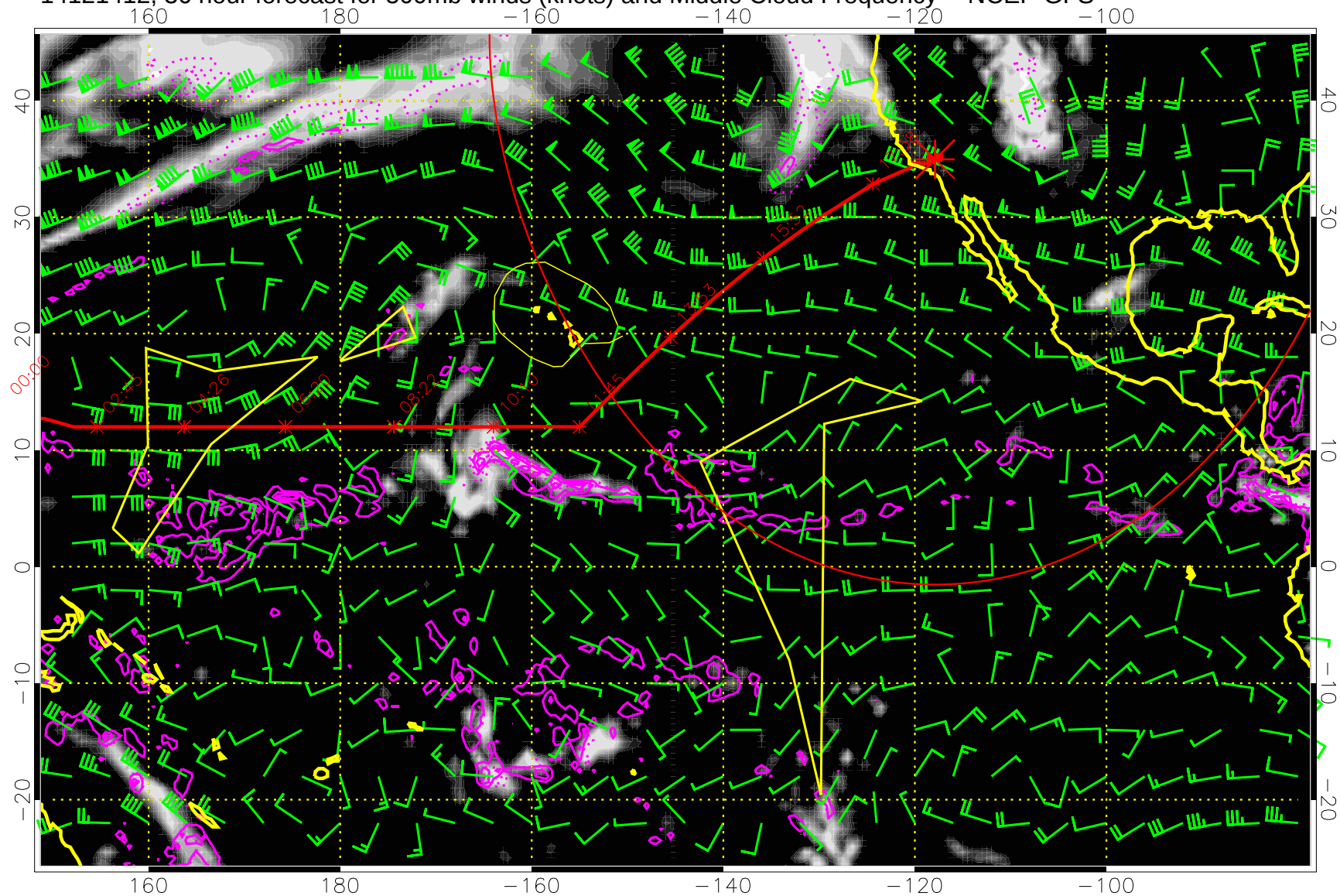
14121412, 36 hour forecast for 500mb winds (knots) and Middle Cloud Frequency -- NCEP GFS
