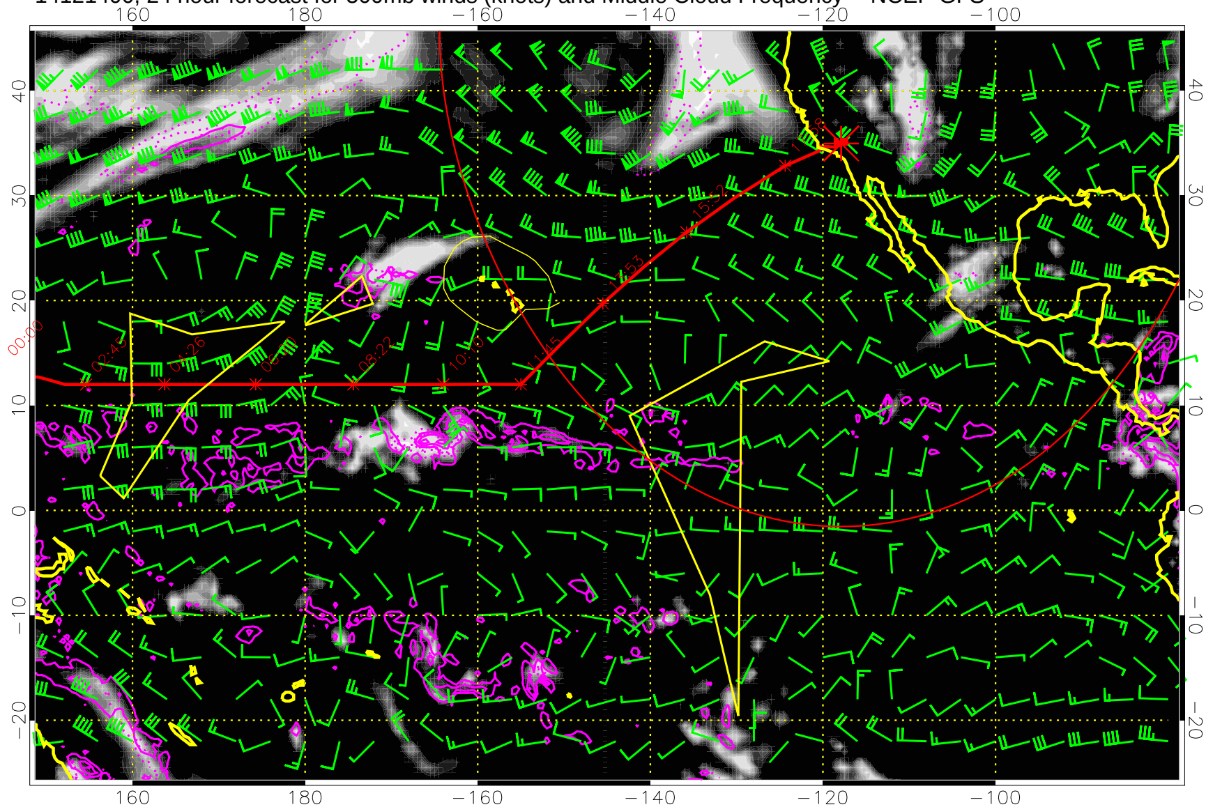
14121400, 24 hour forecast for 500mb winds (knots) and Middle Cloud Frequency -- NCEP GFS
