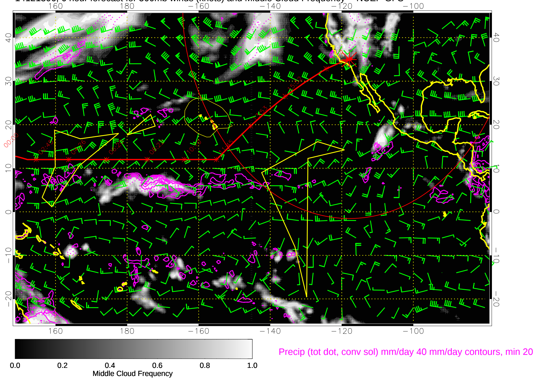
14121306, 6 hour forecast for 500mb winds (knots) and Middle Cloud Frequency -- NCEP GFS
