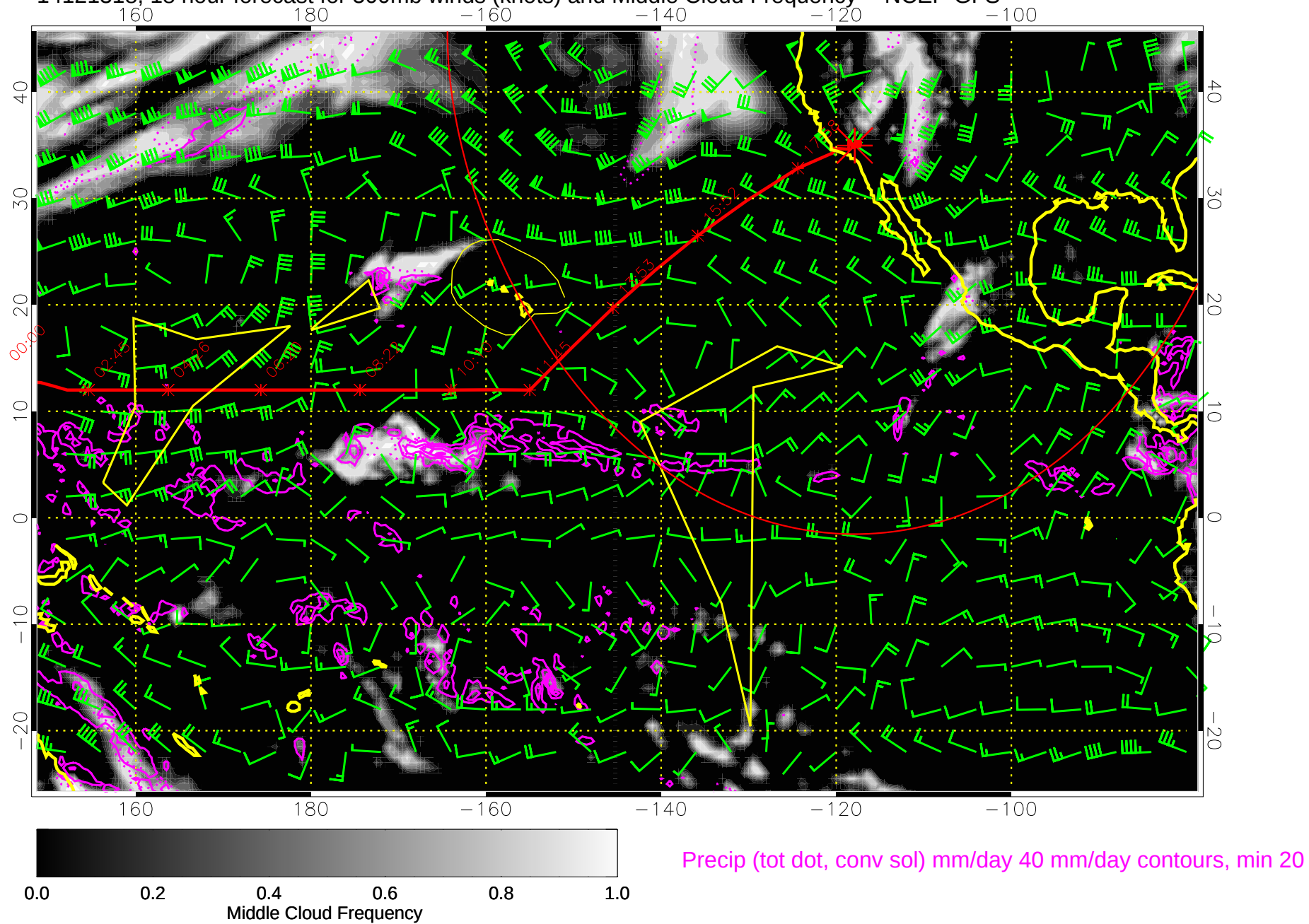
14121318, 18 hour forecast for 500mb winds (knots) and Middle Cloud Frequency -- NCEP GFS
