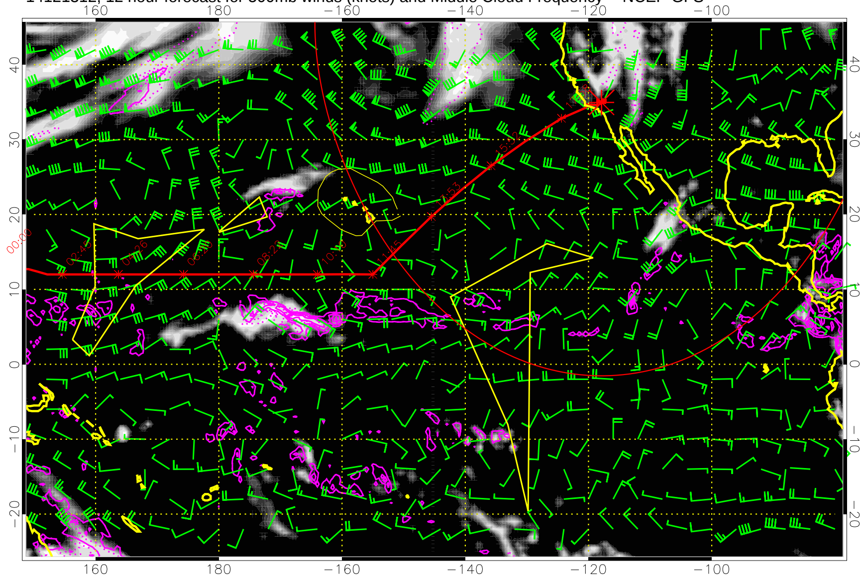
14121312, 12 hour forecast for 500mb winds (knots) and Middle Cloud Frequency -- NCEP GFS
