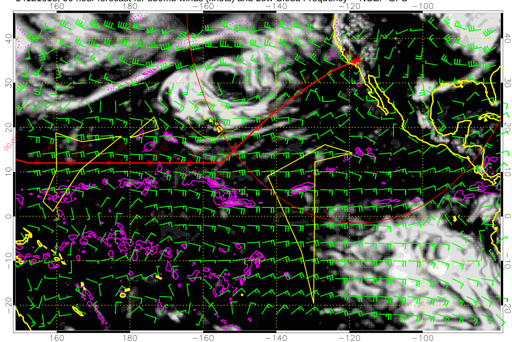
14121618, 90 hour forecast for 850mb winds (knots) and Low Cloud Frequency -- NCEP GFS
