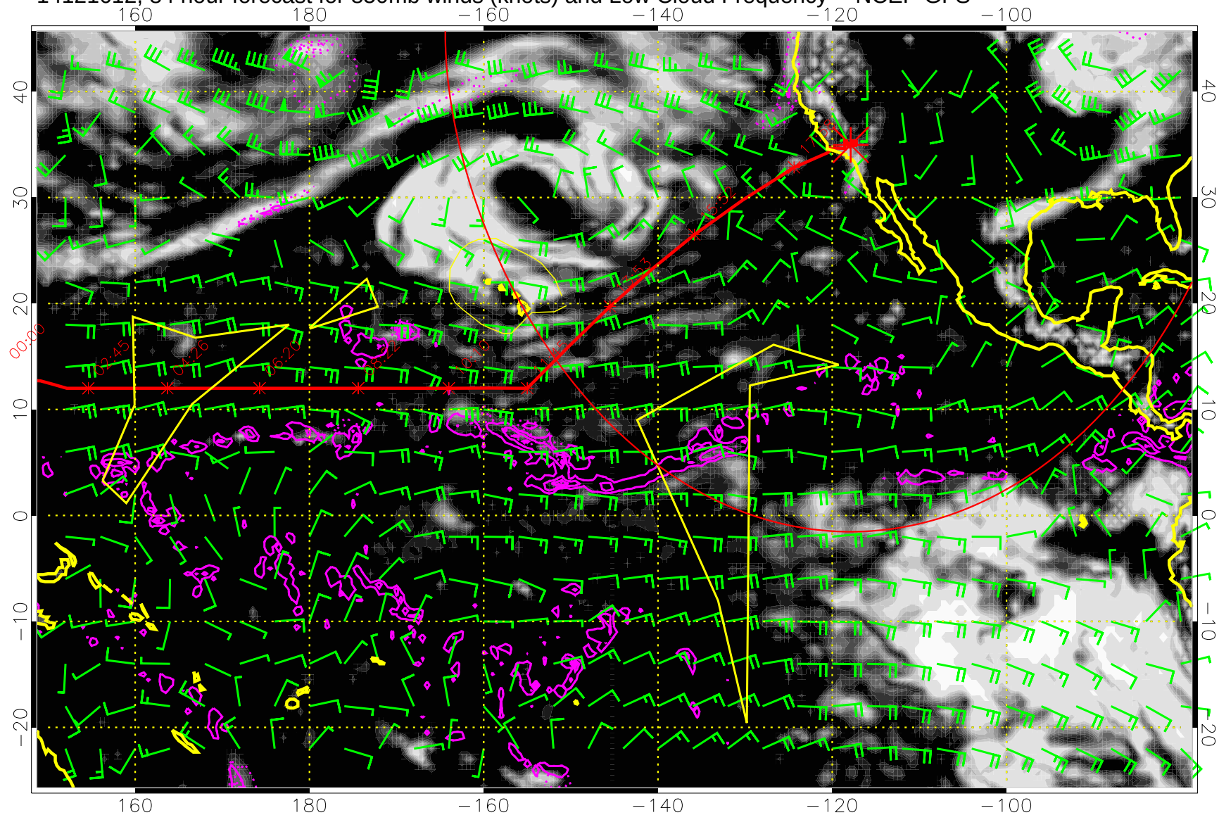
14121612, 84 hour forecast for 850mb winds (knots) and Low Cloud Frequency -- NCEP GFS
