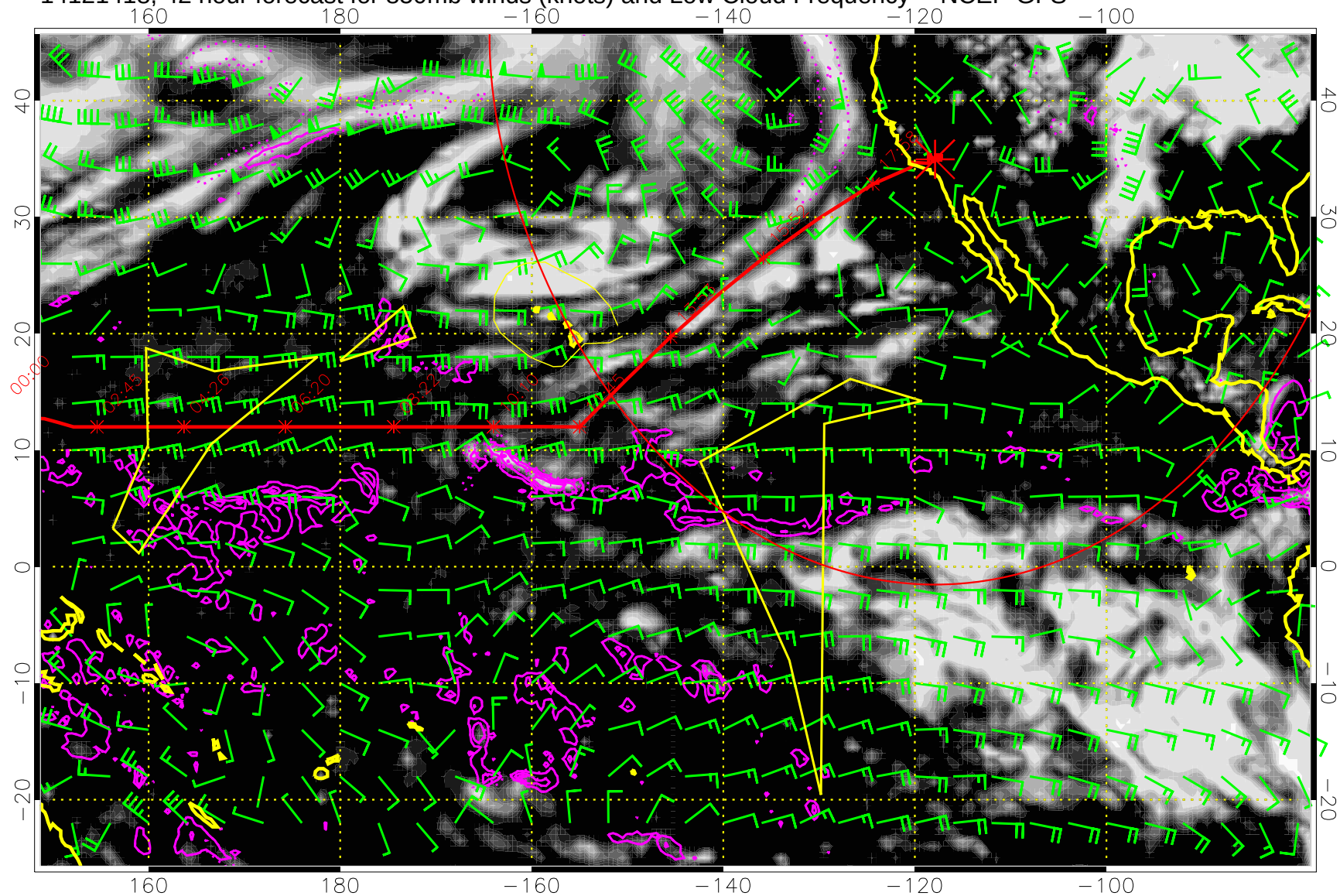
14121418, 42 hour forecast for 850mb winds (knots) and Low Cloud Frequency -- NCEP GFS
