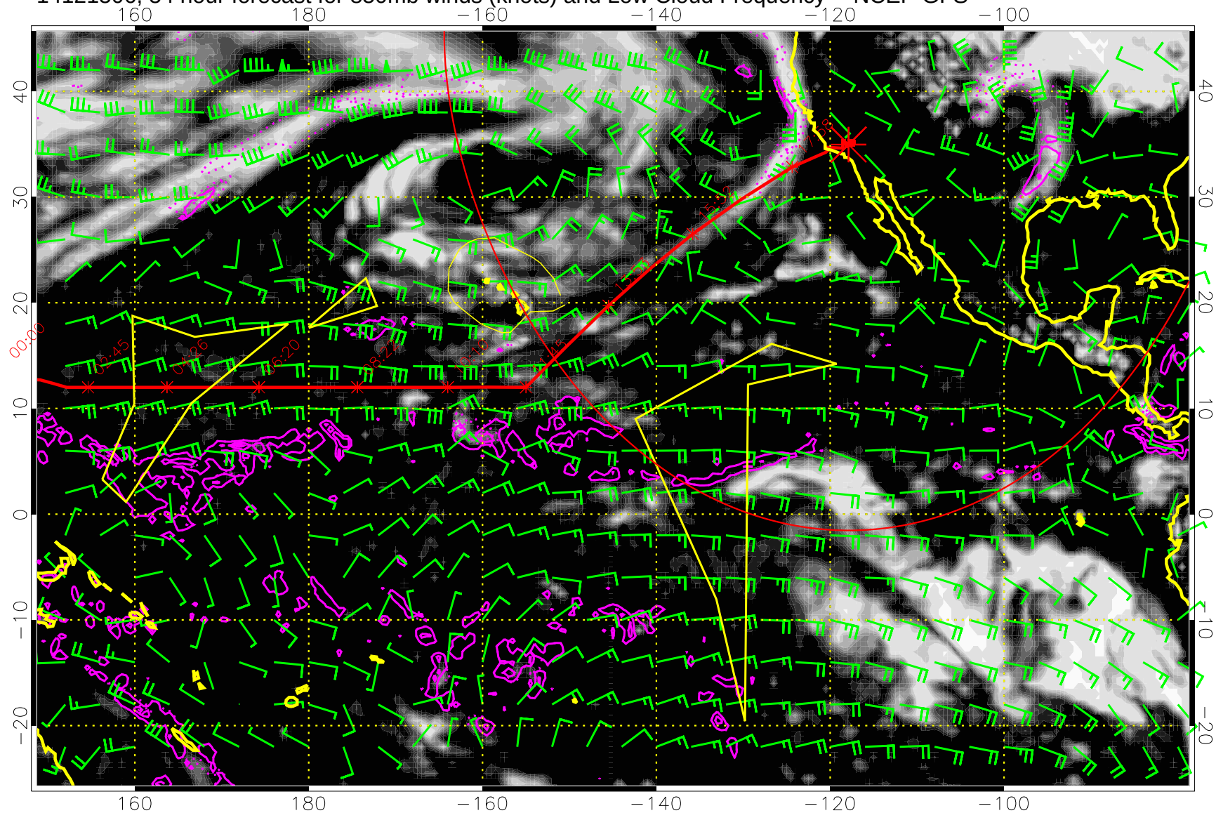
14121506, 54 hour forecast for 850mb winds (knots) and Low Cloud Frequency -- NCEP GFS
