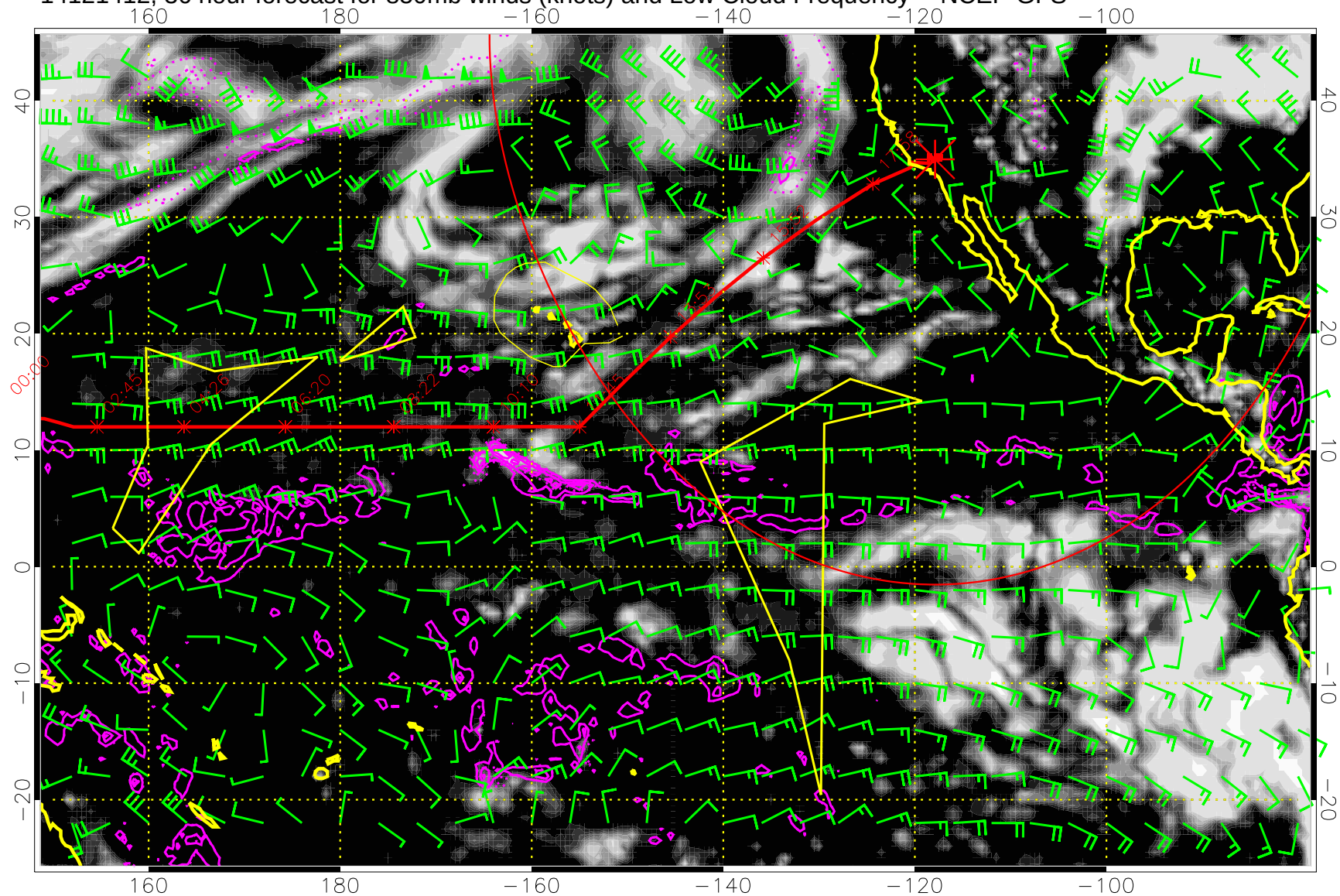
14121412, 36 hour forecast for 850mb winds (knots) and Low Cloud Frequency -- NCEP GFS
