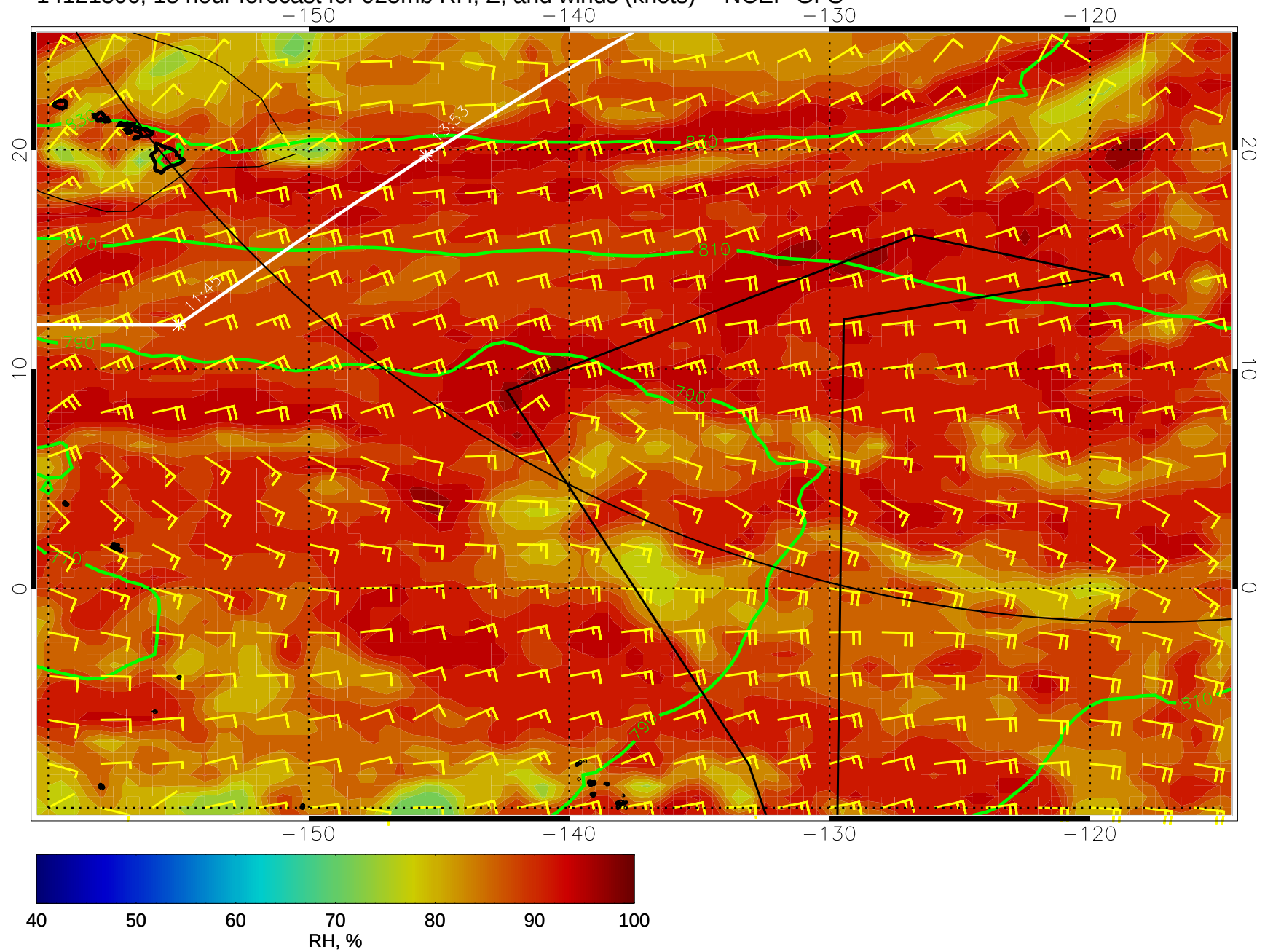
14121306, 18 hour forecast for 925mb RH, Z, and winds (knots) -- NCEP GFS
