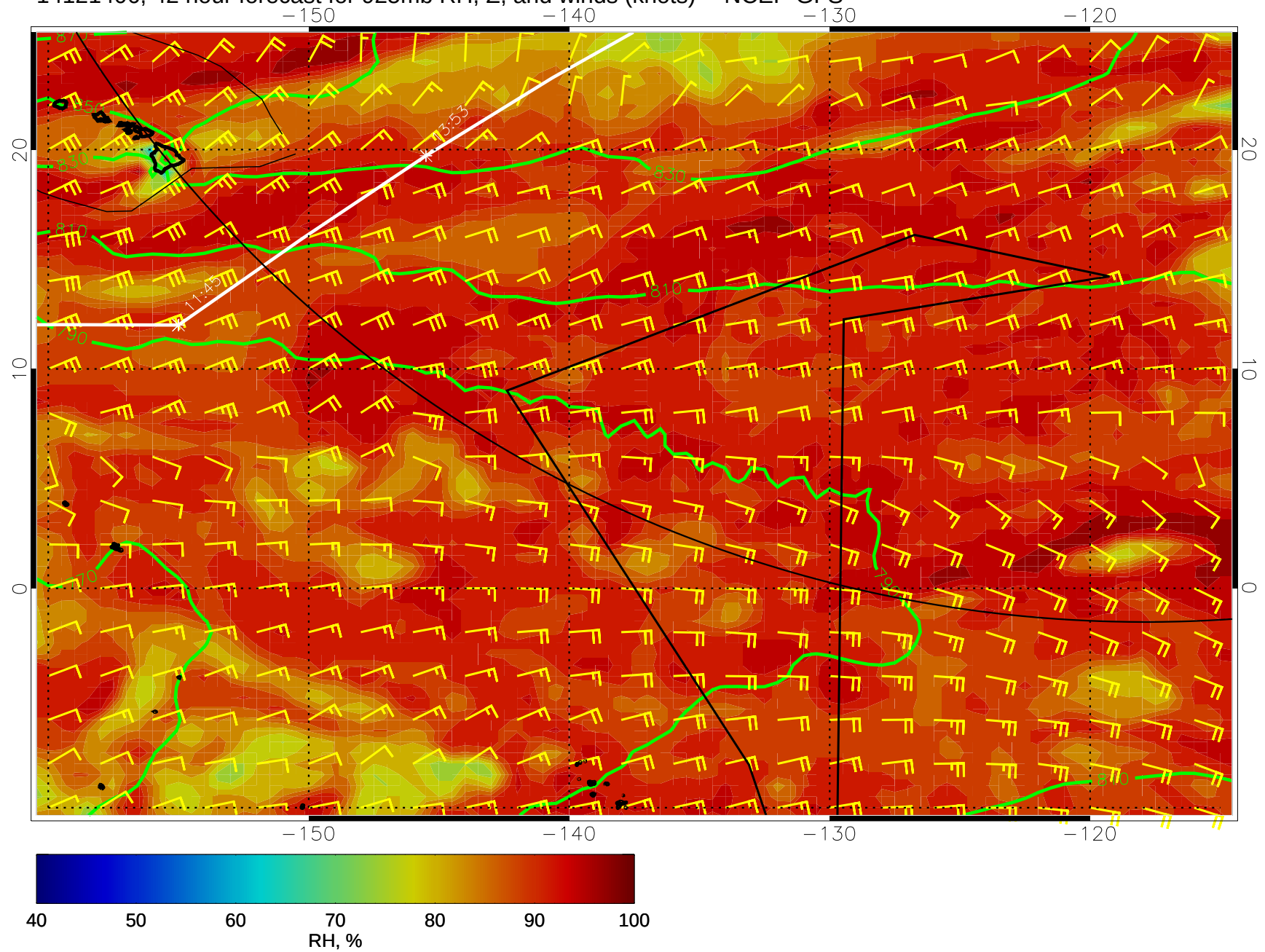
14121406, 42 hour forecast for 925mb RH, Z, and winds (knots) -- NCEP GFS
