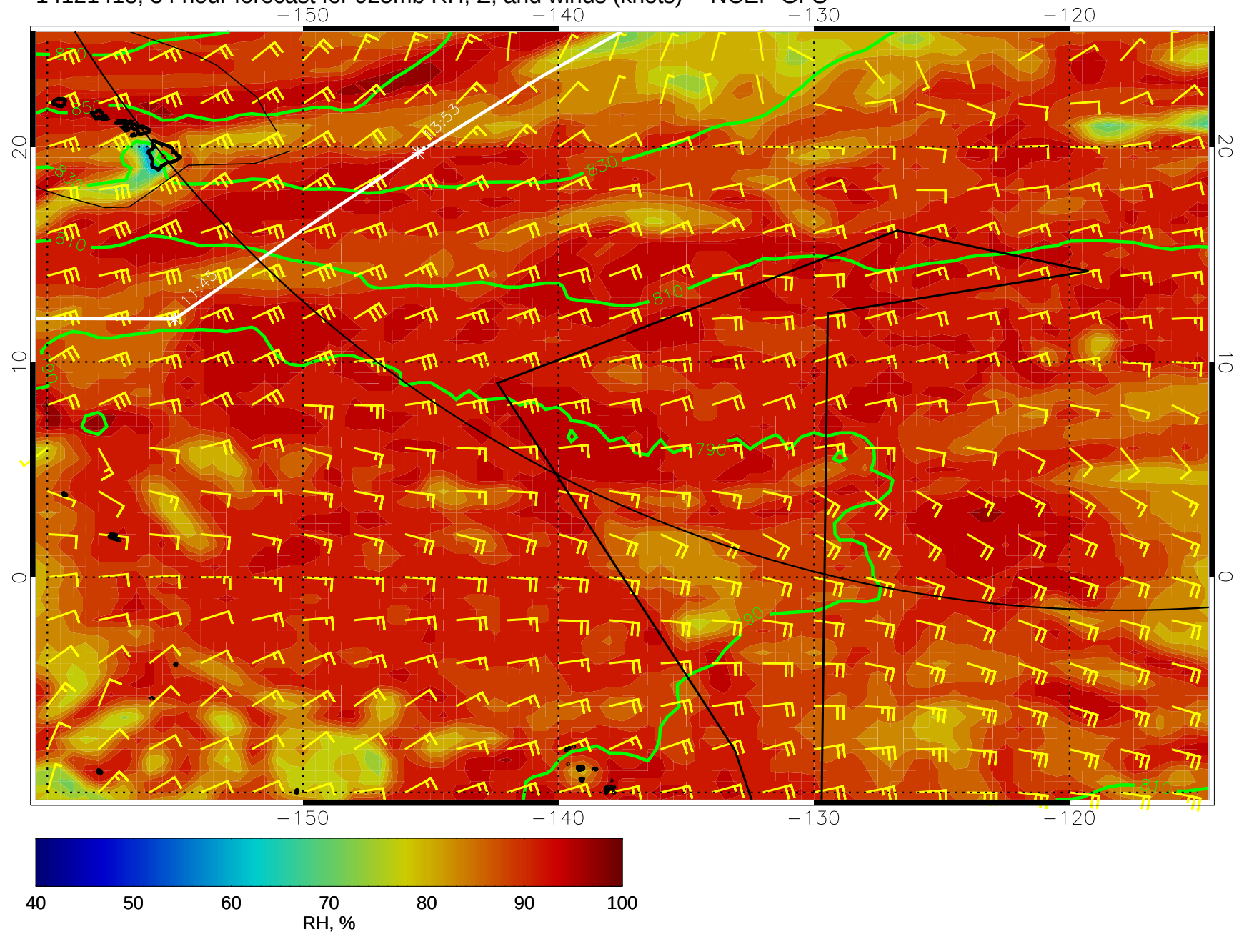
14121418, 54 hour forecast for 925mb RH, Z, and winds (knots) -- NCEP GFS
