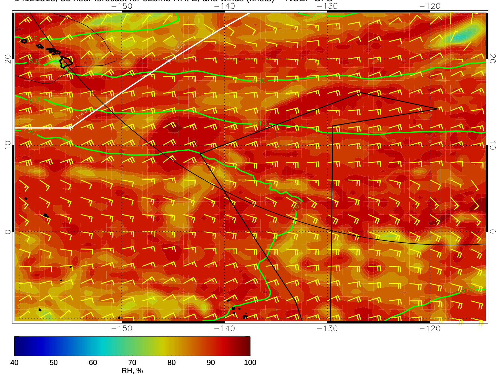
14121318, 30 hour forecast for 925mb RH, Z, and winds (knots) -- NCEP GFS
