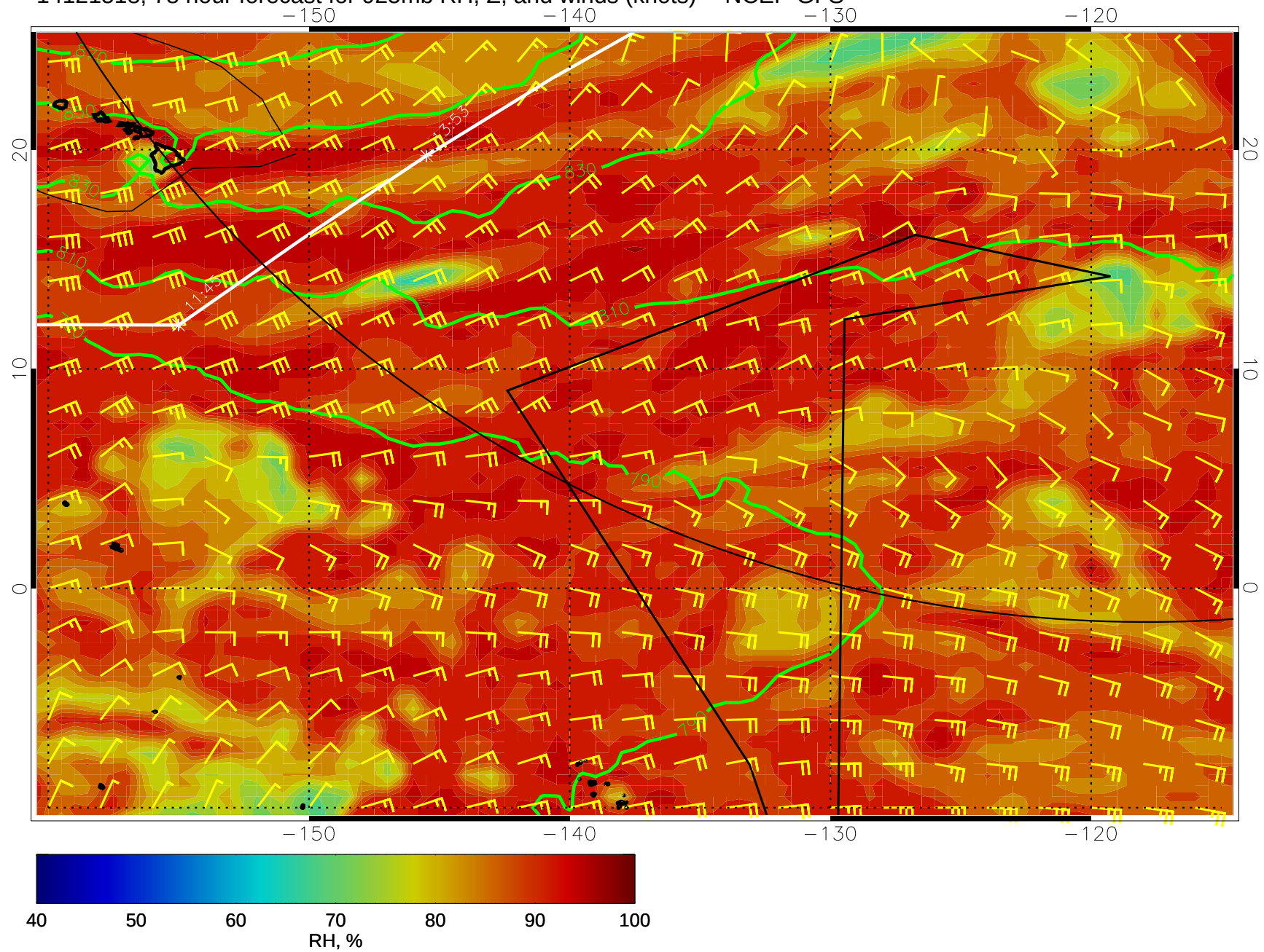
14121518, 78 hour forecast for 925mb RH, Z, and winds (knots) -- NCEP GFS
