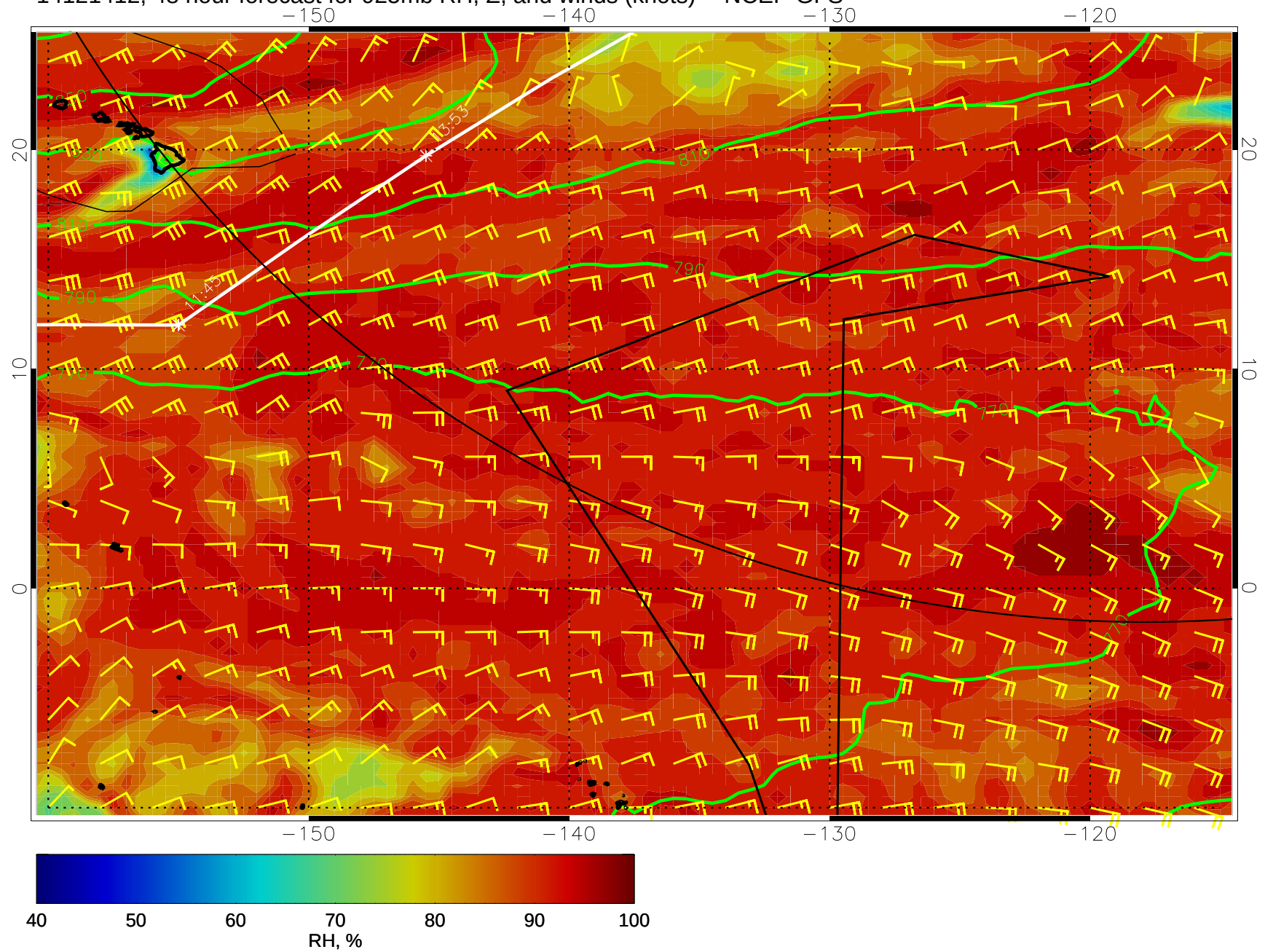
14121412, 48 hour forecast for 925mb RH, Z, and winds (knots) -- NCEP GFS
