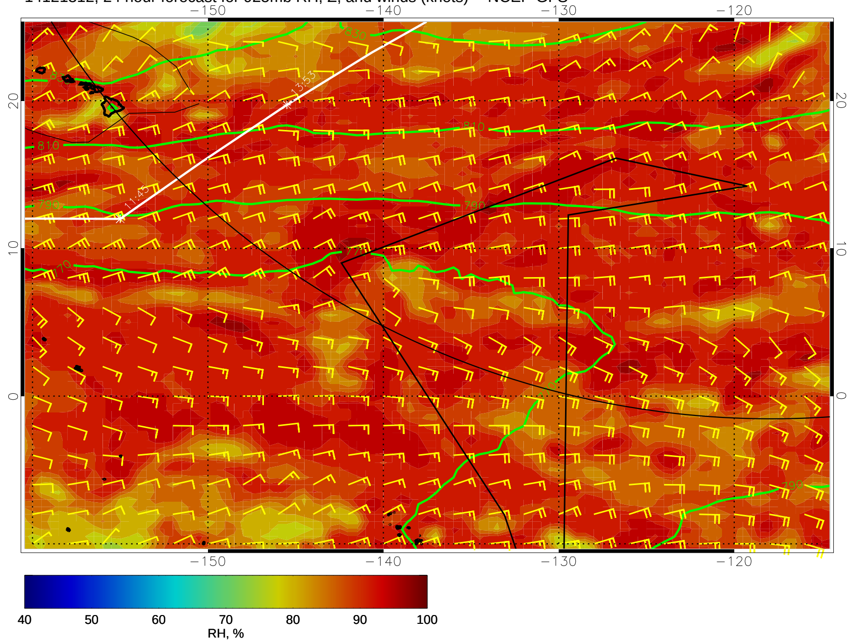
14121312, 24 hour forecast for 925mb RH, Z, and winds (knots) -- NCEP GFS
