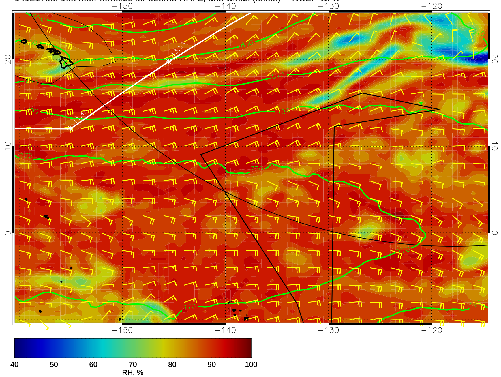
14121700, 108 hour forecast for 925mb RH, Z, and winds (knots) -- NCEP GFS
