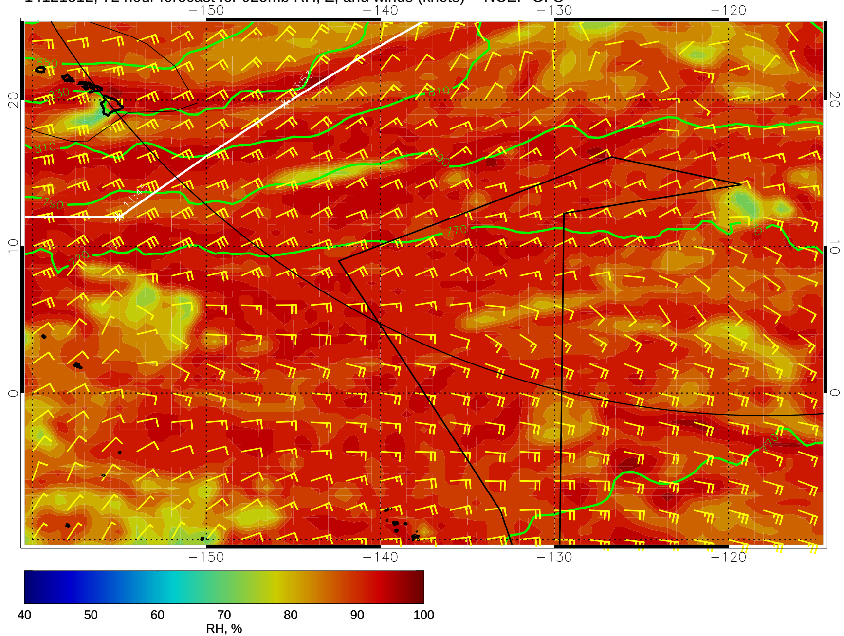
14121512, 72 hour forecast for 925mb RH, Z, and winds (knots) -- NCEP GFS
