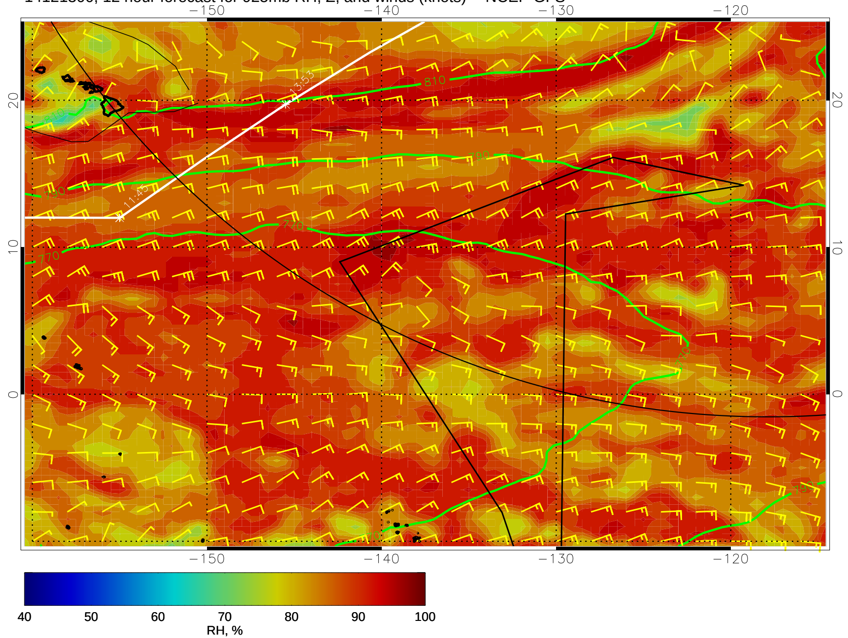
14121300, 12 hour forecast for 925mb RH, Z, and winds (knots) -- NCEP GFS
