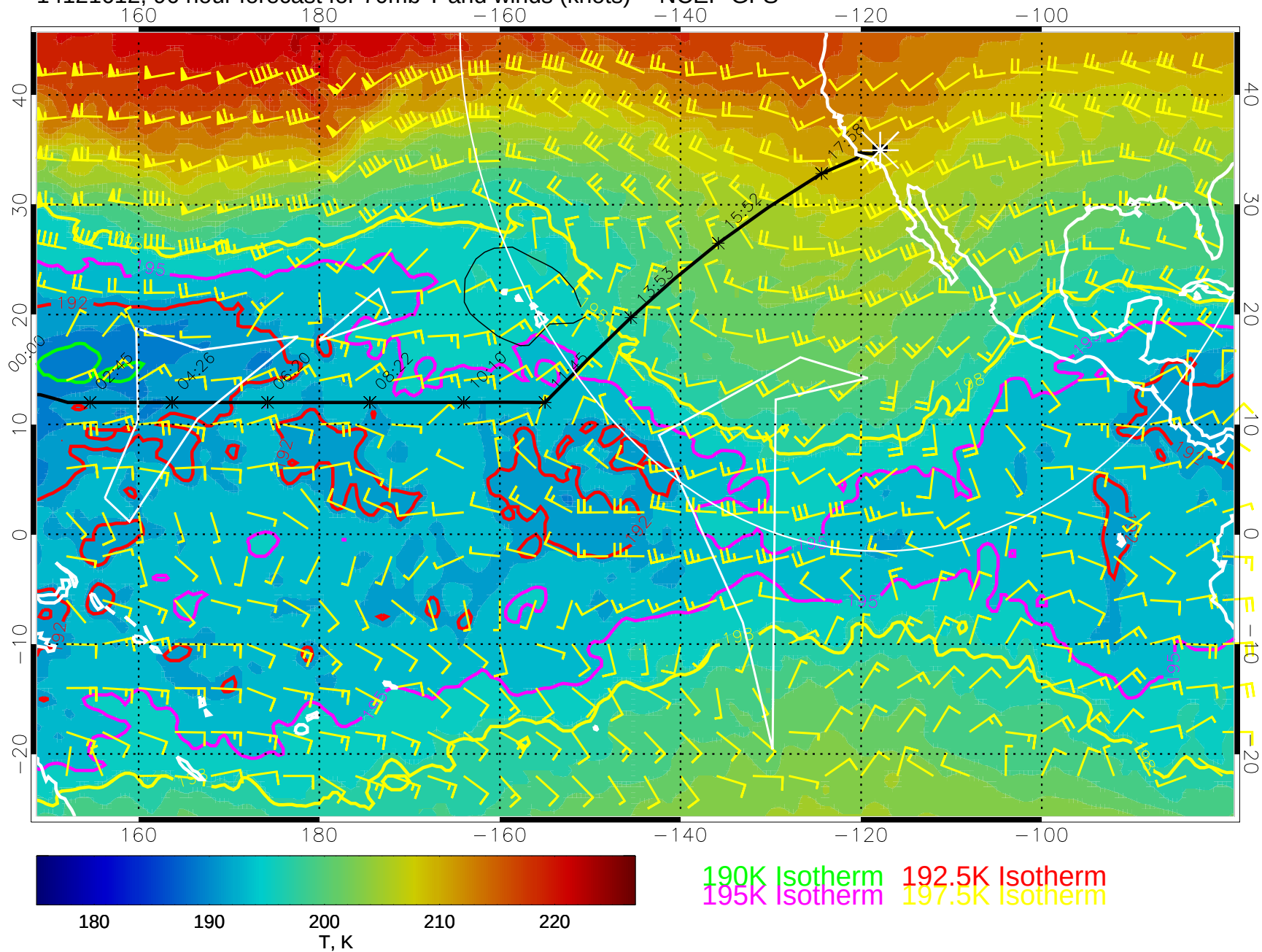
14121612, 96 hour forecast for 70mb T and winds (knots) -- NCEP GFS
