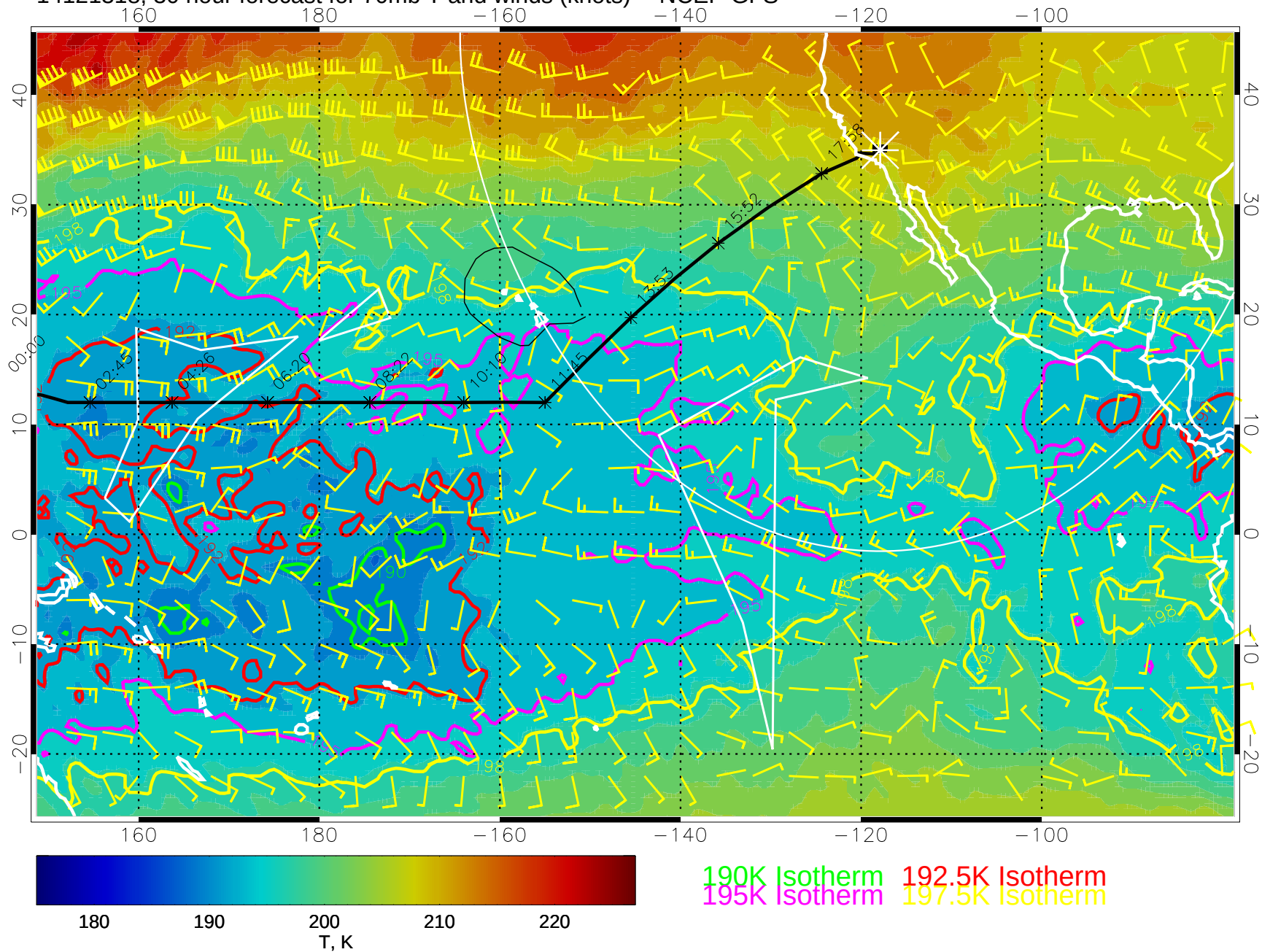
14121318, 30 hour forecast for 70mb T and winds (knots) -- NCEP GFS
