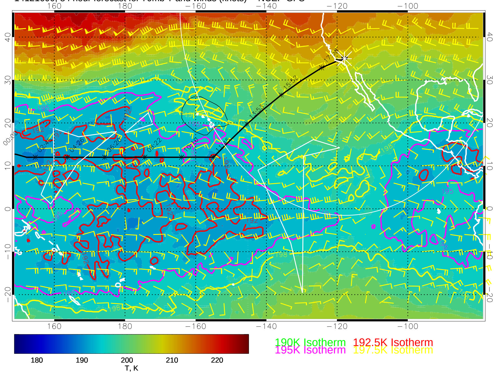
14121600, 84 hour forecast for 70mb T and winds (knots) -- NCEP GFS
