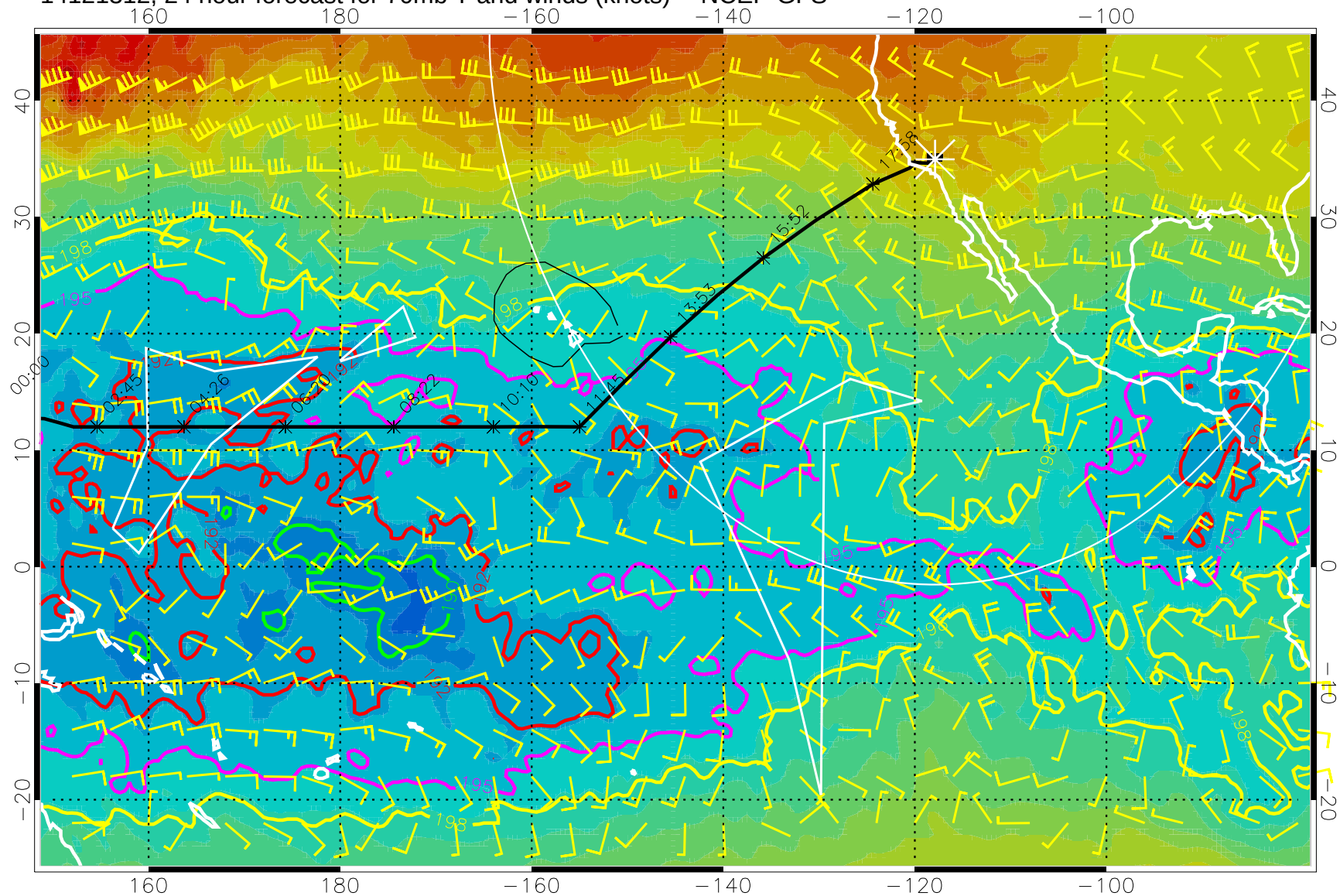
14121312, 24 hour forecast for 70mb T and winds (knots) -- NCEP GFS
