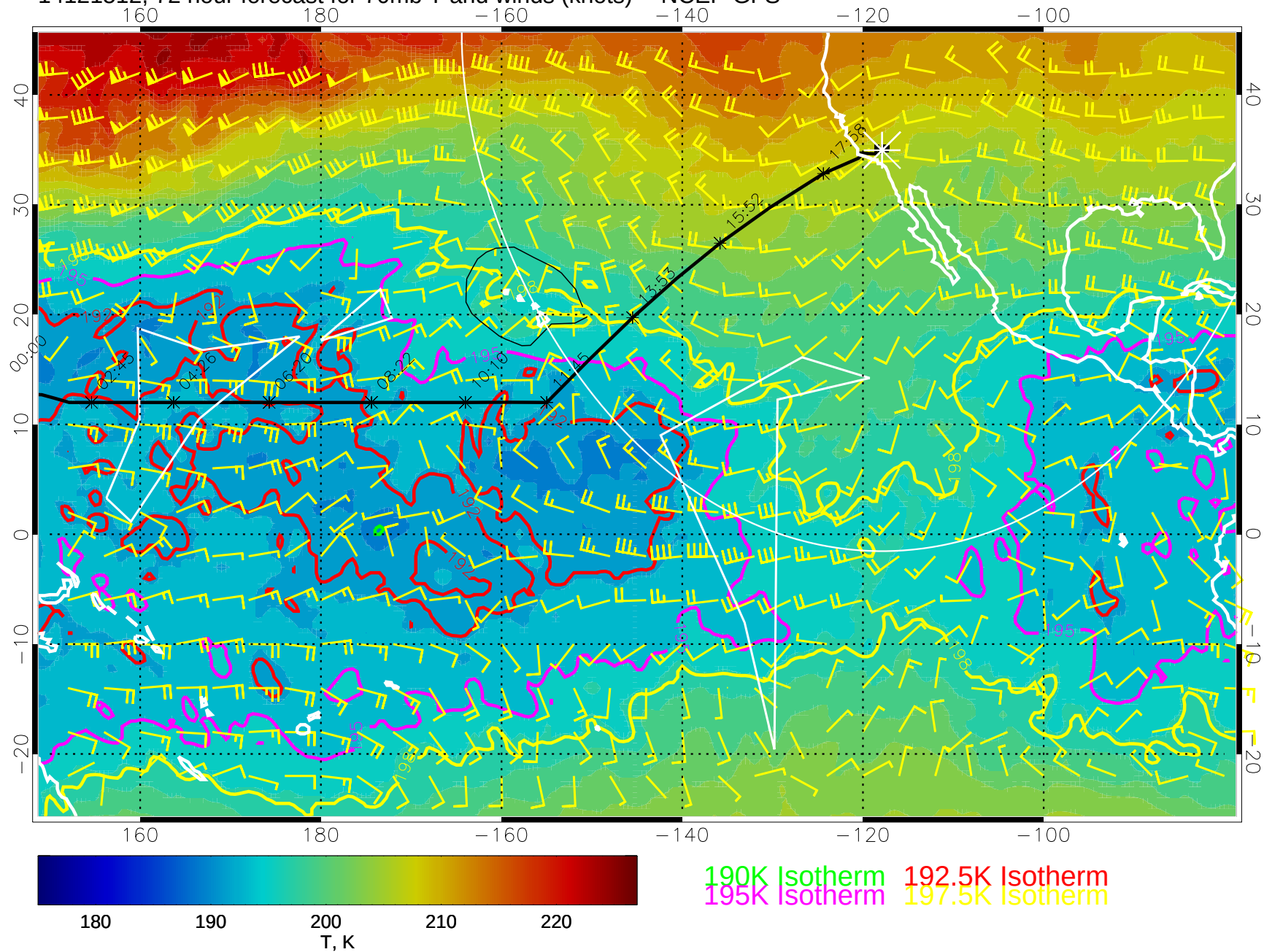
14121512, 72 hour forecast for 70mb T and winds (knots) -- NCEP GFS
