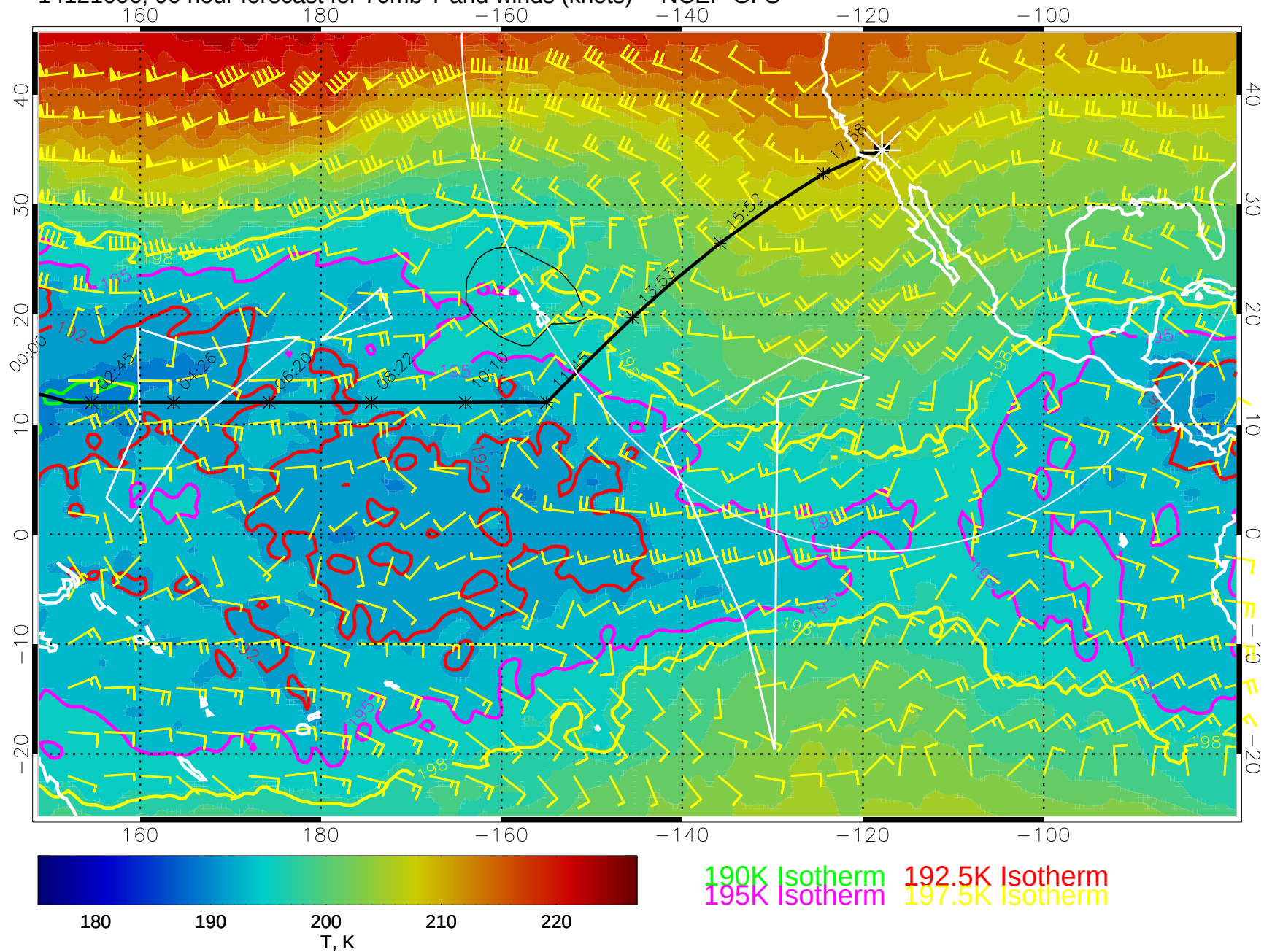
14121606, 90 hour forecast for 70mb T and winds (knots) -- NCEP GFS
