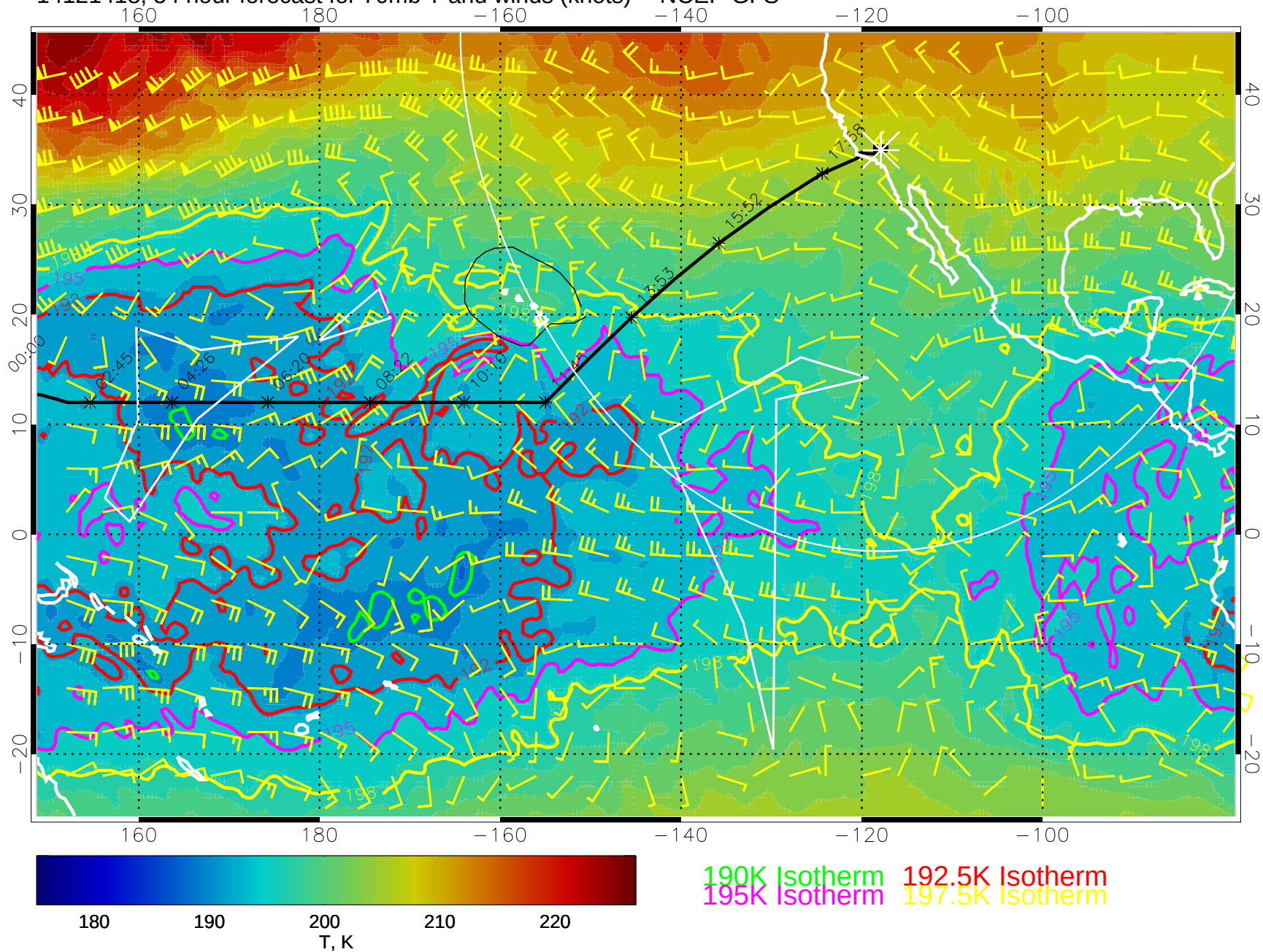
14121418, 54 hour forecast for 70mb T and winds (knots) -- NCEP GFS
