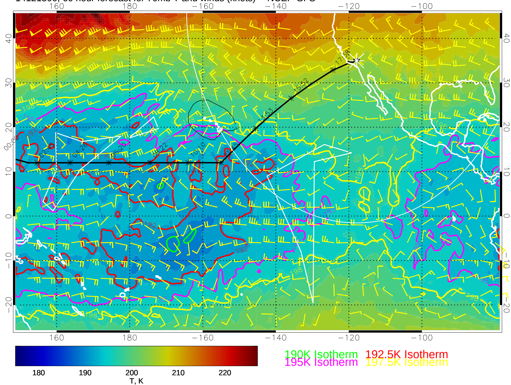
14121500, 60 hour forecast for 70mb T and winds (knots) -- NCEP GFS
