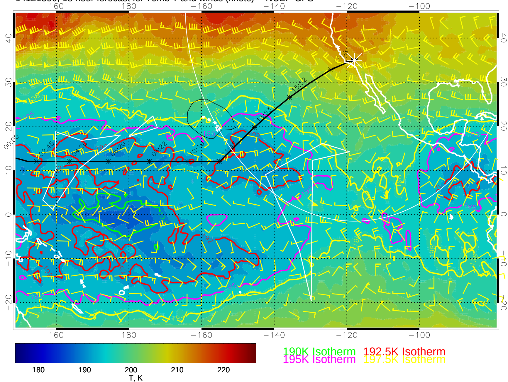
14121306, 18 hour forecast for 70mb T and winds (knots) -- NCEP GFS
