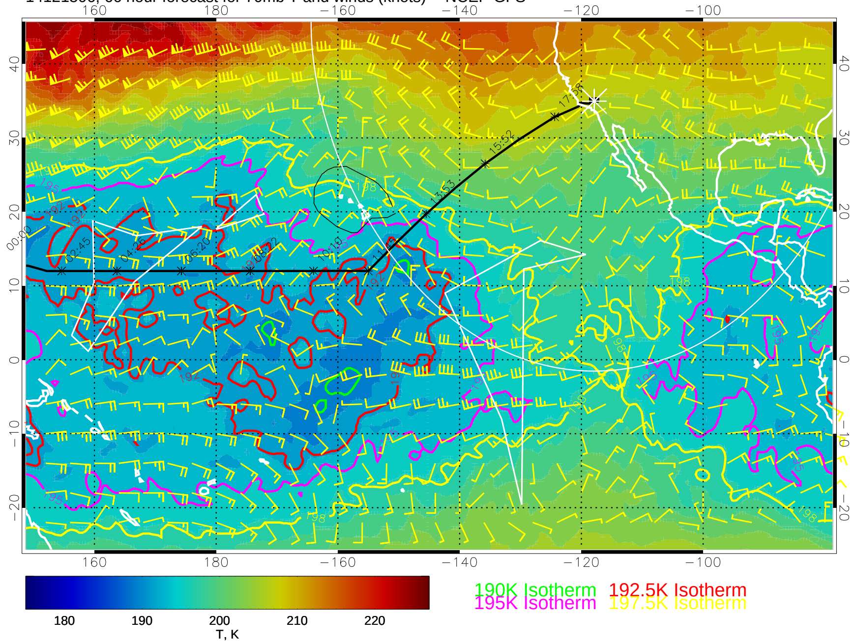
14121506, 66 hour forecast for 70mb T and winds (knots) -- NCEP GFS
