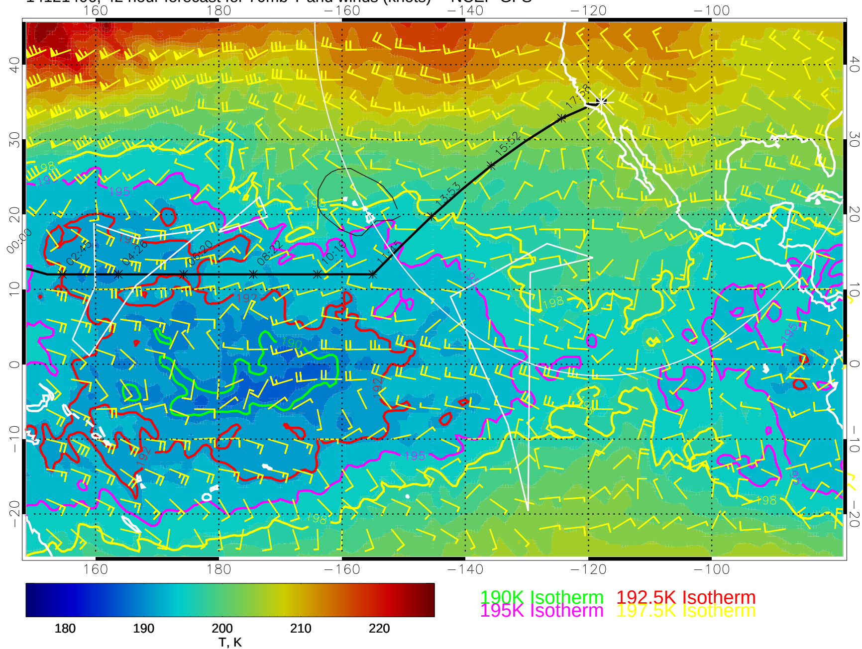
14121406, 42 hour forecast for 70mb T and winds (knots) -- NCEP GFS
