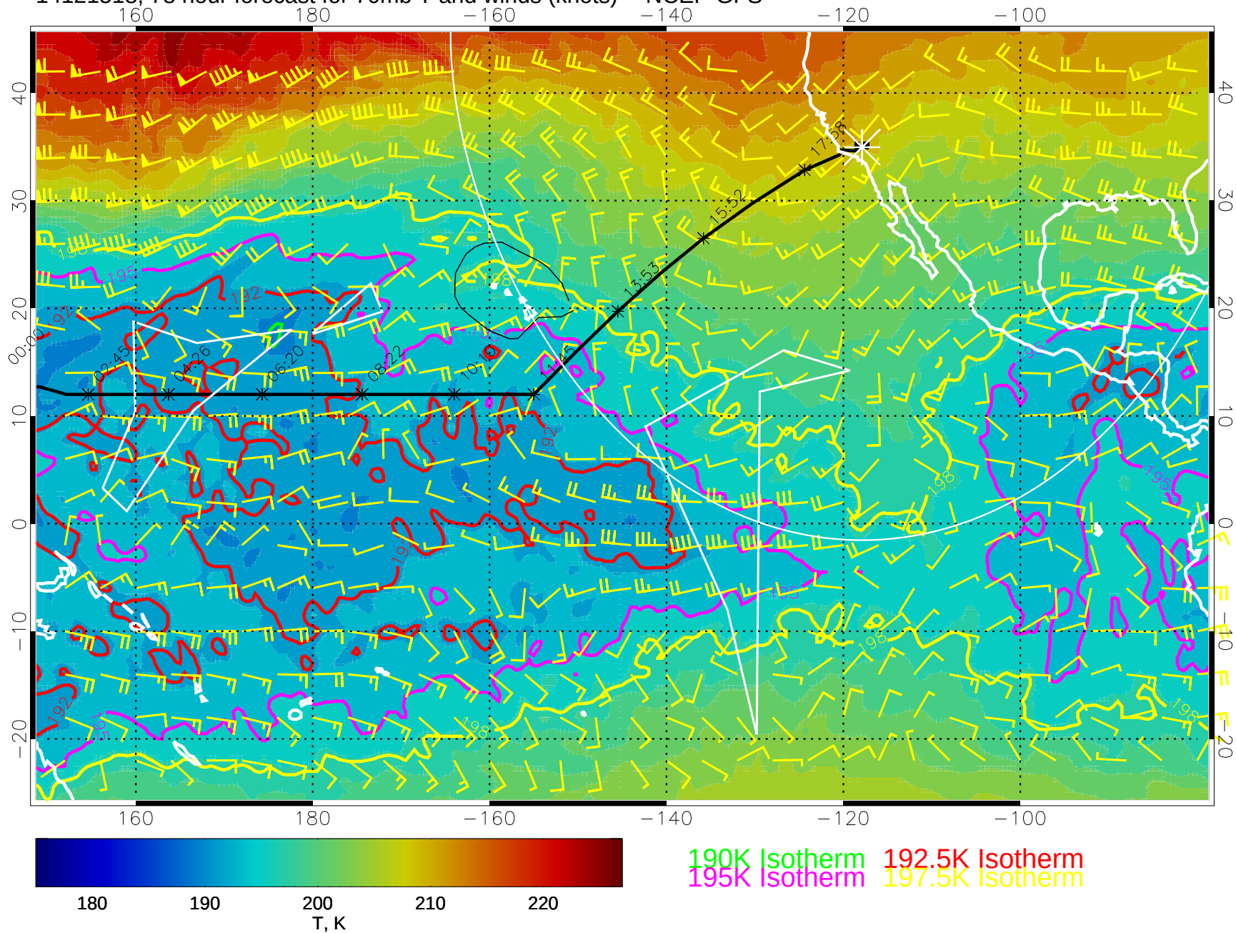
14121518, 78 hour forecast for 70mb T and winds (knots) -- NCEP GFS
