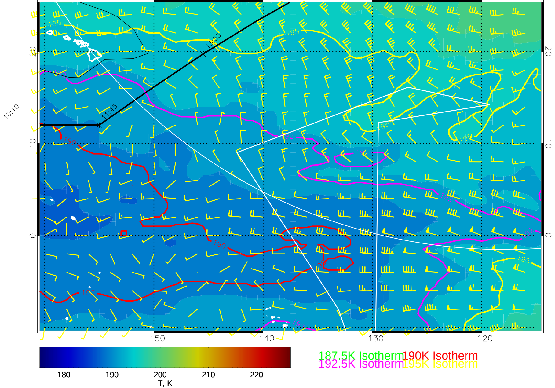
14121300, 12 hour forecast for 100mb T and winds (knots) -- NCEP GFS
