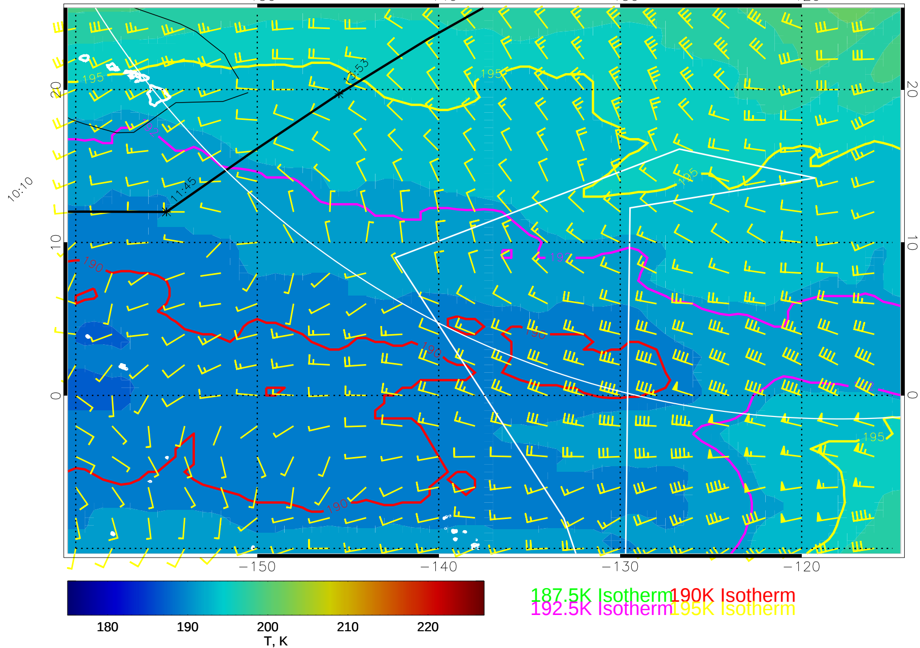
14121306, 18 hour forecast for 100mb T and winds (knots) -- NCEP GFS
