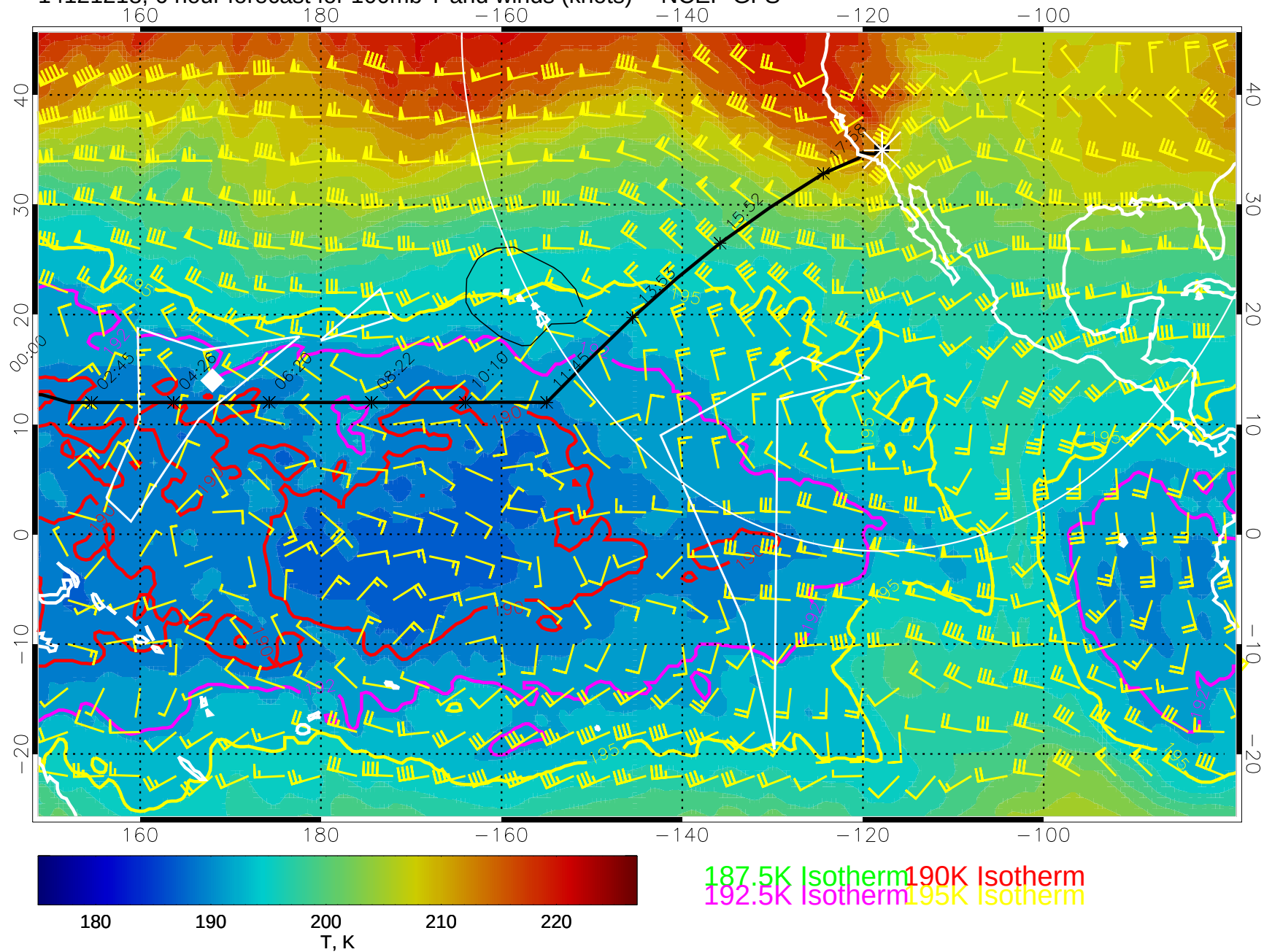
14121218, 6 hour forecast for 100mb T and winds (knots) -- NCEP GFS
