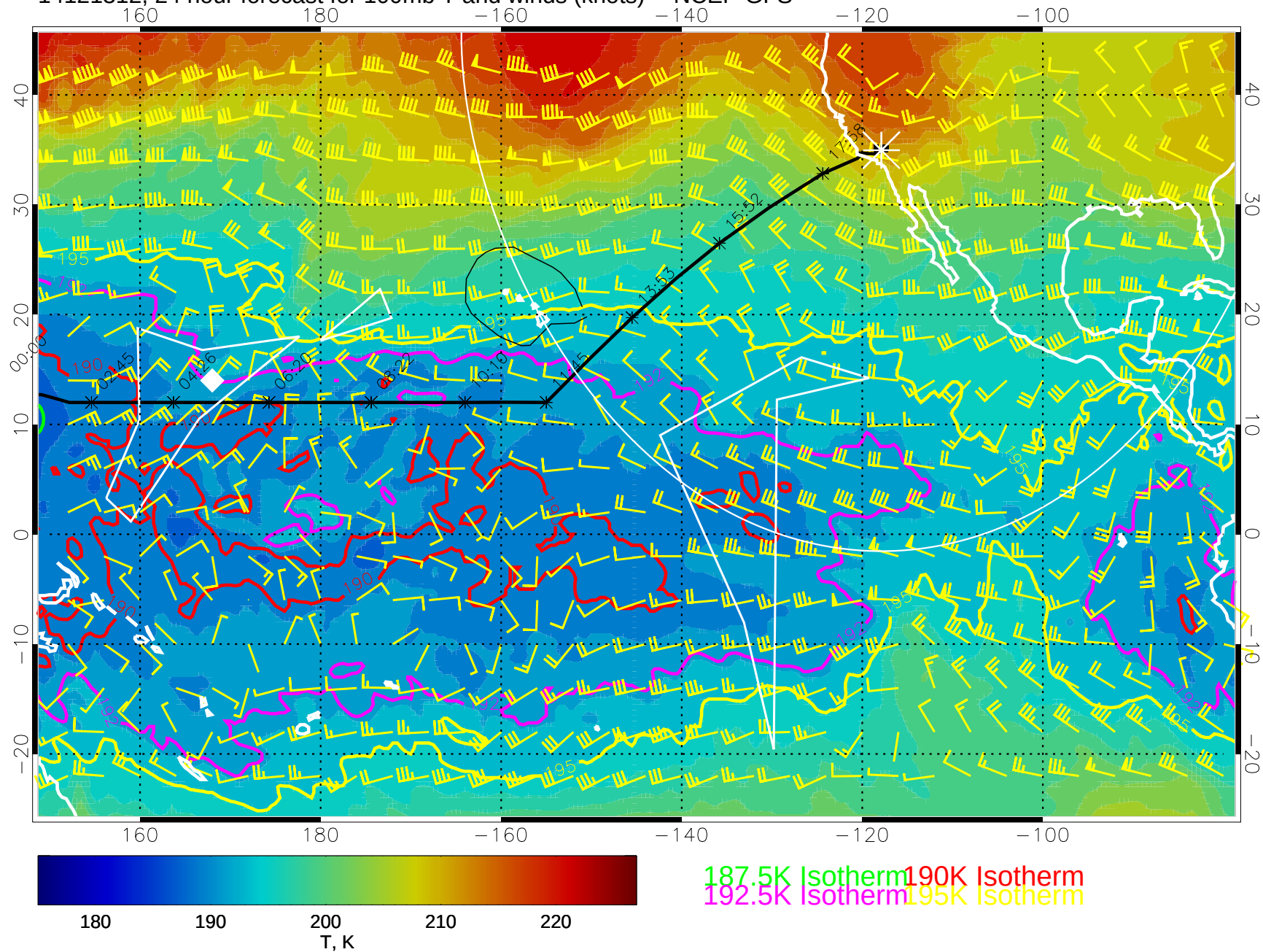
14121312, 24 hour forecast for 100mb T and winds (knots) -- NCEP GFS
