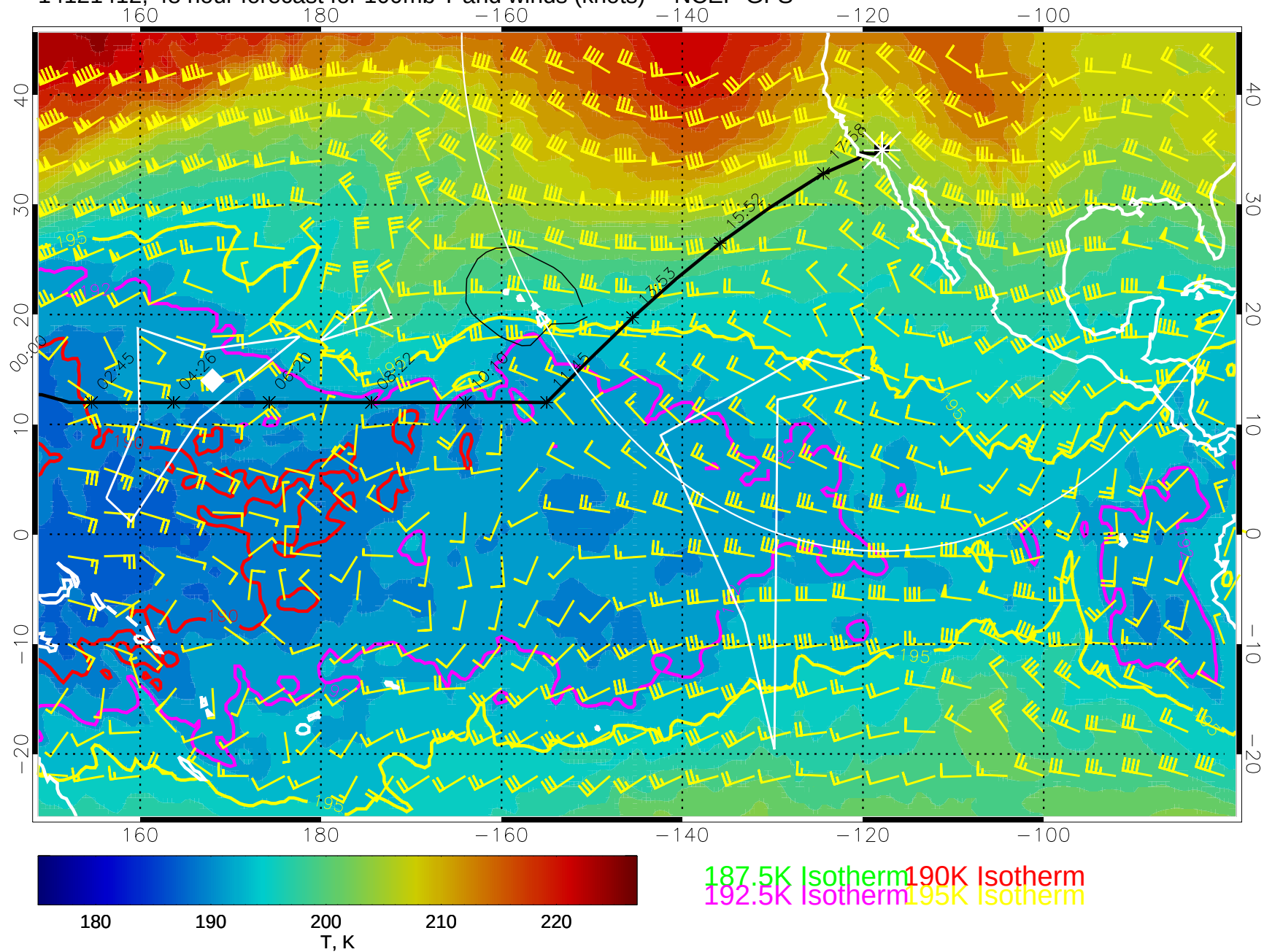
14121412, 48 hour forecast for 100mb T and winds (knots) -- NCEP GFS
