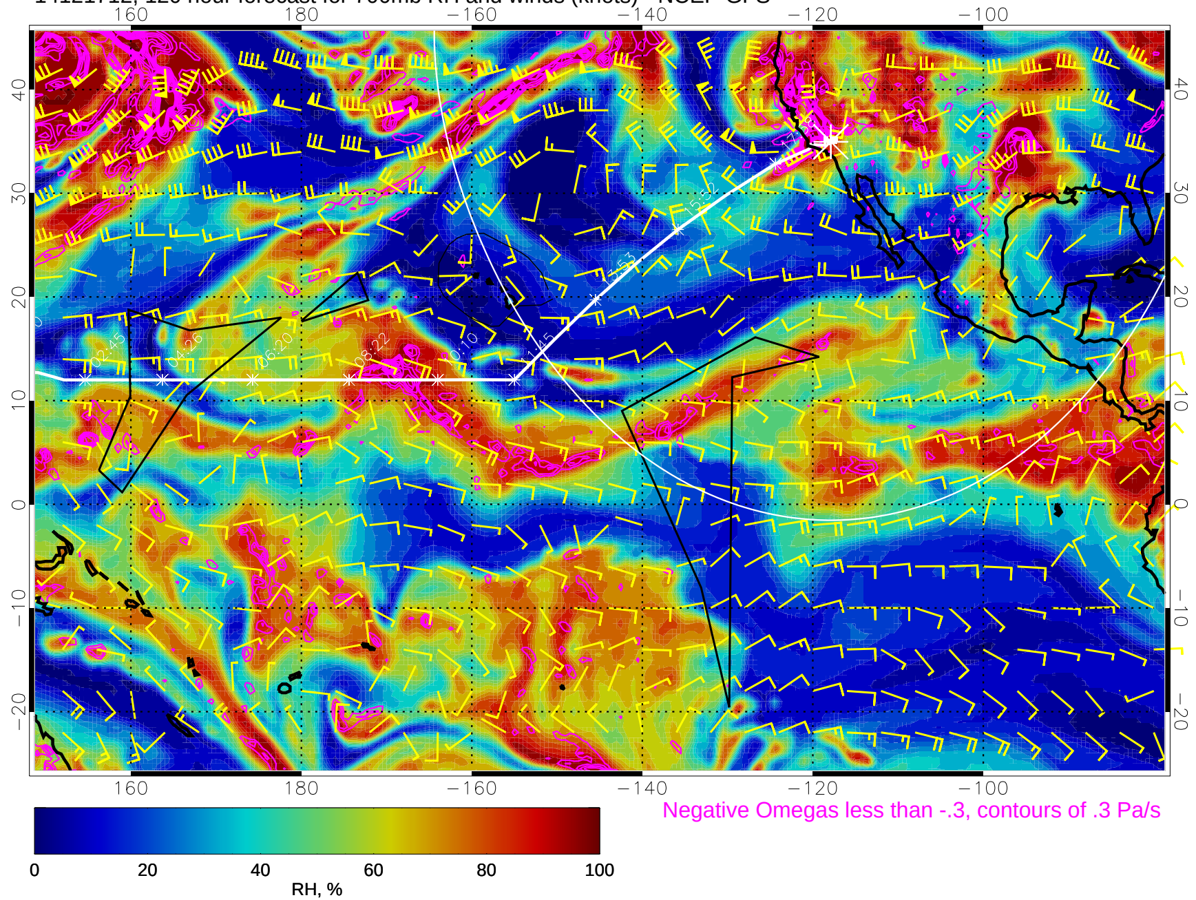
14121712, 120 hour forecast for 700mb RH and winds (knots) - NCEP GFS
