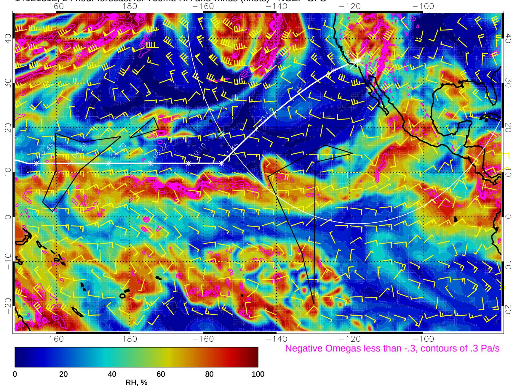
14121312, 24 hour forecast for 700mb RH and winds (knots) - NCEP GFS
