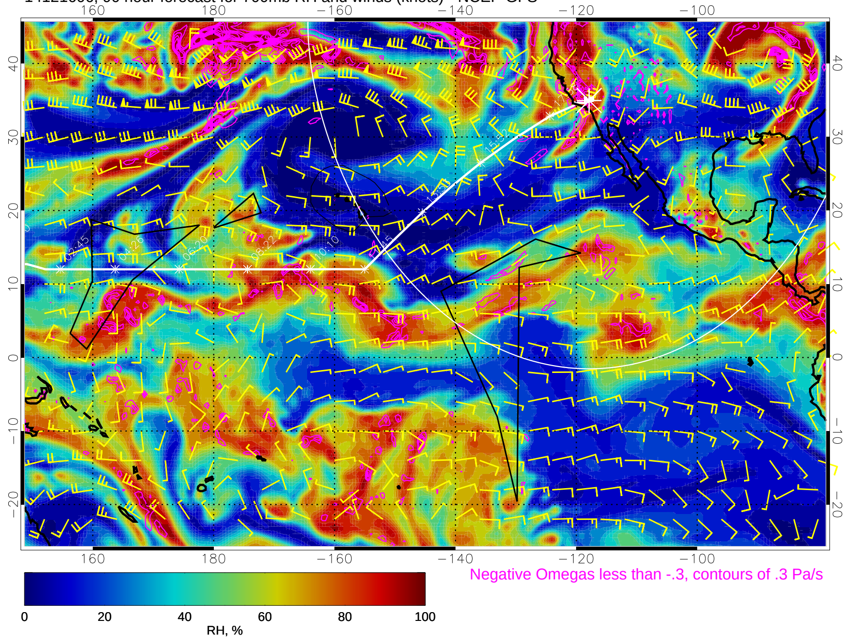
14121606, 90 hour forecast for 700mb RH and winds (knots) - NCEP GFS
