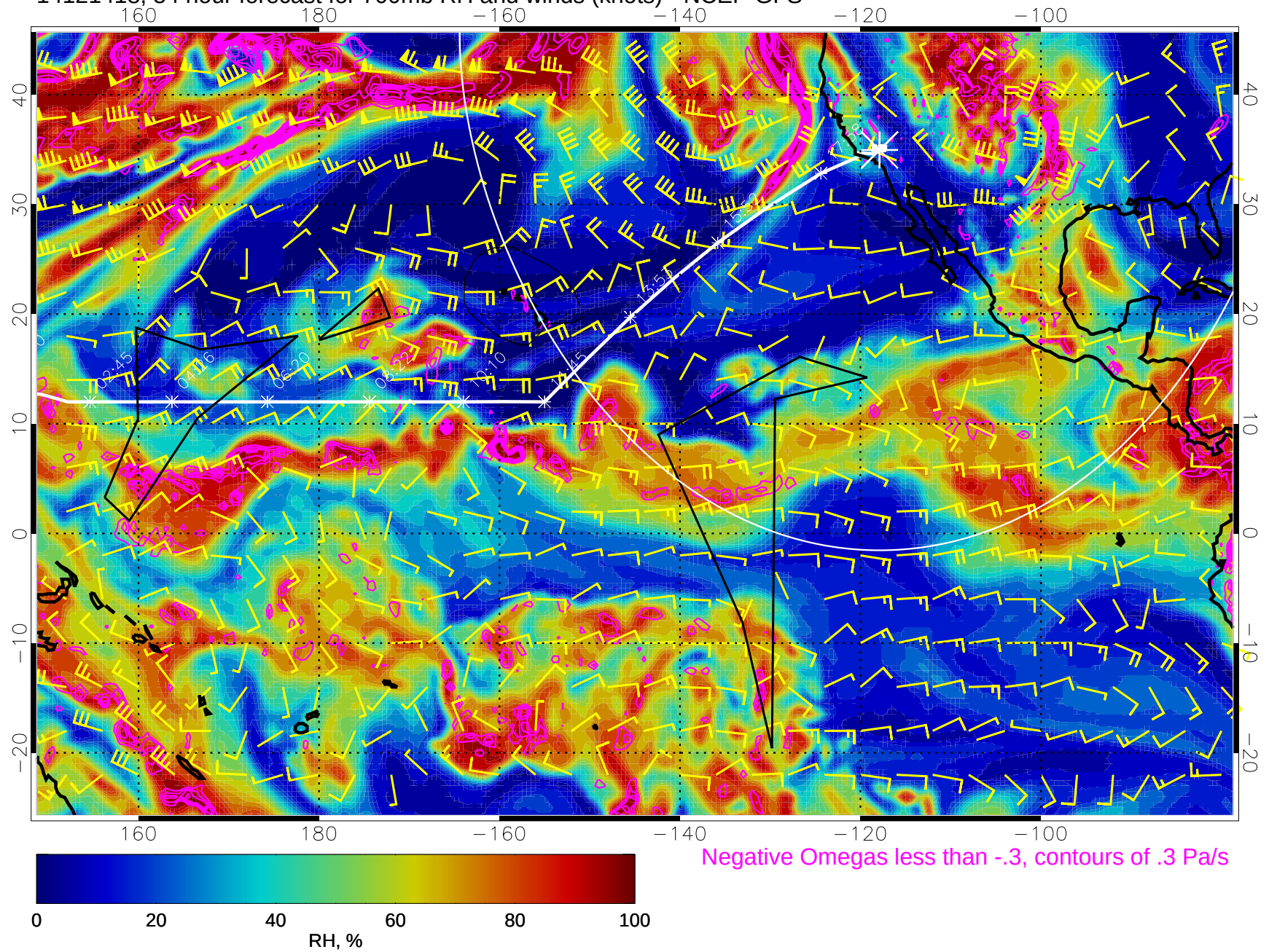
14121418, 54 hour forecast for 700mb RH and winds (knots) - NCEP GFS
