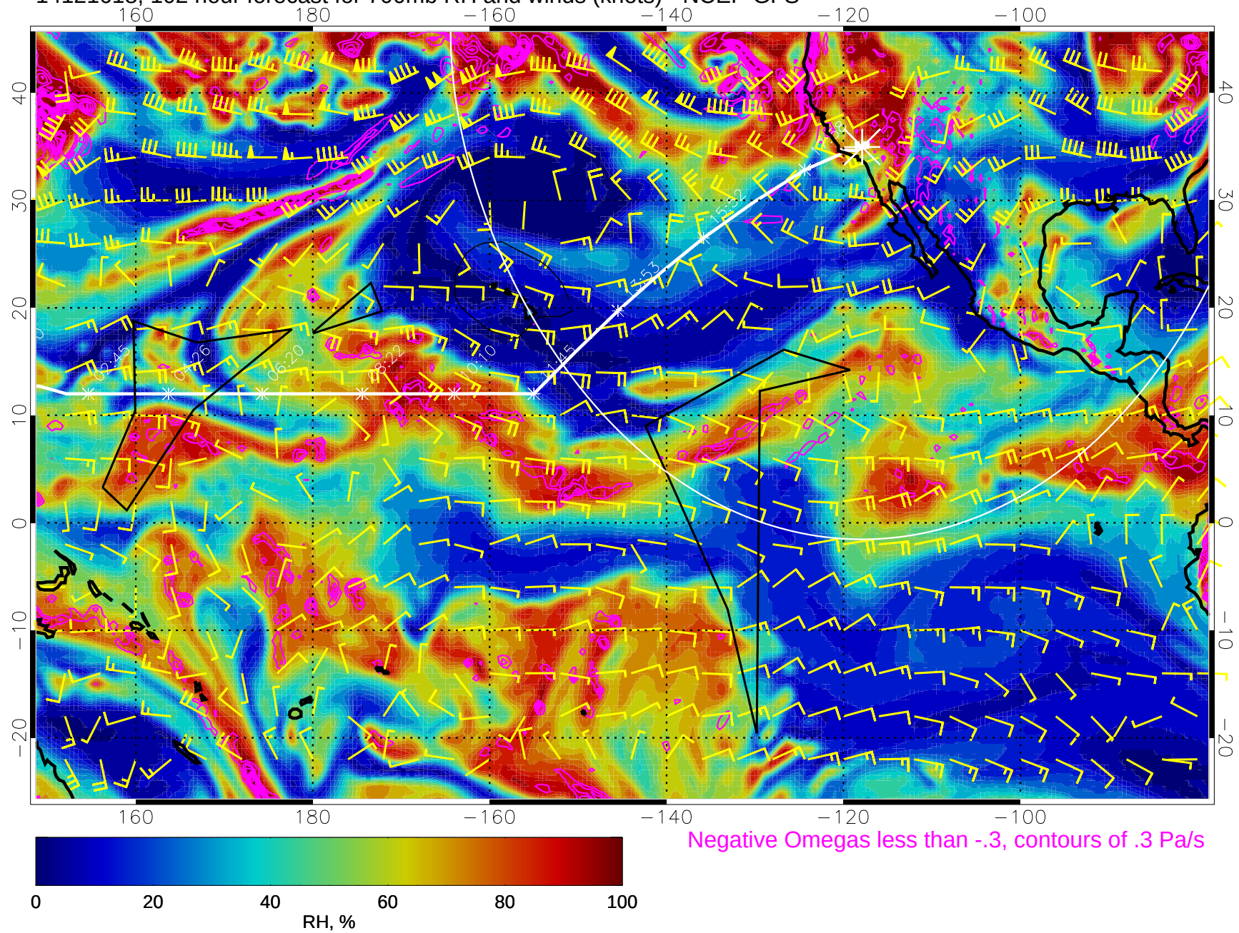
14121618, 102 hour forecast for 700mb RH and winds (knots) - NCEP GFS
