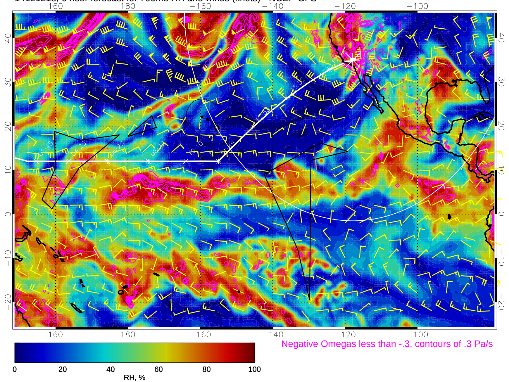
14121218, 6 hour forecast for 700mb RH and winds (knots) - NCEP GFS
