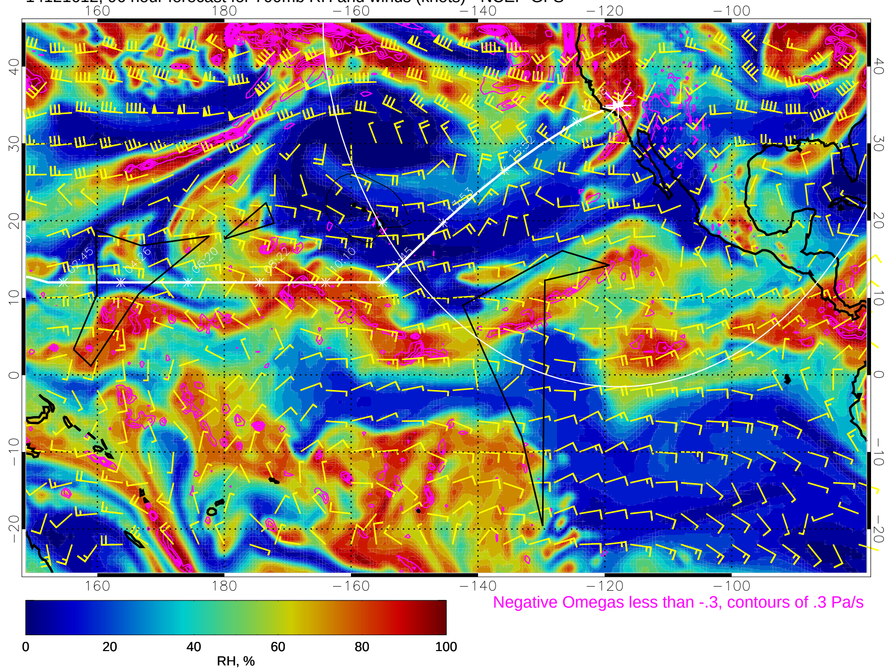
14121612, 96 hour forecast for 700mb RH and winds (knots) - NCEP GFS
