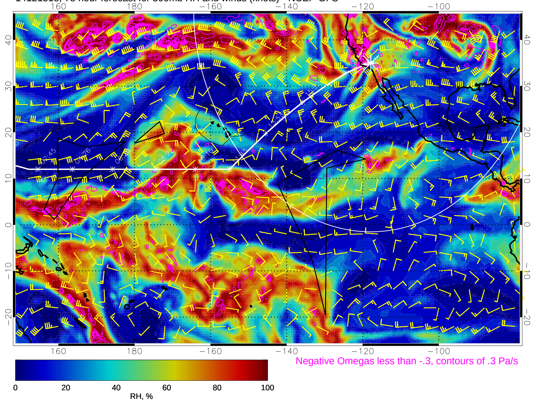
14121518, 78 hour forecast for 500mb RH and winds (knots) - NCEP GFS
