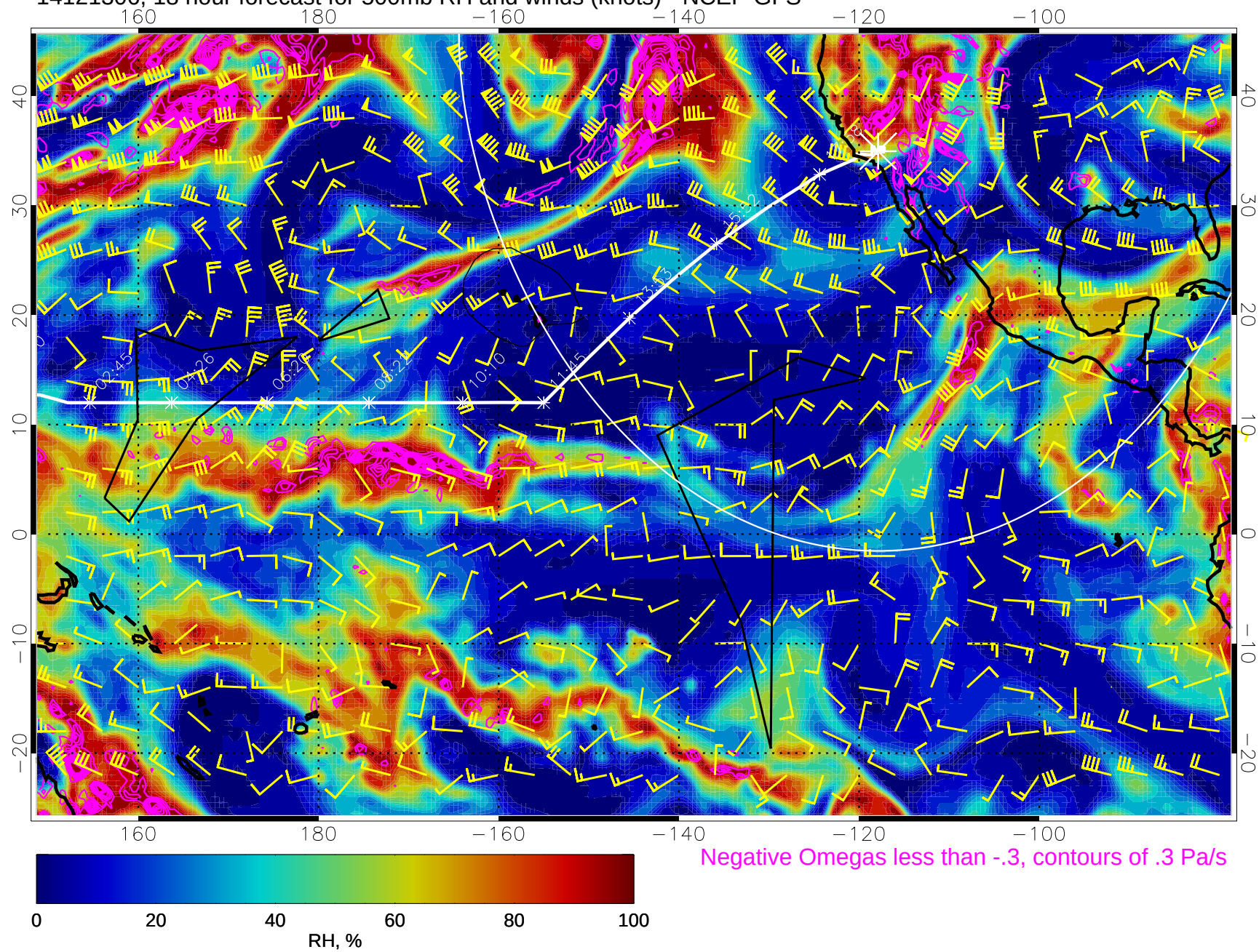
14121306, 18 hour forecast for 500mb RH and winds (knots) - NCEP GFS
