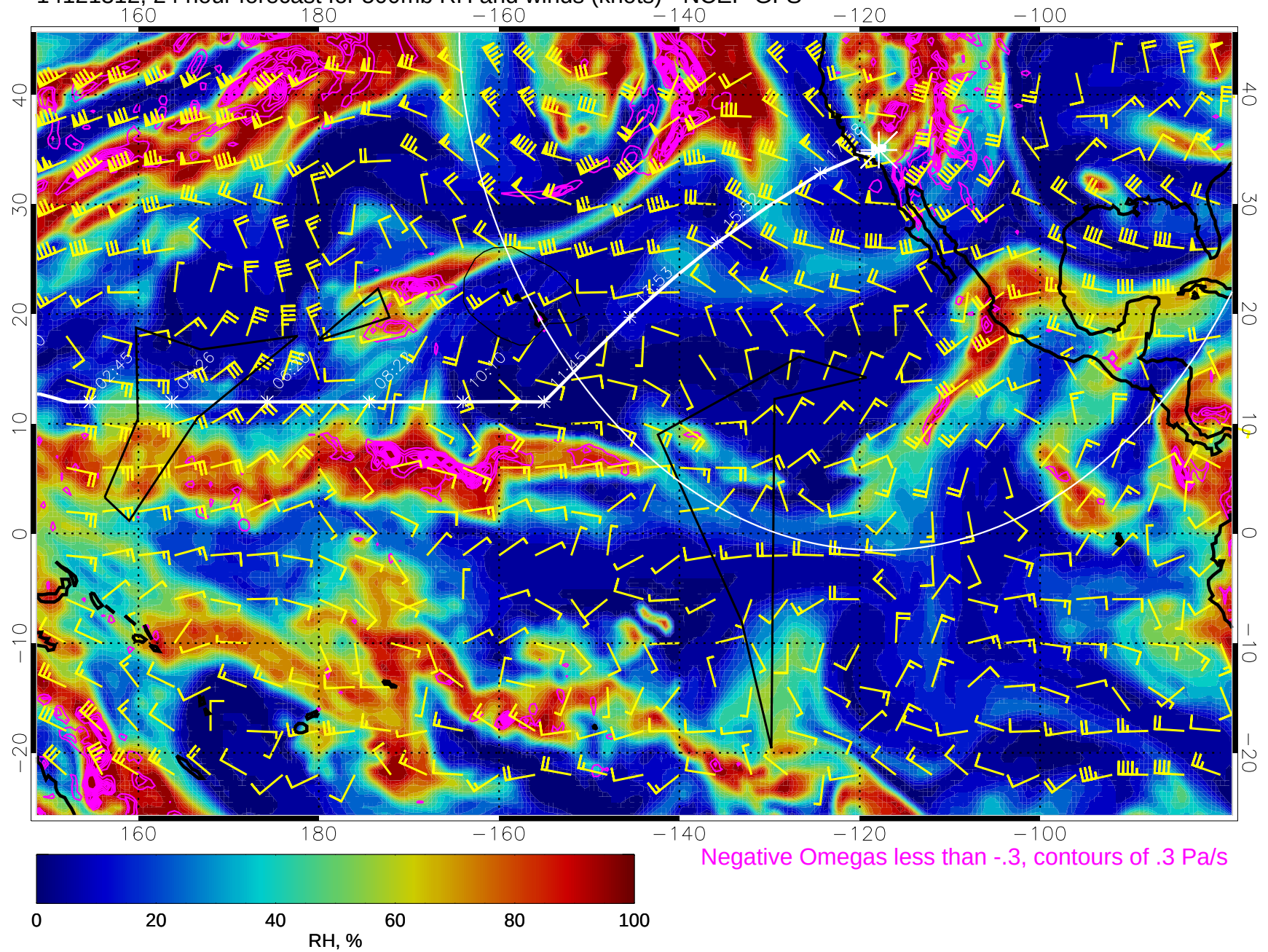
14121312, 24 hour forecast for 500mb RH and winds (knots) - NCEP GFS
