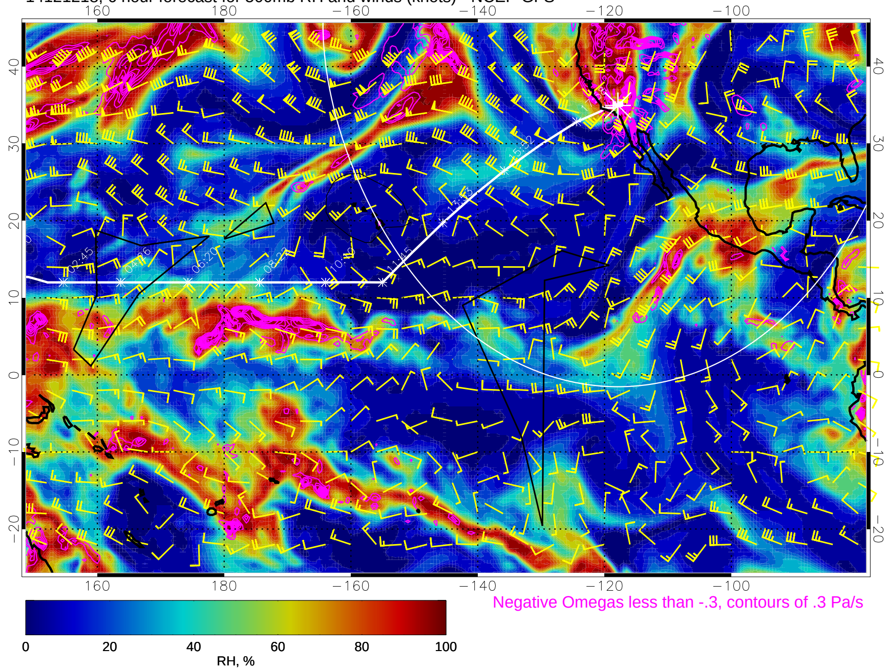
14121218, 6 hour forecast for 500mb RH and winds (knots) - NCEP GFS
