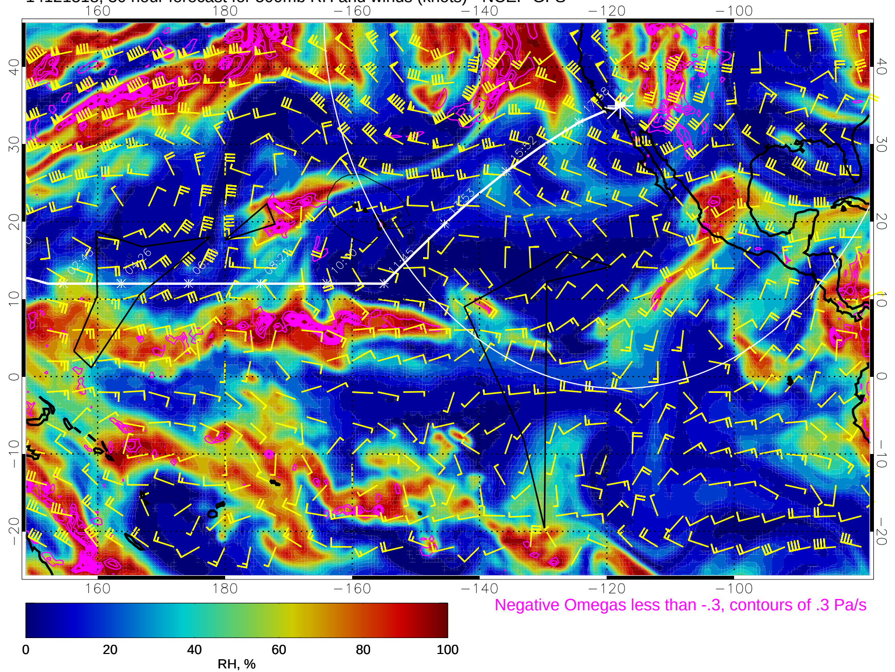
14121318, 30 hour forecast for 500mb RH and winds (knots) - NCEP GFS
