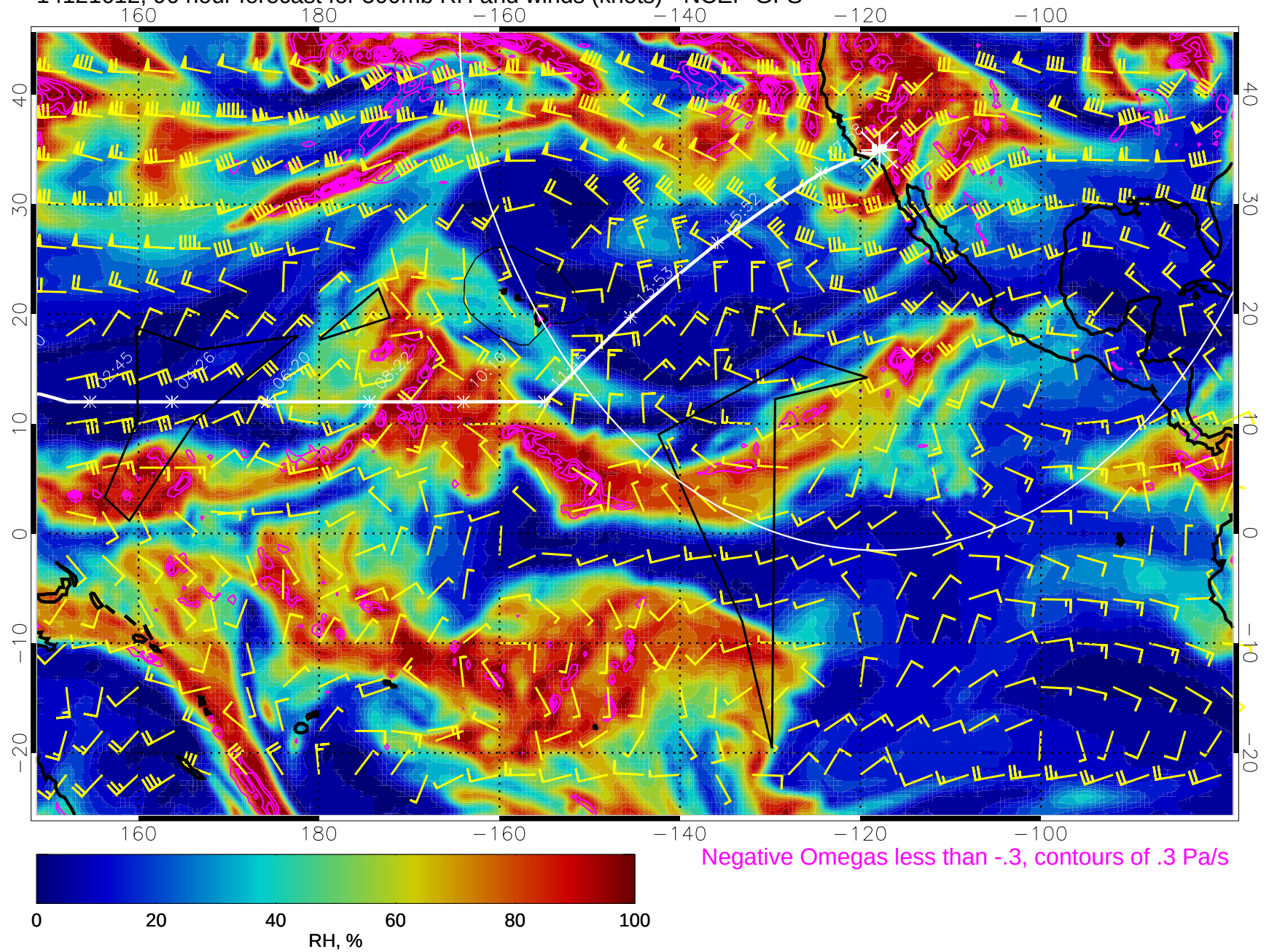
14121612, 96 hour forecast for 500mb RH and winds (knots) - NCEP GFS
