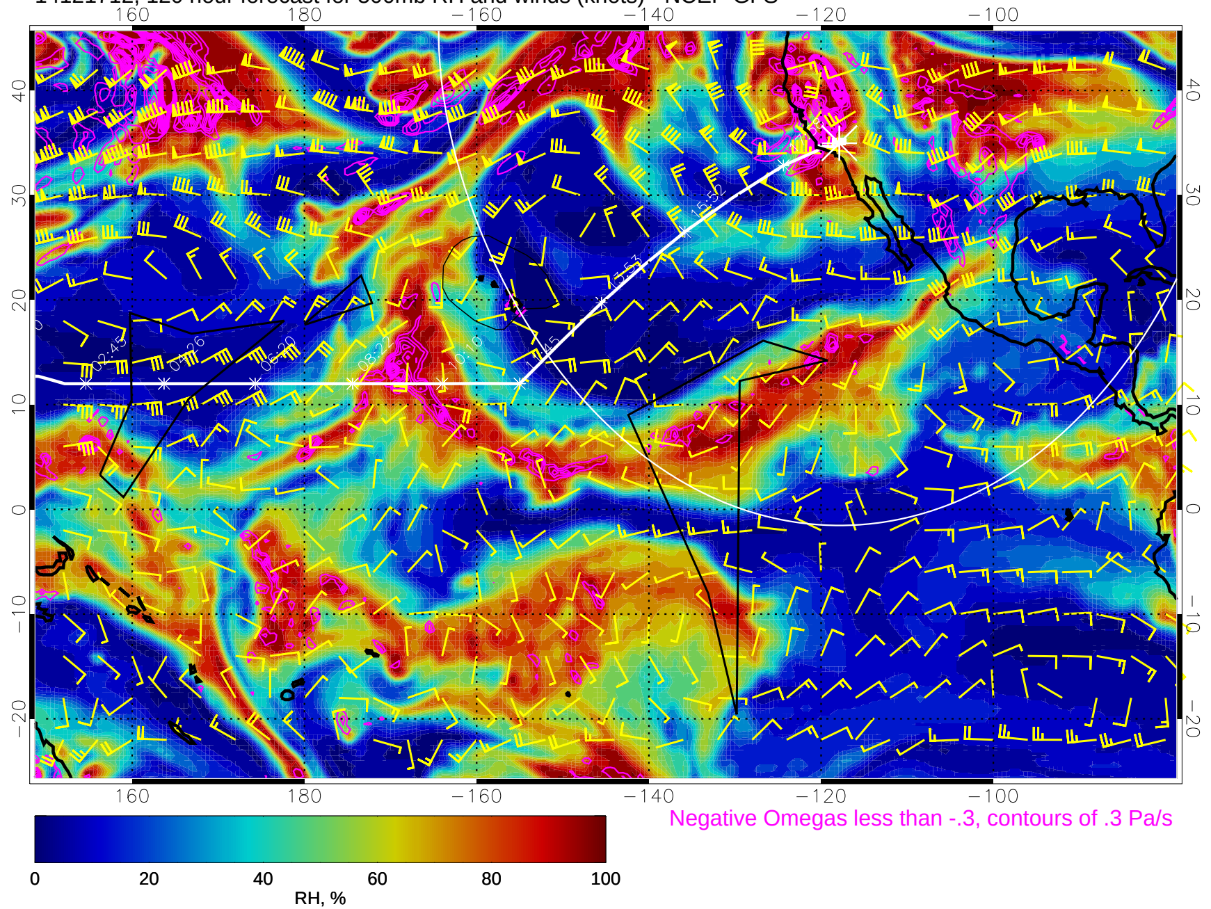
14121712, 120 hour forecast for 500mb RH and winds (knots) - NCEP GFS
