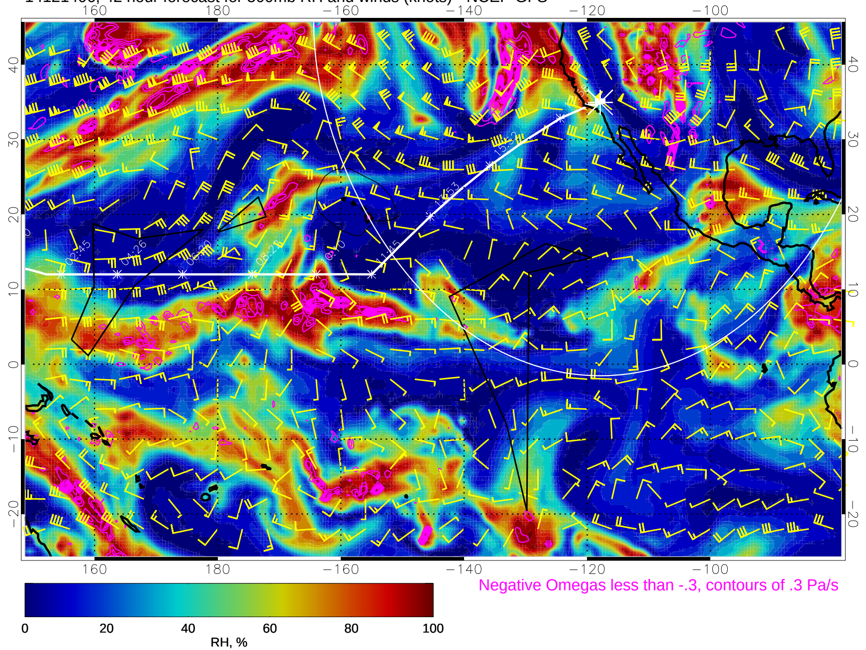
14121406, 42 hour forecast for 500mb RH and winds (knots) - NCEP GFS
