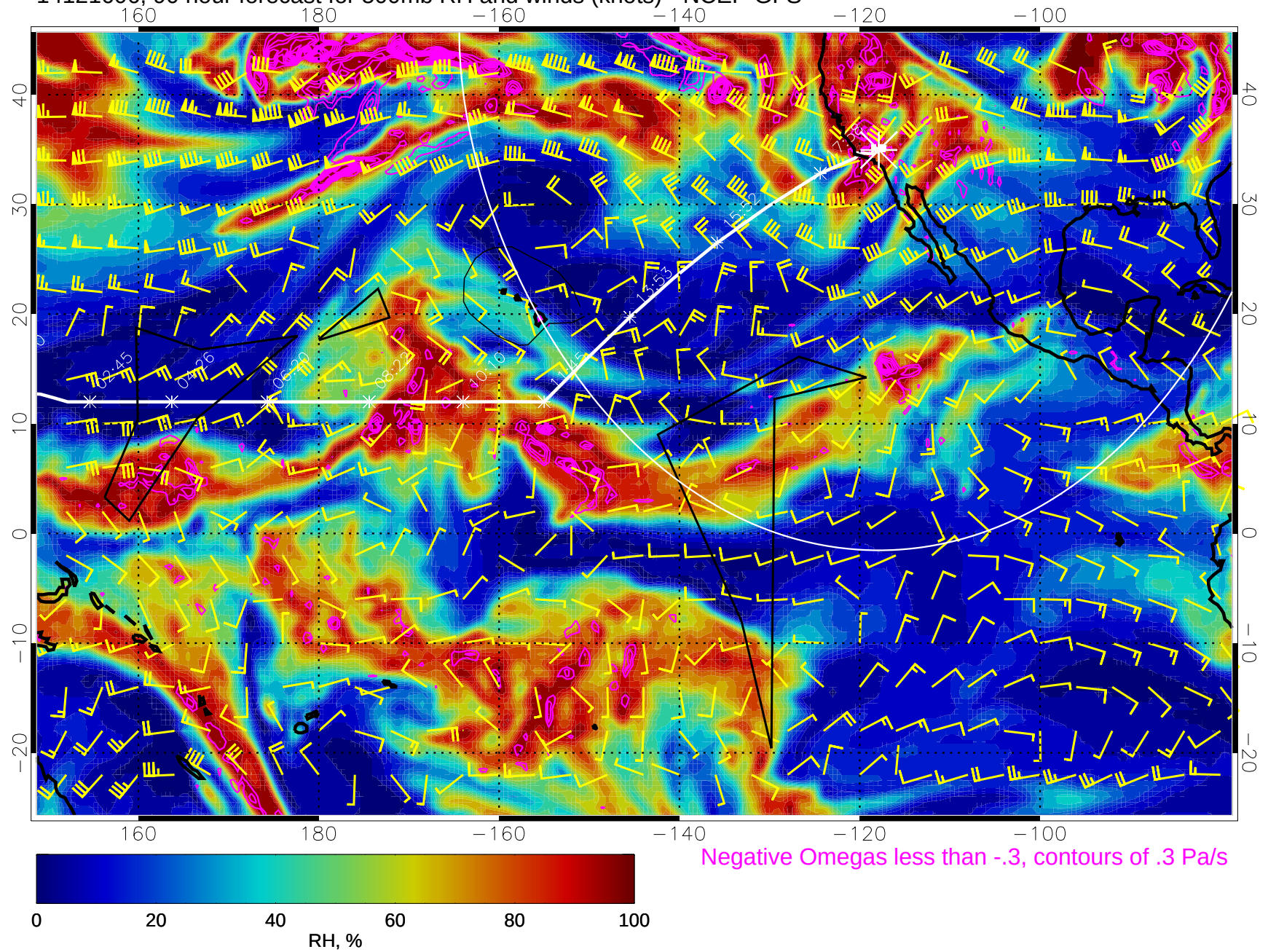
14121606, 90 hour forecast for 500mb RH and winds (knots) - NCEP GFS
