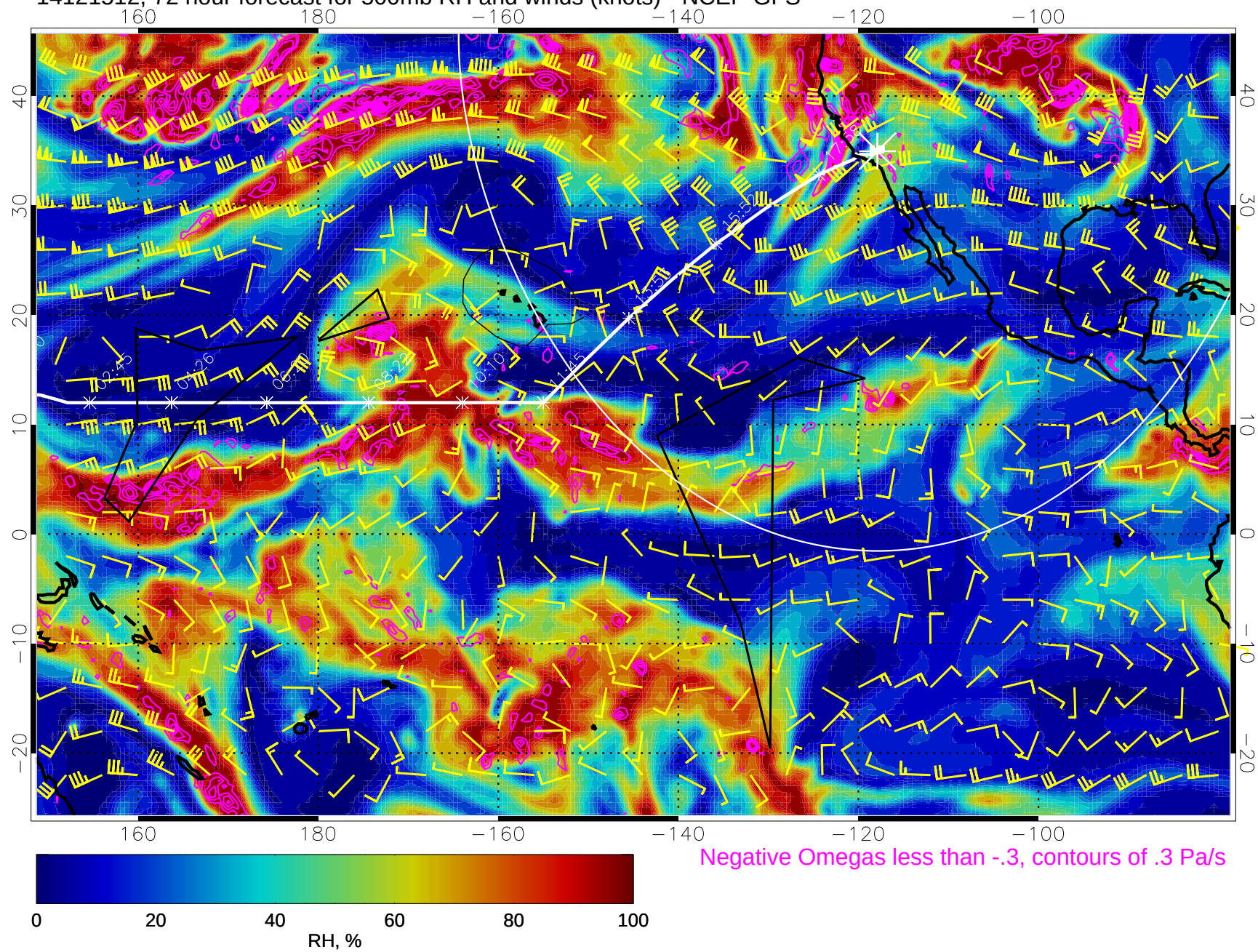
14121512, 72 hour forecast for 500mb RH and winds (knots) - NCEP GFS
