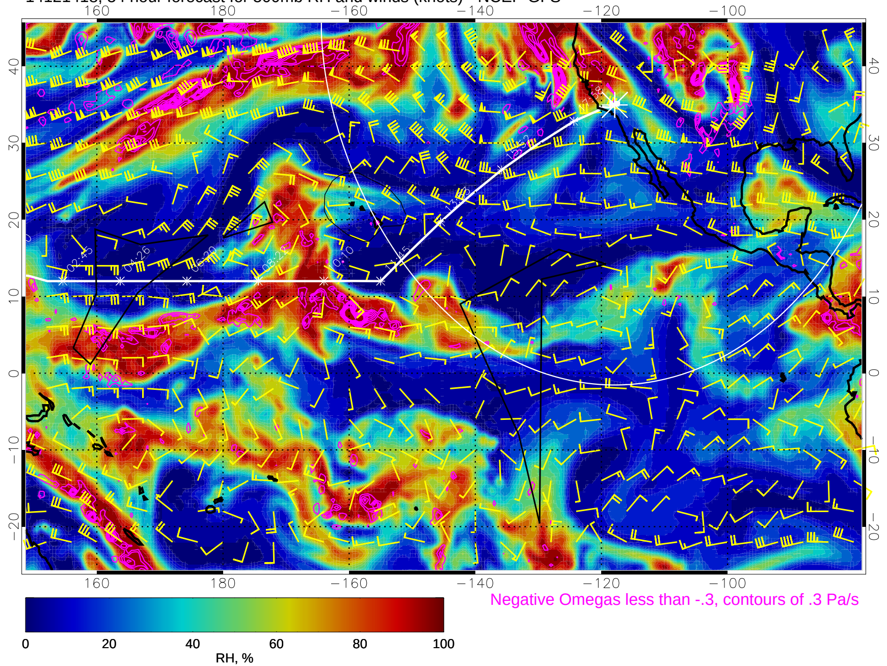
14121418, 54 hour forecast for 500mb RH and winds (knots) - NCEP GFS
