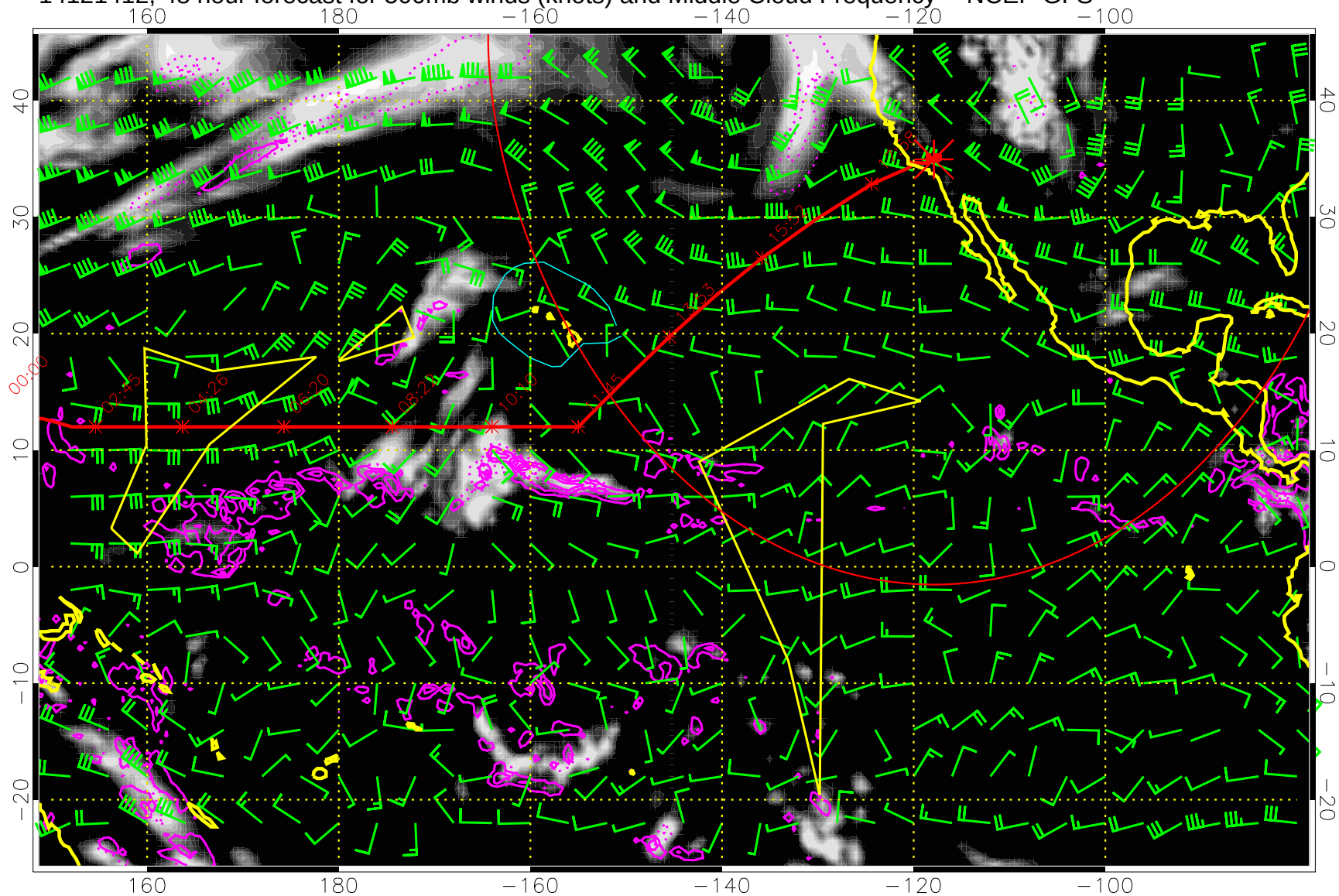
14121412, 48 hour forecast for 500mb winds (knots) and Middle Cloud Frequency -- NCEP GFS
