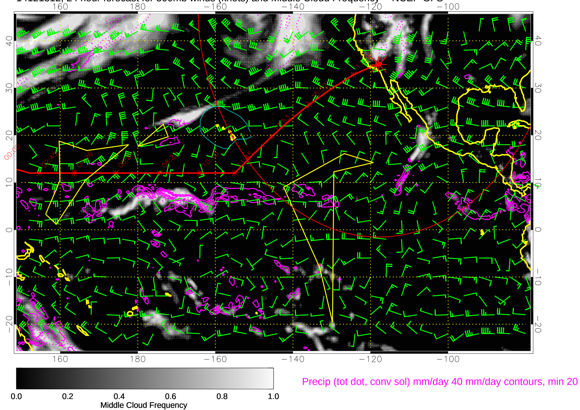
14121312, 24 hour forecast for 500mb winds (knots) and Middle Cloud Frequency -- NCEP GFS
