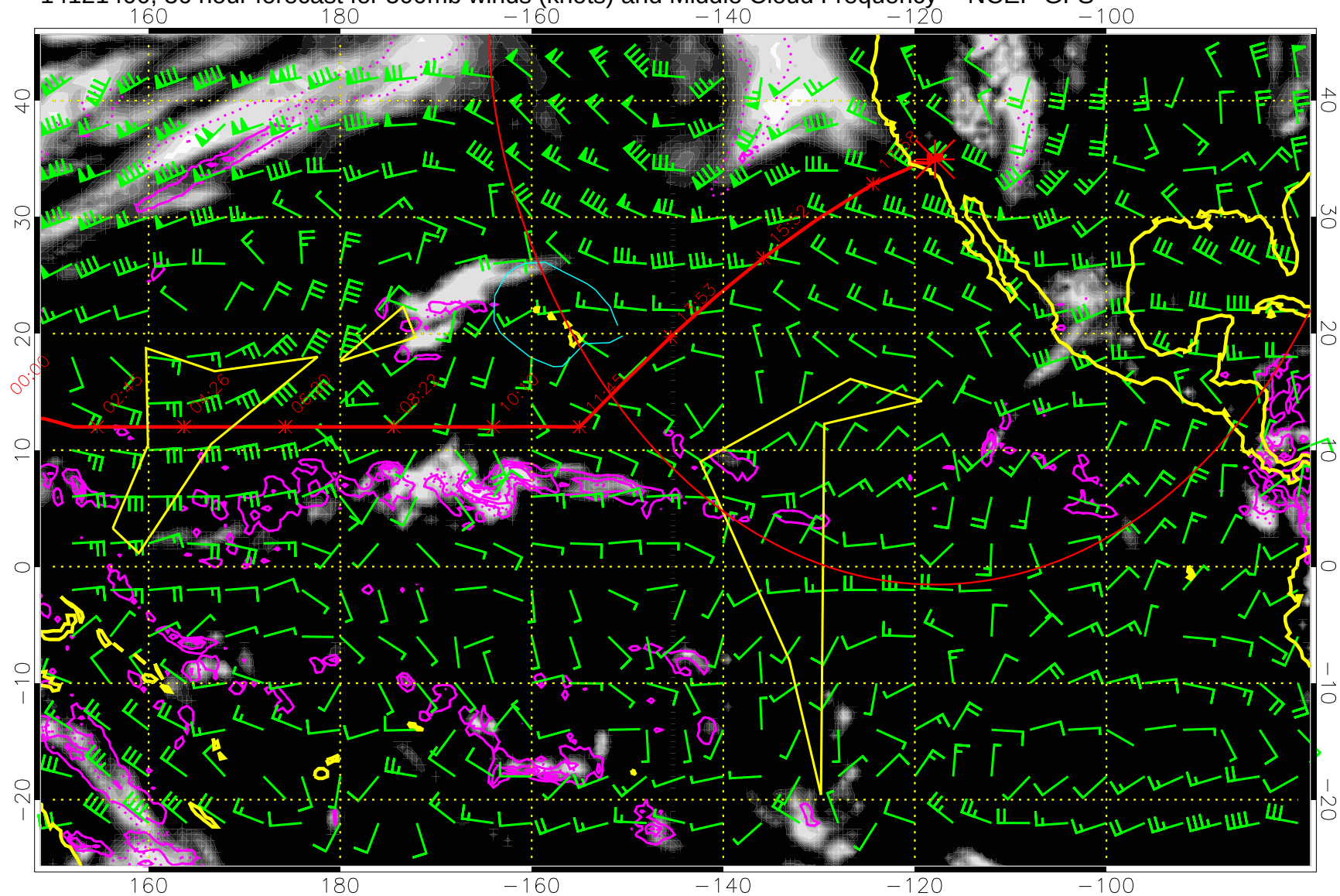
14121400, 36 hour forecast for 500mb winds (knots) and Middle Cloud Frequency -- NCEP GFS
