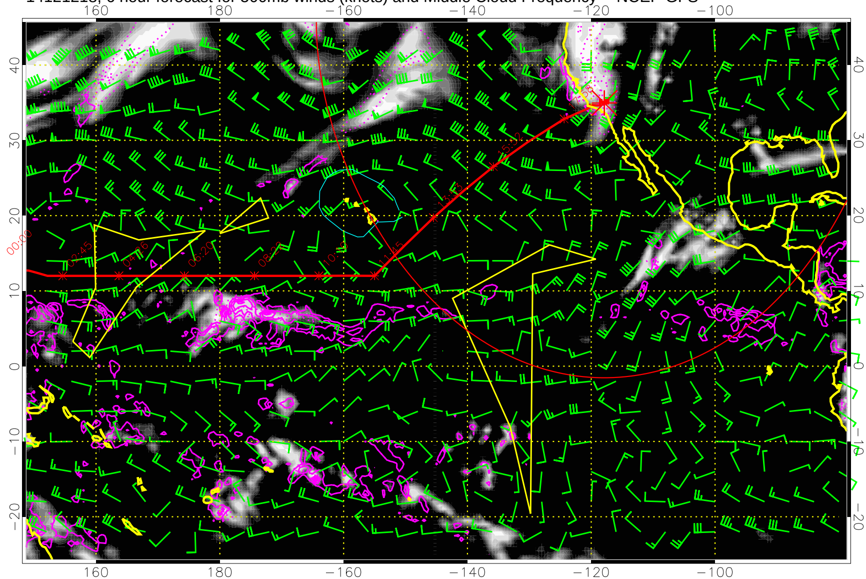
14121218, 6 hour forecast for 500mb winds (knots) and Middle Cloud Frequency -- NCEP GFS
