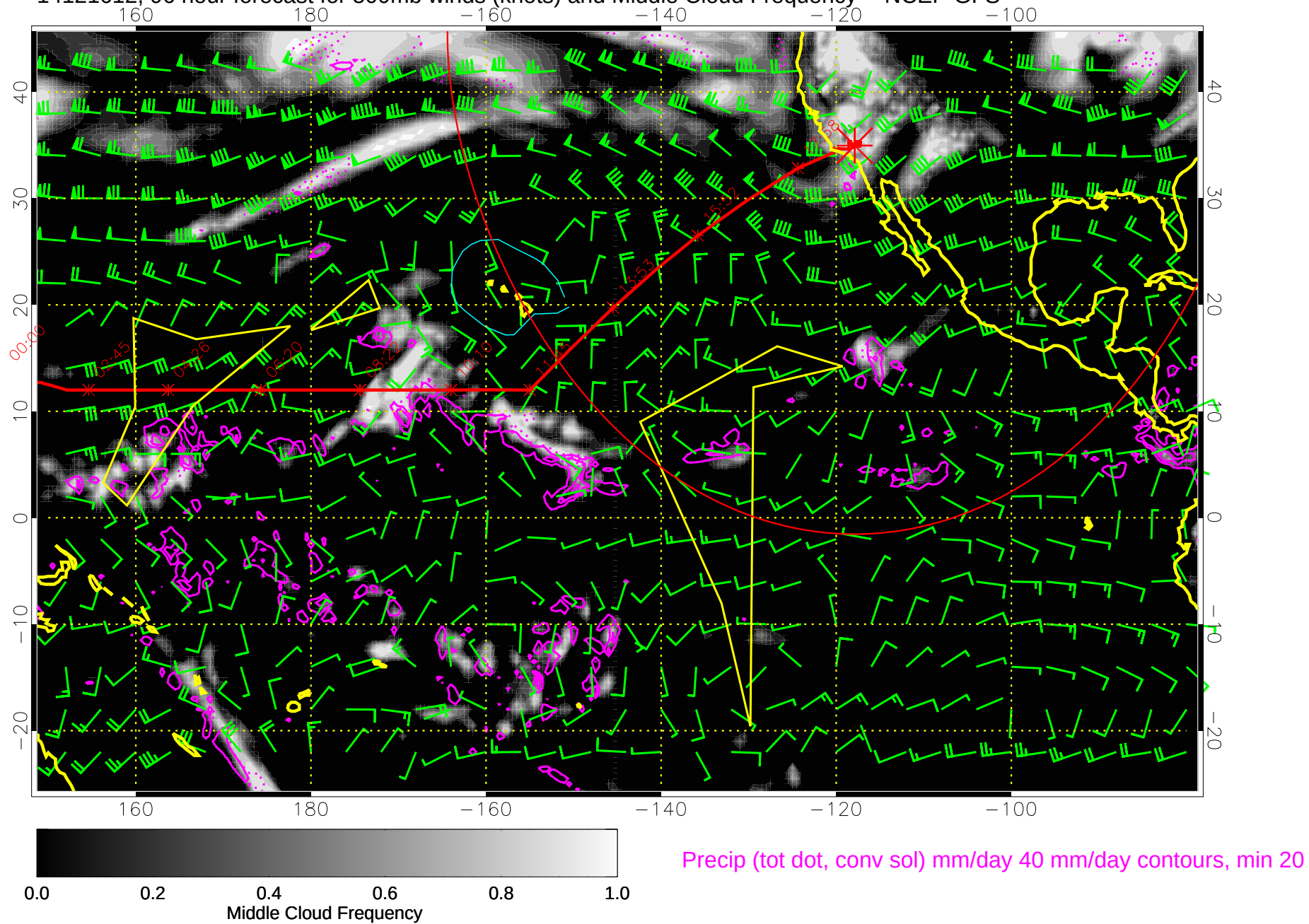
14121612, 96 hour forecast for 500mb winds (knots) and Middle Cloud Frequency -- NCEP GFS
