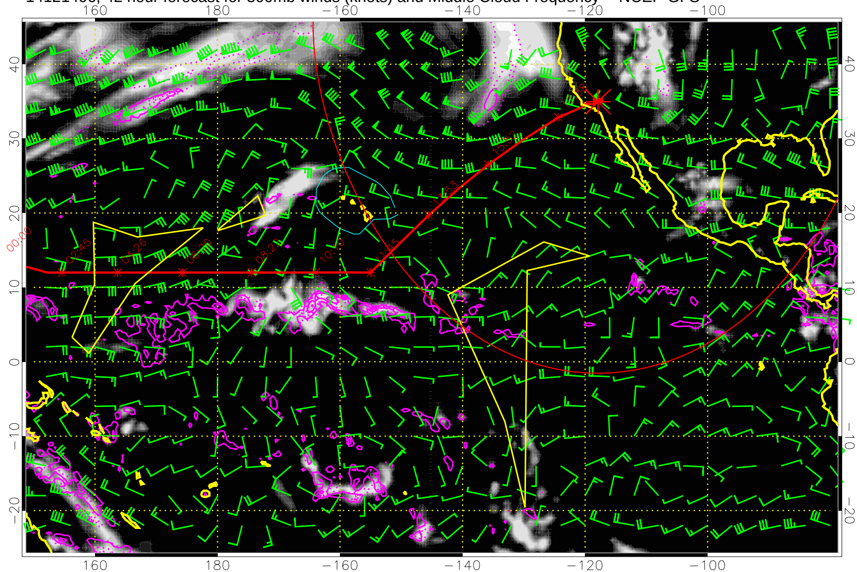
14121406, 42 hour forecast for 500mb winds (knots) and Middle Cloud Frequency -- NCEP GFS
