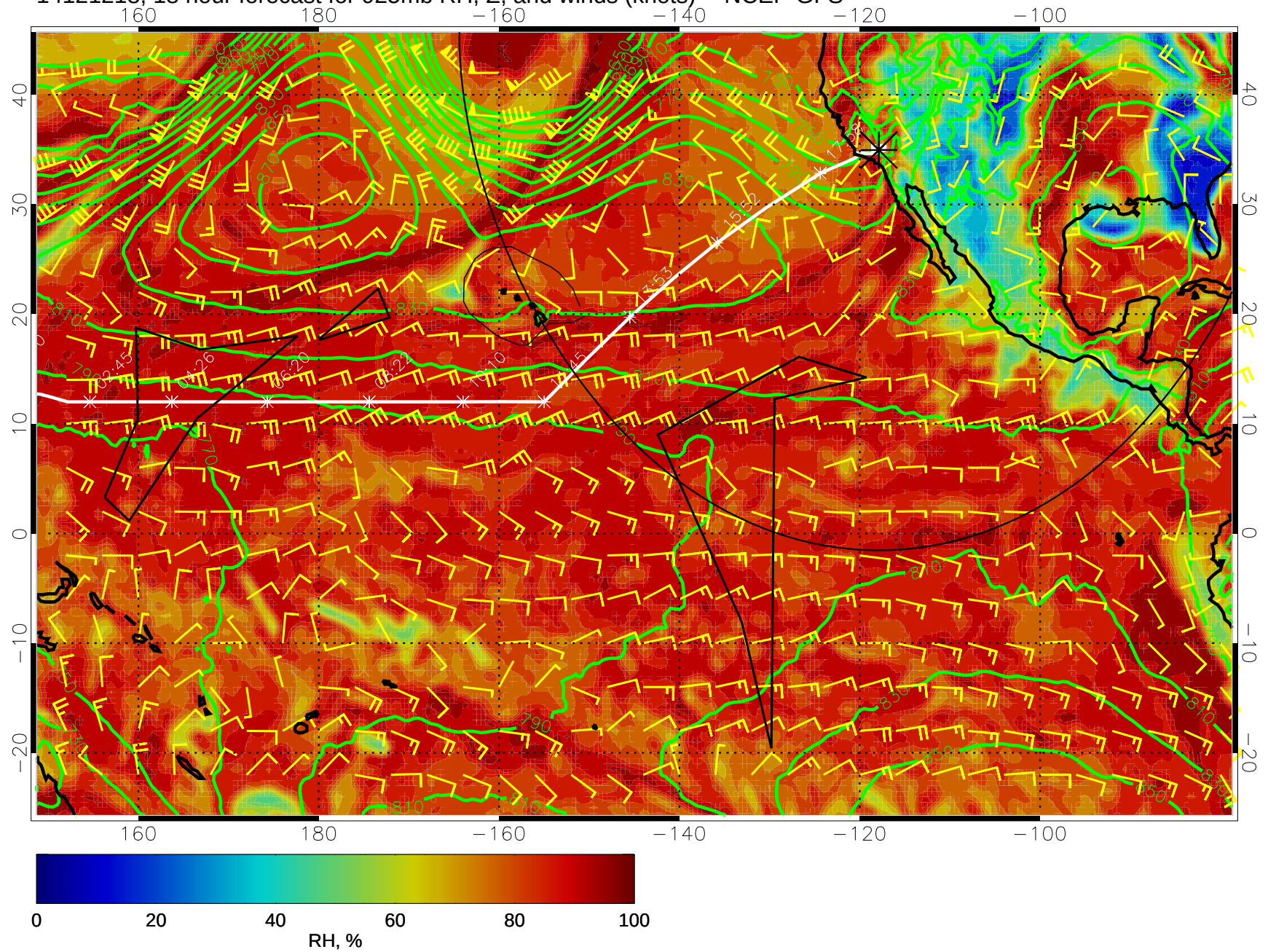
14121218, 18 hour forecast for 925mb RH, Z, and winds (knots) -- NCEP GFS
