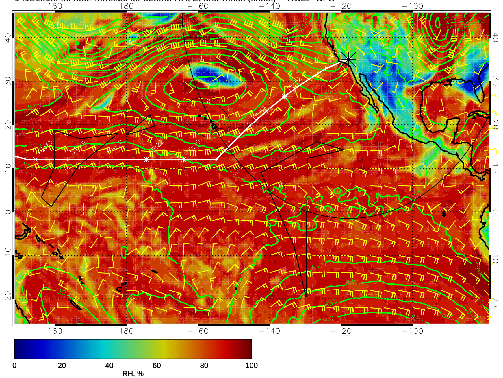
14121518, 90 hour forecast for 925mb RH, Z, and winds (knots) -- NCEP GFS
