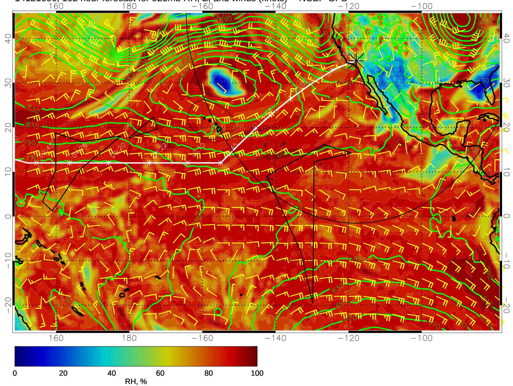
14121606, 102 hour forecast for 925mb RH, Z, and winds (knots) -- NCEP GFS
