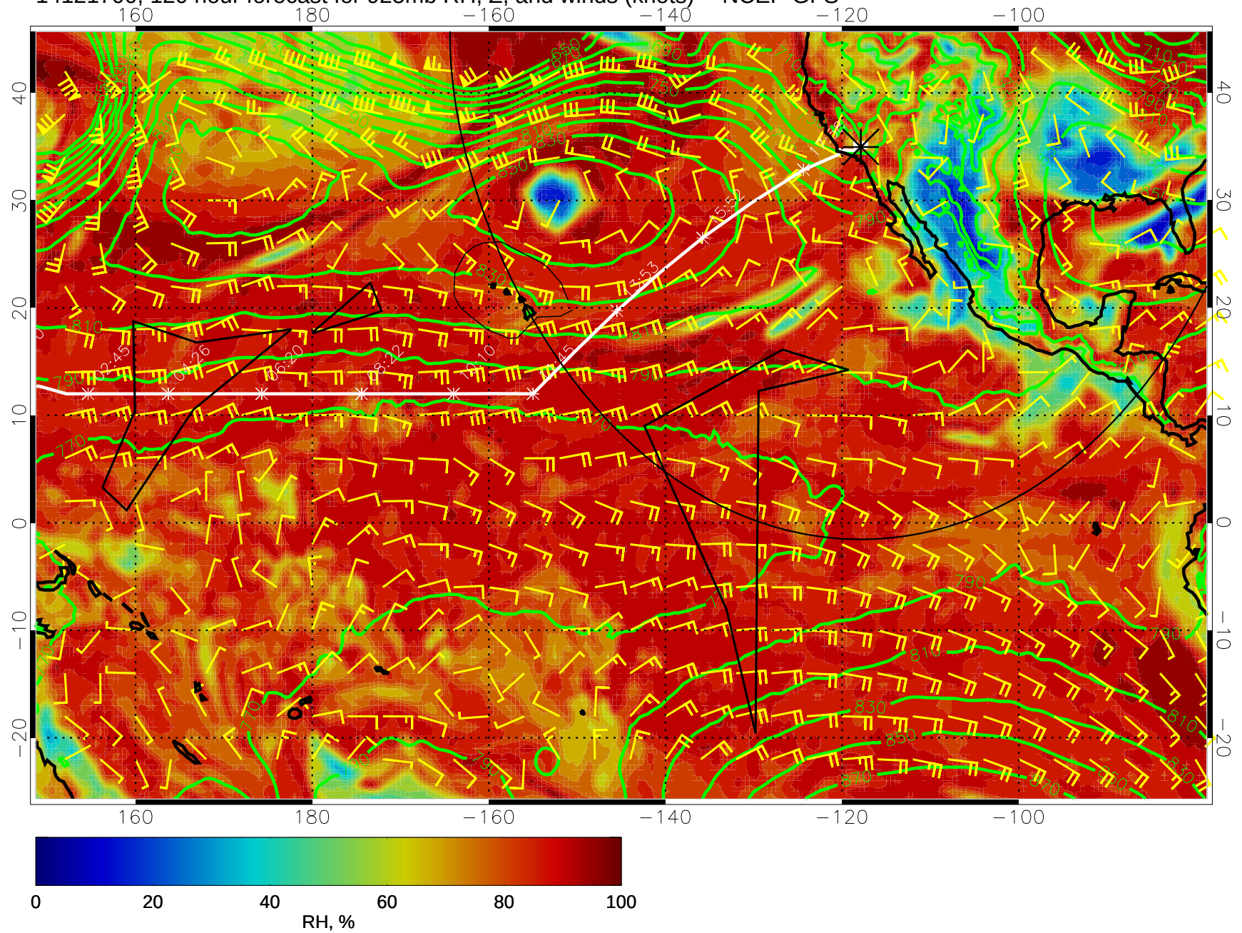
14121700, 120 hour forecast for 925mb RH, Z, and winds (knots) -- NCEP GFS
