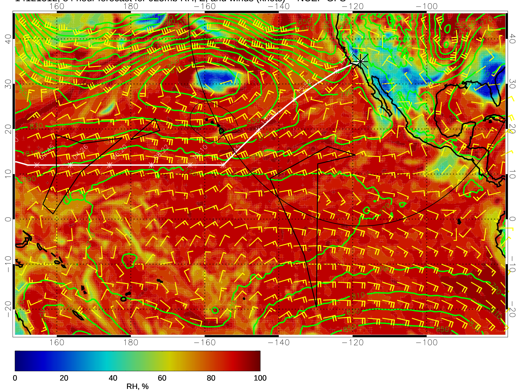
14121512, 84 hour forecast for 925mb RH, Z, and winds (knots) -- NCEP GFS
