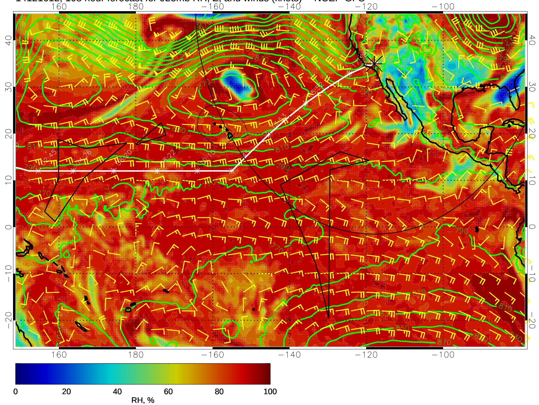
14121612, 108 hour forecast for 925mb RH, Z, and winds (knots) -- NCEP GFS
