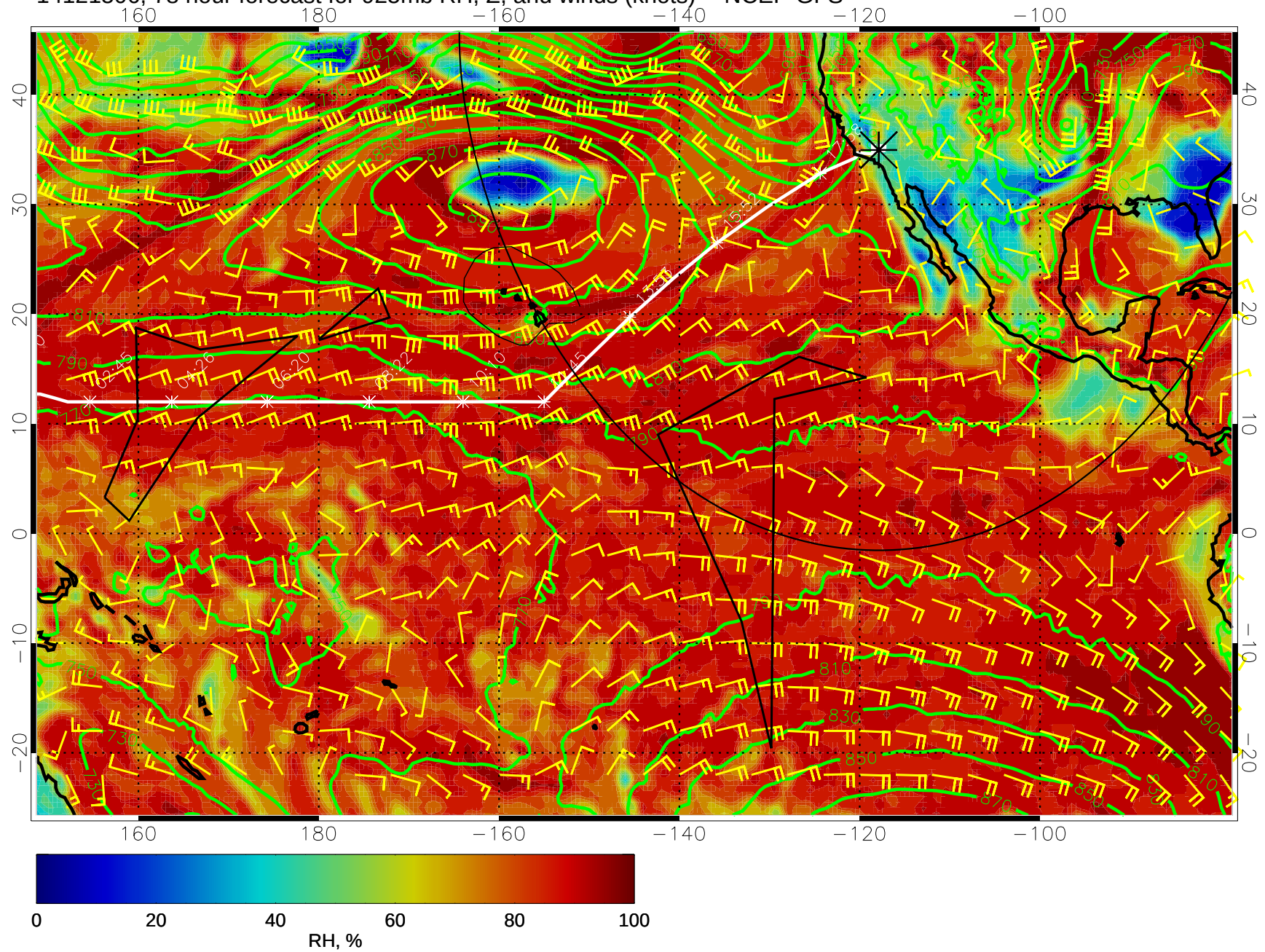
14121506, 78 hour forecast for 925mb RH, Z, and winds (knots) -- NCEP GFS
