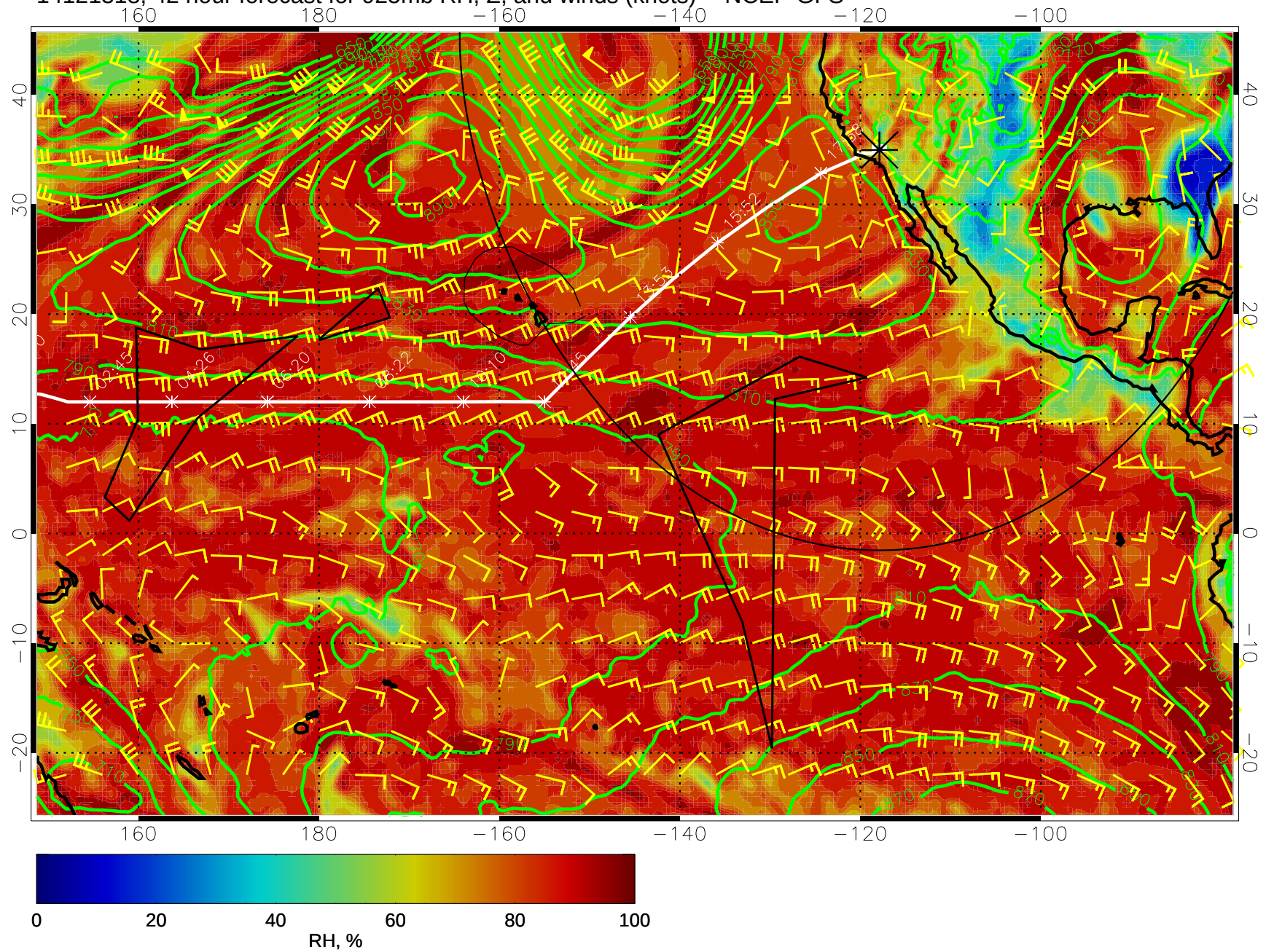
14121318, 42 hour forecast for 925mb RH, Z, and winds (knots) -- NCEP GFS
