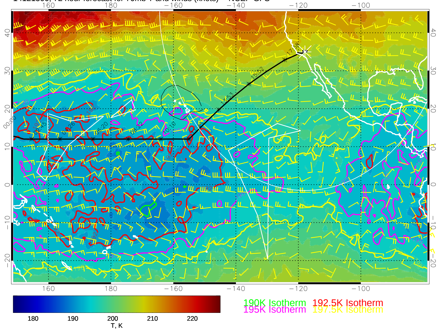
14121500, 72 hour forecast for 70mb T and winds (knots) -- NCEP GFS
