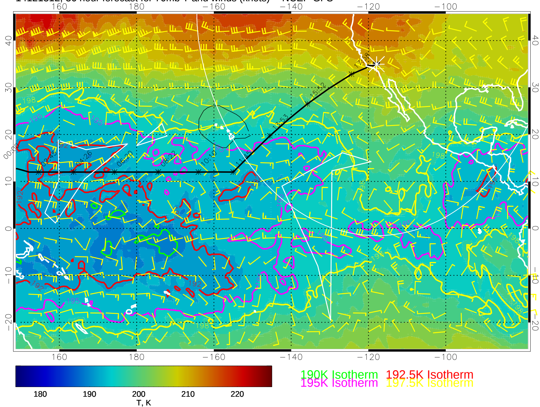
14121312, 36 hour forecast for 70mb T and winds (knots) -- NCEP GFS
