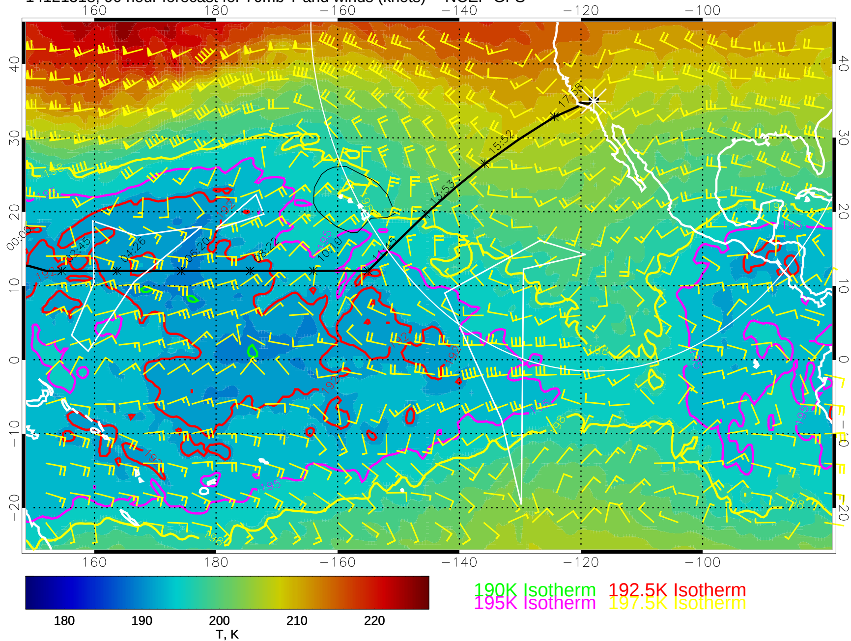
14121518, 90 hour forecast for 70mb T and winds (knots) -- NCEP GFS
