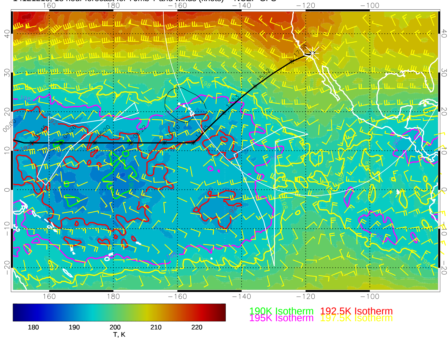
14121218, 18 hour forecast for 70mb T and winds (knots) -- NCEP GFS
