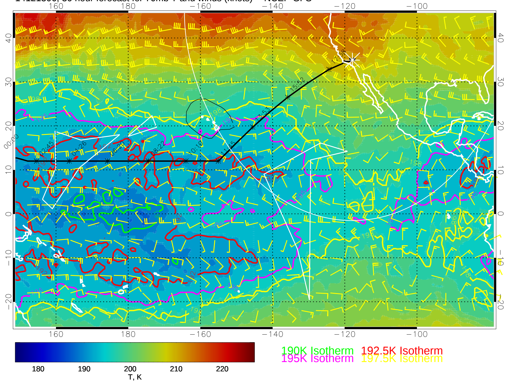
14121306, 30 hour forecast for 70mb T and winds (knots) -- NCEP GFS
