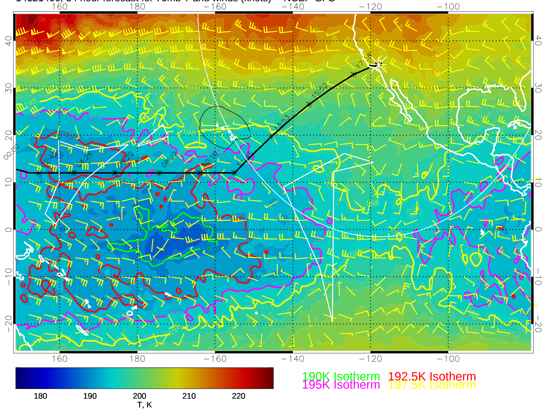
14121406, 54 hour forecast for 70mb T and winds (knots) -- NCEP GFS
