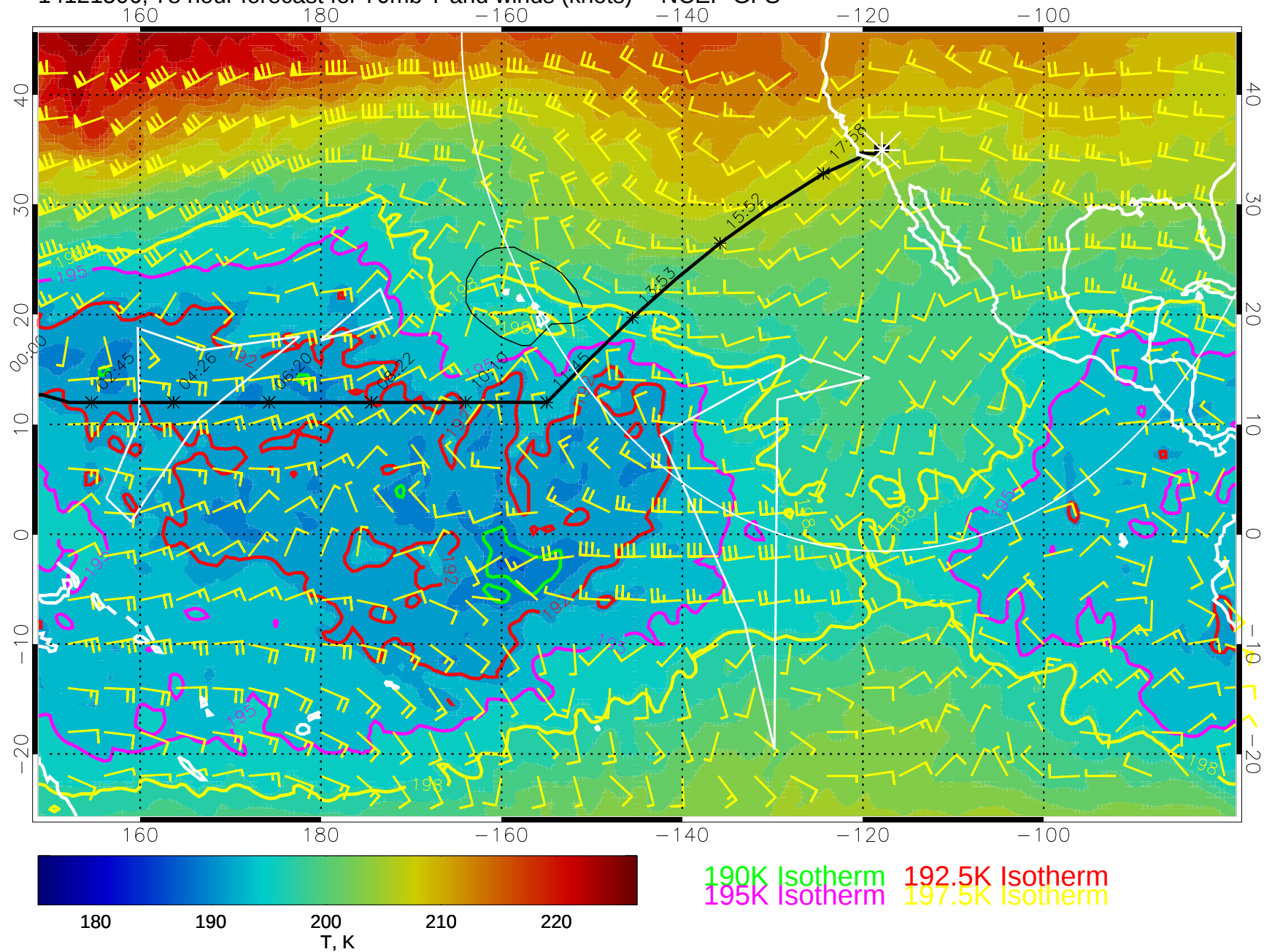
14121506, 78 hour forecast for 70mb T and winds (knots) -- NCEP GFS
