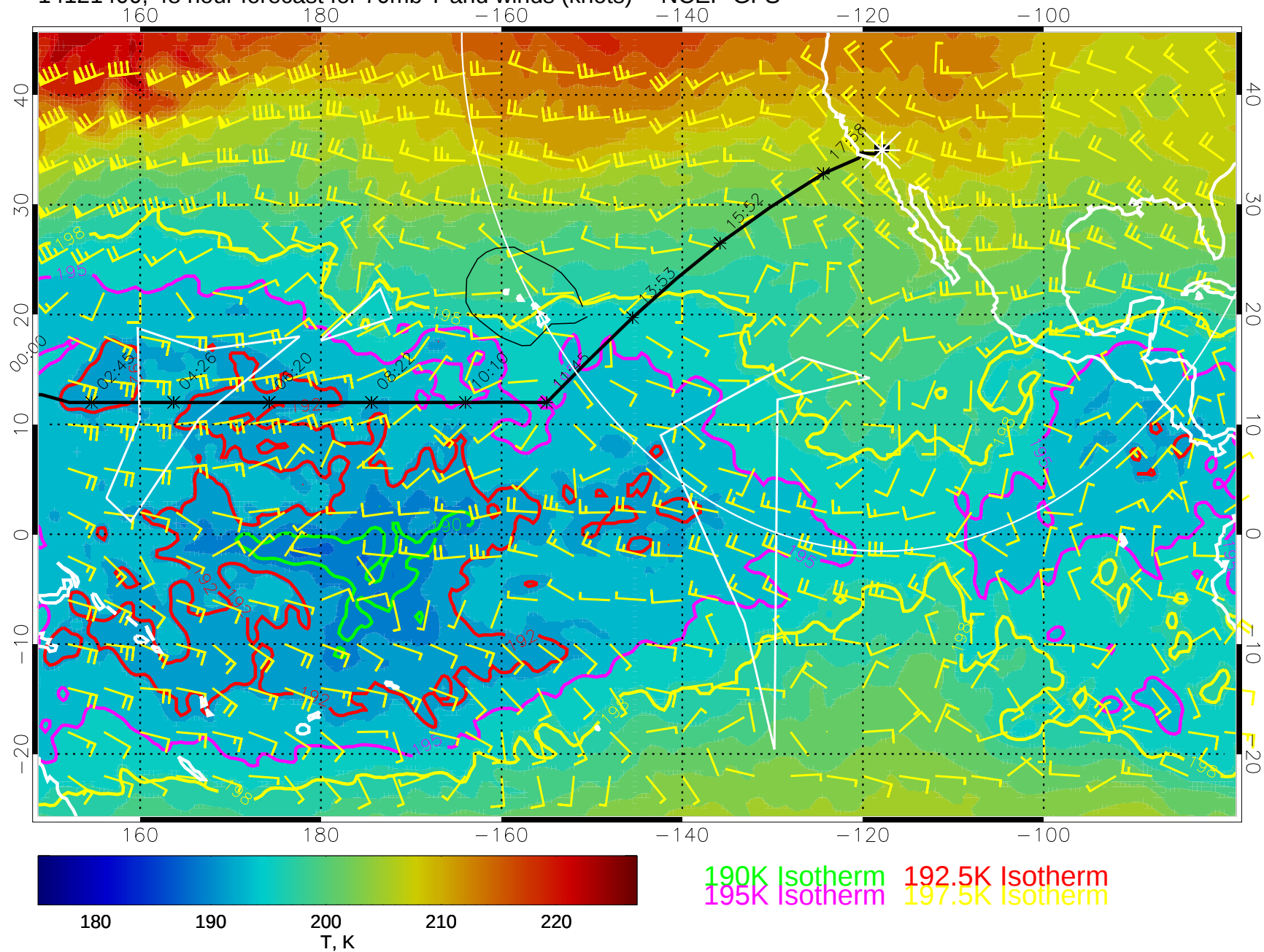
14121400, 48 hour forecast for 70mb T and winds (knots) -- NCEP GFS
