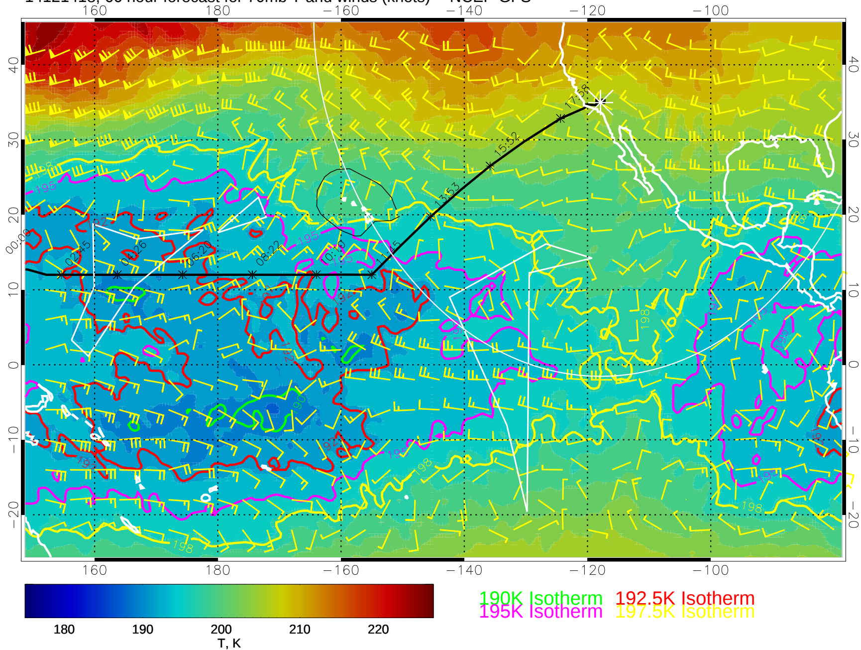
14121418, 66 hour forecast for 70mb T and winds (knots) -- NCEP GFS
