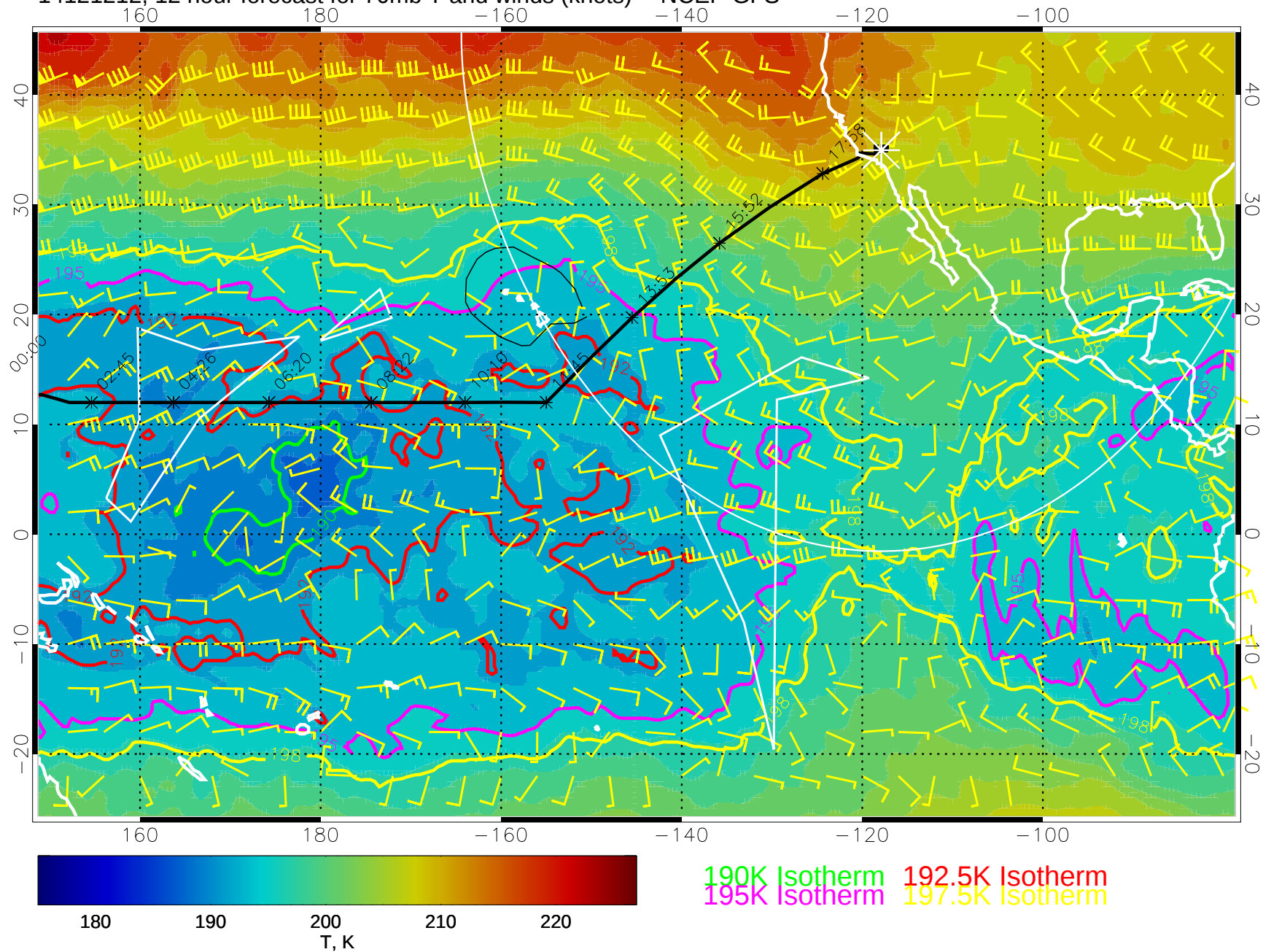
14121212, 12 hour forecast for 70mb T and winds (knots) -- NCEP GFS
