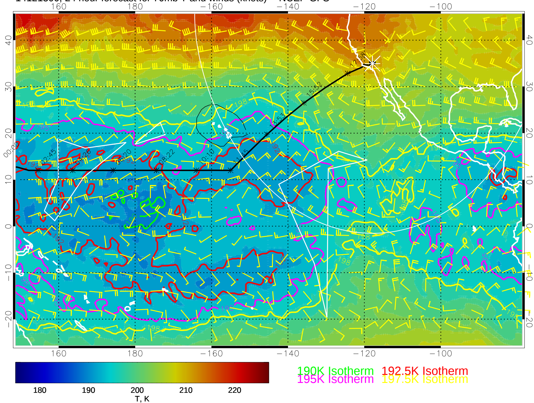
14121300, 24 hour forecast for 70mb T and winds (knots) -- NCEP GFS
