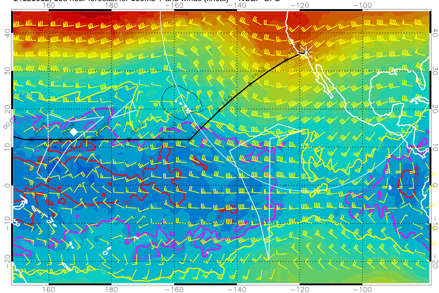
14121612, 108 hour forecast for 100mb T and winds (knots) -- NCEP GFS
