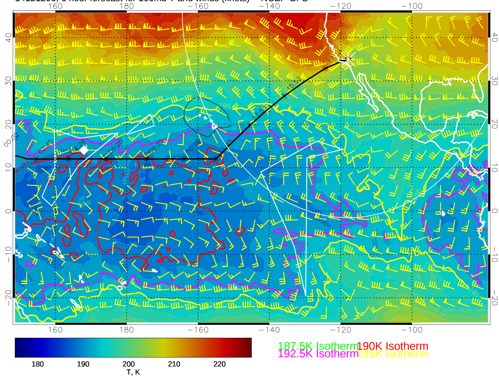
14121206, 6 hour forecast for 100mb T and winds (knots) -- NCEP GFS
