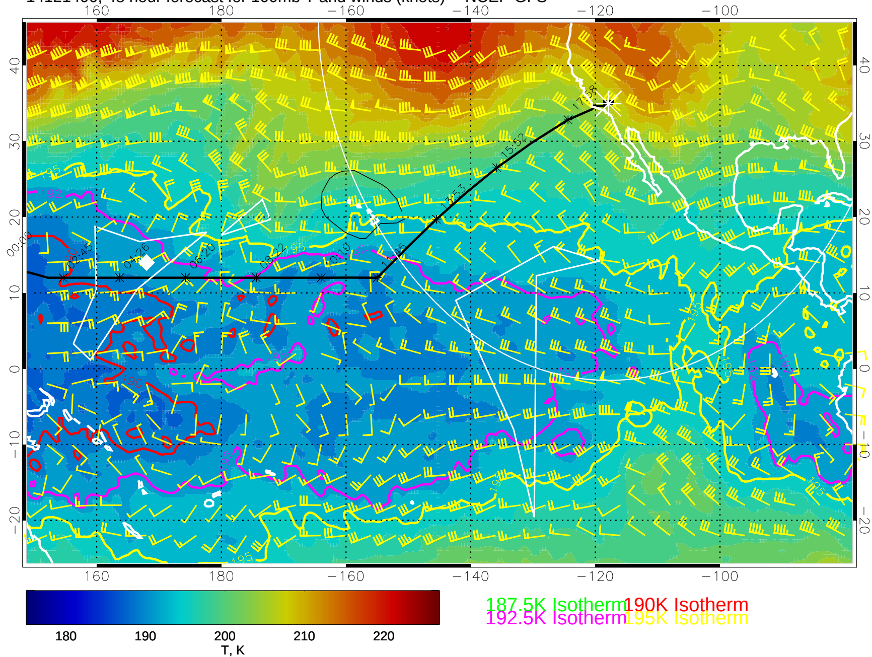
14121400, 48 hour forecast for 100mb T and winds (knots) -- NCEP GFS
