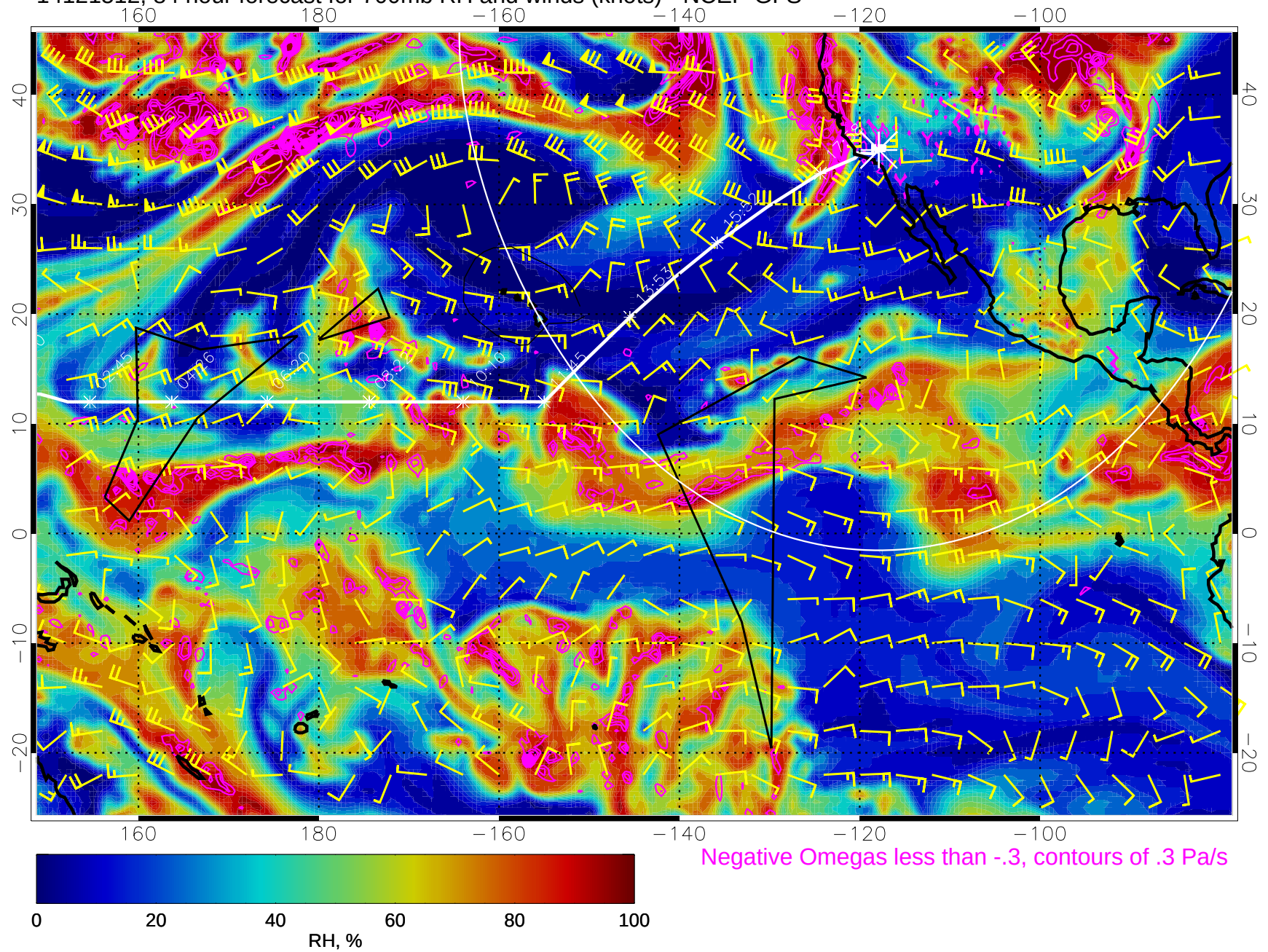
14121512, 84 hour forecast for 700mb RH and winds (knots) - NCEP GFS
