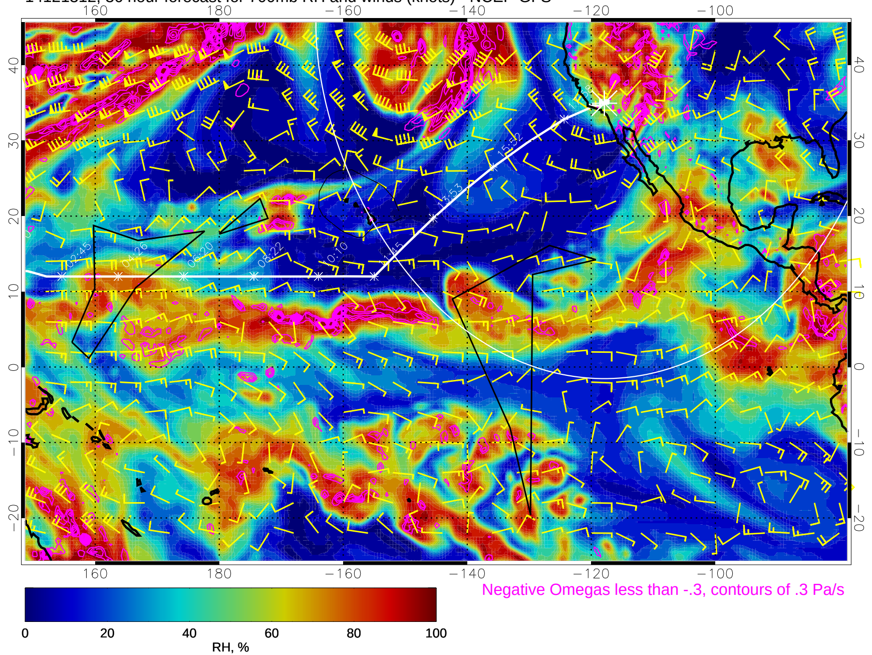
14121312, 36 hour forecast for 700mb RH and winds (knots) - NCEP GFS
