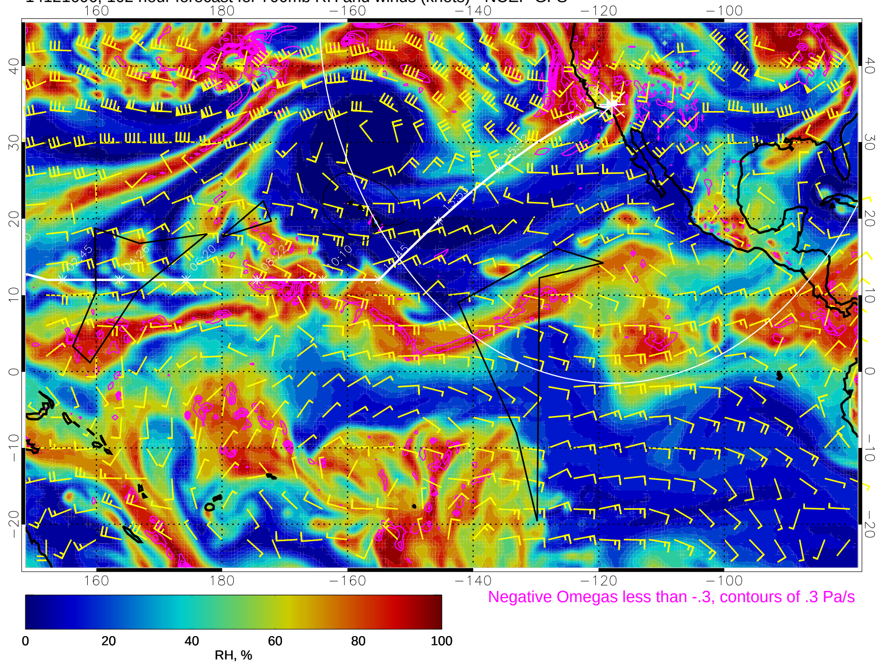
14121606, 102 hour forecast for 700mb RH and winds (knots) - NCEP GFS
