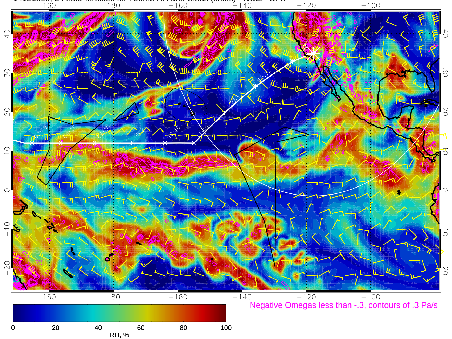
14121300, 24 hour forecast for 700mb RH and winds (knots) - NCEP GFS
