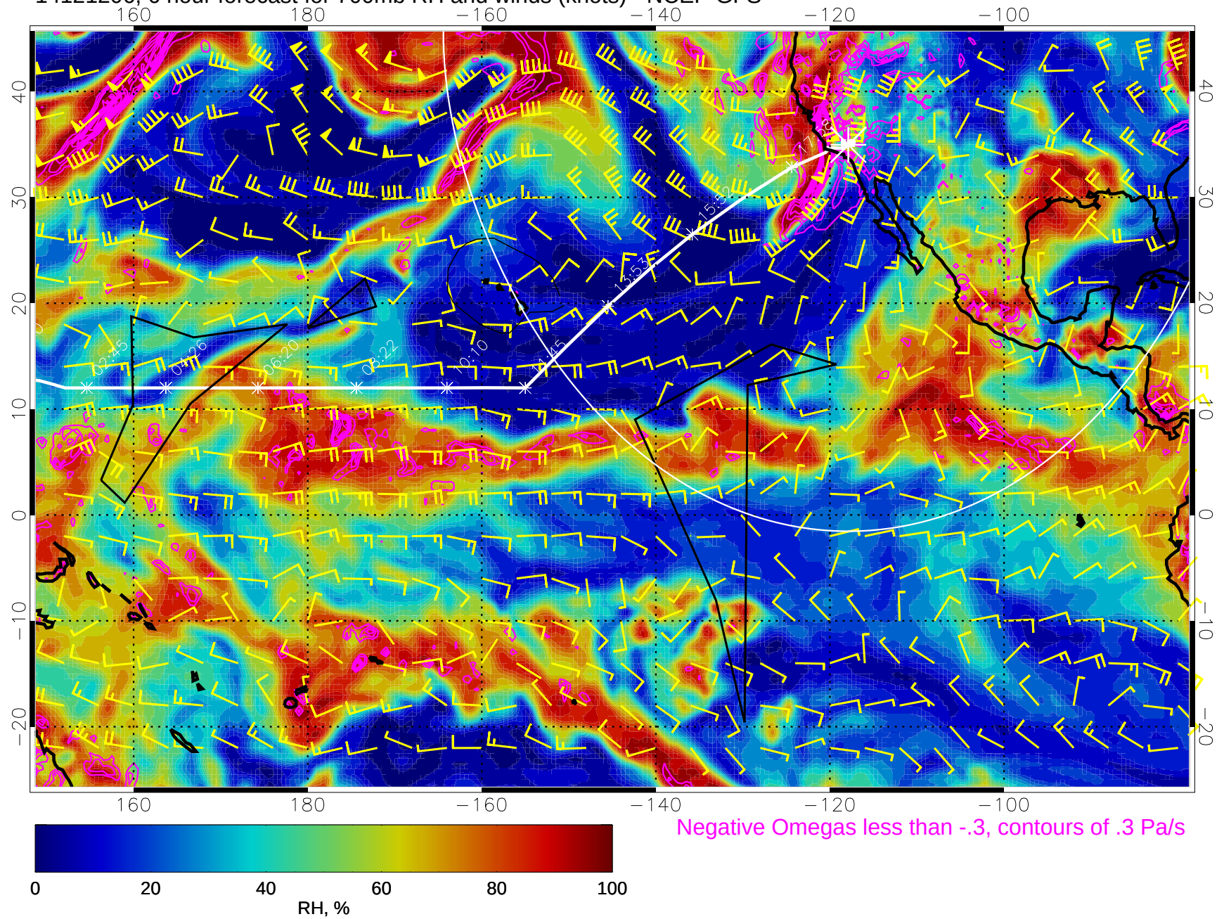
14121206, 6 hour forecast for 700mb RH and winds (knots) - NCEP GFS
