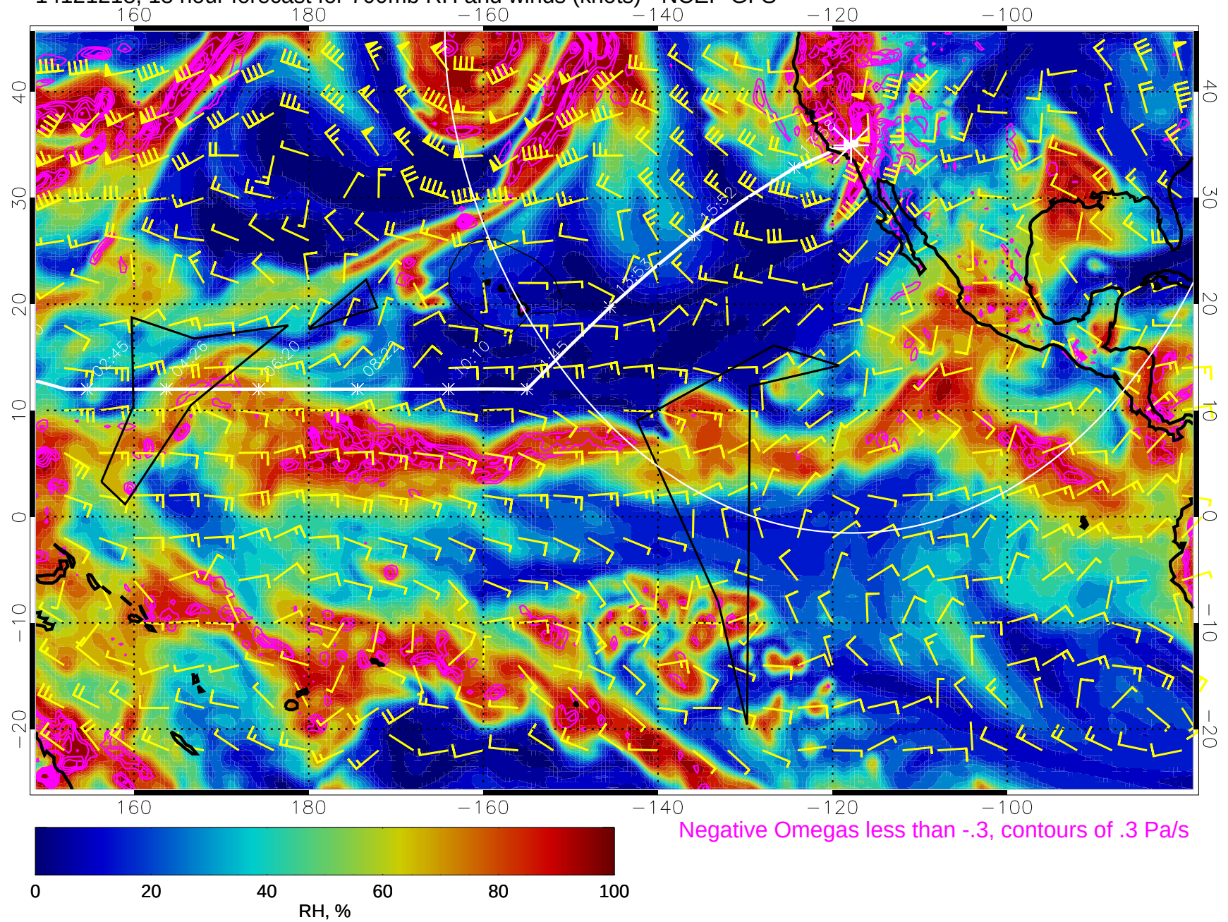
14121218, 18 hour forecast for 700mb RH and winds (knots) - NCEP GFS
