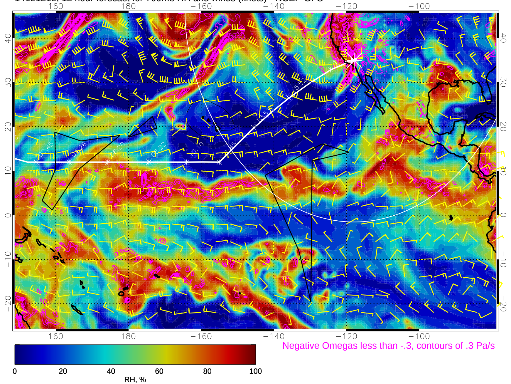
14121212, 12 hour forecast for 700mb RH and winds (knots) - NCEP GFS
