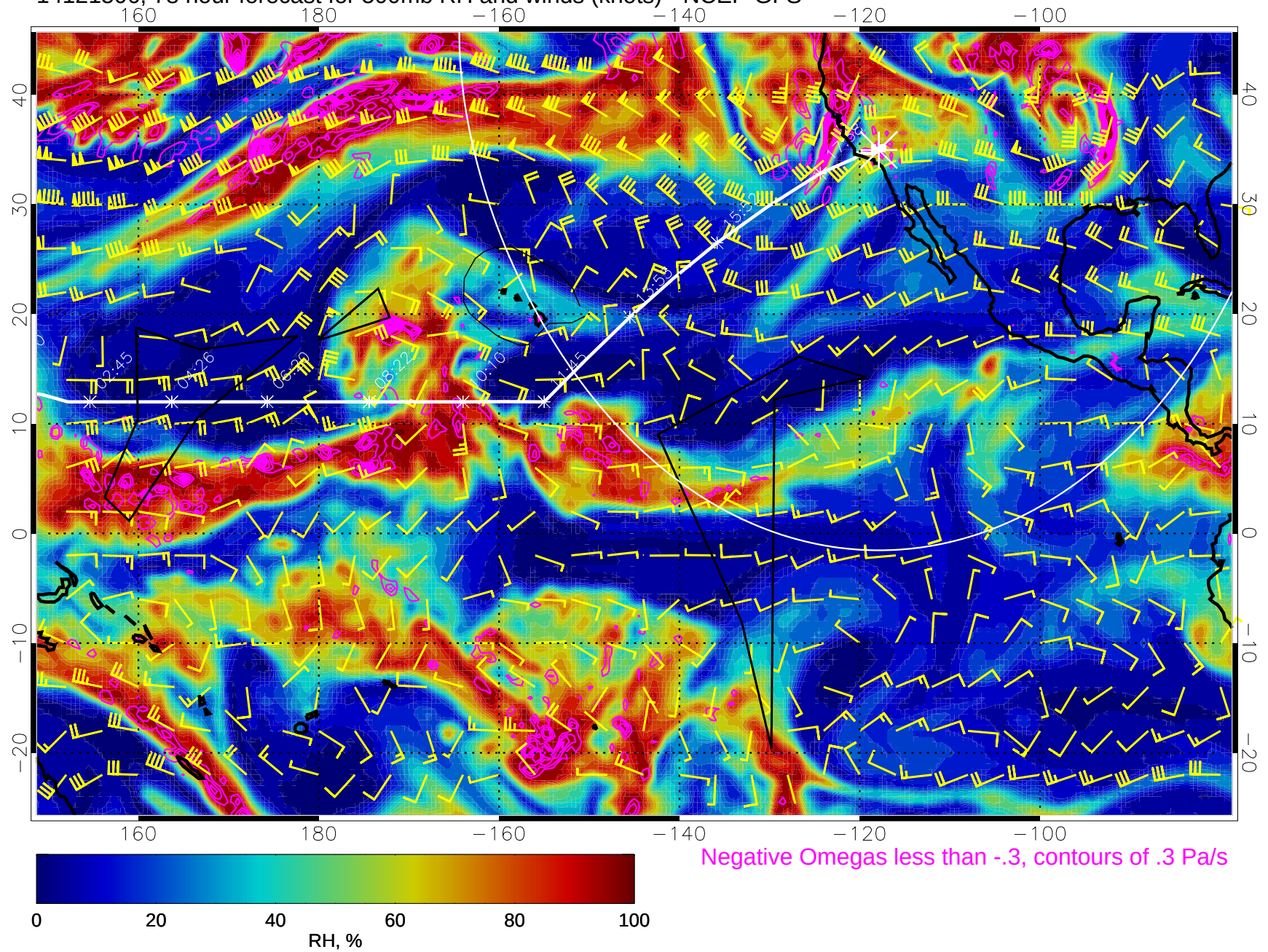
14121506, 78 hour forecast for 500mb RH and winds (knots) - NCEP GFS
