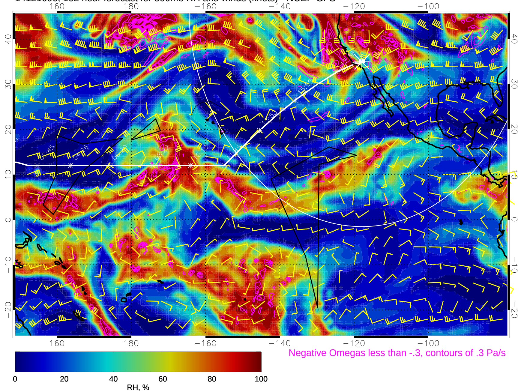
14121606, 102 hour forecast for 500mb RH and winds (knots) - NCEP GFS
