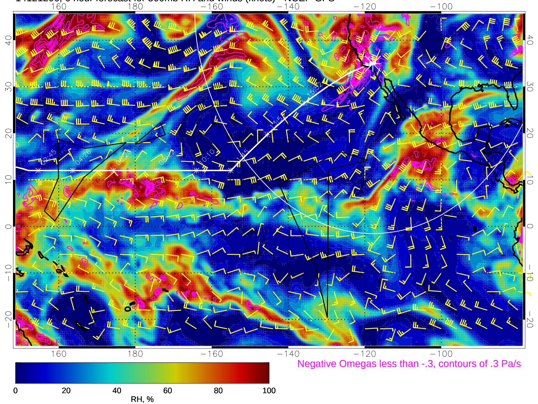
14121206, 6 hour forecast for 500mb RH and winds (knots) - NCEP GFS
