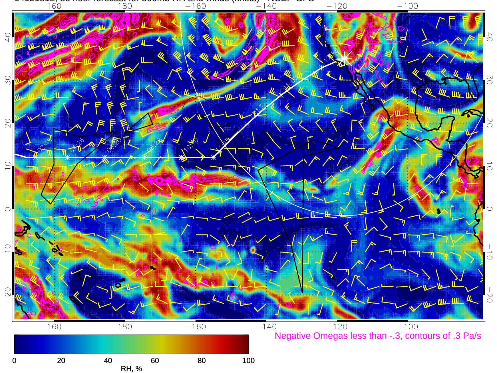
14121312, 36 hour forecast for 500mb RH and winds (knots) - NCEP GFS
