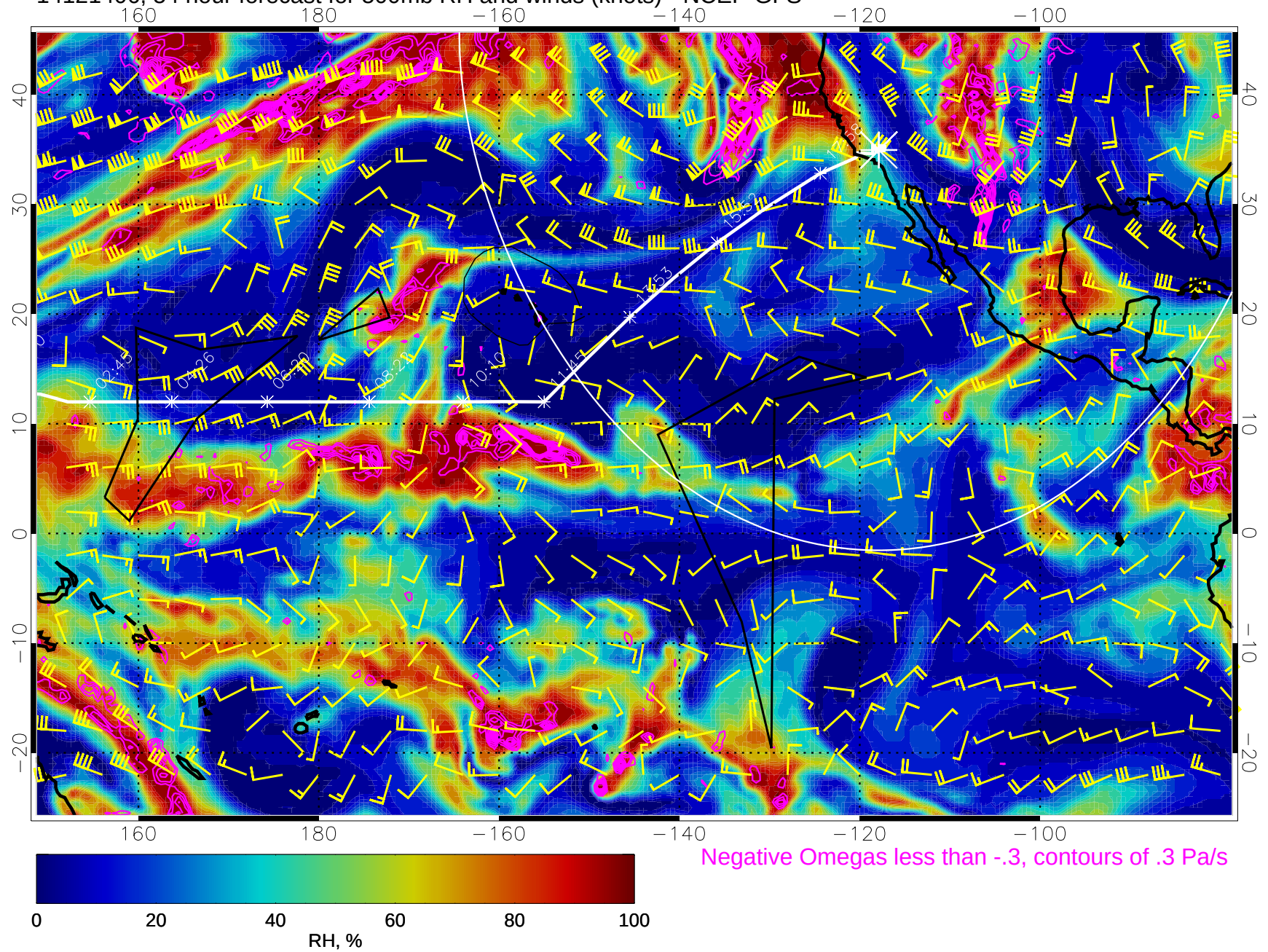
14121406, 54 hour forecast for 500mb RH and winds (knots) - NCEP GFS
