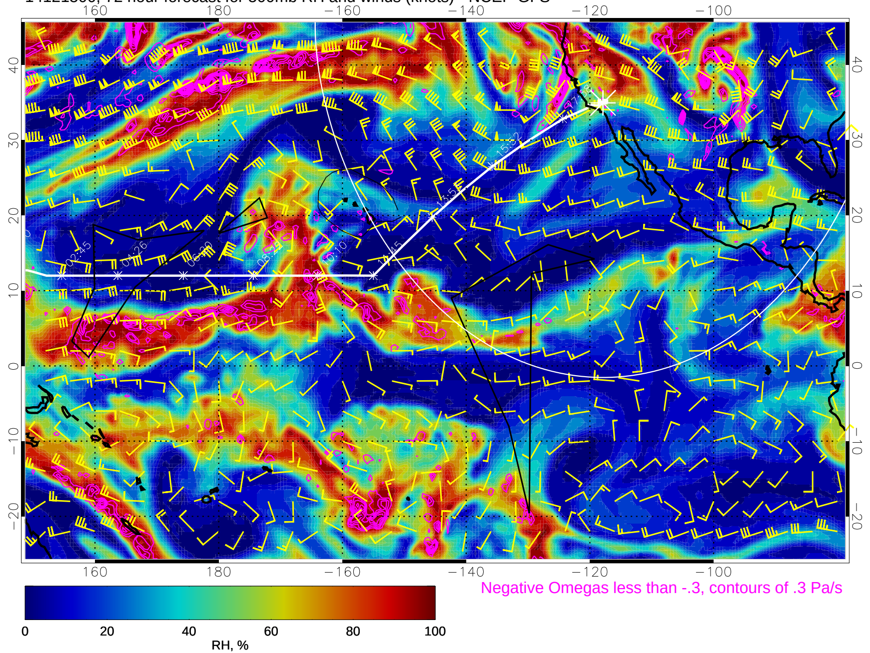
14121500, 72 hour forecast for 500mb RH and winds (knots) - NCEP GFS
