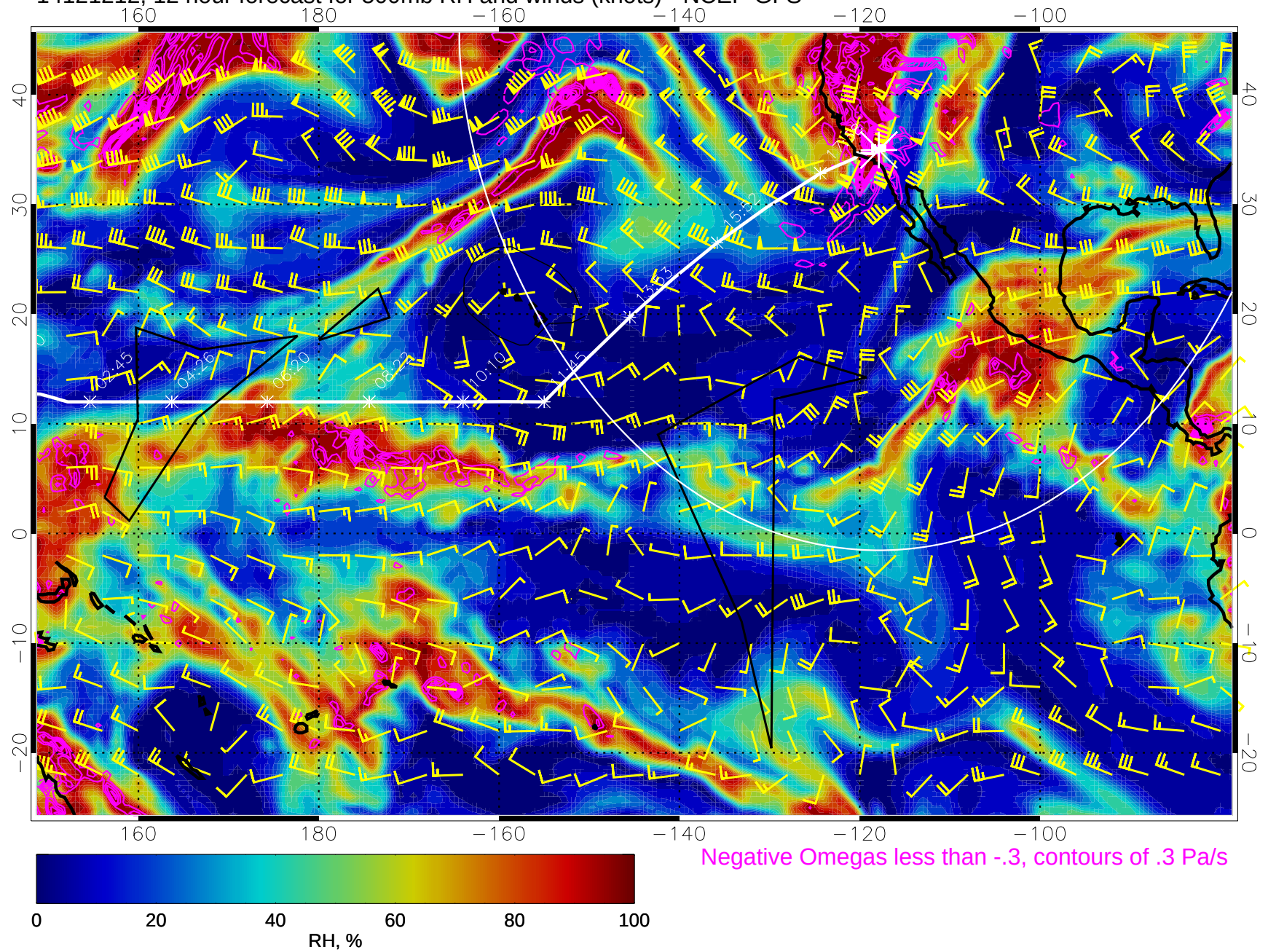
14121212, 12 hour forecast for 500mb RH and winds (knots) - NCEP GFS
