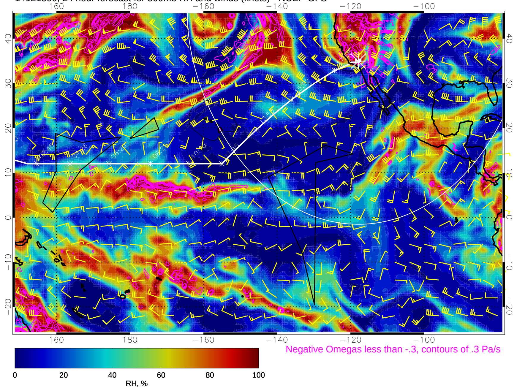
14121300, 24 hour forecast for 500mb RH and winds (knots) - NCEP GFS
