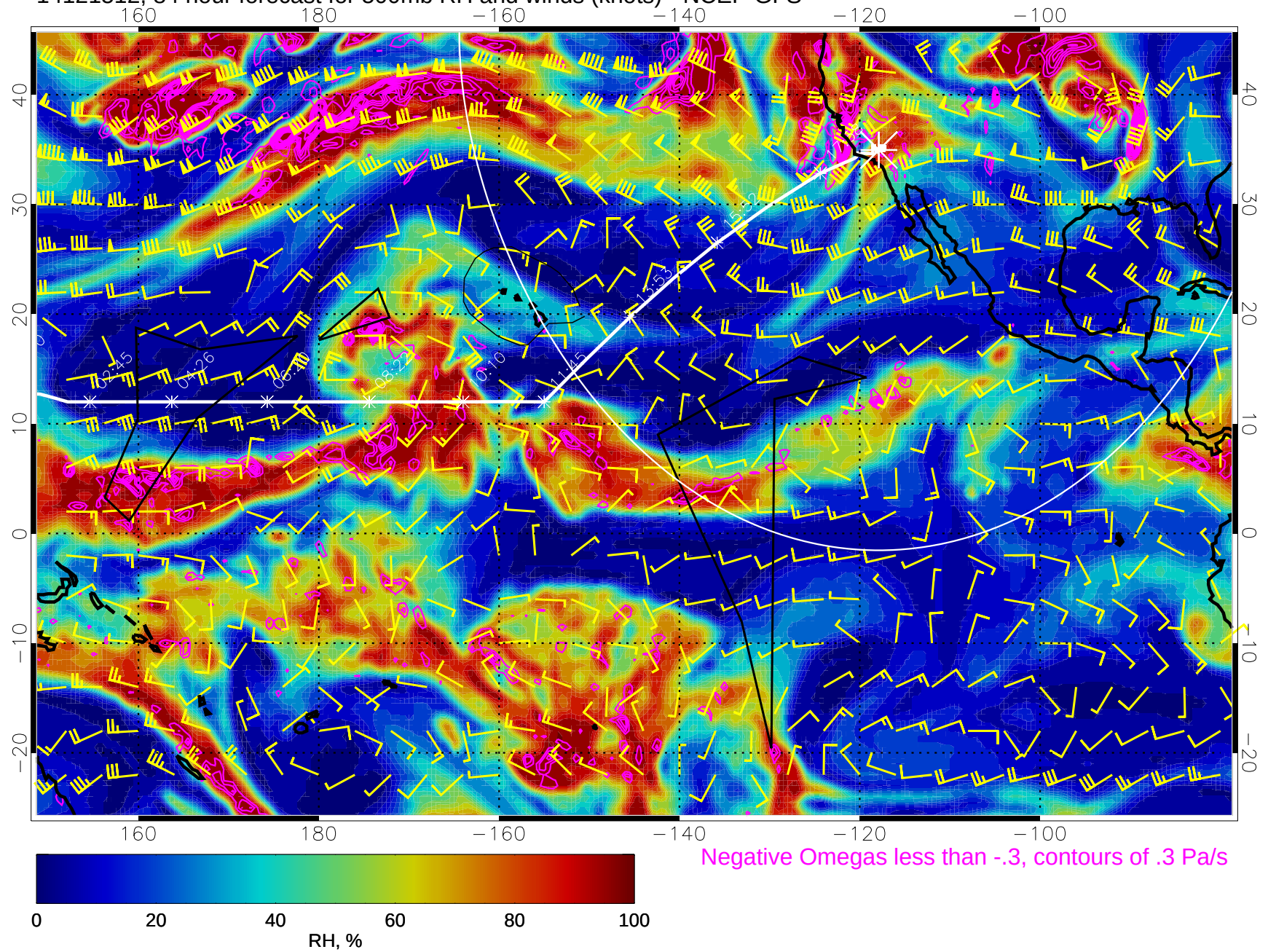
14121512, 84 hour forecast for 500mb RH and winds (knots) - NCEP GFS
