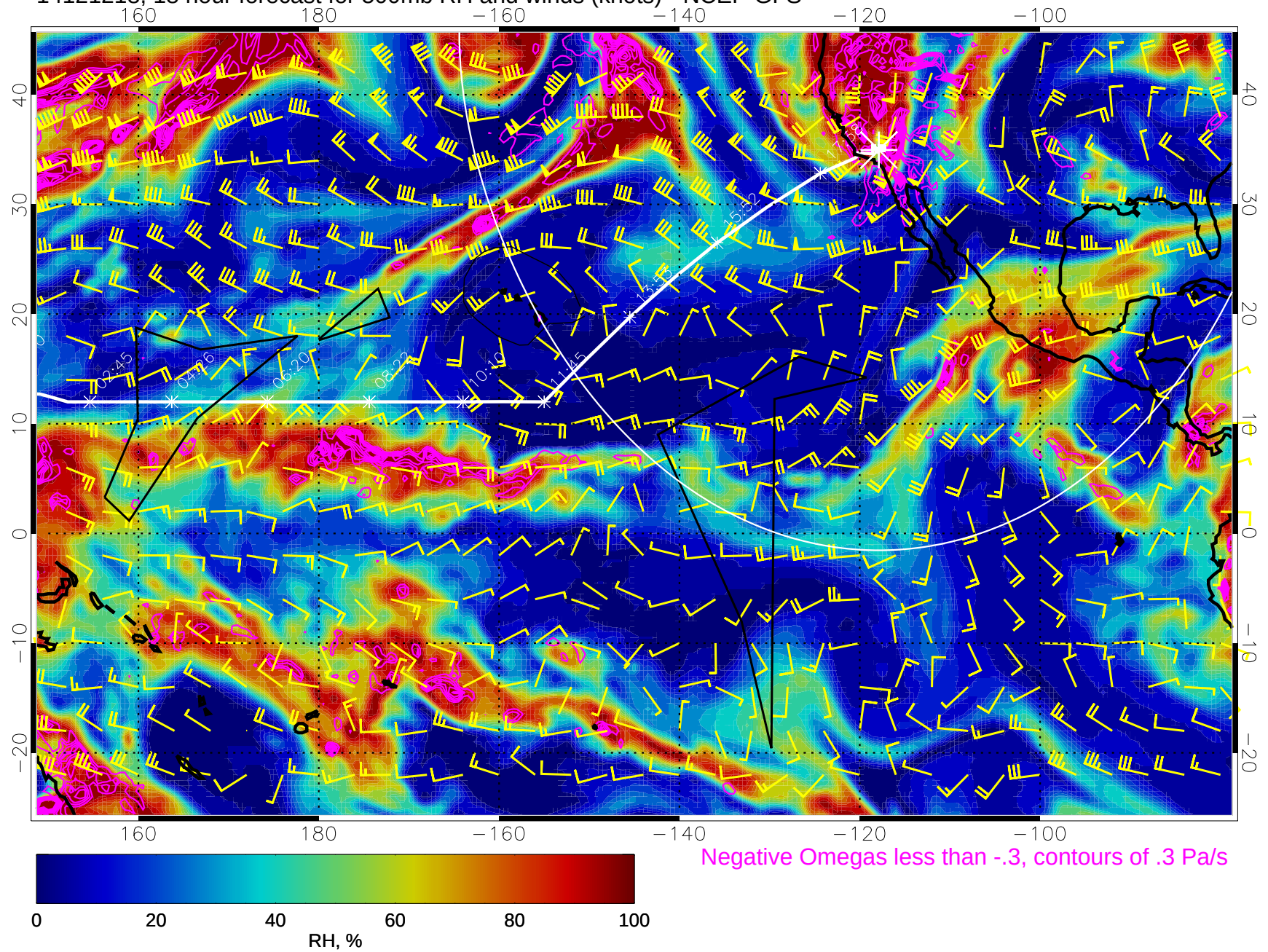
14121218, 18 hour forecast for 500mb RH and winds (knots) - NCEP GFS
