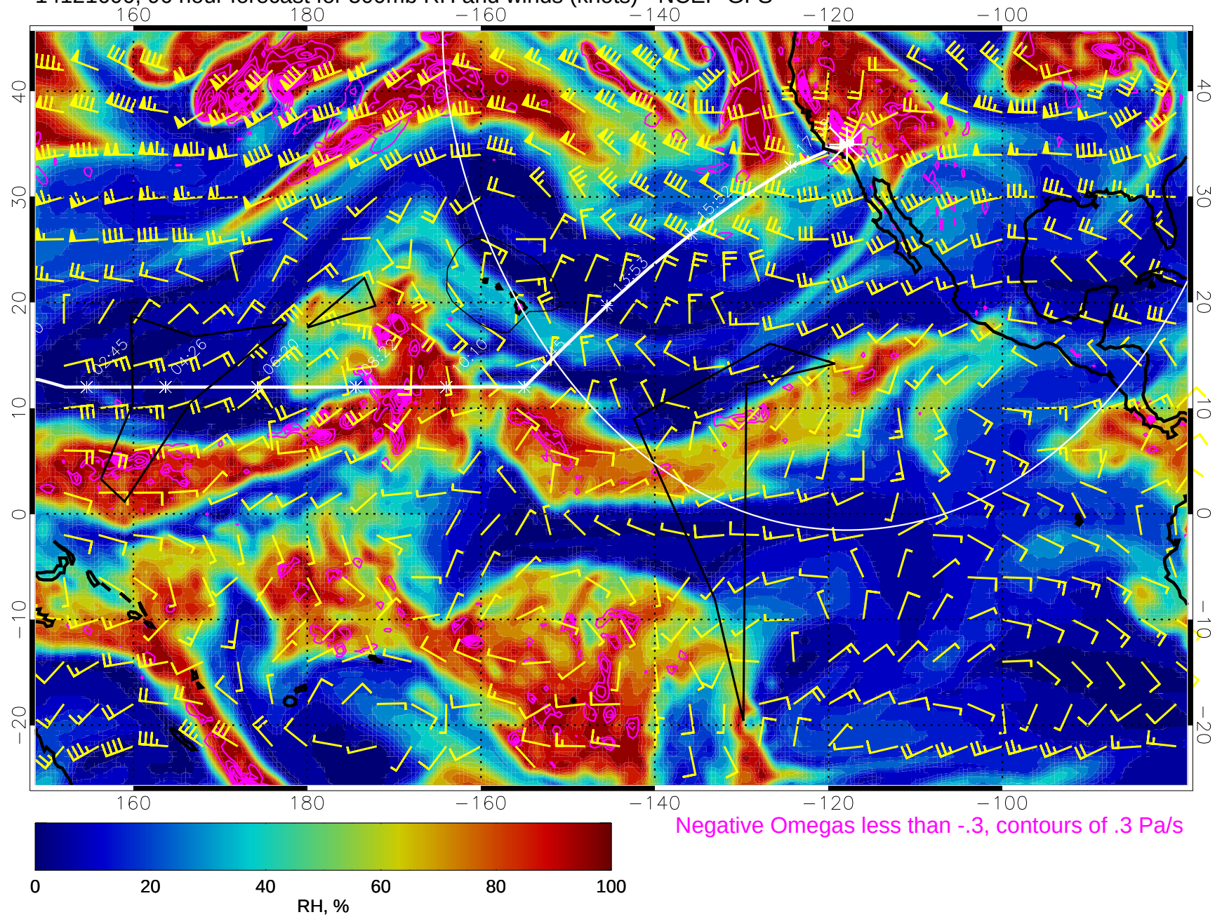
14121600, 96 hour forecast for 500mb RH and winds (knots) - NCEP GFS
