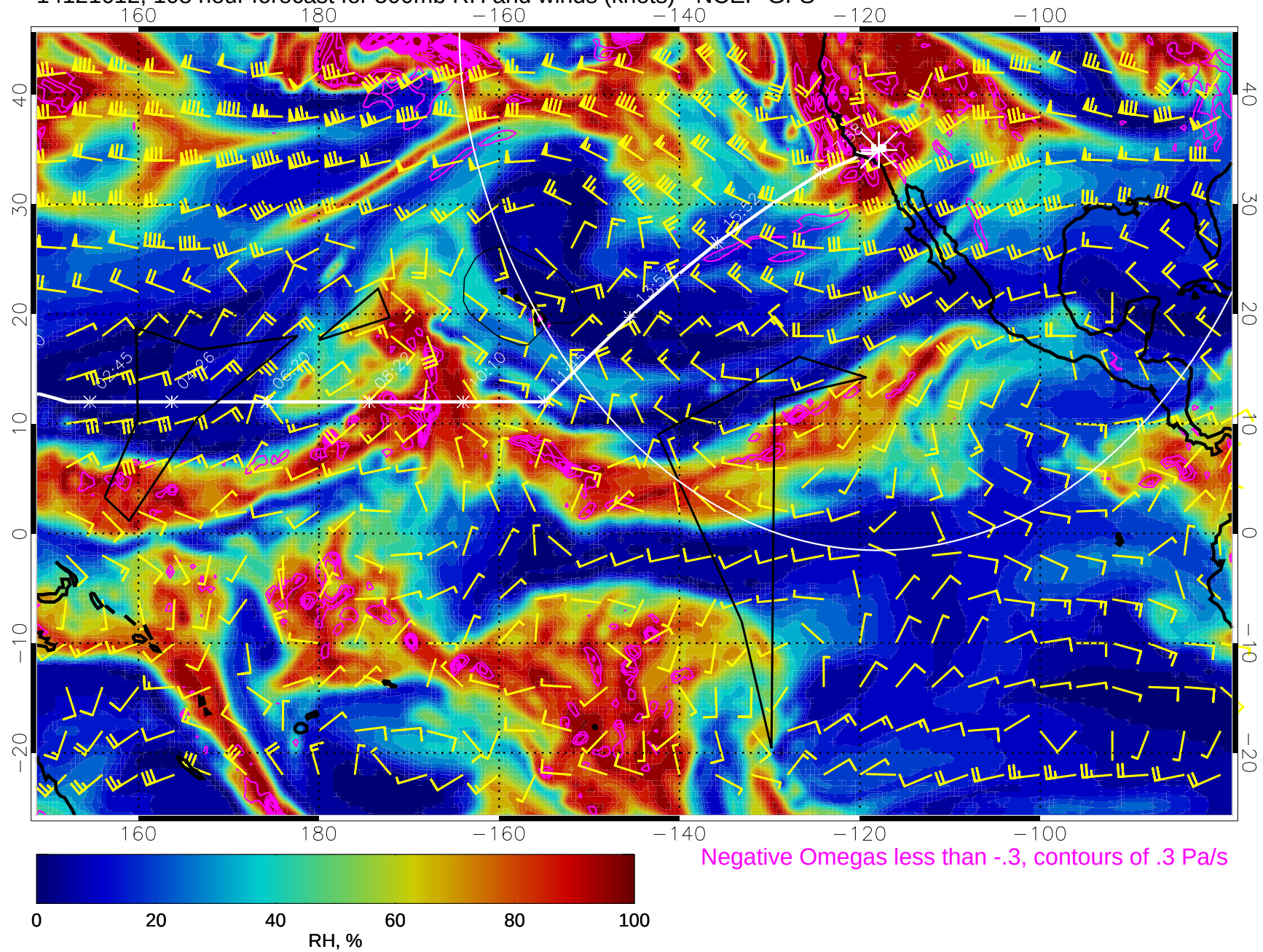
14121612, 108 hour forecast for 500mb RH and winds (knots) - NCEP GFS
