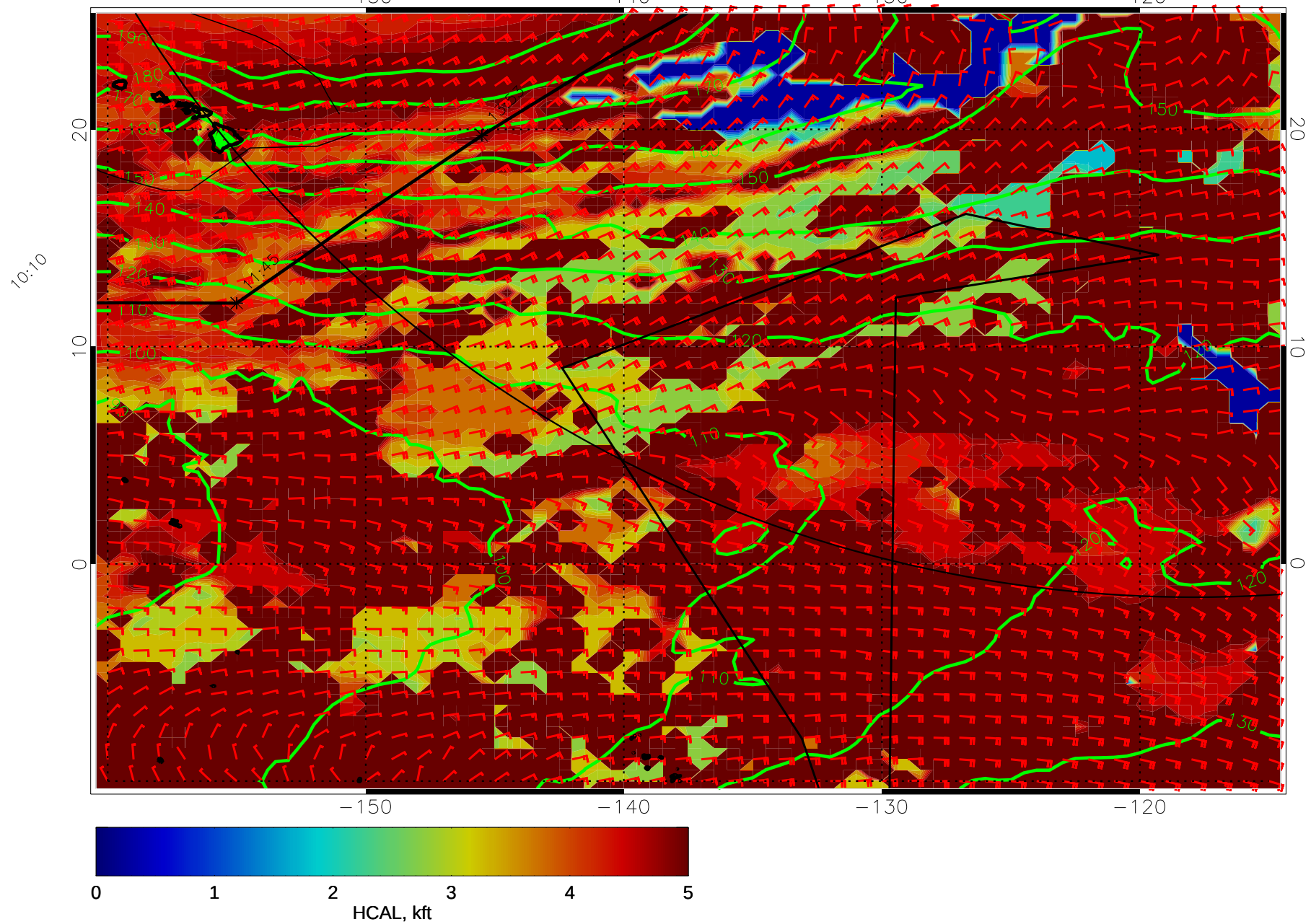
14121606, 102 hour forecast for HCAL, 1000mb Z, and winds (knots) -- NCEP GFS
