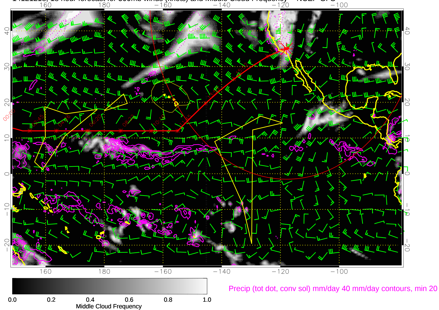
14121218, 18 hour forecast for 500mb winds (knots) and Middle Cloud Frequency -- NCEP GFS
