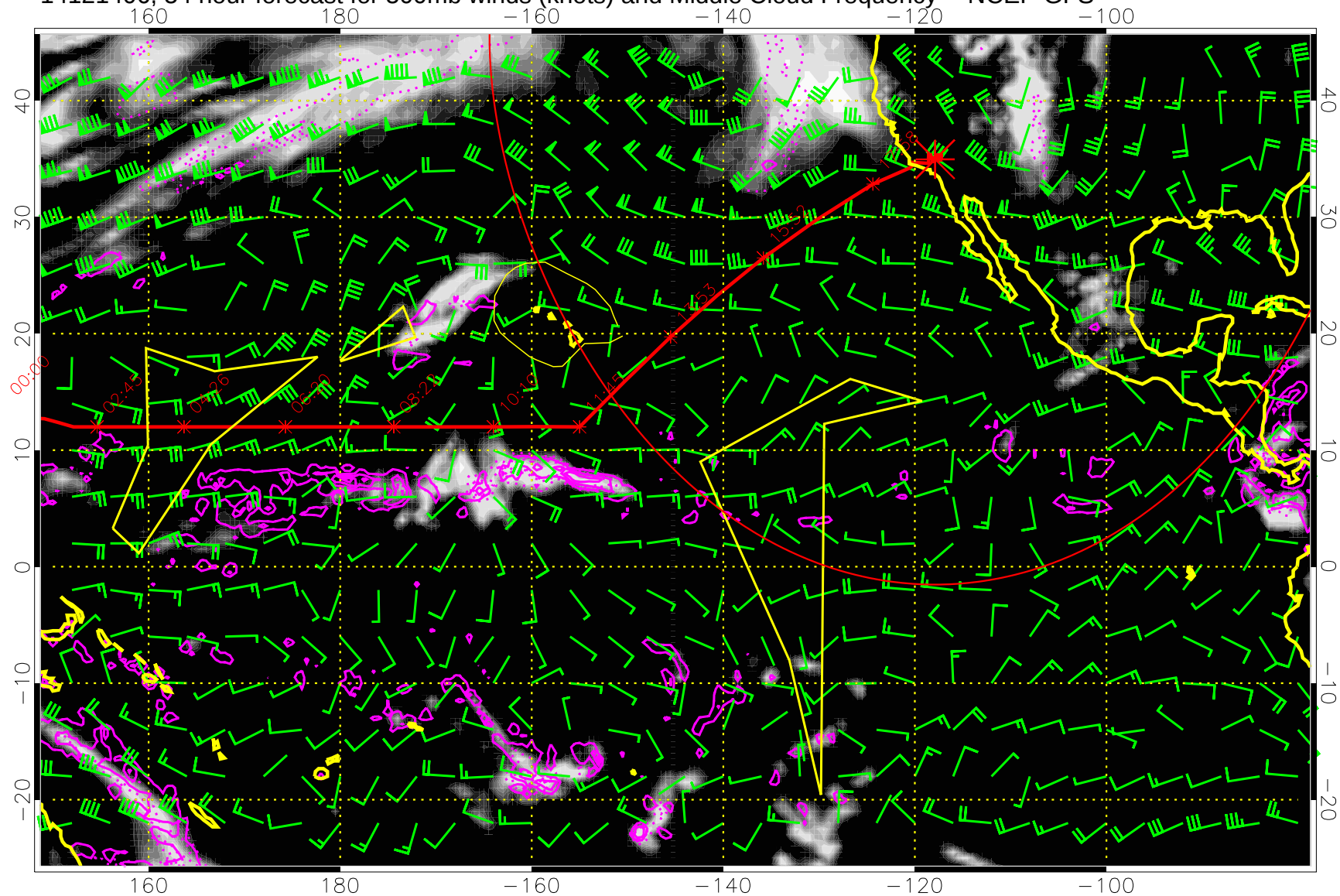
14121406, 54 hour forecast for 500mb winds (knots) and Middle Cloud Frequency -- NCEP GFS
