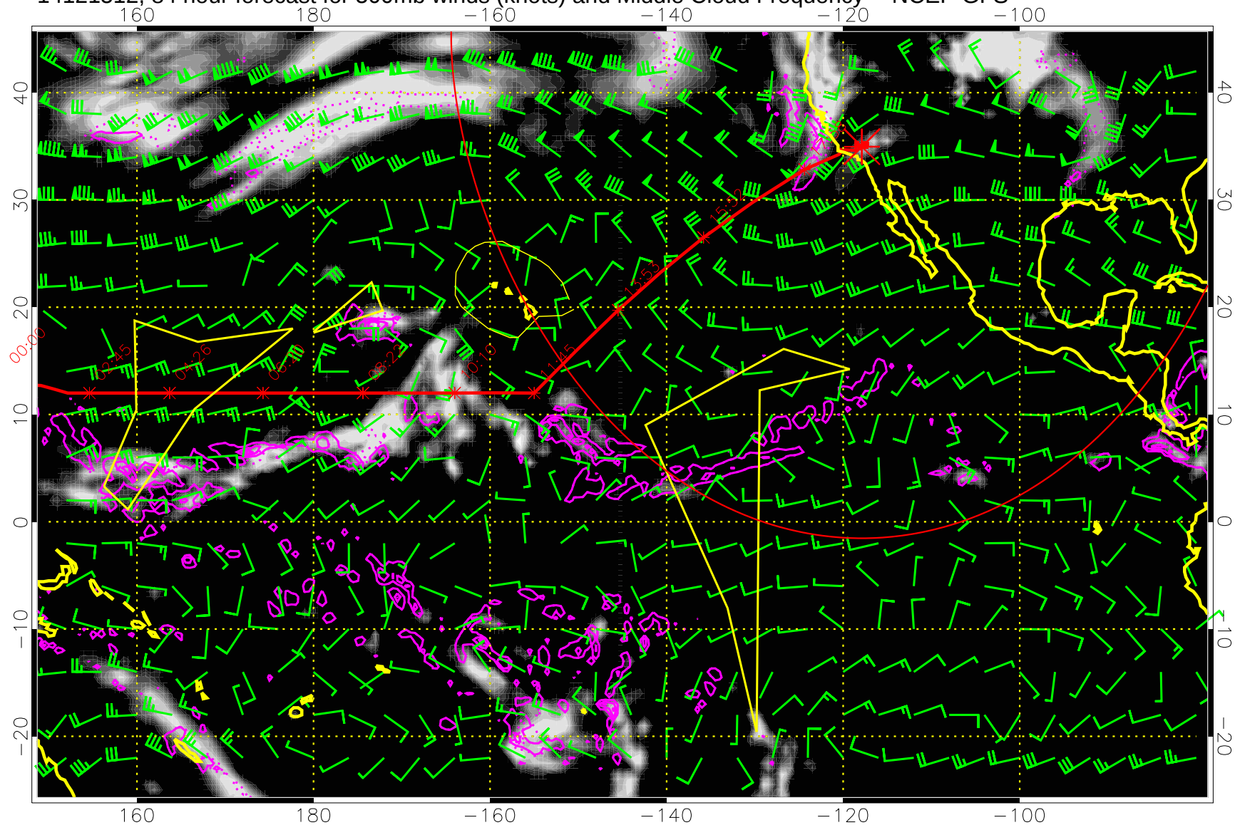
14121512, 84 hour forecast for 500mb winds (knots) and Middle Cloud Frequency -- NCEP GFS
