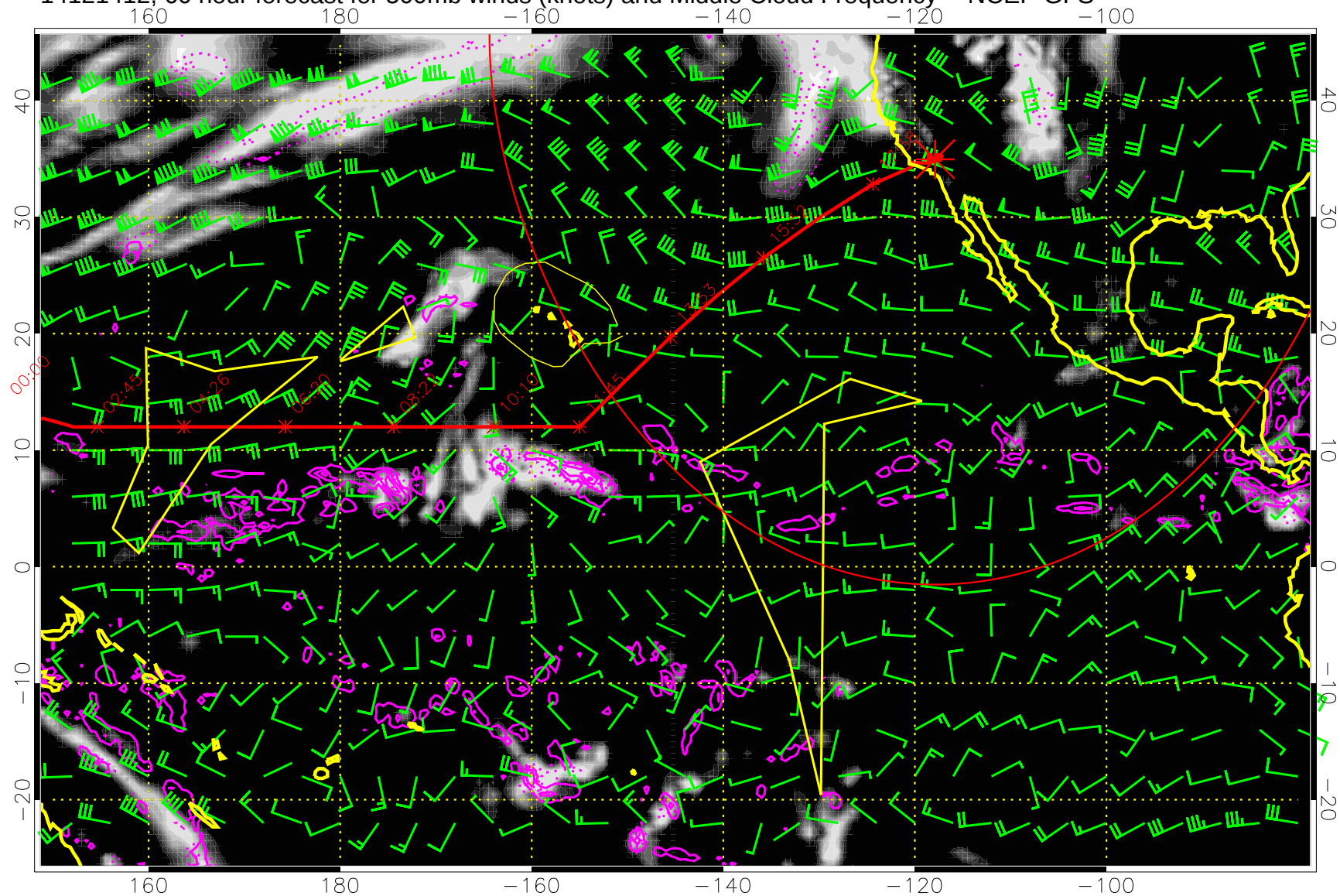
14121412, 60 hour forecast for 500mb winds (knots) and Middle Cloud Frequency -- NCEP GFS
