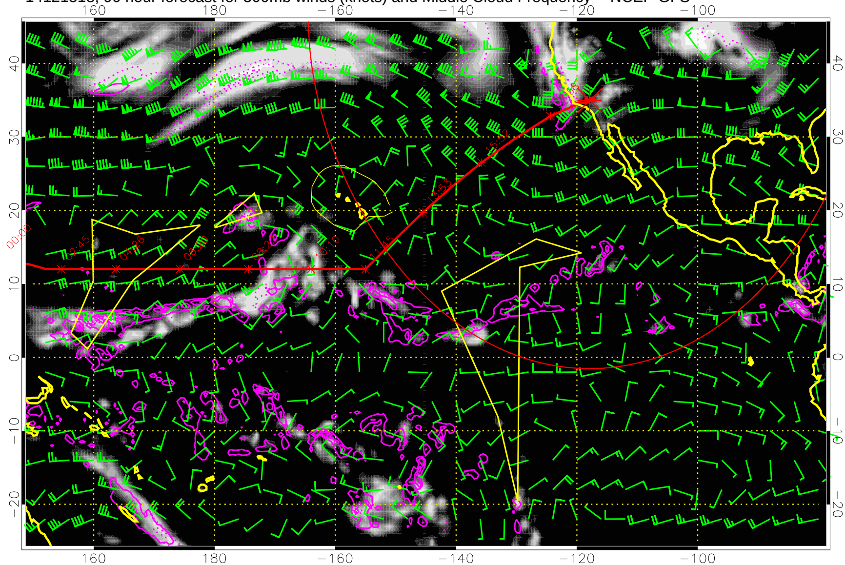
14121518, 90 hour forecast for 500mb winds (knots) and Middle Cloud Frequency -- NCEP GFS
