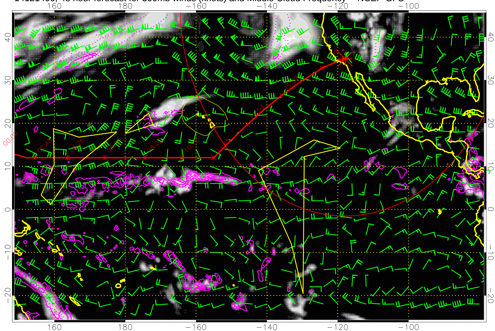
14121400, 48 hour forecast for 500mb winds (knots) and Middle Cloud Frequency -- NCEP GFS
