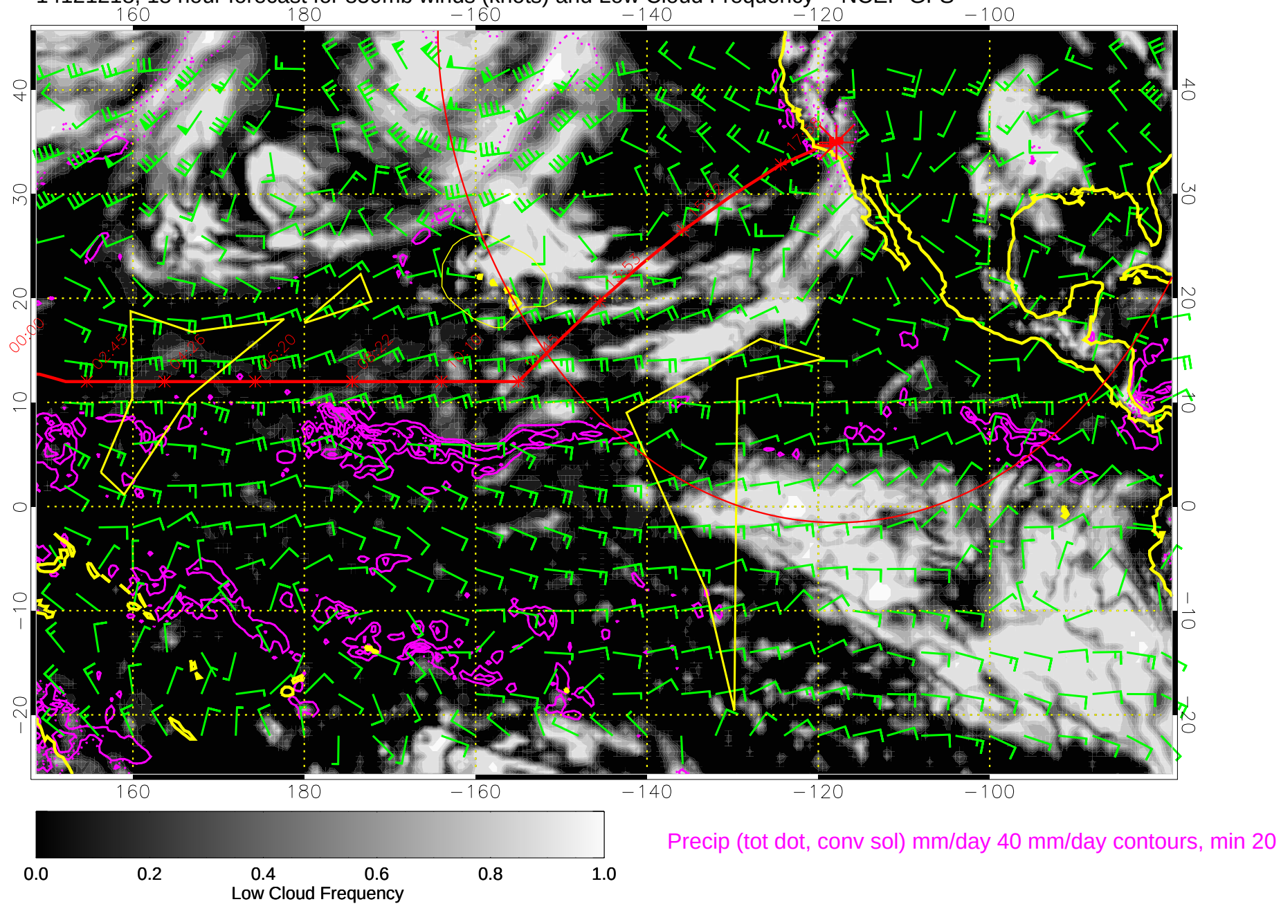
14121218, 18 hour forecast for 850mb winds (knots) and Low Cloud Frequency -- NCEP GFS
