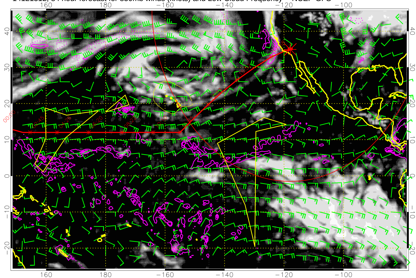
14121512, 84 hour forecast for 850mb winds (knots) and Low Cloud Frequency -- NCEP GFS
