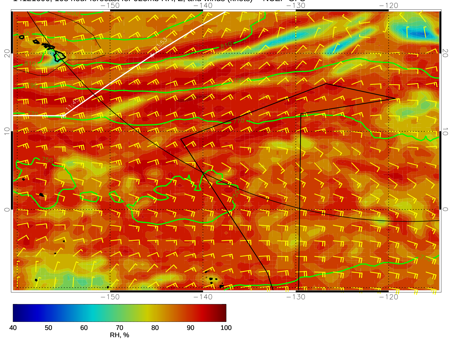
14121600, 108 hour forecast for 925mb RH, Z, and winds (knots) -- NCEP GFS
