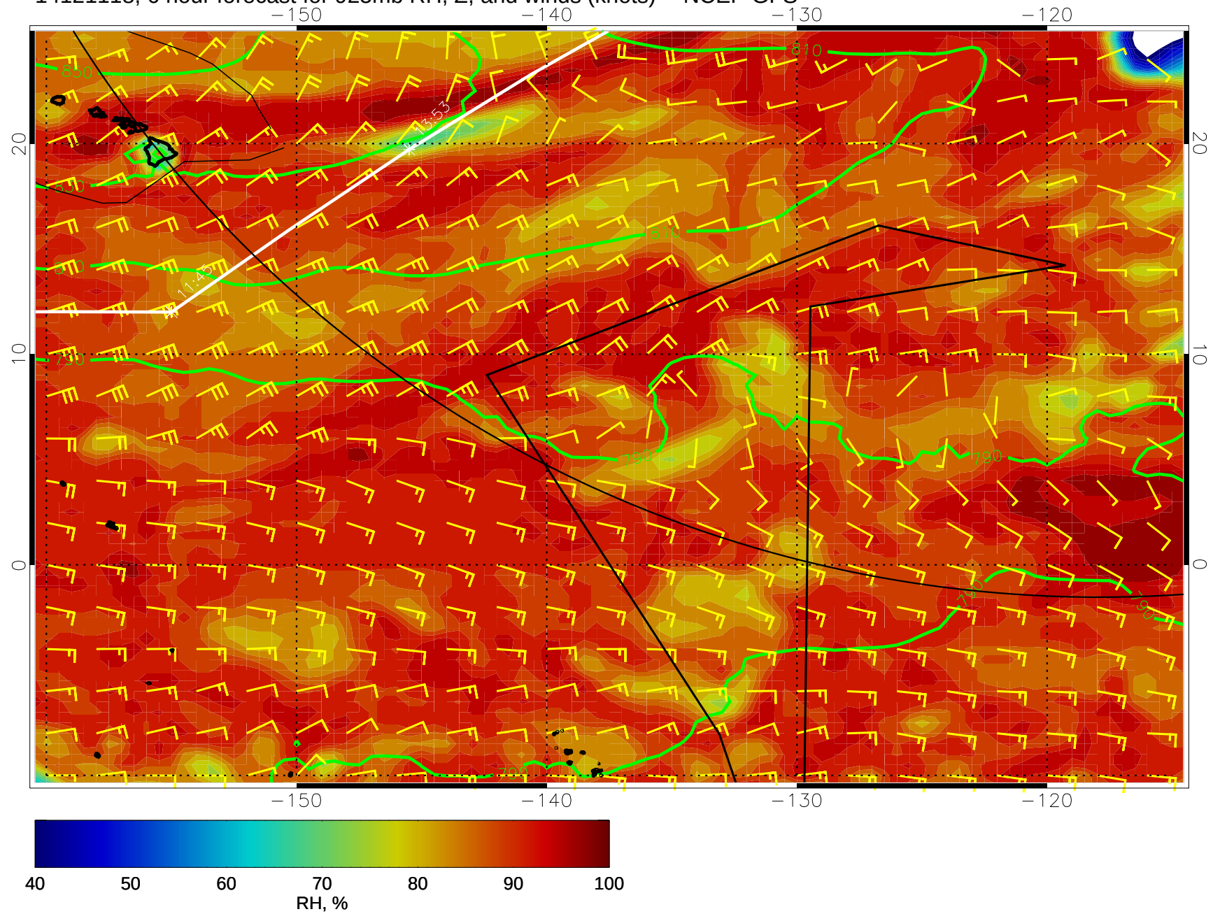
14121118, 6 hour forecast for 925mb RH, Z, and winds (knots) -- NCEP GFS
