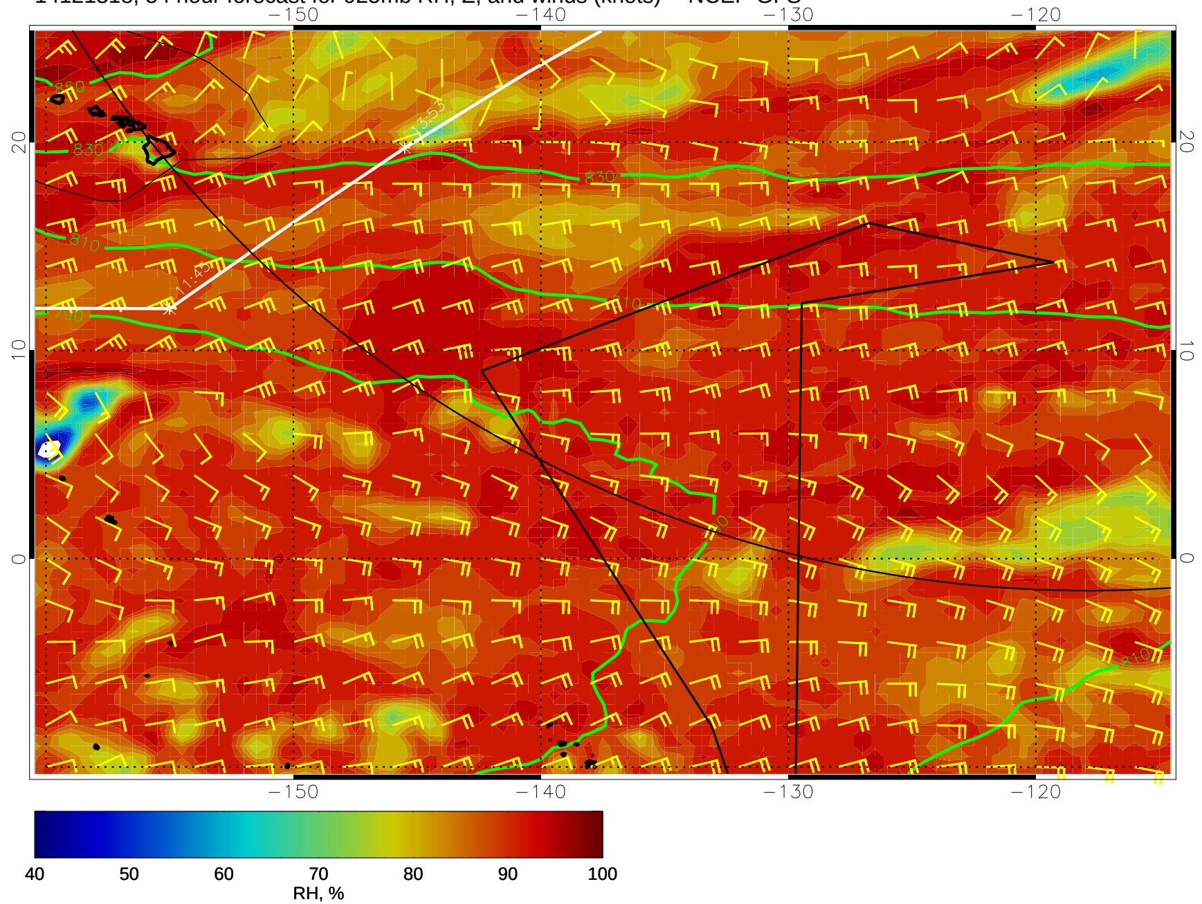
14121318, 54 hour forecast for 925mb RH, Z, and winds (knots) -- NCEP GFS
