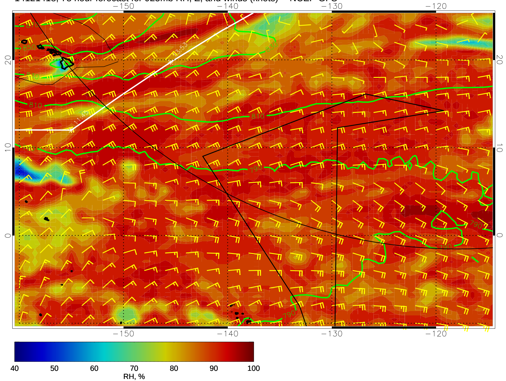
14121418, 78 hour forecast for 925mb RH, Z, and winds (knots) -- NCEP GFS
