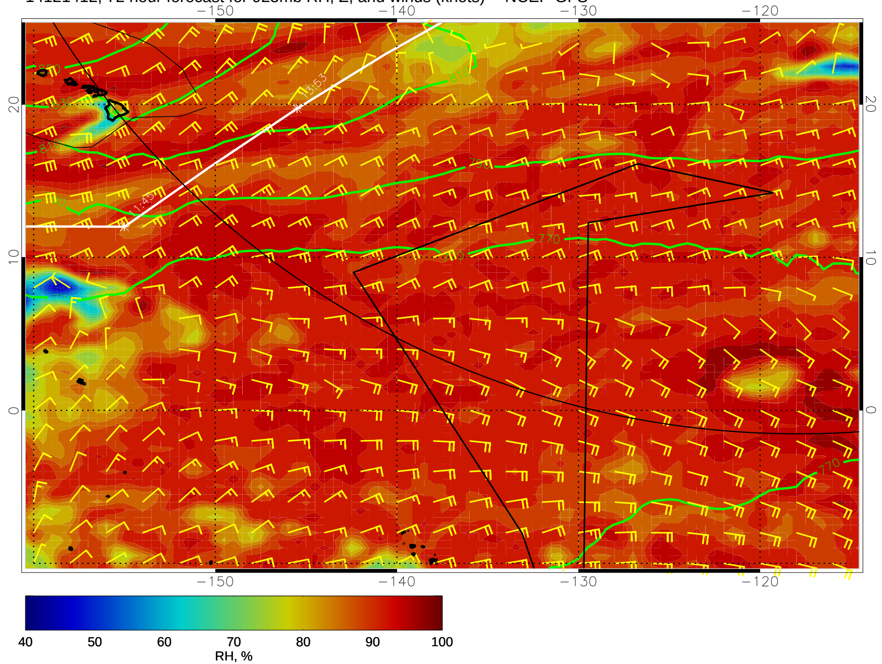
14121412, 72 hour forecast for 925mb RH, Z, and winds (knots) -- NCEP GFS
