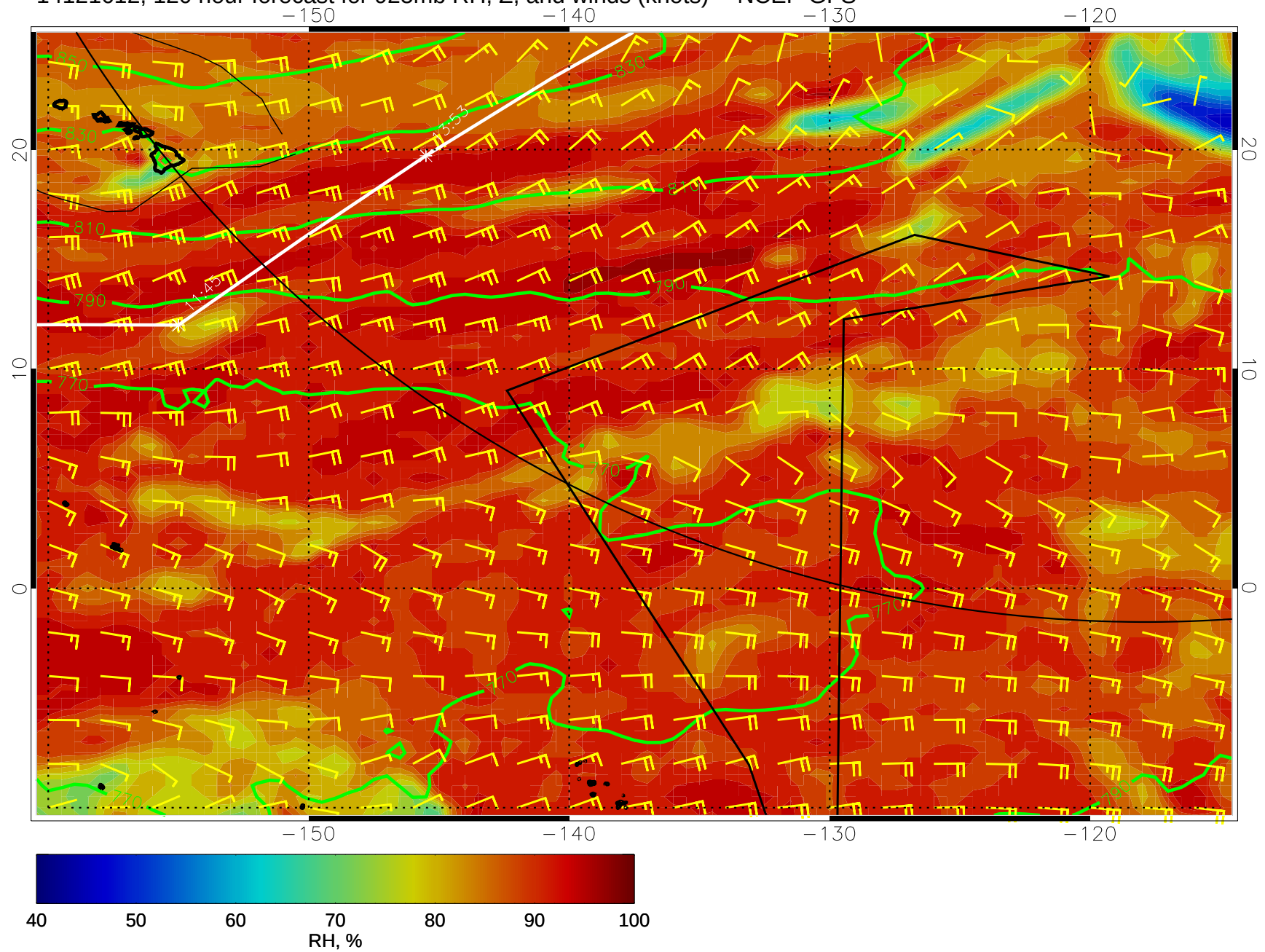
14121612, 120 hour forecast for 925mb RH, Z, and winds (knots) -- NCEP GFS
