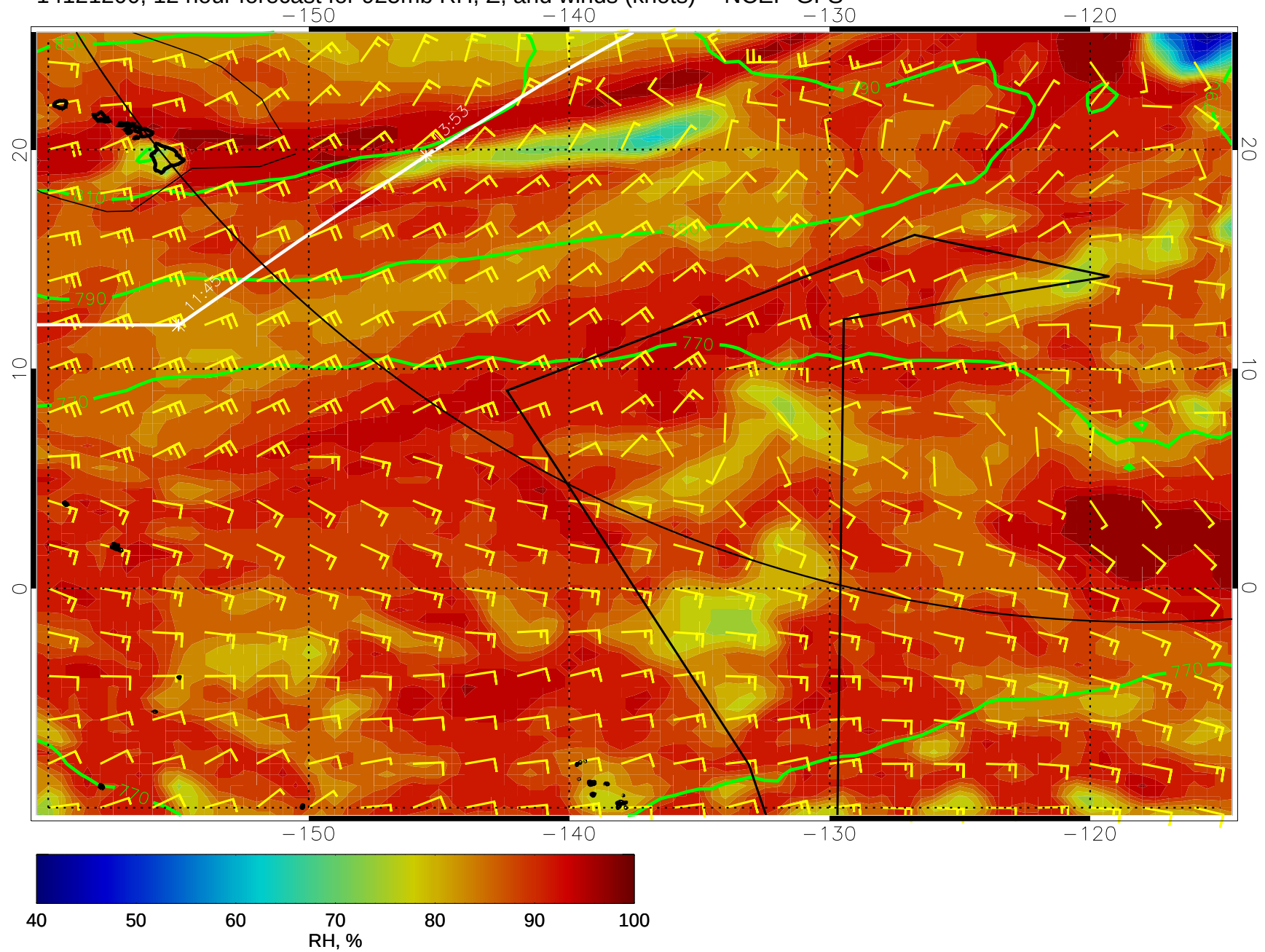
14121200, 12 hour forecast for 925mb RH, Z, and winds (knots) -- NCEP GFS
