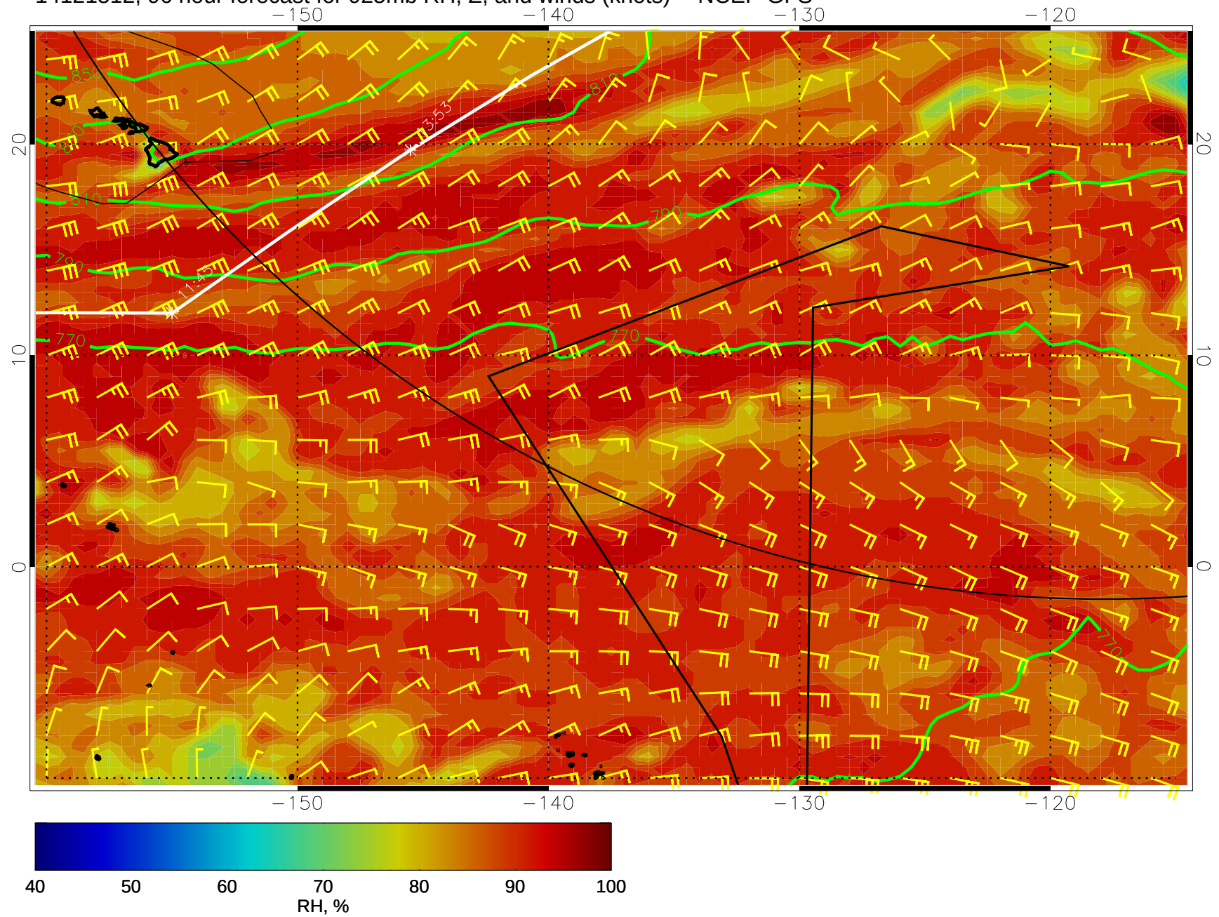
14121512, 96 hour forecast for 925mb RH, Z, and winds (knots) -- NCEP GFS
