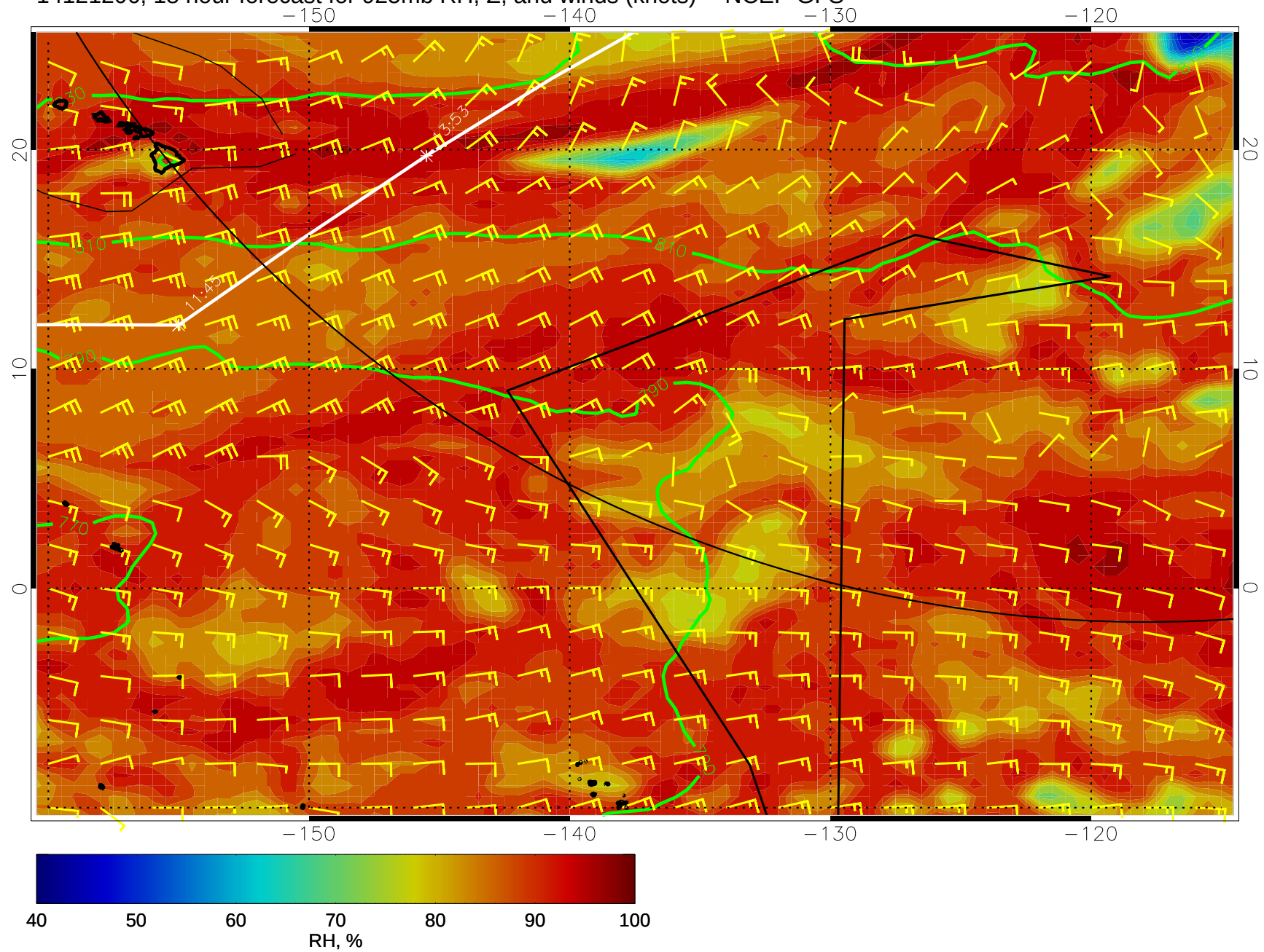
14121206, 18 hour forecast for 925mb RH, Z, and winds (knots) -- NCEP GFS
