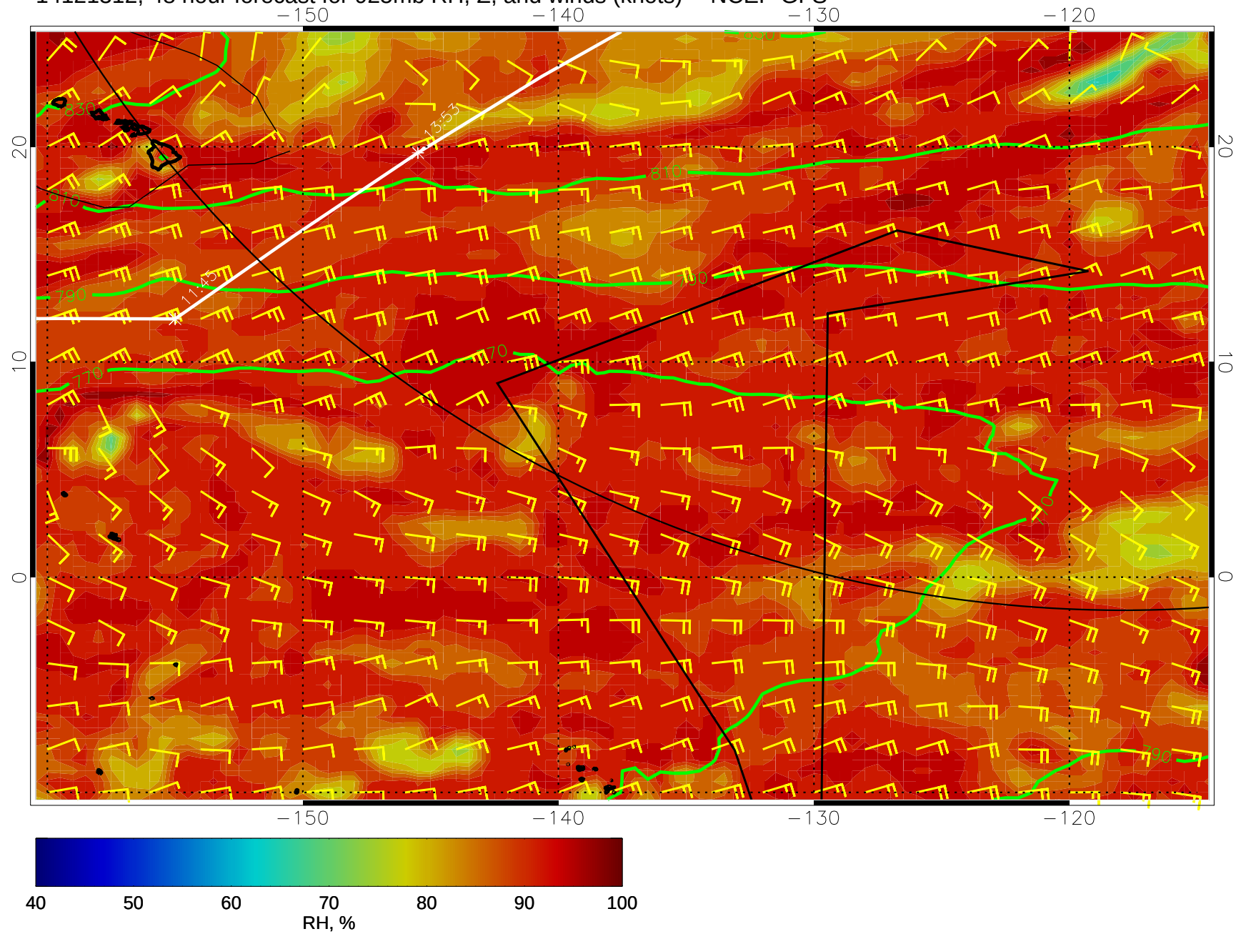
14121312, 48 hour forecast for 925mb RH, Z, and winds (knots) -- NCEP GFS
