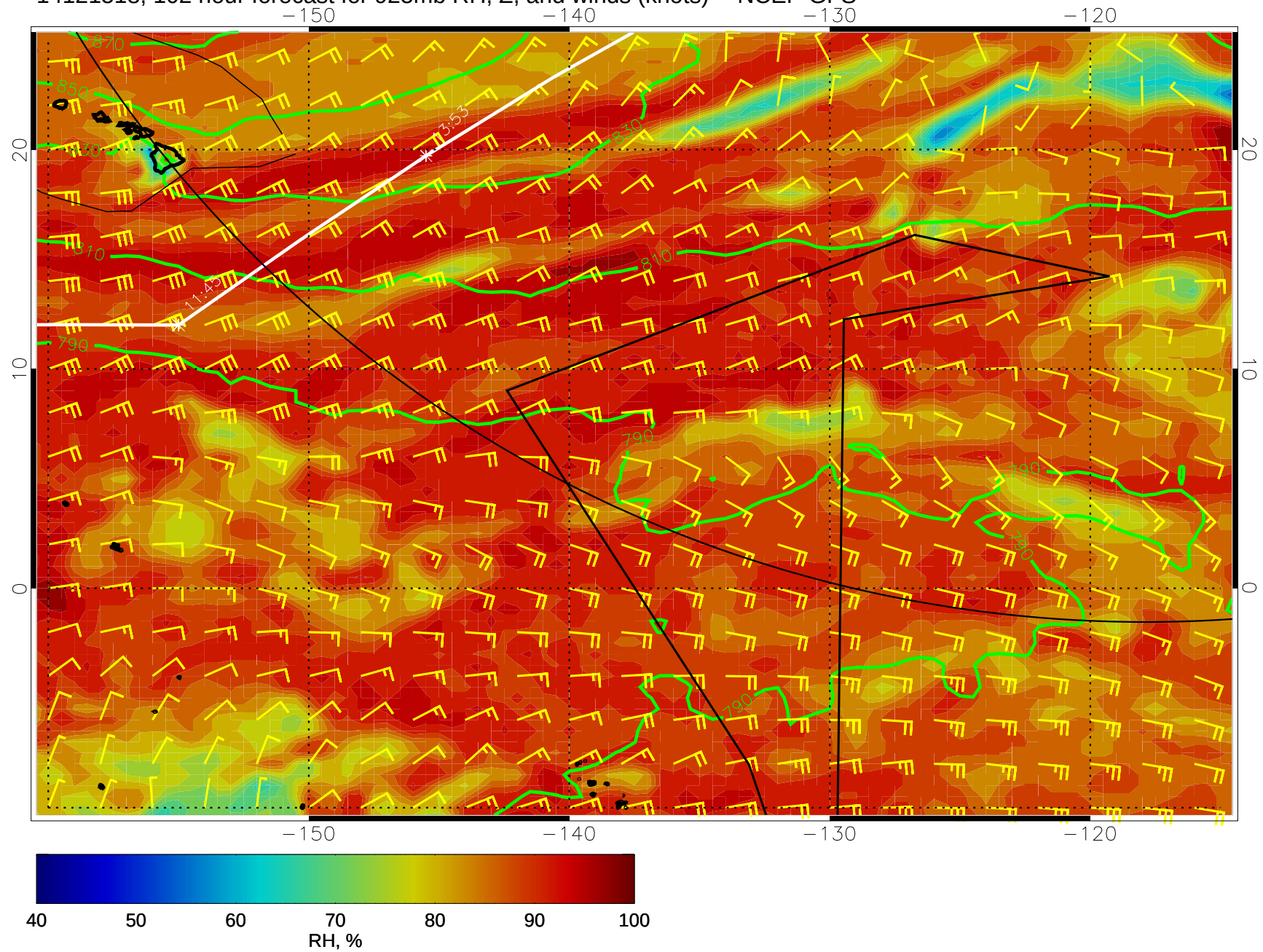
14121518, 102 hour forecast for 925mb RH, Z, and winds (knots) -- NCEP GFS
