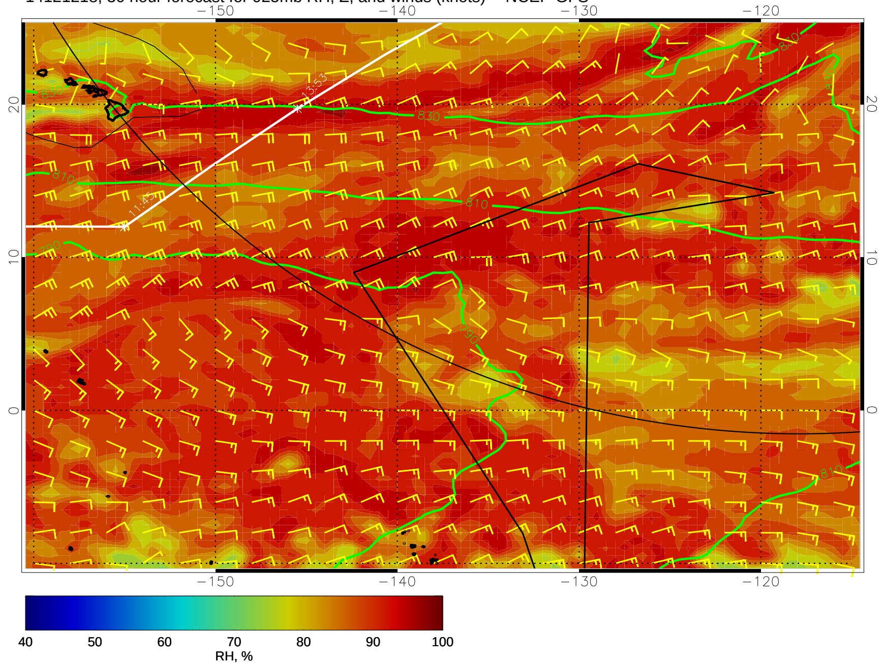
14121218, 30 hour forecast for 925mb RH, Z, and winds (knots) -- NCEP GFS
