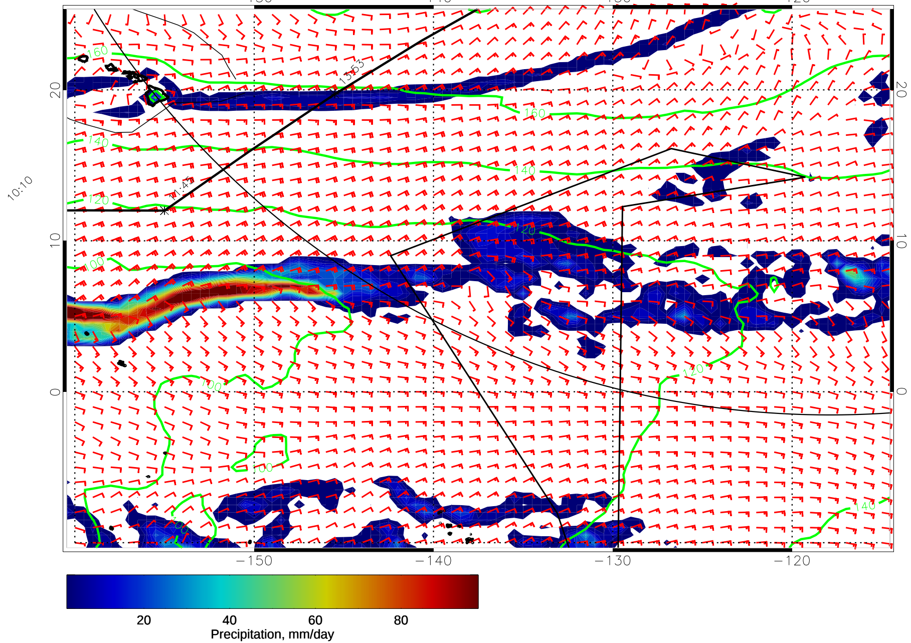
14121218, 30 hour forecast for precip, 1000mb Z, and winds (knots) -- NCEP GFS
