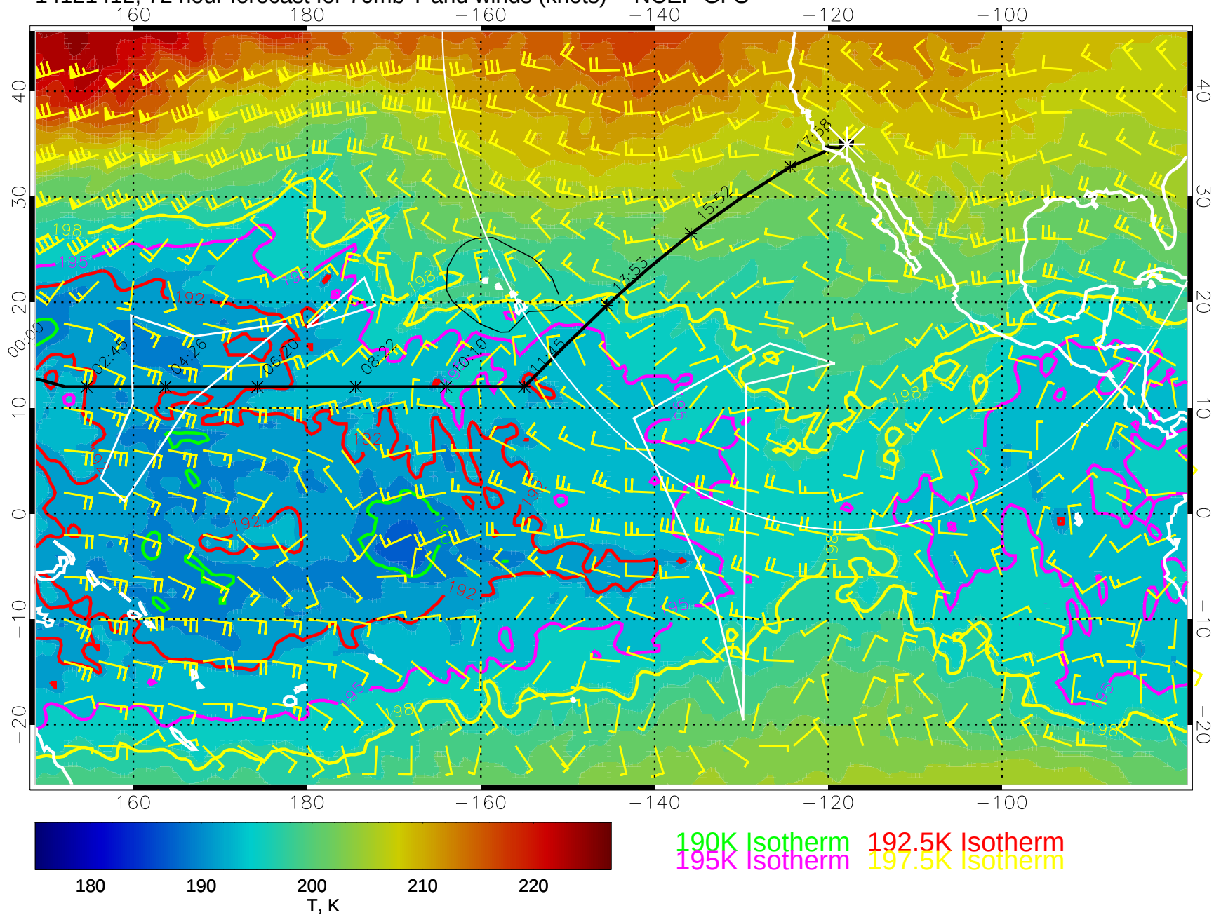
14121412, 72 hour forecast for 70mb T and winds (knots) -- NCEP GFS
