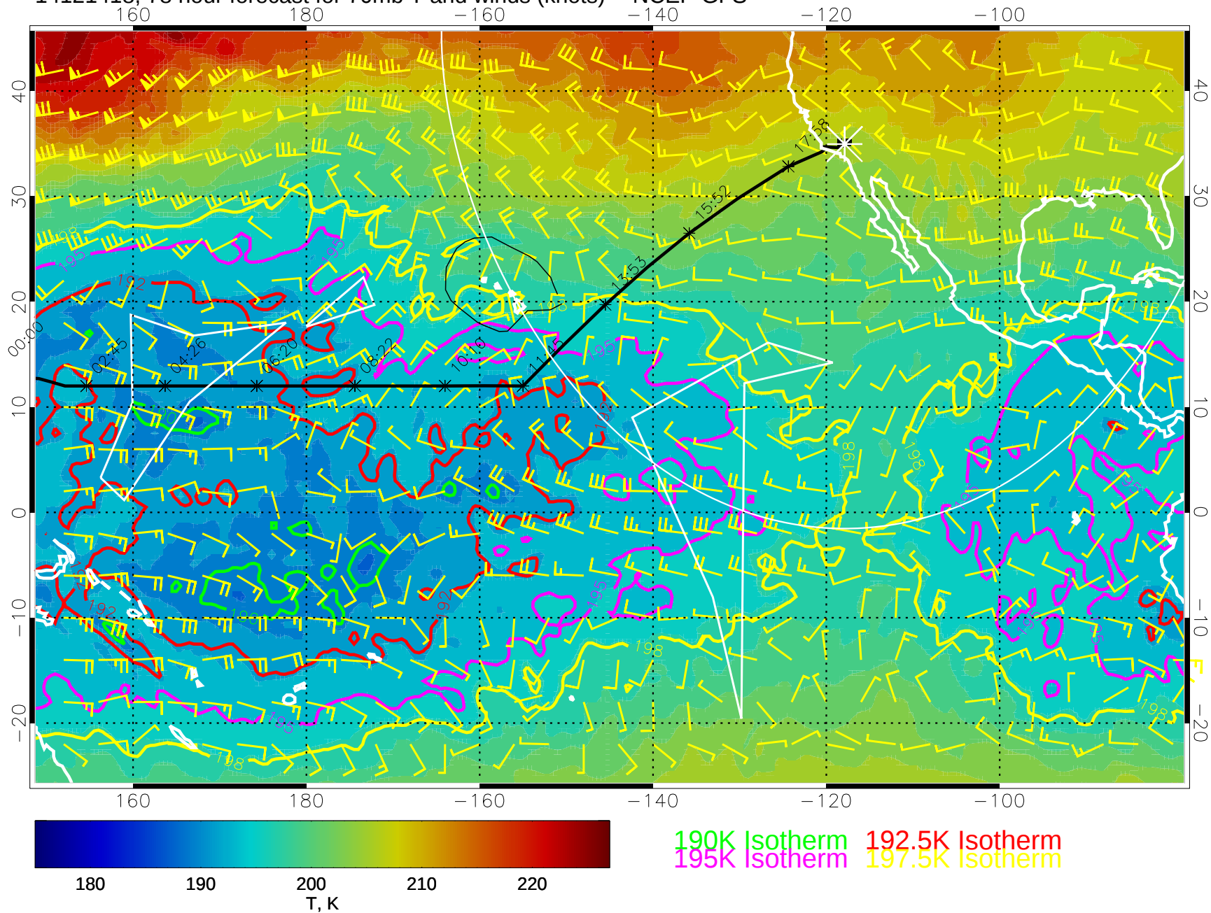
14121418, 78 hour forecast for 70mb T and winds (knots) -- NCEP GFS
