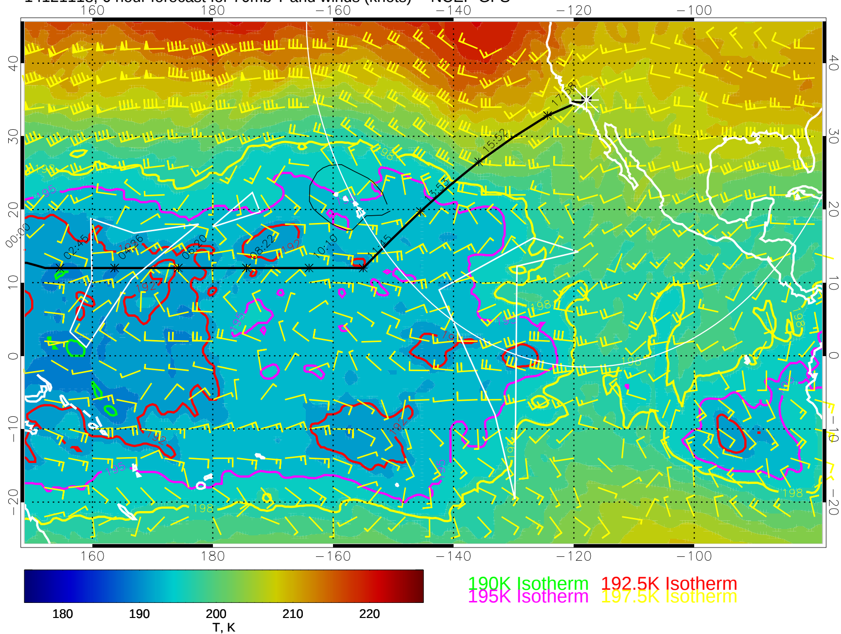
14121118, 6 hour forecast for 70mb T and winds (knots) -- NCEP GFS
