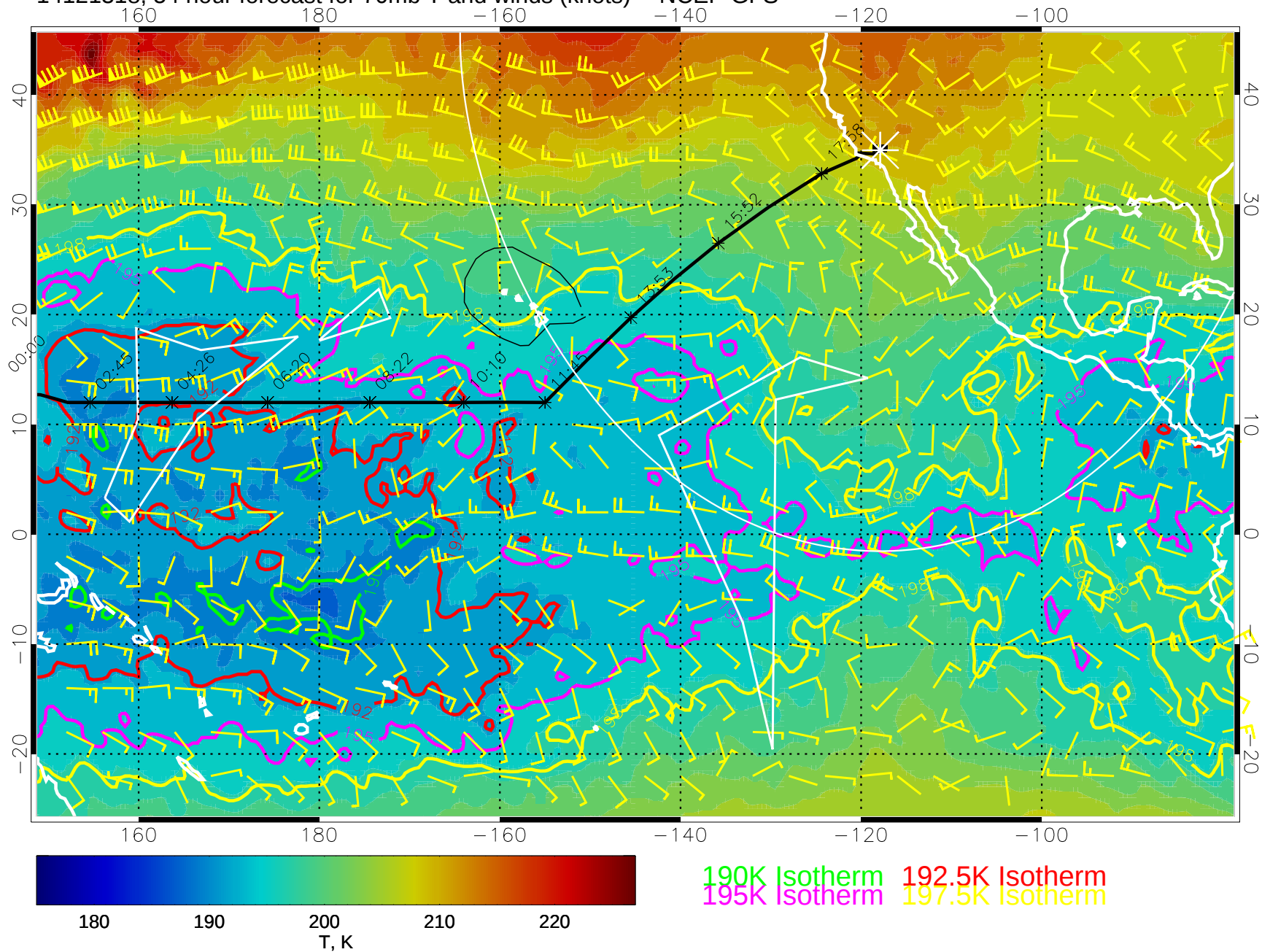
14121318, 54 hour forecast for 70mb T and winds (knots) -- NCEP GFS
