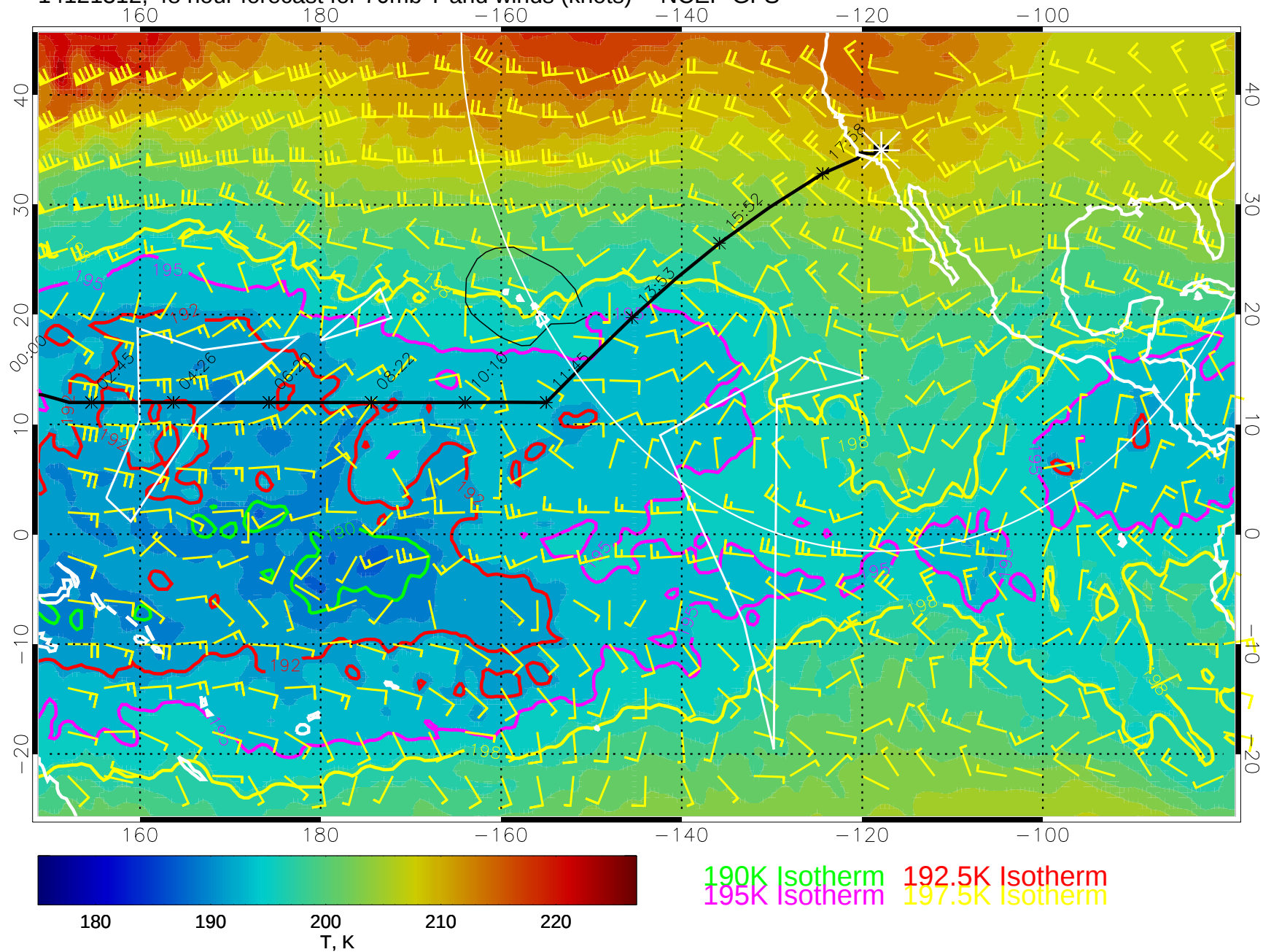
14121312, 48 hour forecast for 70mb T and winds (knots) -- NCEP GFS
