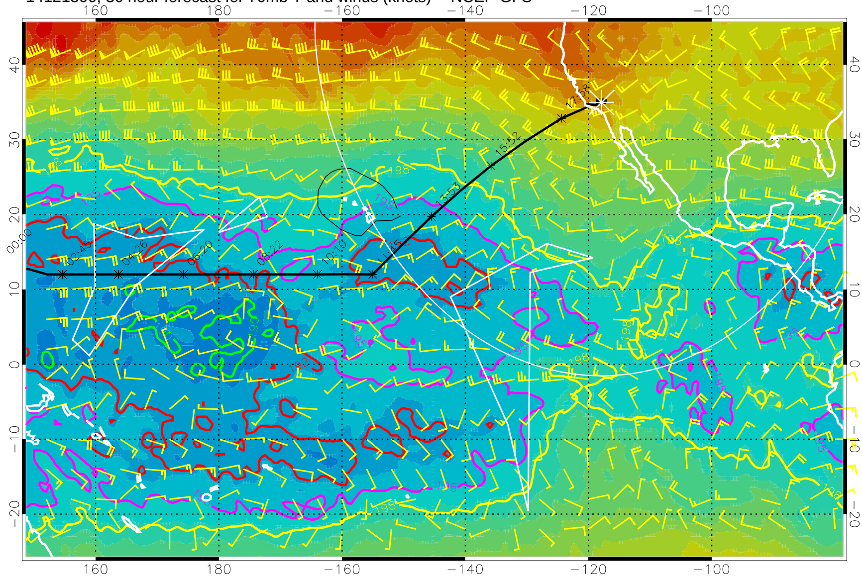
14121300, 36 hour forecast for 70mb T and winds (knots) -- NCEP GFS
