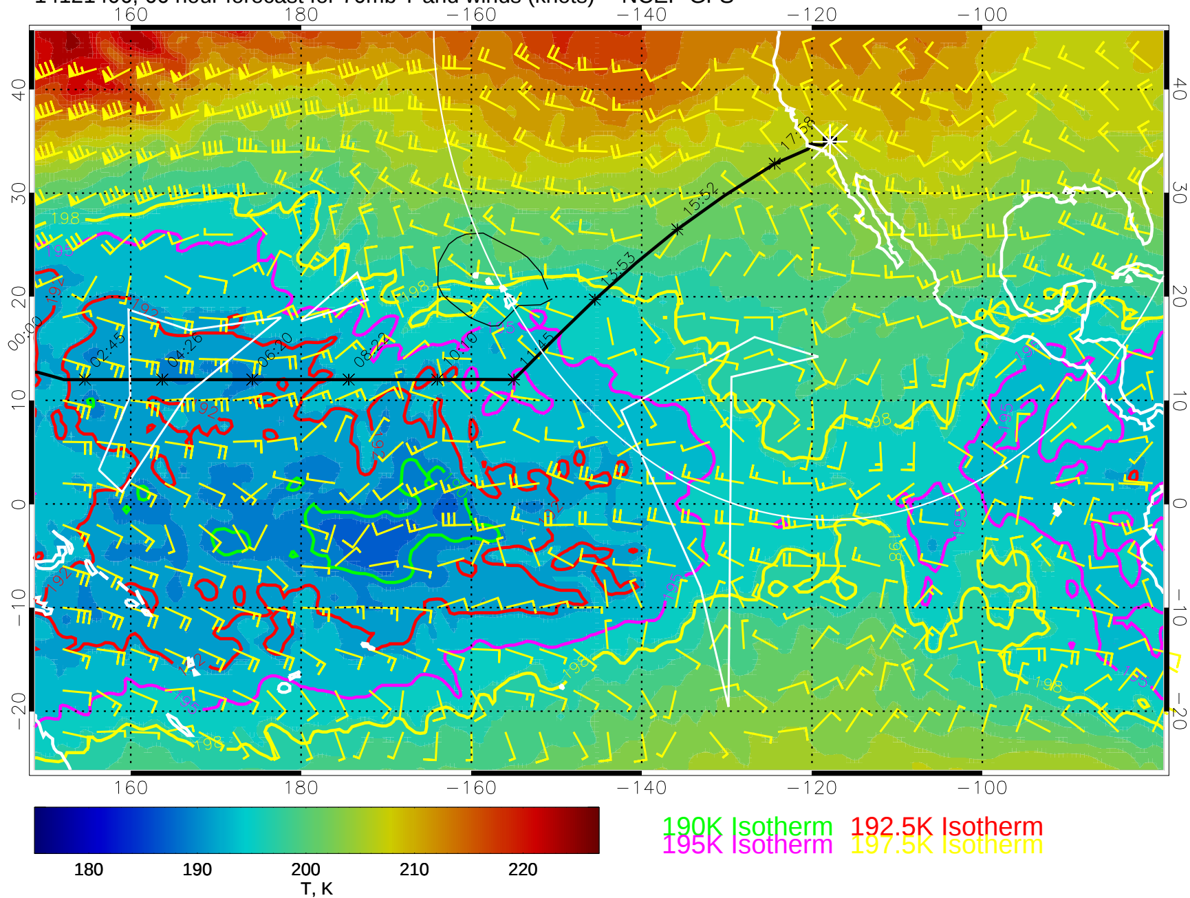
14121406, 66 hour forecast for 70mb T and winds (knots) -- NCEP GFS
