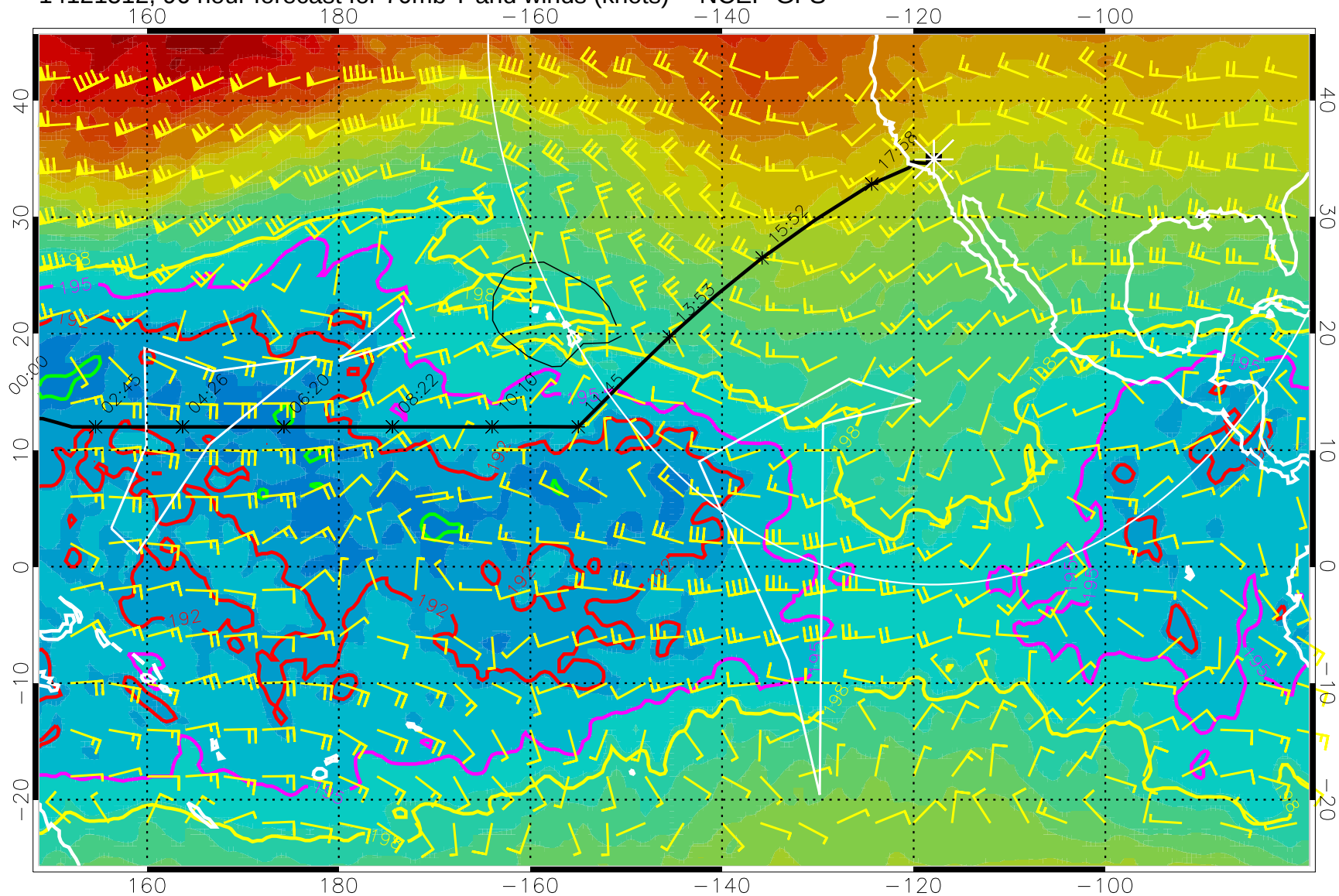
14121512, 96 hour forecast for 70mb T and winds (knots) -- NCEP GFS
