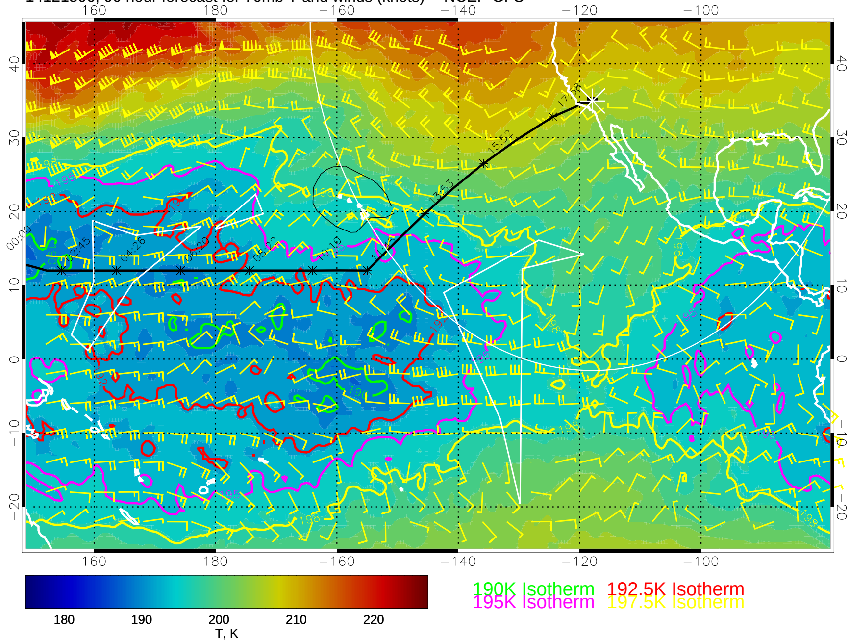
14121506, 90 hour forecast for 70mb T and winds (knots) -- NCEP GFS
