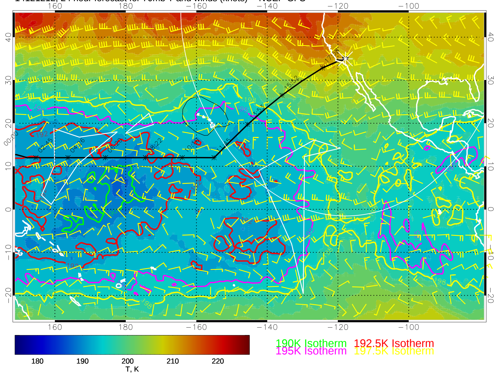
14121212, 24 hour forecast for 70mb T and winds (knots) -- NCEP GFS
