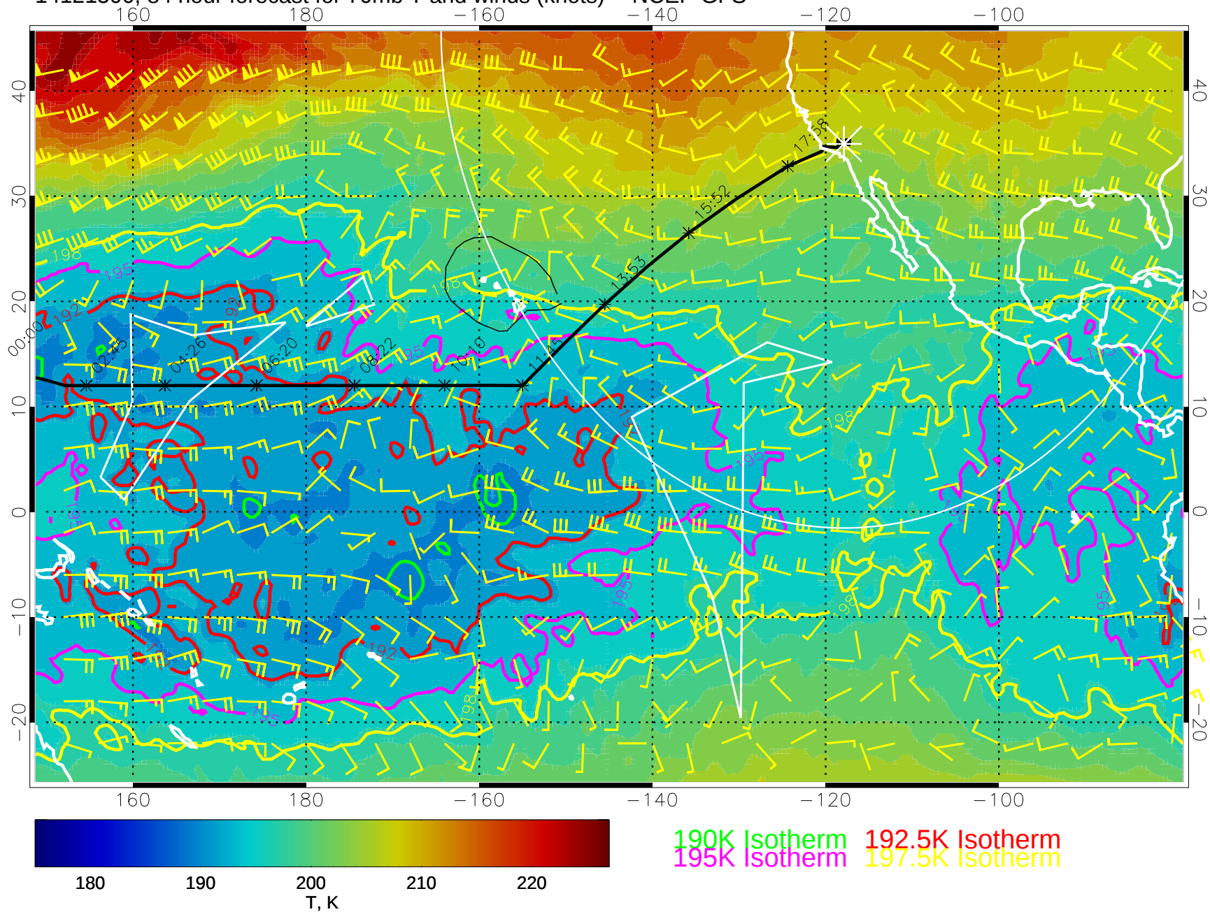
14121500, 84 hour forecast for 70mb T and winds (knots) -- NCEP GFS
