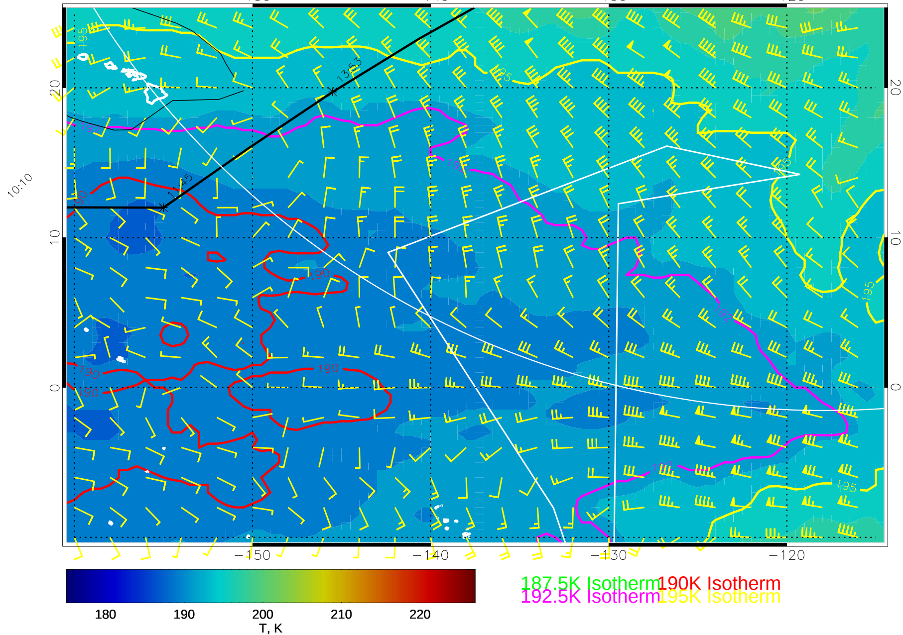
14121212, 24 hour forecast for 100mb T and winds (knots) -- NCEP GFS
