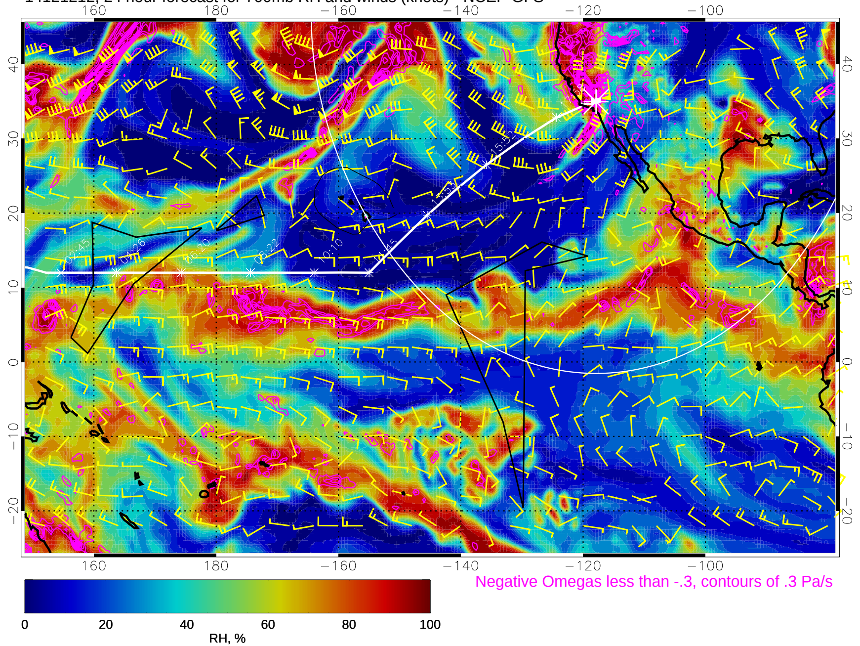
14121212, 24 hour forecast for 700mb RH and winds (knots) - NCEP GFS
