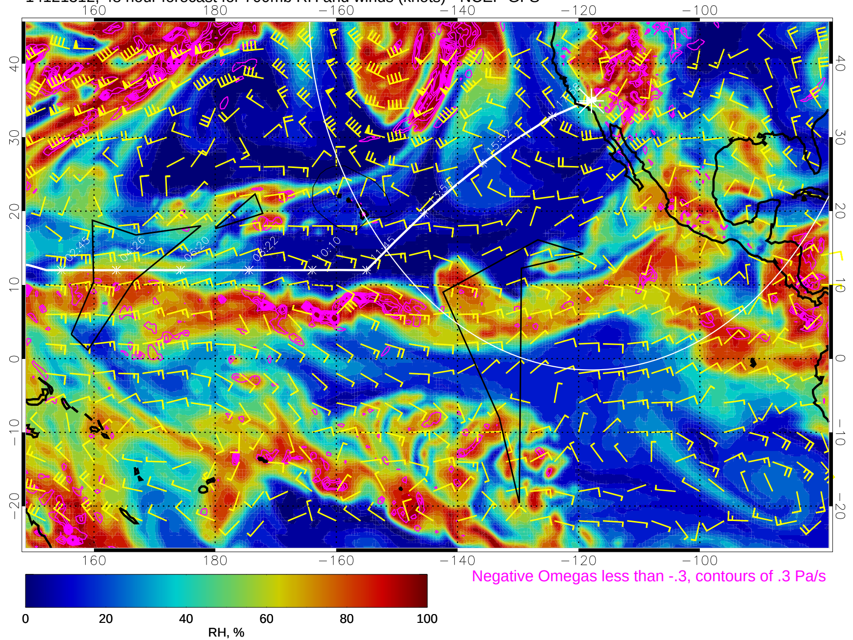
14121312, 48 hour forecast for 700mb RH and winds (knots) - NCEP GFS
