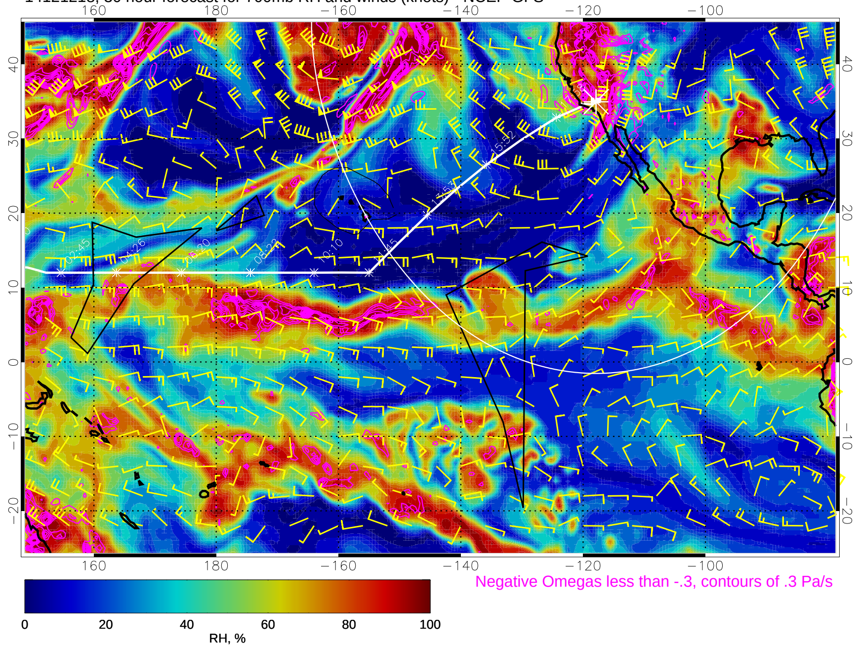
14121218, 30 hour forecast for 700mb RH and winds (knots) - NCEP GFS
