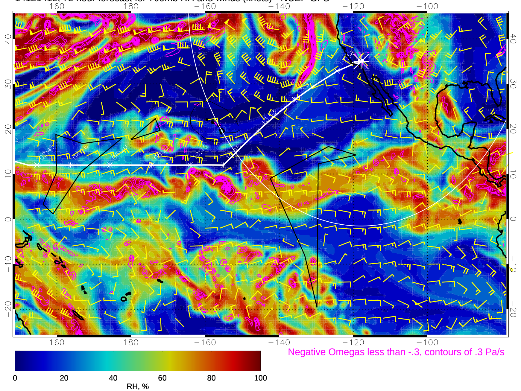
14121412, 72 hour forecast for 700mb RH and winds (knots) - NCEP GFS
