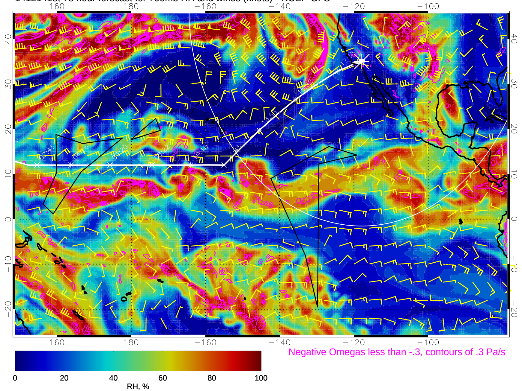
14121418, 78 hour forecast for 700mb RH and winds (knots) - NCEP GFS
