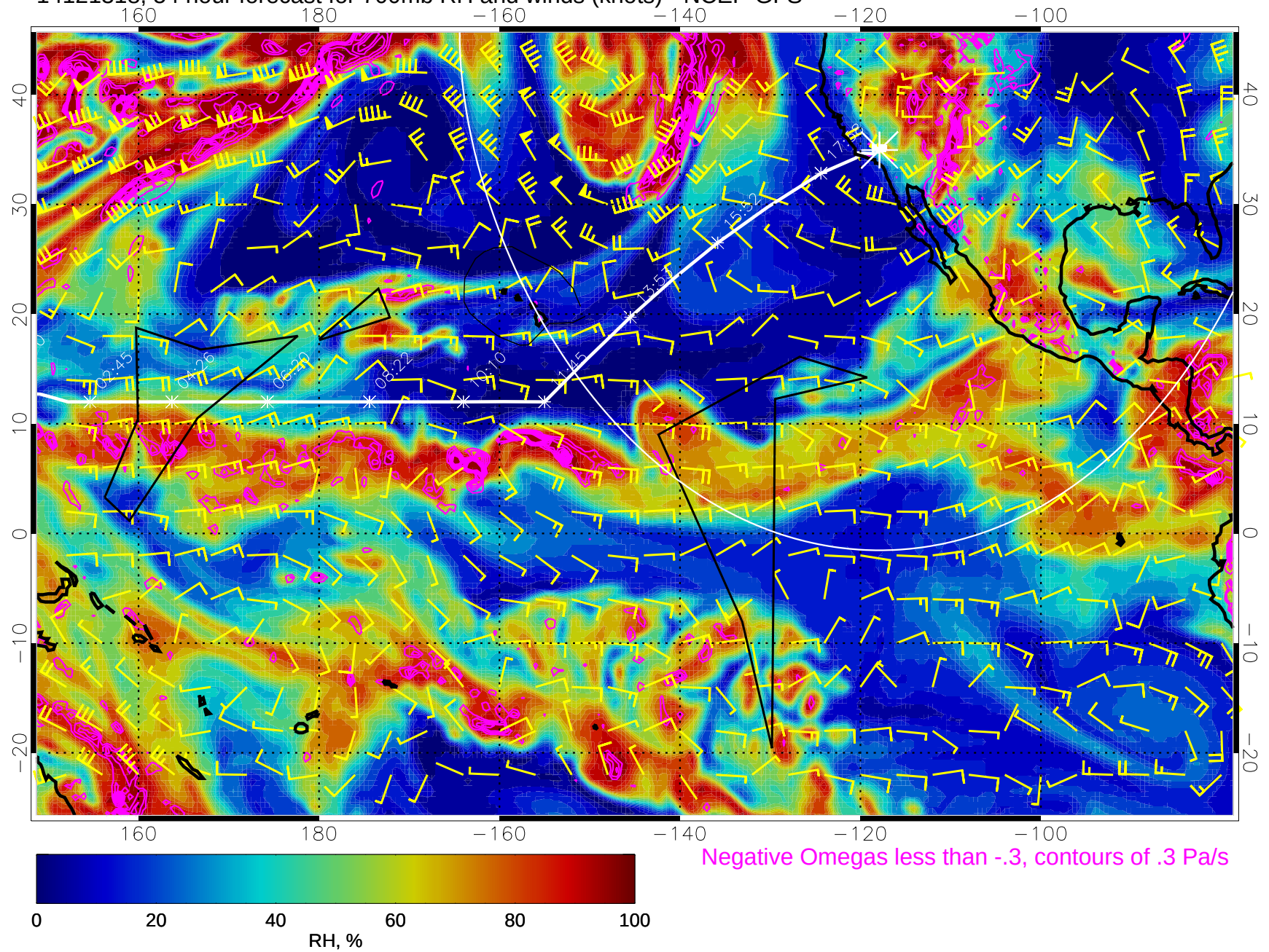
14121318, 54 hour forecast for 700mb RH and winds (knots) - NCEP GFS
