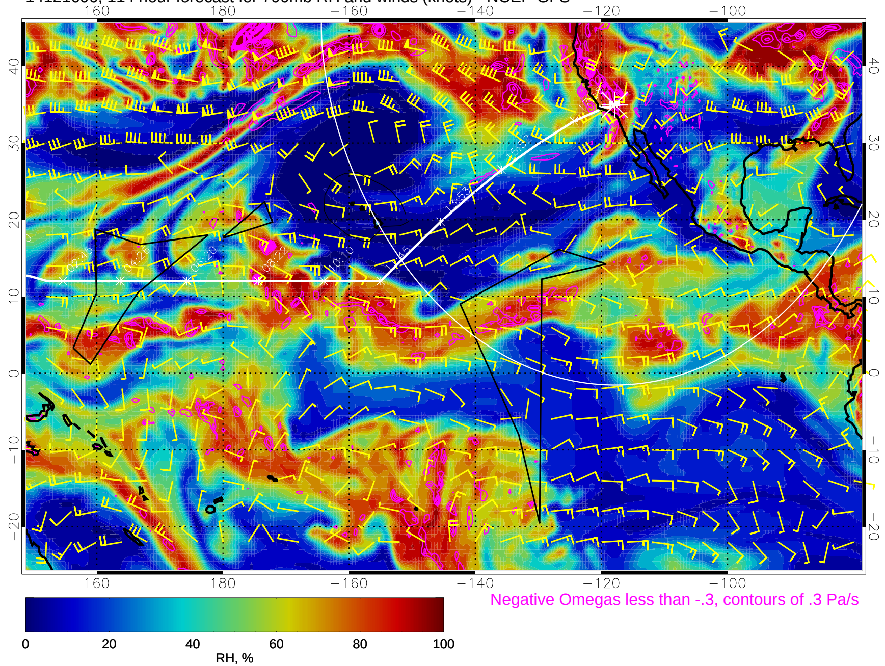
14121606, 114 hour forecast for 700mb RH and winds (knots) - NCEP GFS
