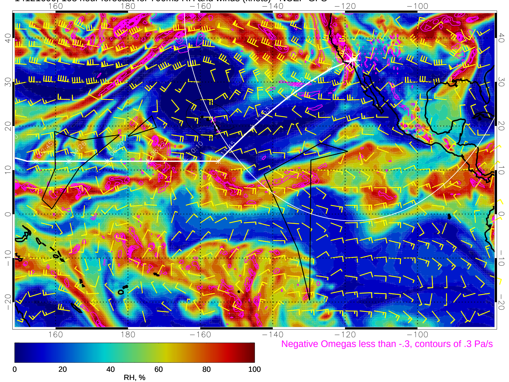
14121600, 108 hour forecast for 700mb RH and winds (knots) - NCEP GFS
