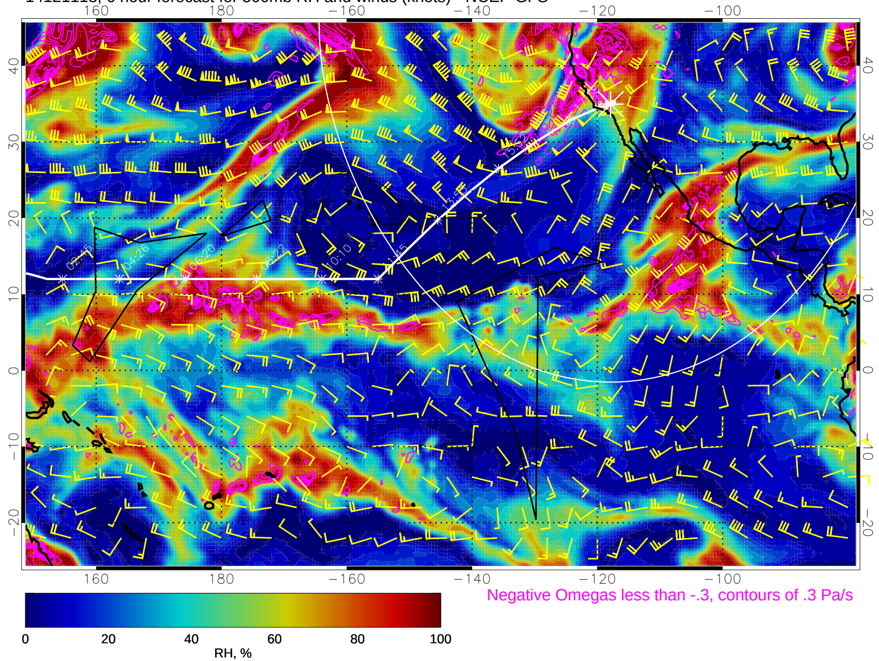
14121118, 6 hour forecast for 500mb RH and winds (knots) - NCEP GFS
