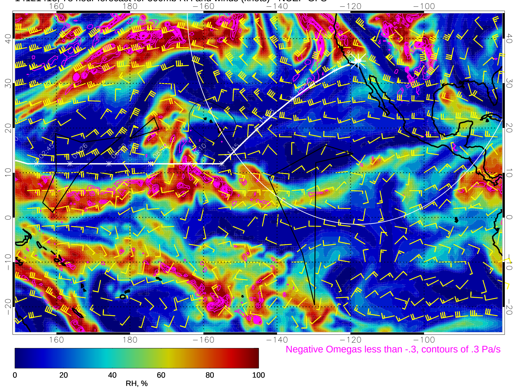
14121418, 78 hour forecast for 500mb RH and winds (knots) - NCEP GFS
