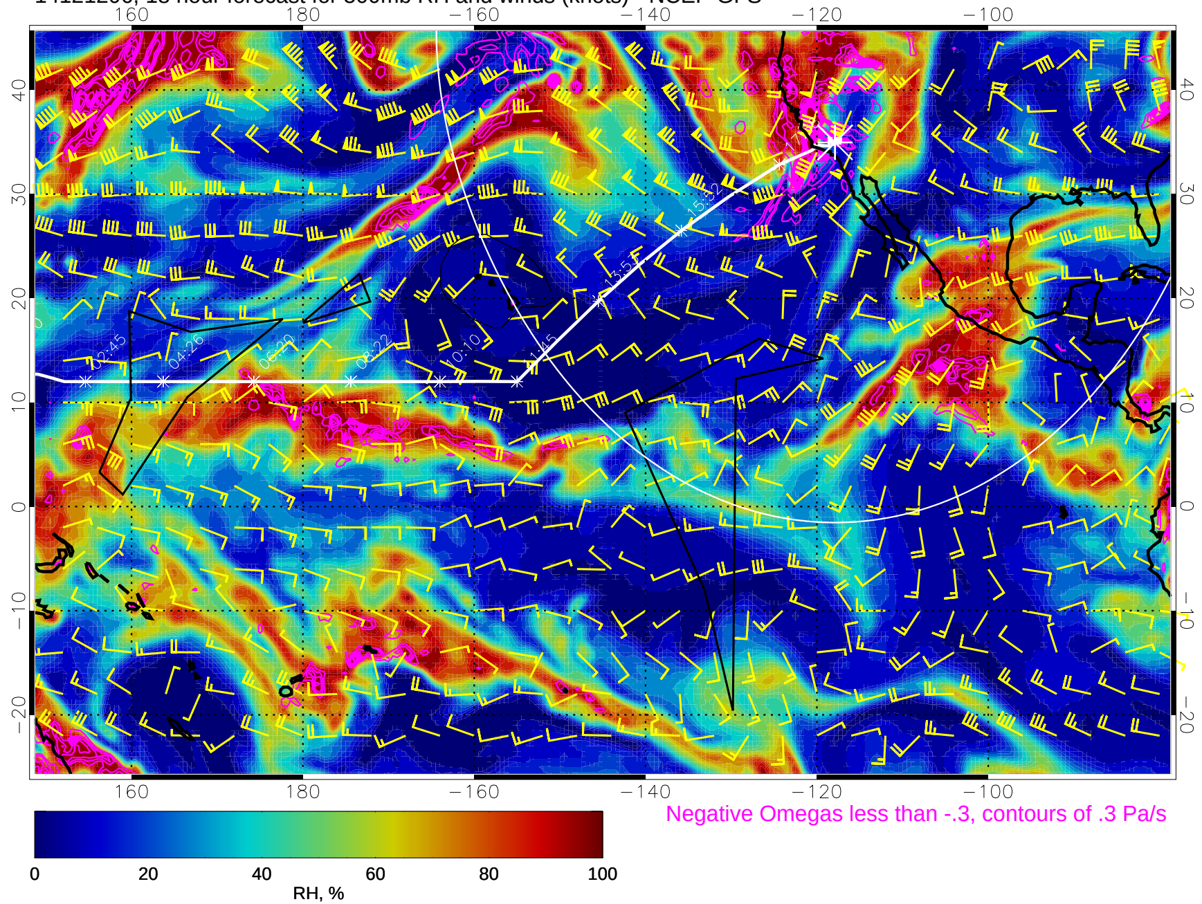
14121206, 18 hour forecast for 500mb RH and winds (knots) - NCEP GFS
