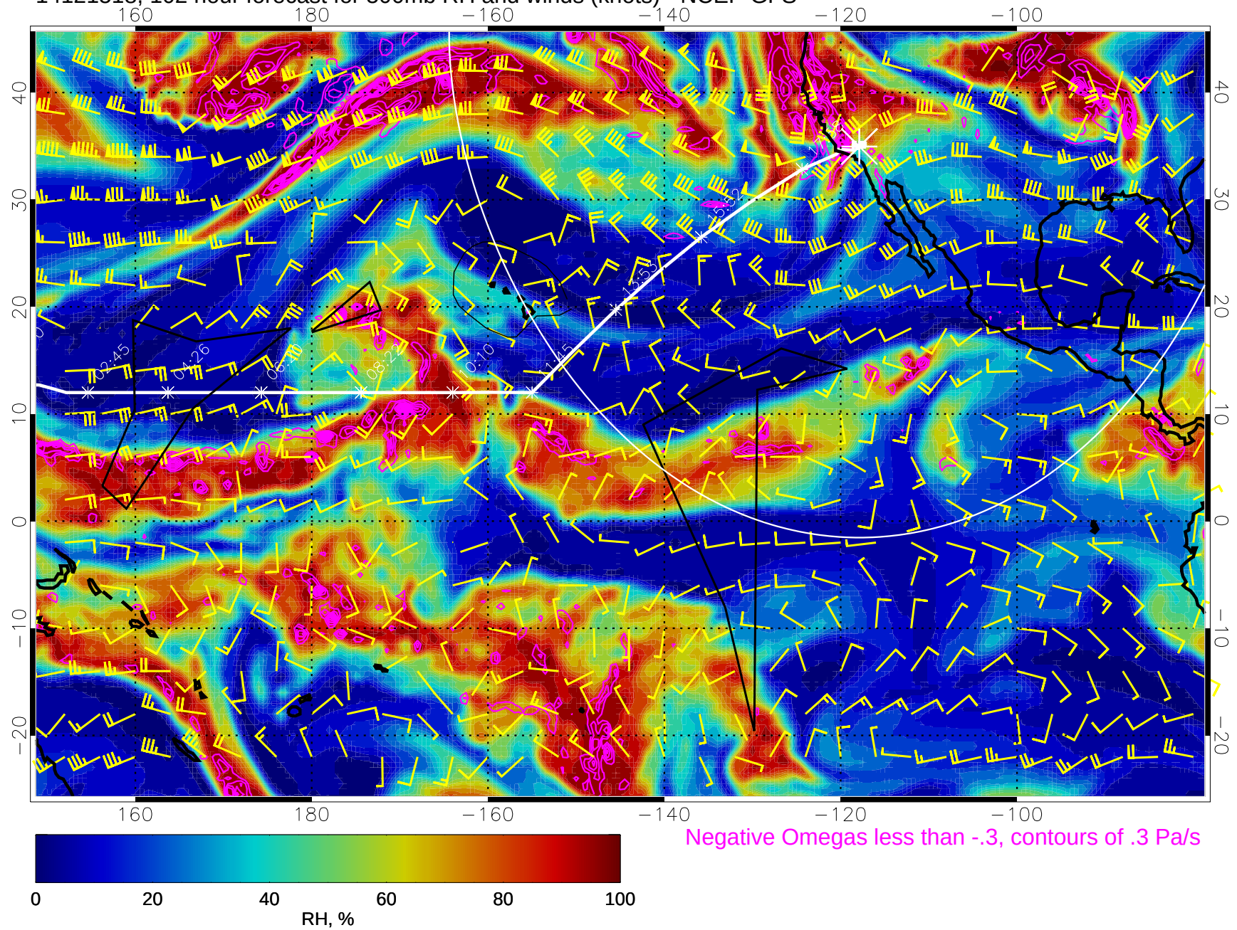
14121518, 102 hour forecast for 500mb RH and winds (knots) - NCEP GFS
