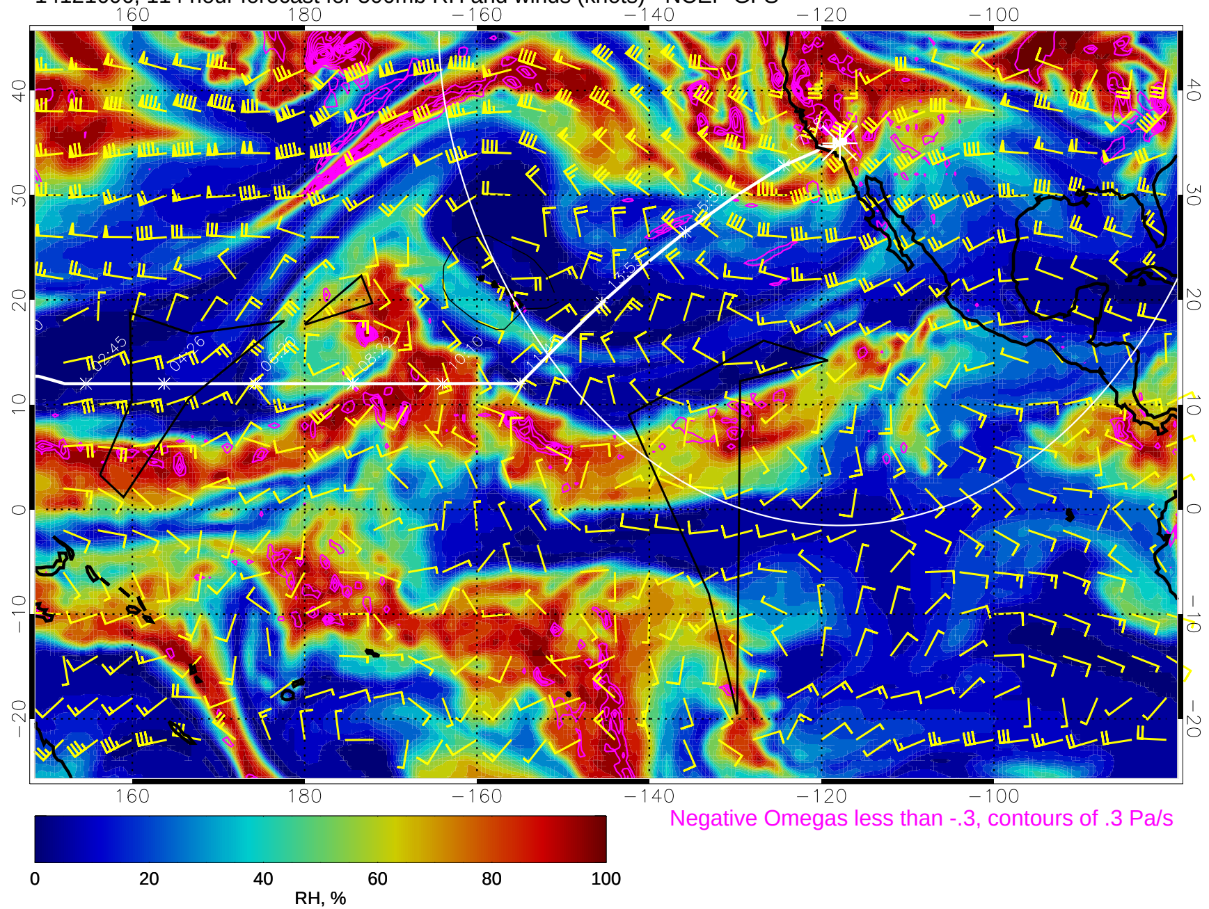
14121606, 114 hour forecast for 500mb RH and winds (knots) - NCEP GFS
