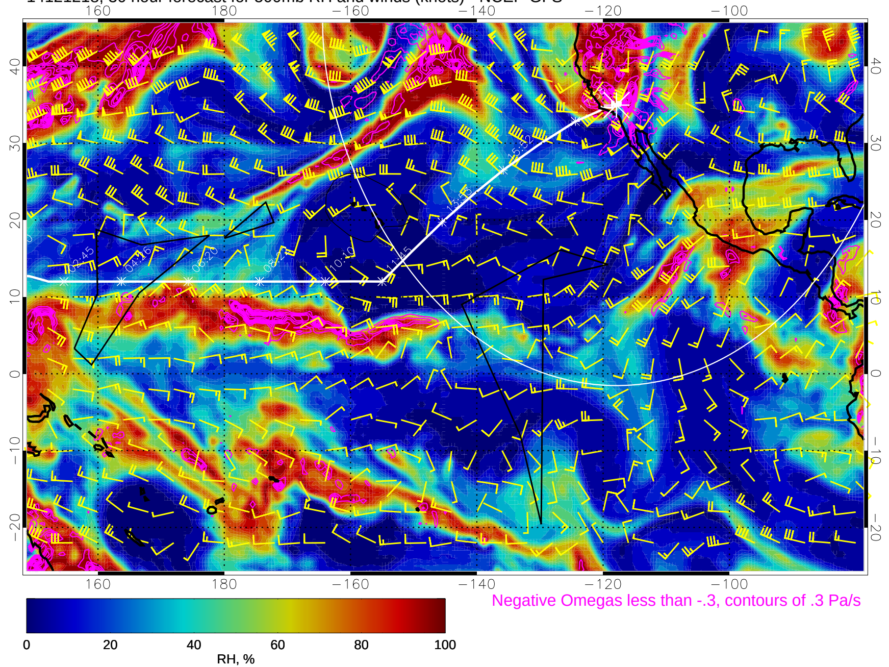
14121218, 30 hour forecast for 500mb RH and winds (knots) - NCEP GFS
