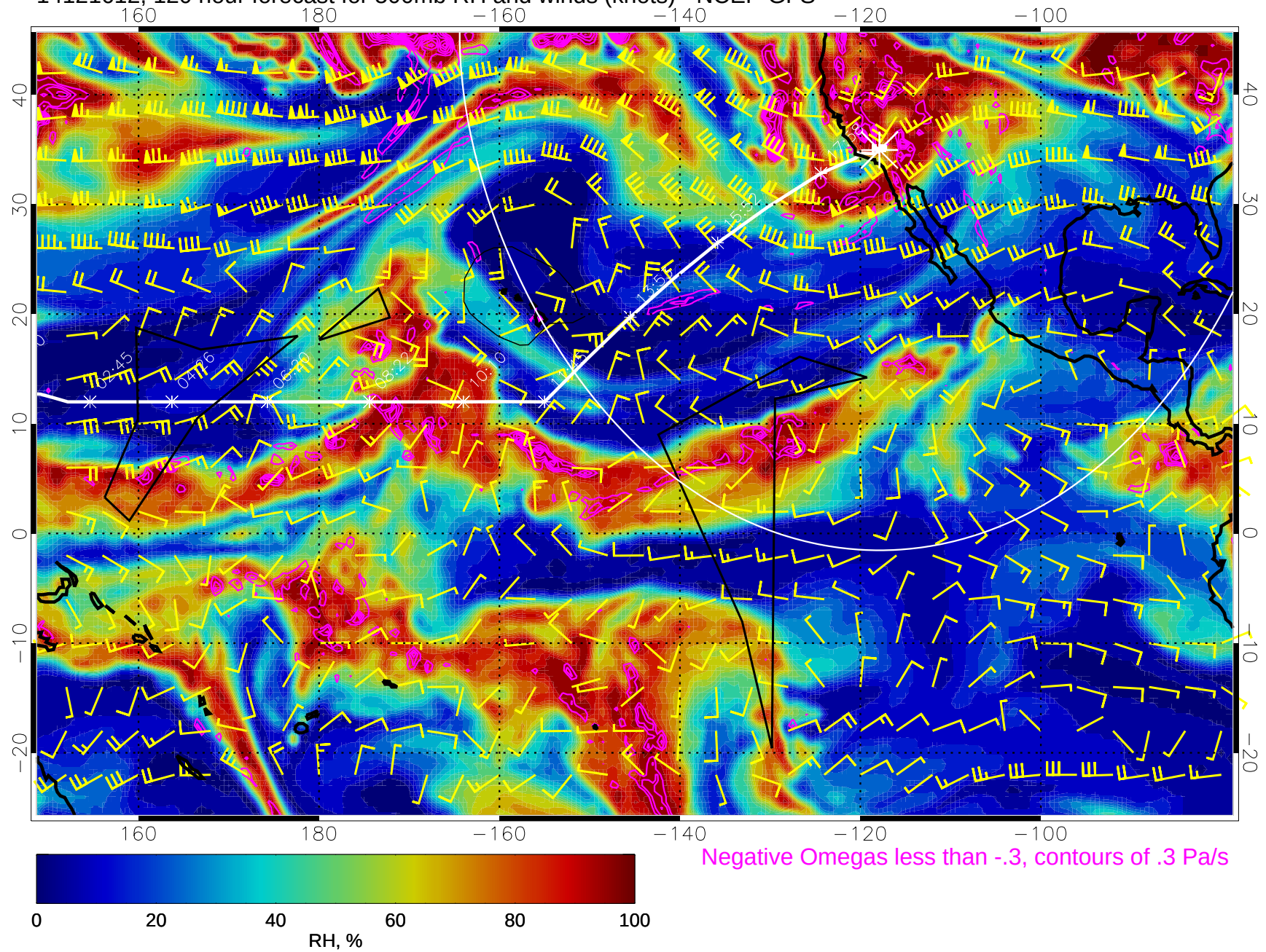
14121612, 120 hour forecast for 500mb RH and winds (knots) - NCEP GFS
