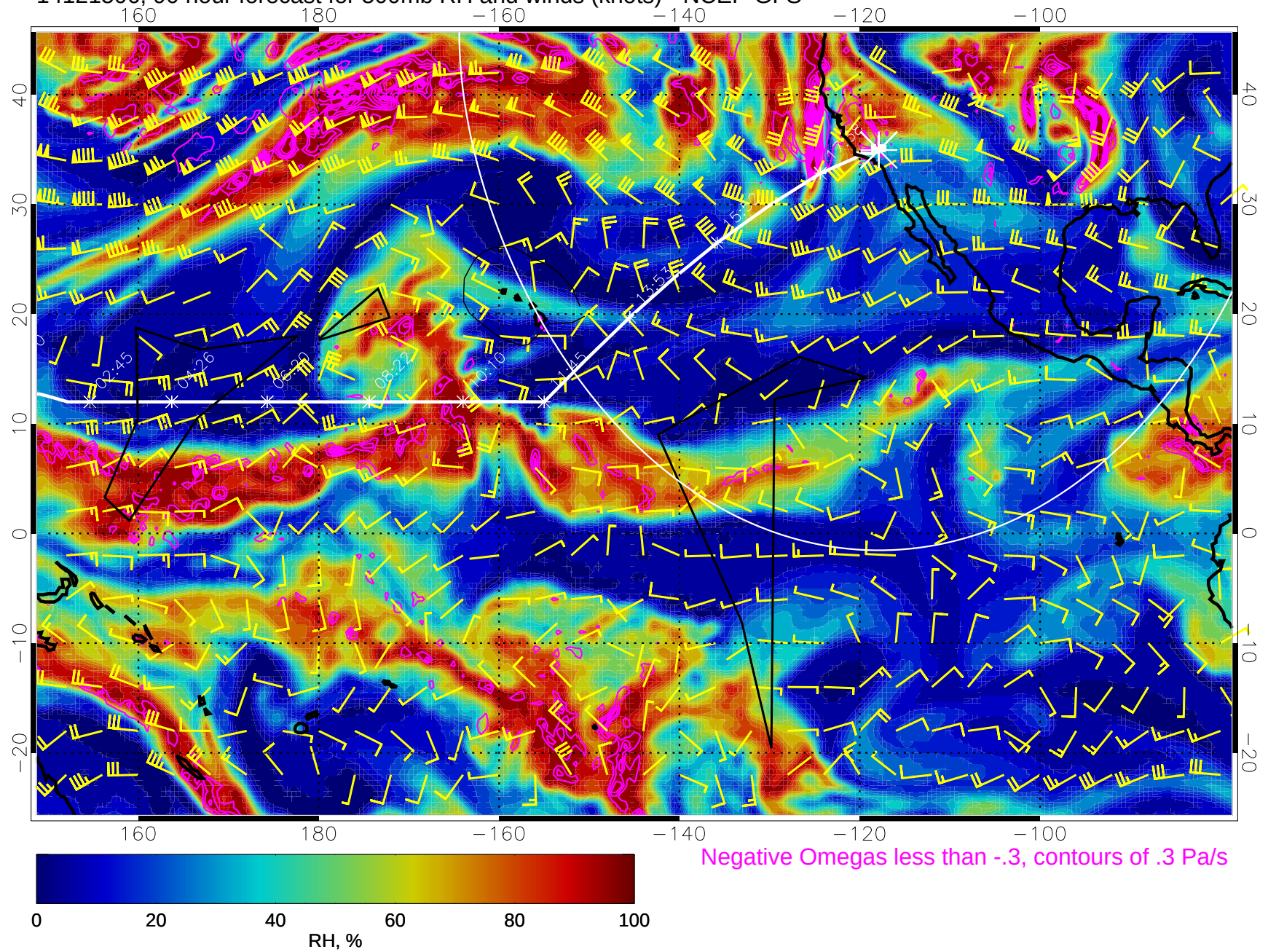
14121506, 90 hour forecast for 500mb RH and winds (knots) - NCEP GFS
