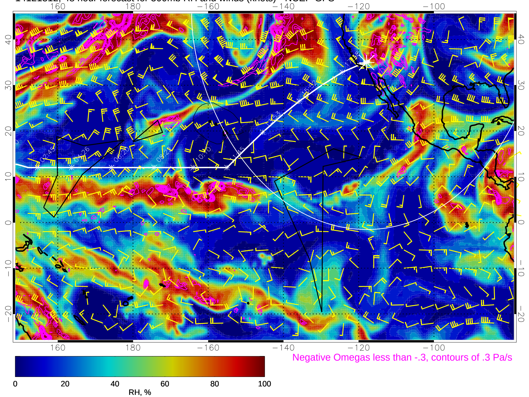
14121312, 48 hour forecast for 500mb RH and winds (knots) - NCEP GFS
