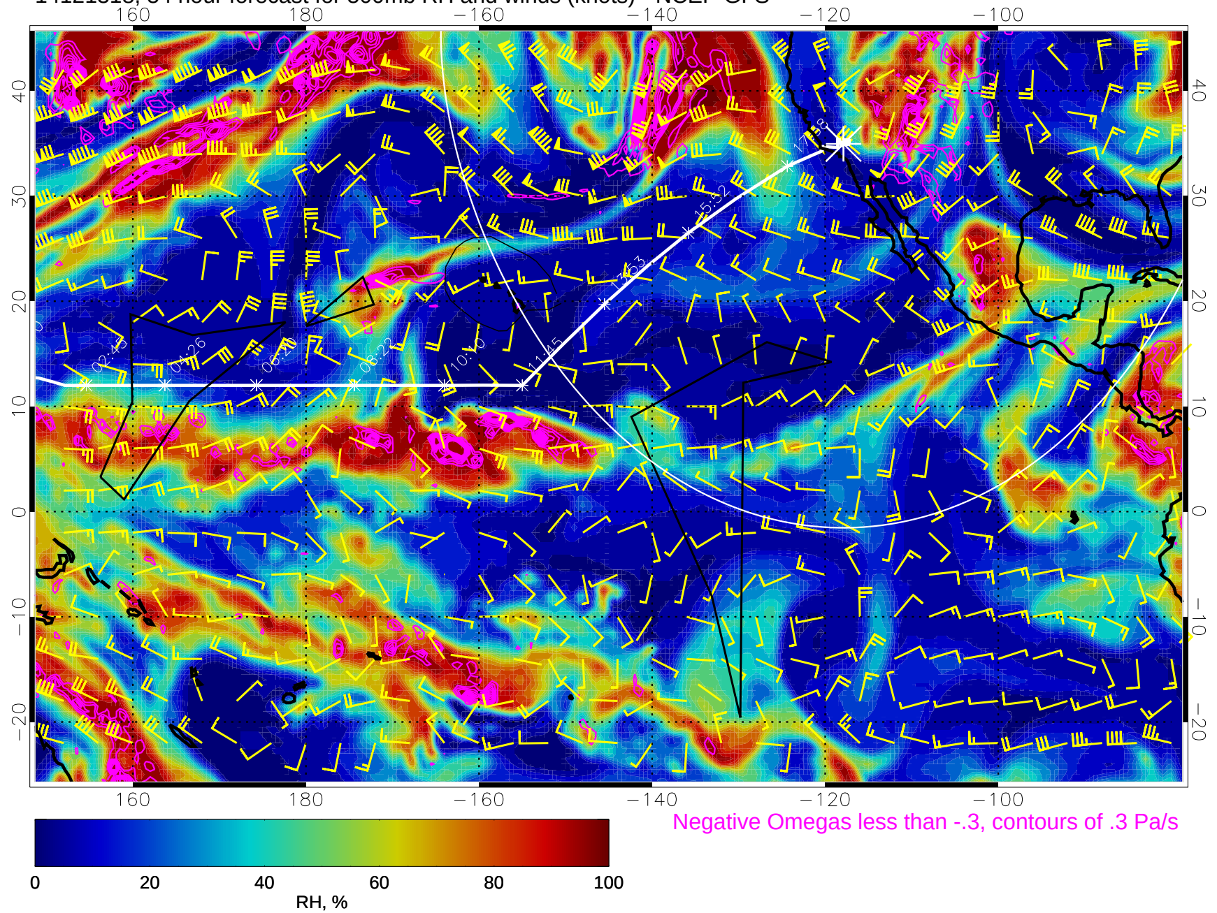
14121318, 54 hour forecast for 500mb RH and winds (knots) - NCEP GFS
