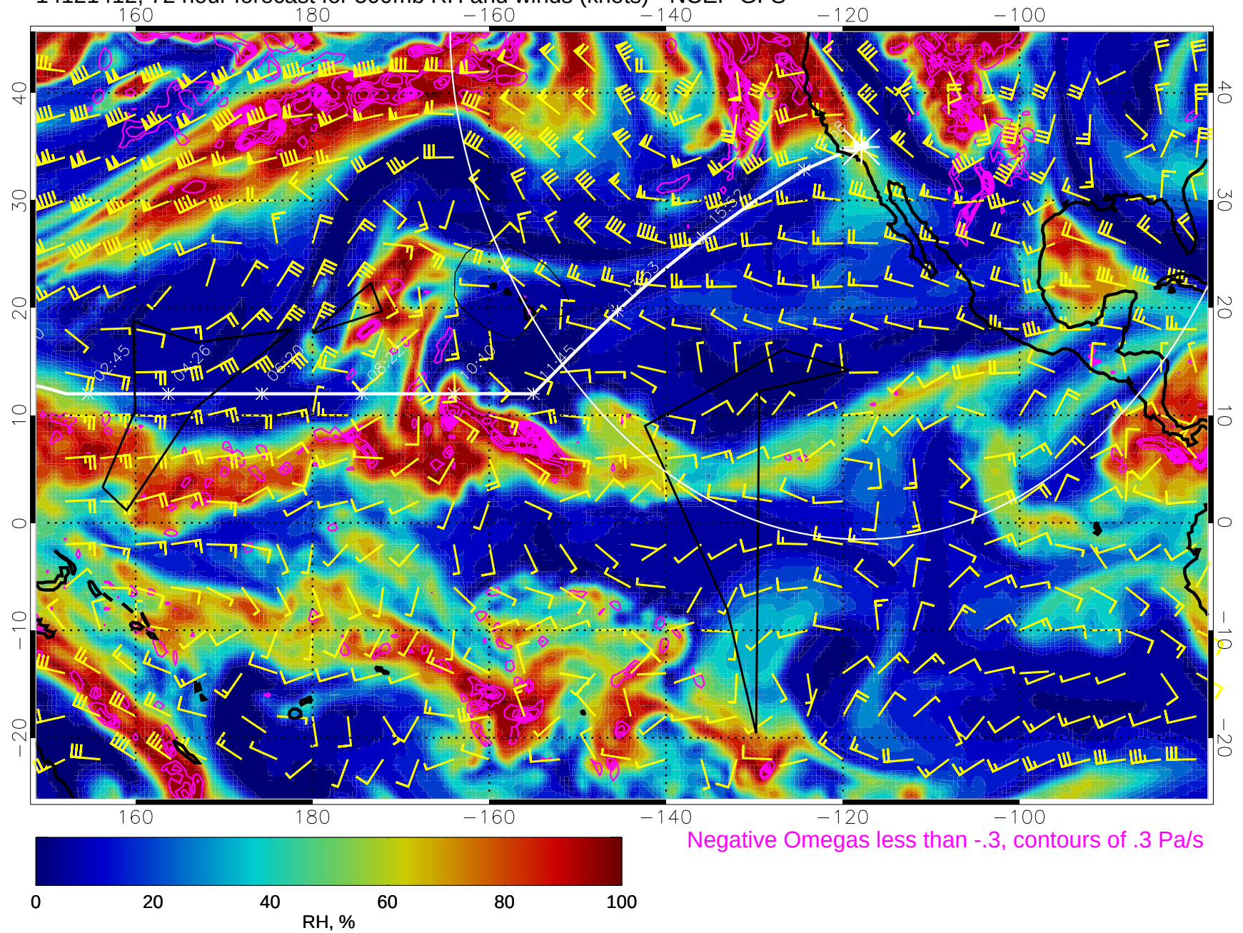
14121412, 72 hour forecast for 500mb RH and winds (knots) - NCEP GFS
