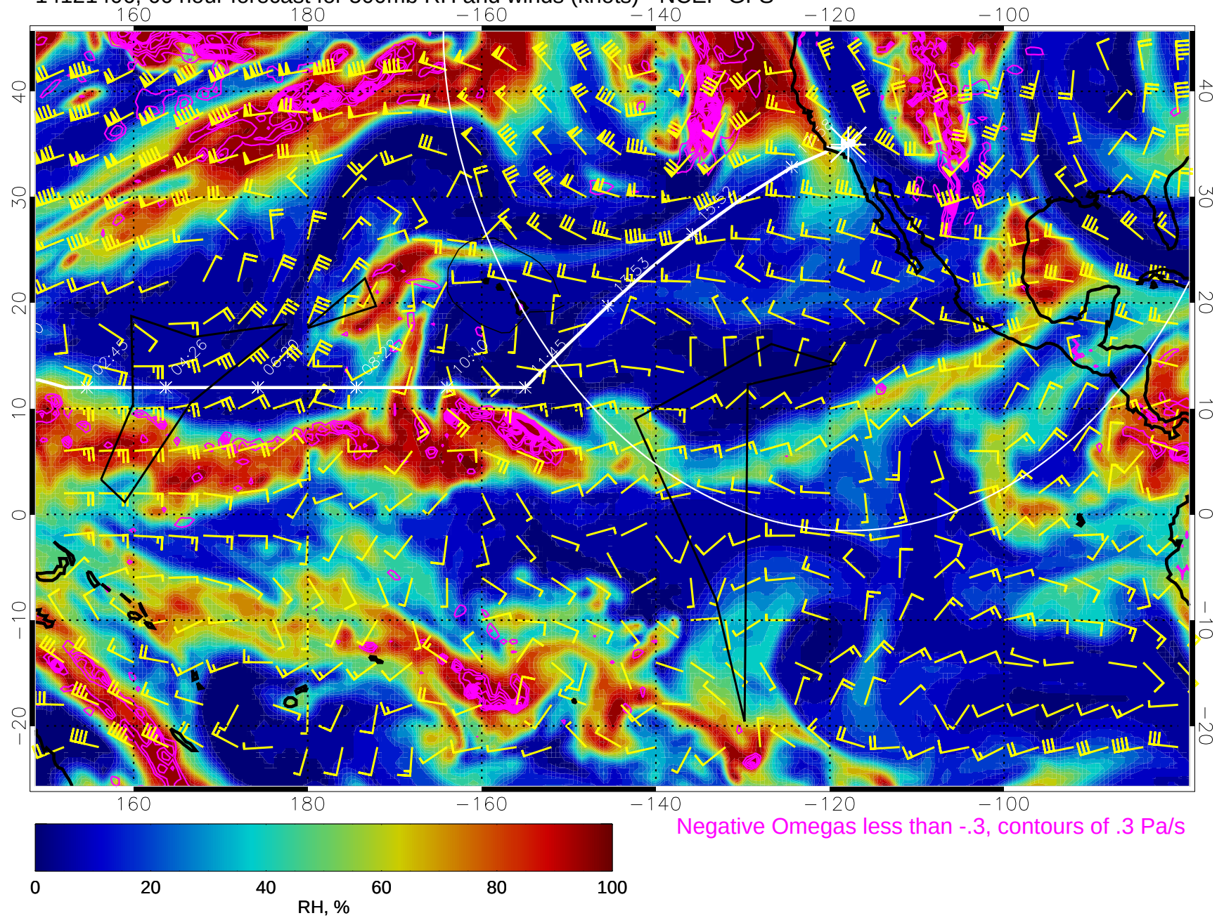
14121406, 66 hour forecast for 500mb RH and winds (knots) - NCEP GFS
