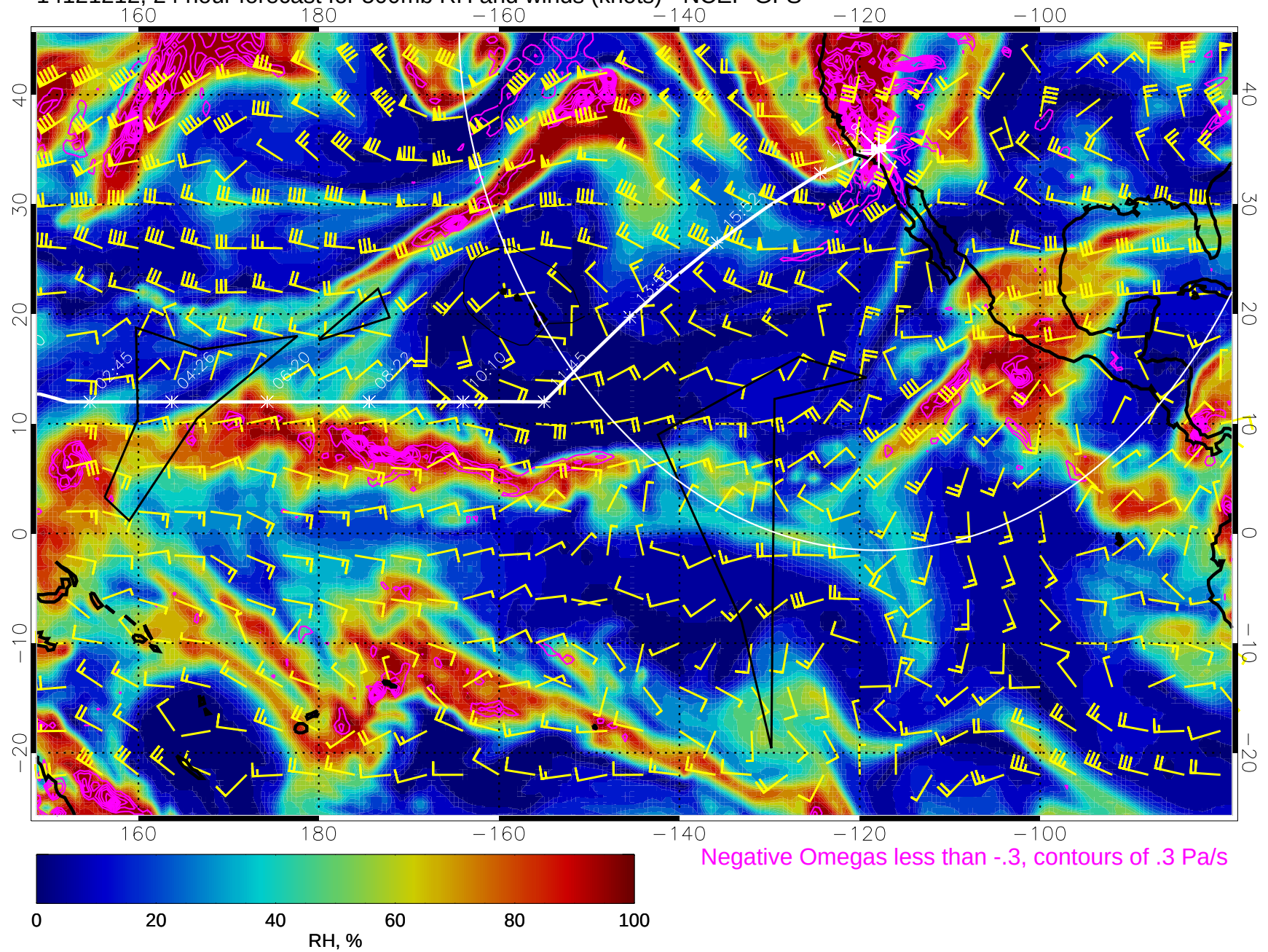
14121212, 24 hour forecast for 500mb RH and winds (knots) - NCEP GFS
