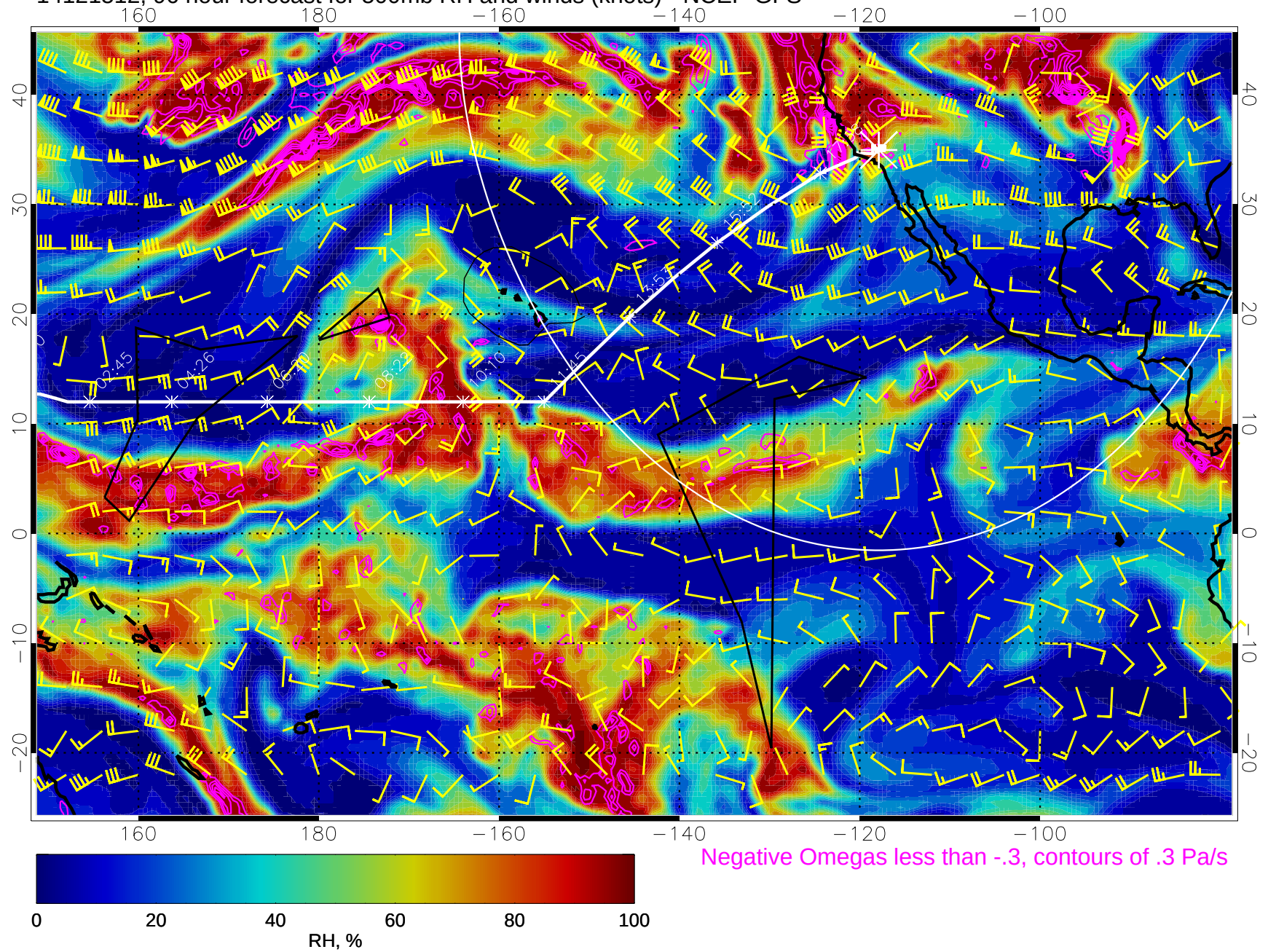
14121512, 96 hour forecast for 500mb RH and winds (knots) - NCEP GFS
