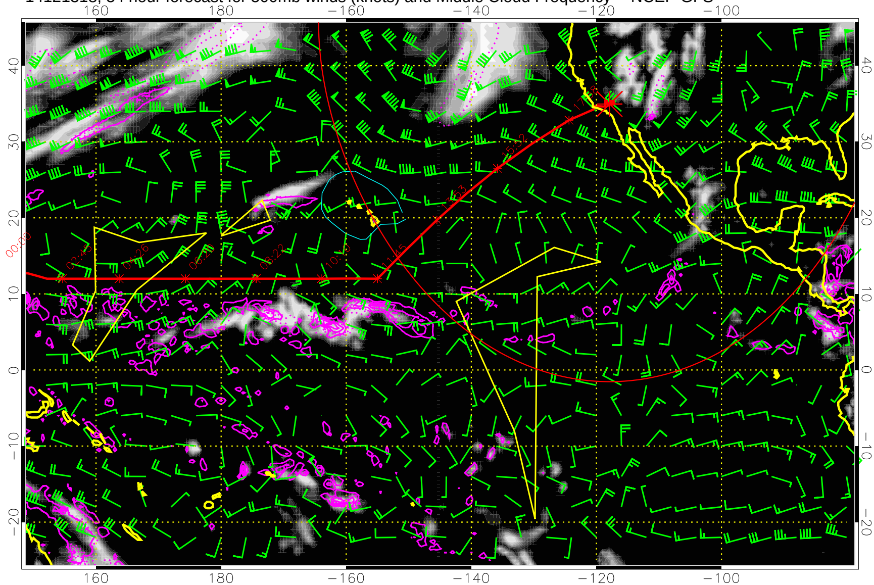
14121318, 54 hour forecast for 500mb winds (knots) and Middle Cloud Frequency -- NCEP GFS
