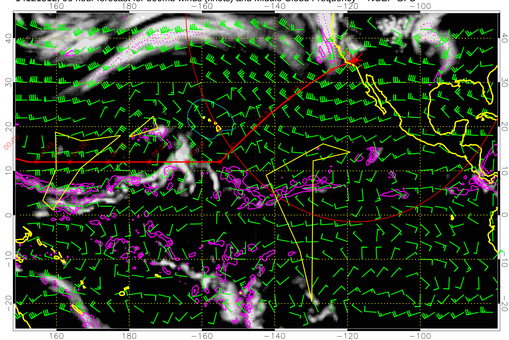
14121512, 96 hour forecast for 500mb winds (knots) and Middle Cloud Frequency -- NCEP GFS
