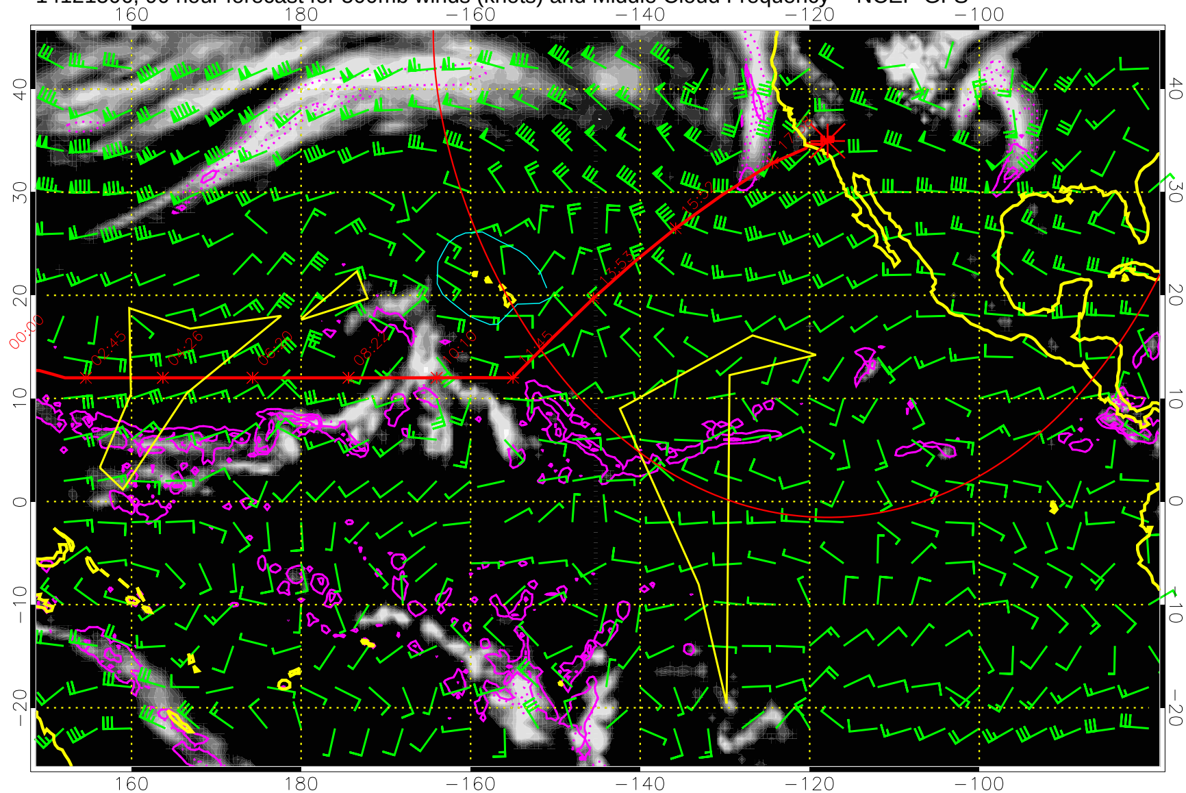
14121506, 90 hour forecast for 500mb winds (knots) and Middle Cloud Frequency -- NCEP GFS
