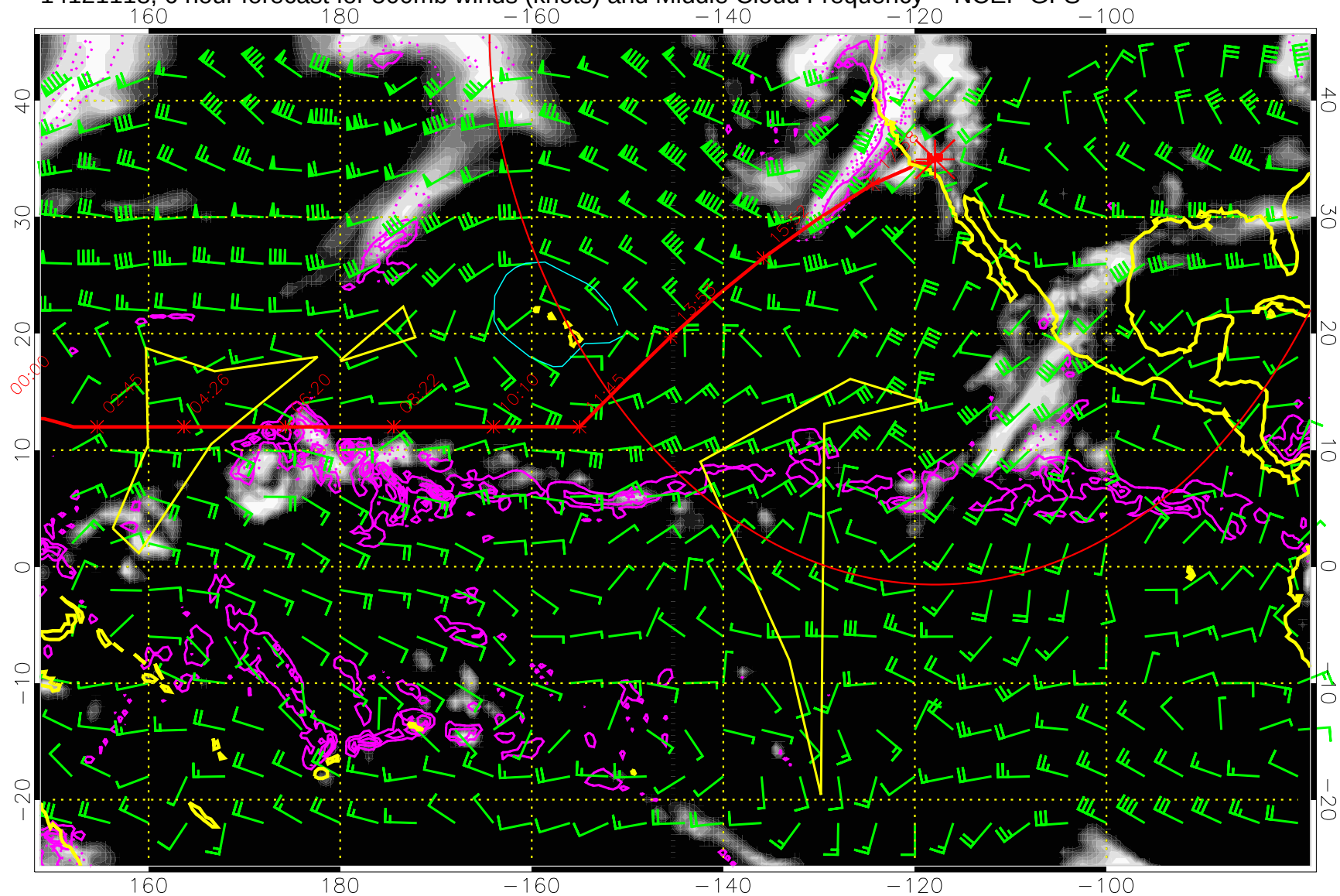
14121118, 6 hour forecast for 500mb winds (knots) and Middle Cloud Frequency -- NCEP GFS
