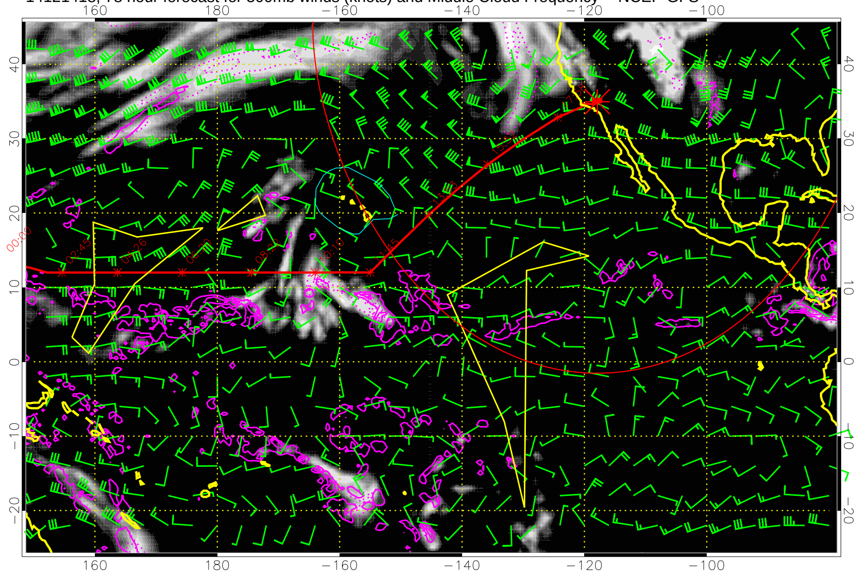
14121418, 78 hour forecast for 500mb winds (knots) and Middle Cloud Frequency -- NCEP GFS
