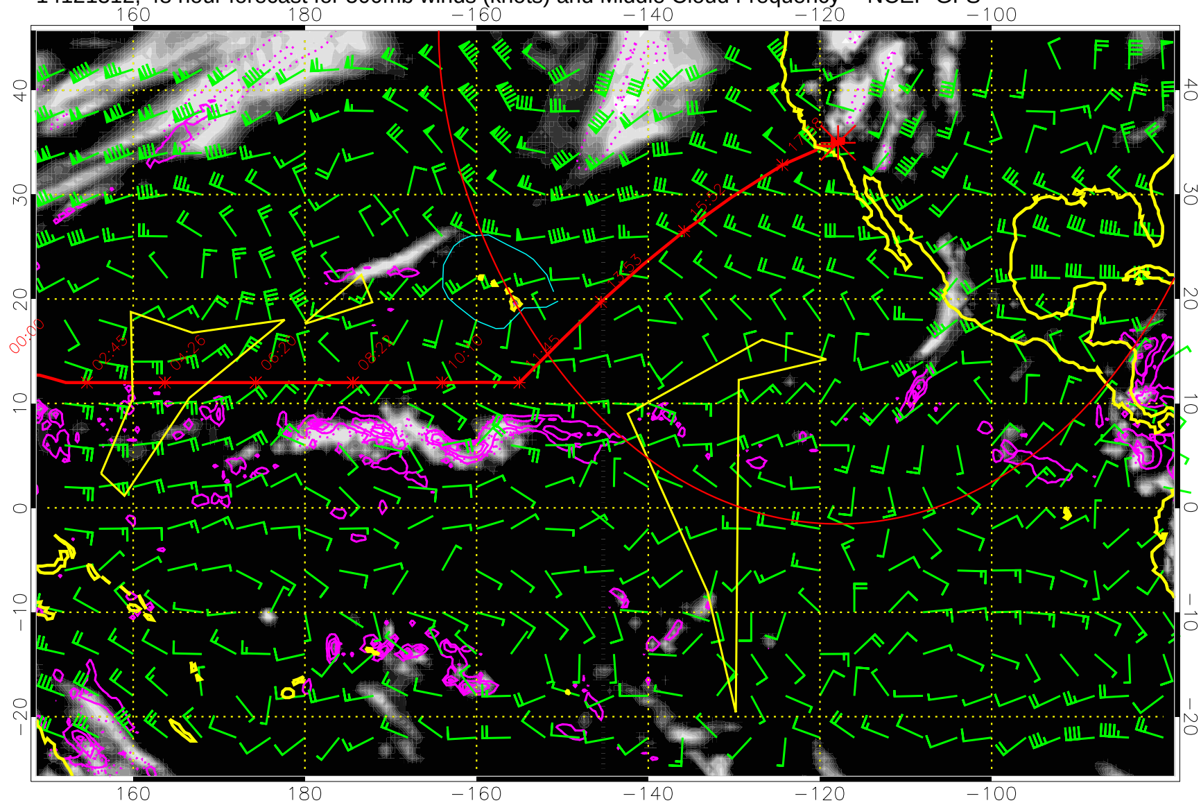
14121312, 48 hour forecast for 500mb winds (knots) and Middle Cloud Frequency -- NCEP GFS
