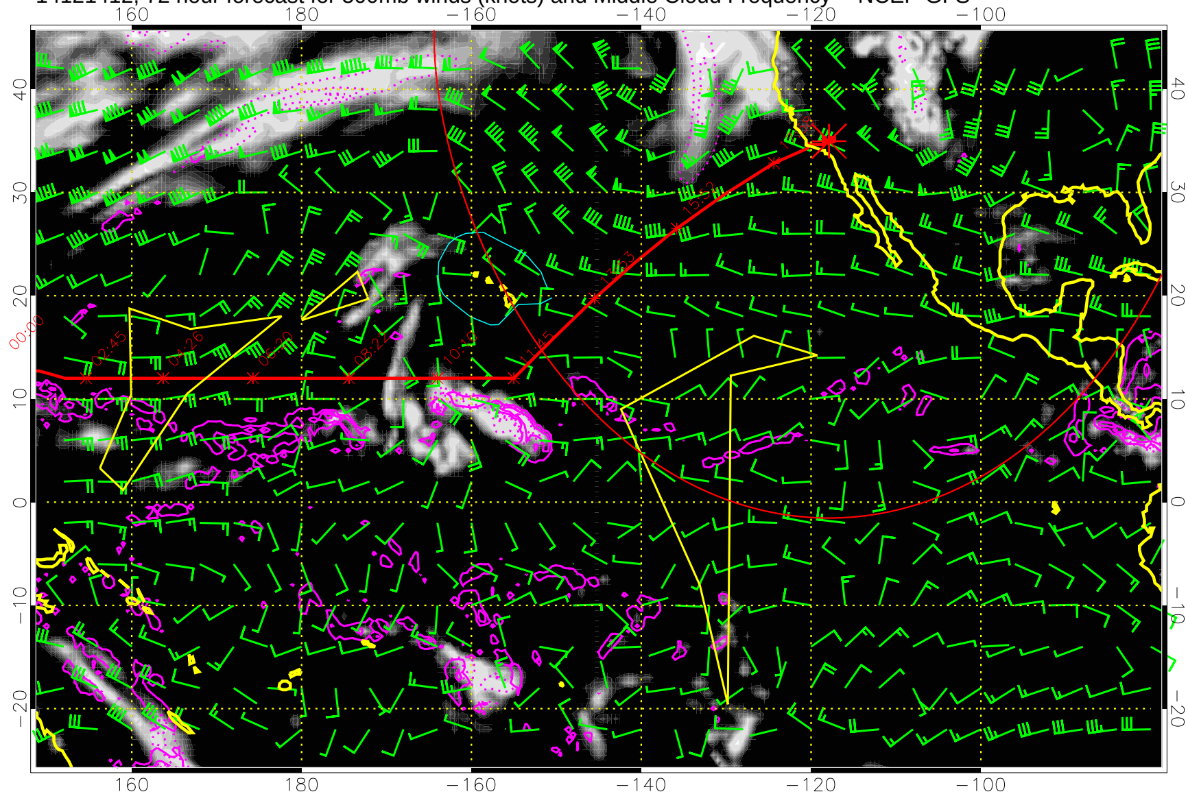
14121412, 72 hour forecast for 500mb winds (knots) and Middle Cloud Frequency -- NCEP GFS
