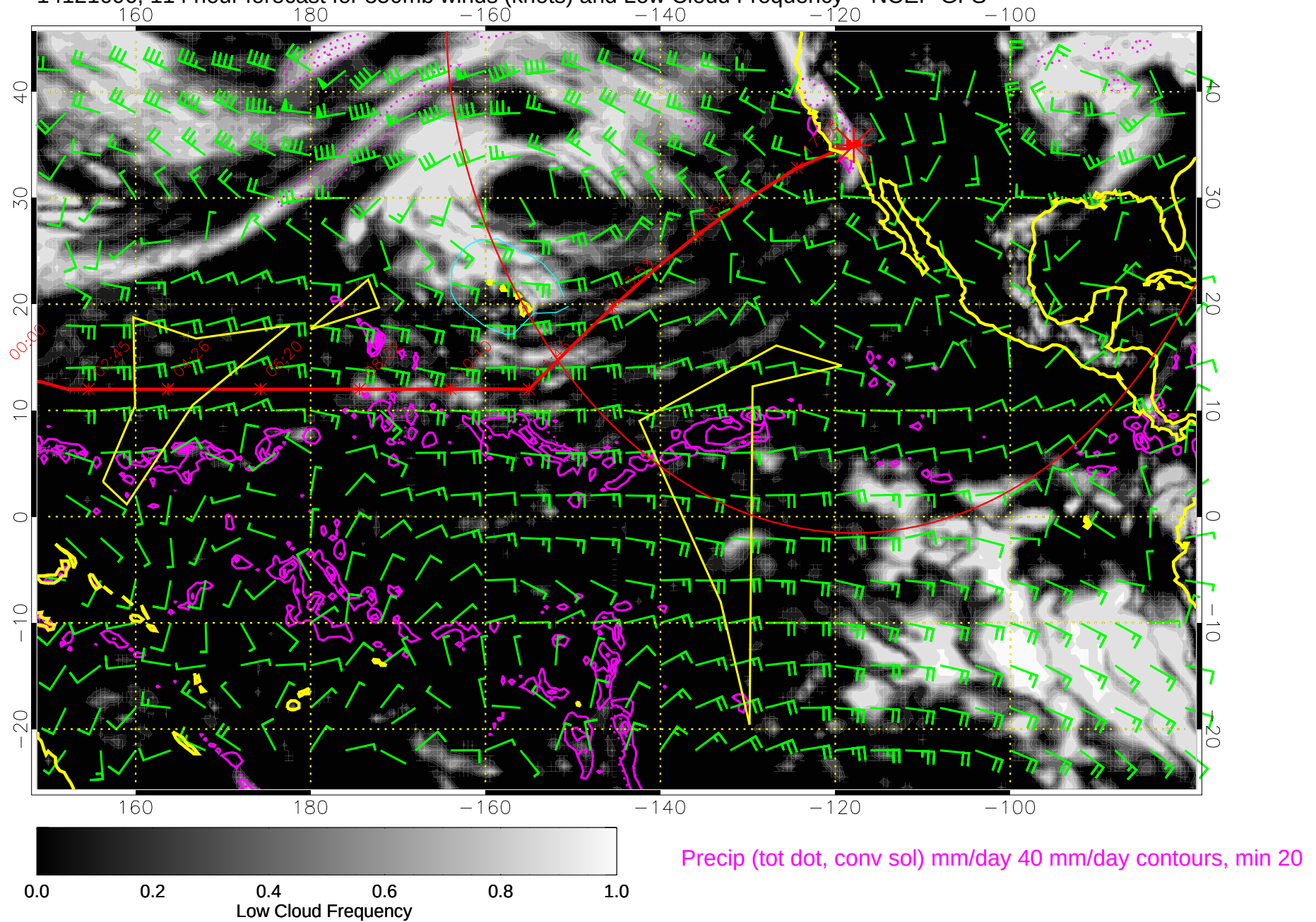
14121606, 114 hour forecast for 850mb winds (knots) and Low Cloud Frequency -- NCEP GFS
