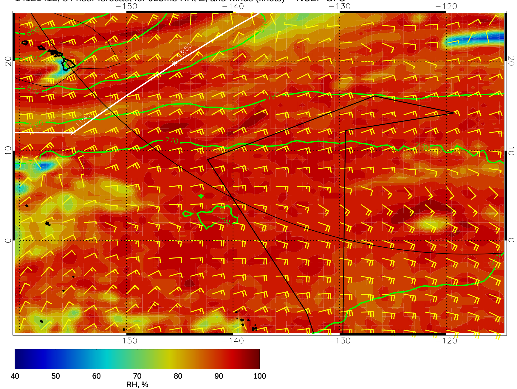
14121412, 84 hour forecast for 925mb RH, Z, and winds (knots) -- NCEP GFS
