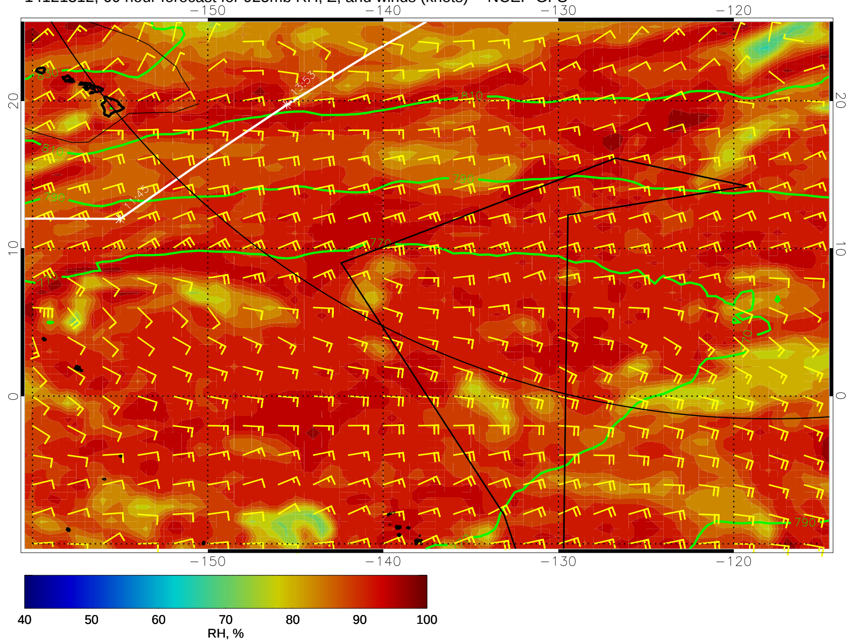
14121312, 60 hour forecast for 925mb RH, Z, and winds (knots) -- NCEP GFS
