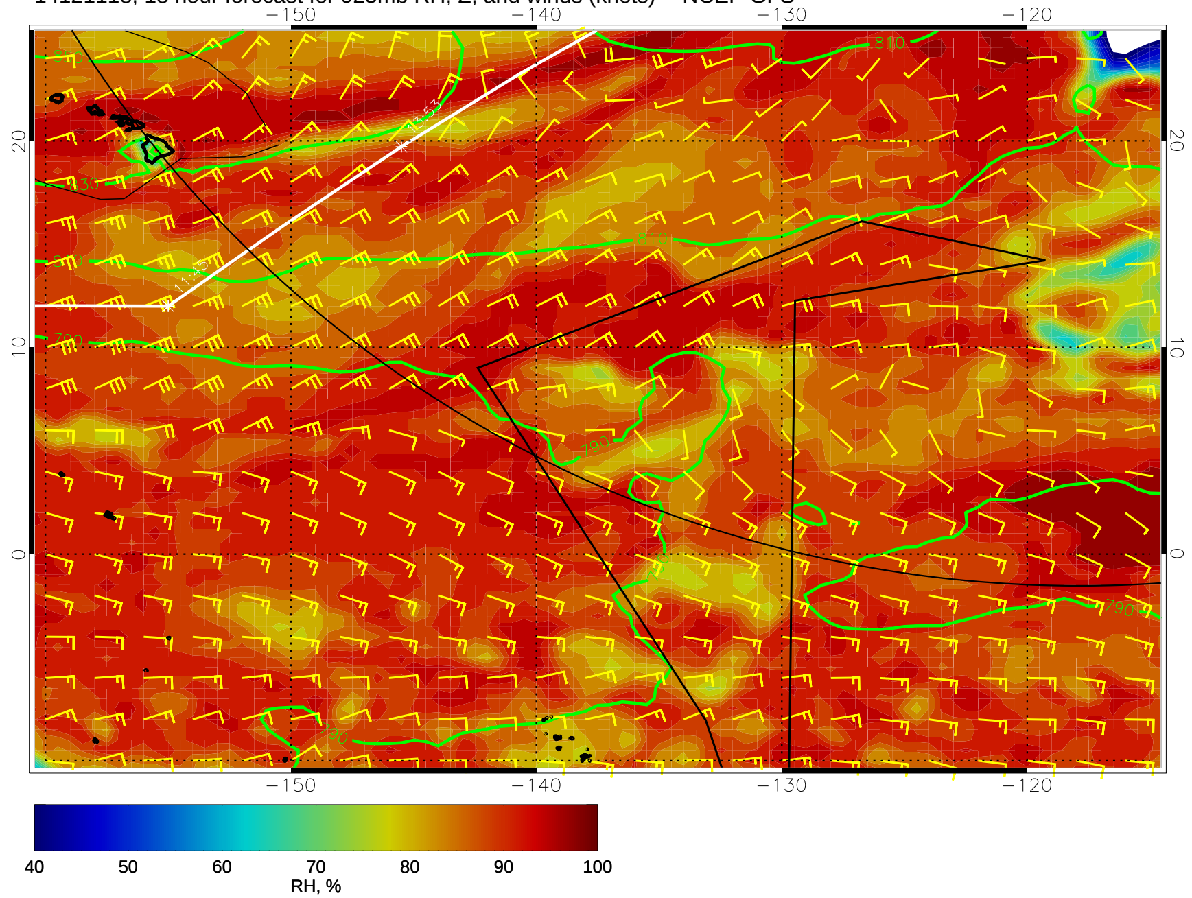
14121118, 18 hour forecast for 925mb RH, Z, and winds (knots) -- NCEP GFS
