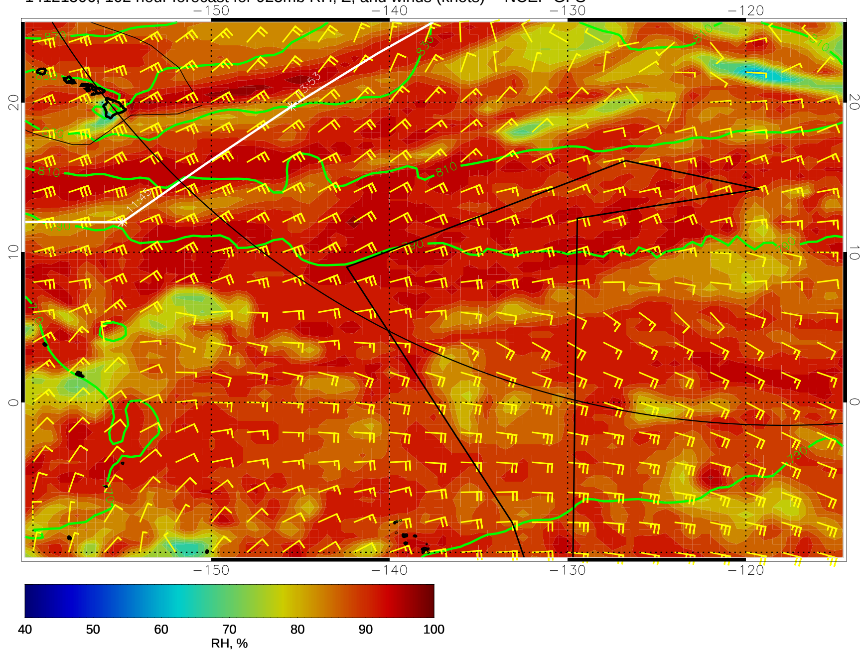
14121506, 102 hour forecast for 925mb RH, Z, and winds (knots) -- NCEP GFS
