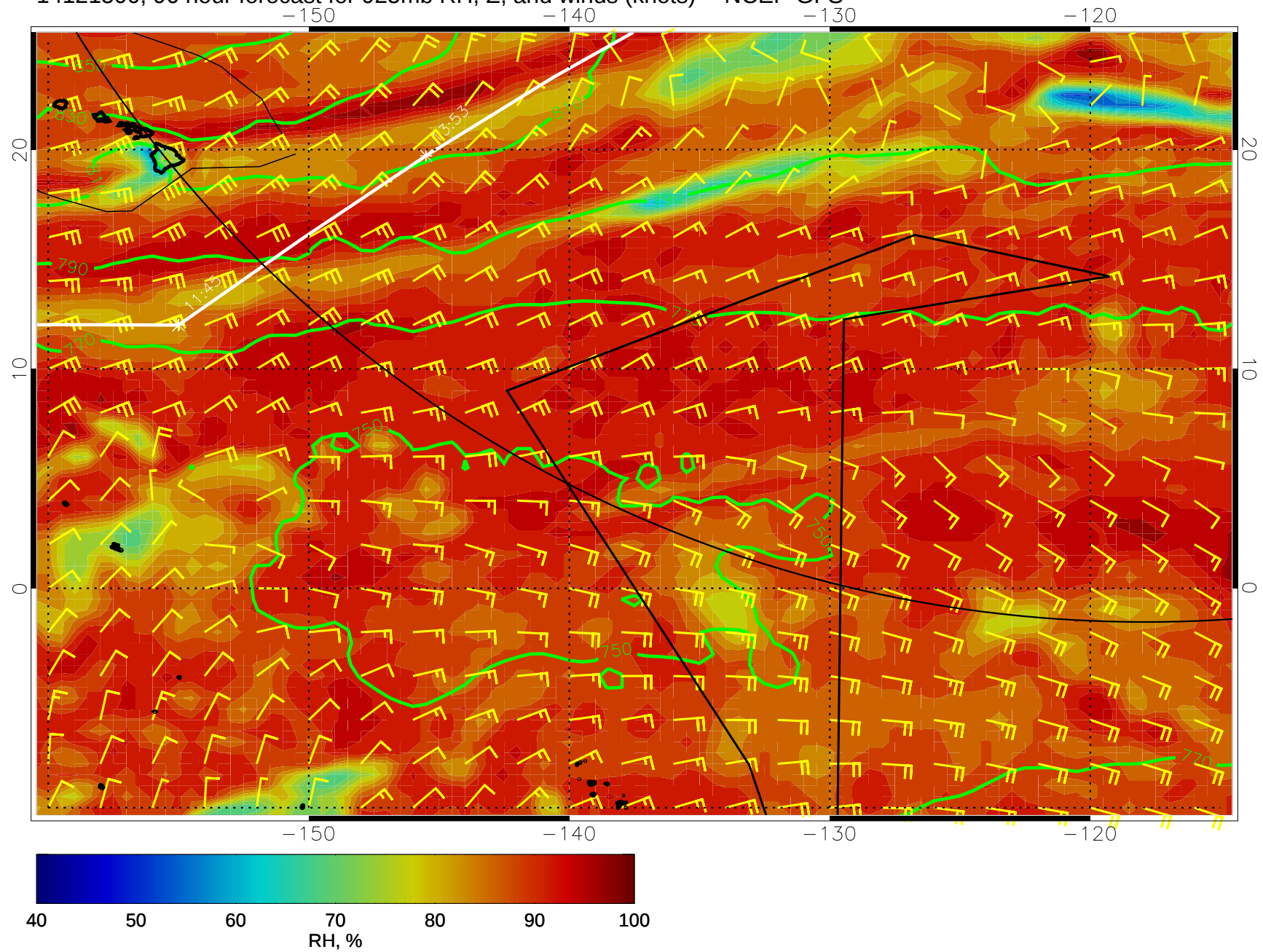
14121500, 96 hour forecast for 925mb RH, Z, and winds (knots) -- NCEP GFS
