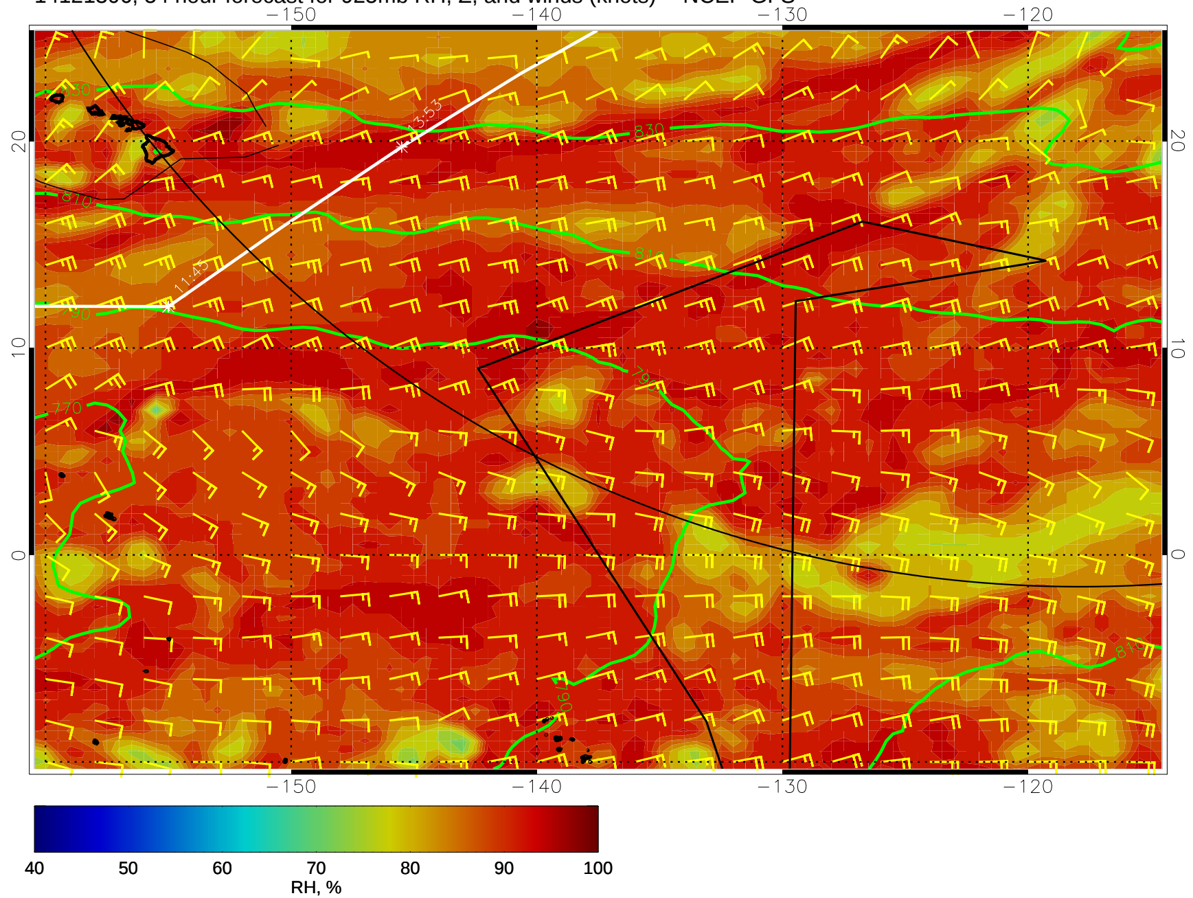
14121306, 54 hour forecast for 925mb RH, Z, and winds (knots) -- NCEP GFS
