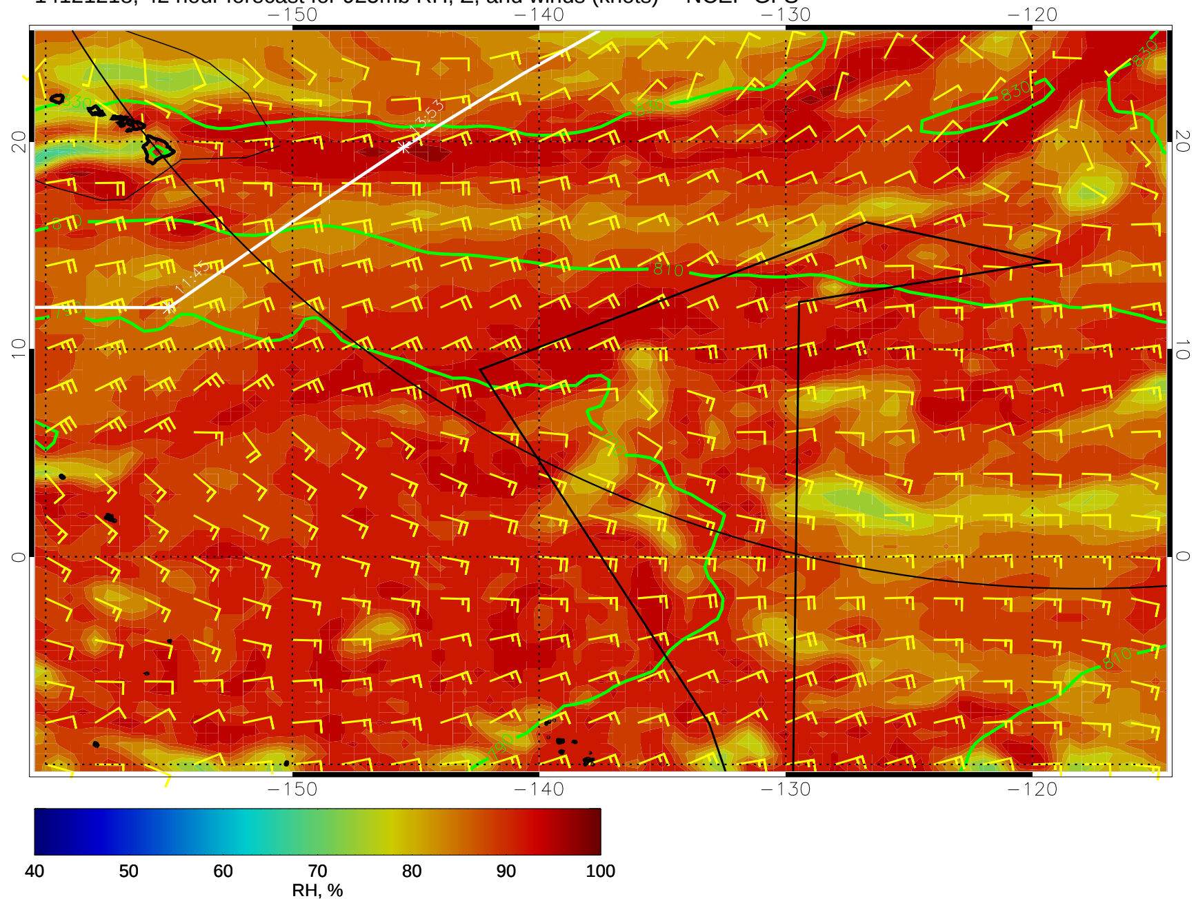
14121218, 42 hour forecast for 925mb RH, Z, and winds (knots) -- NCEP GFS
