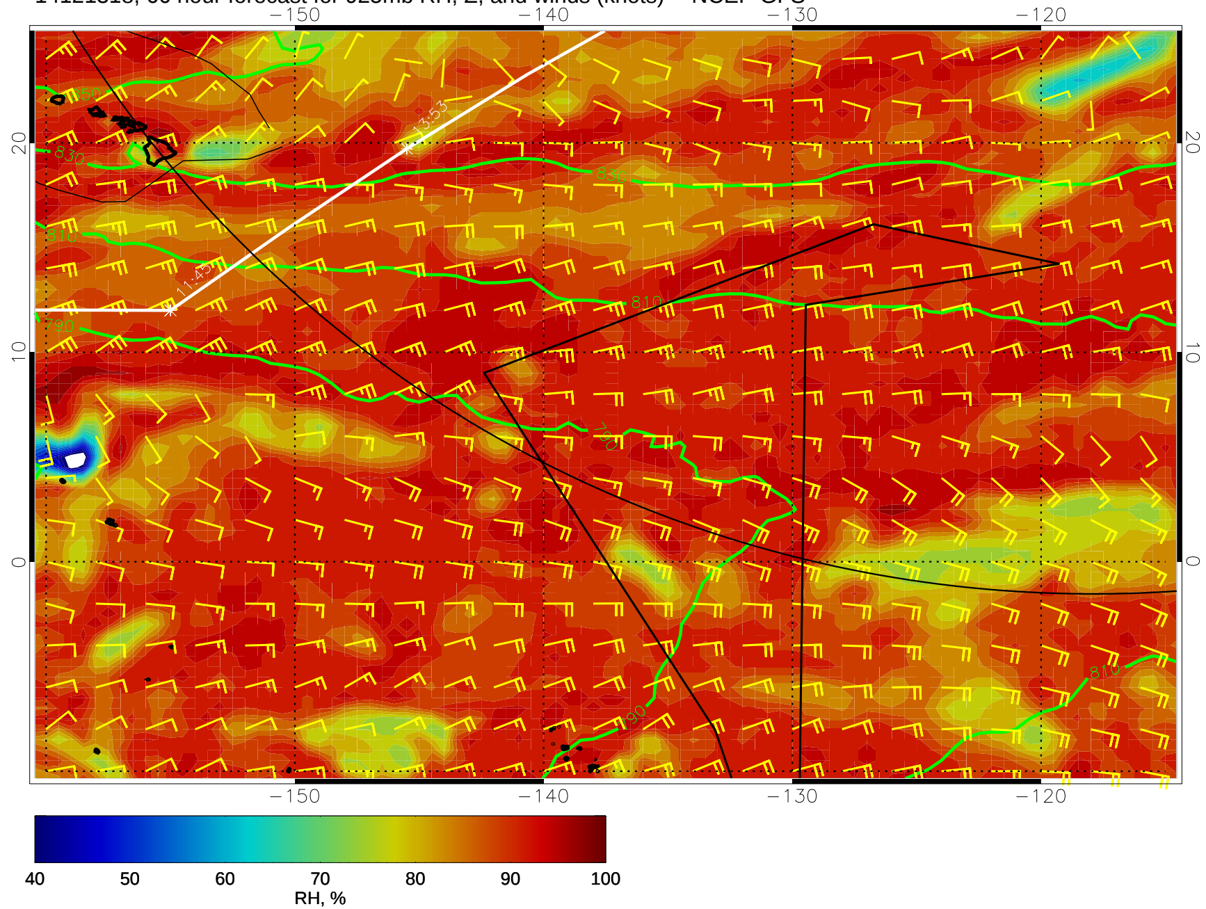
14121318, 66 hour forecast for 925mb RH, Z, and winds (knots) -- NCEP GFS
