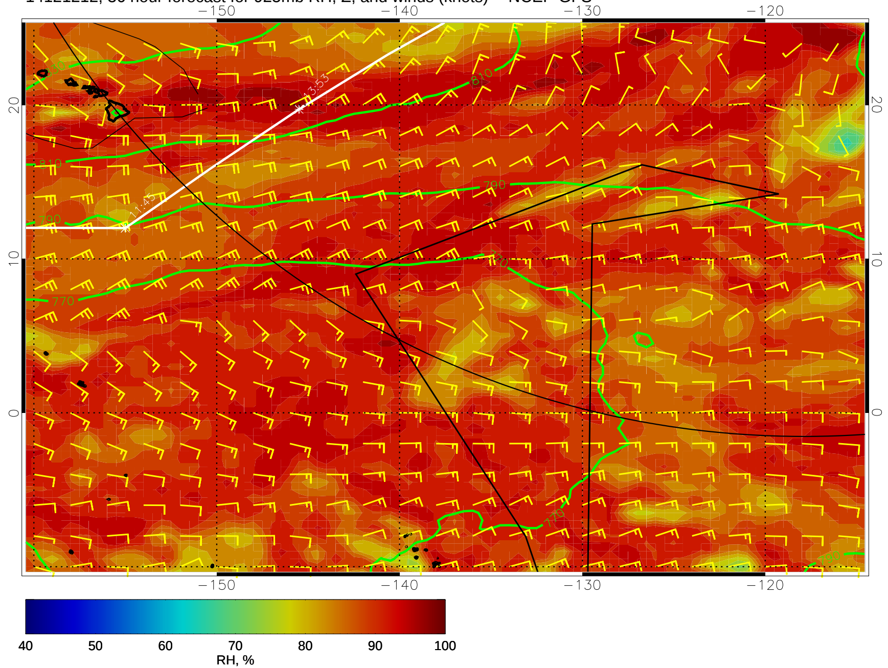
14121212, 36 hour forecast for 925mb RH, Z, and winds (knots) -- NCEP GFS
