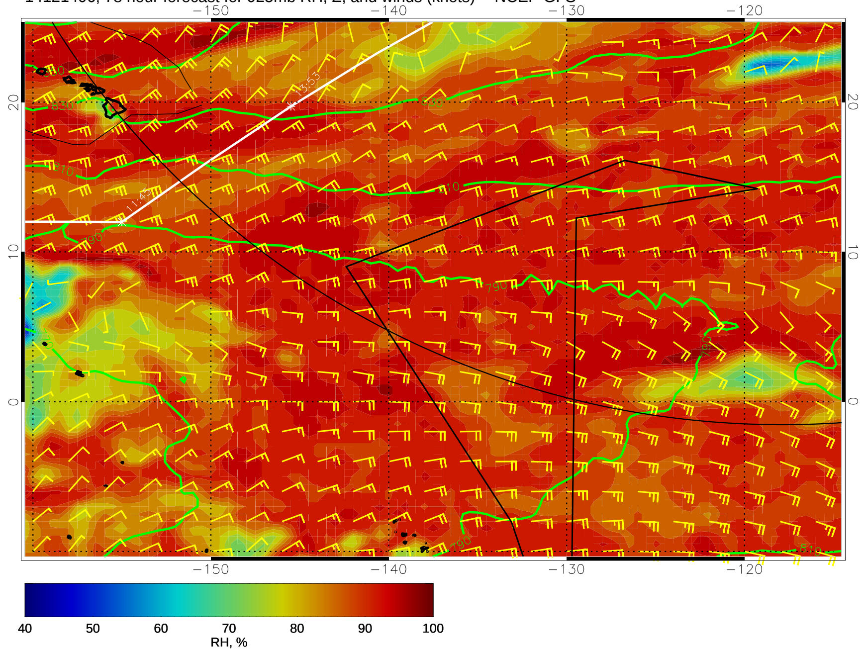
14121406, 78 hour forecast for 925mb RH, Z, and winds (knots) -- NCEP GFS
