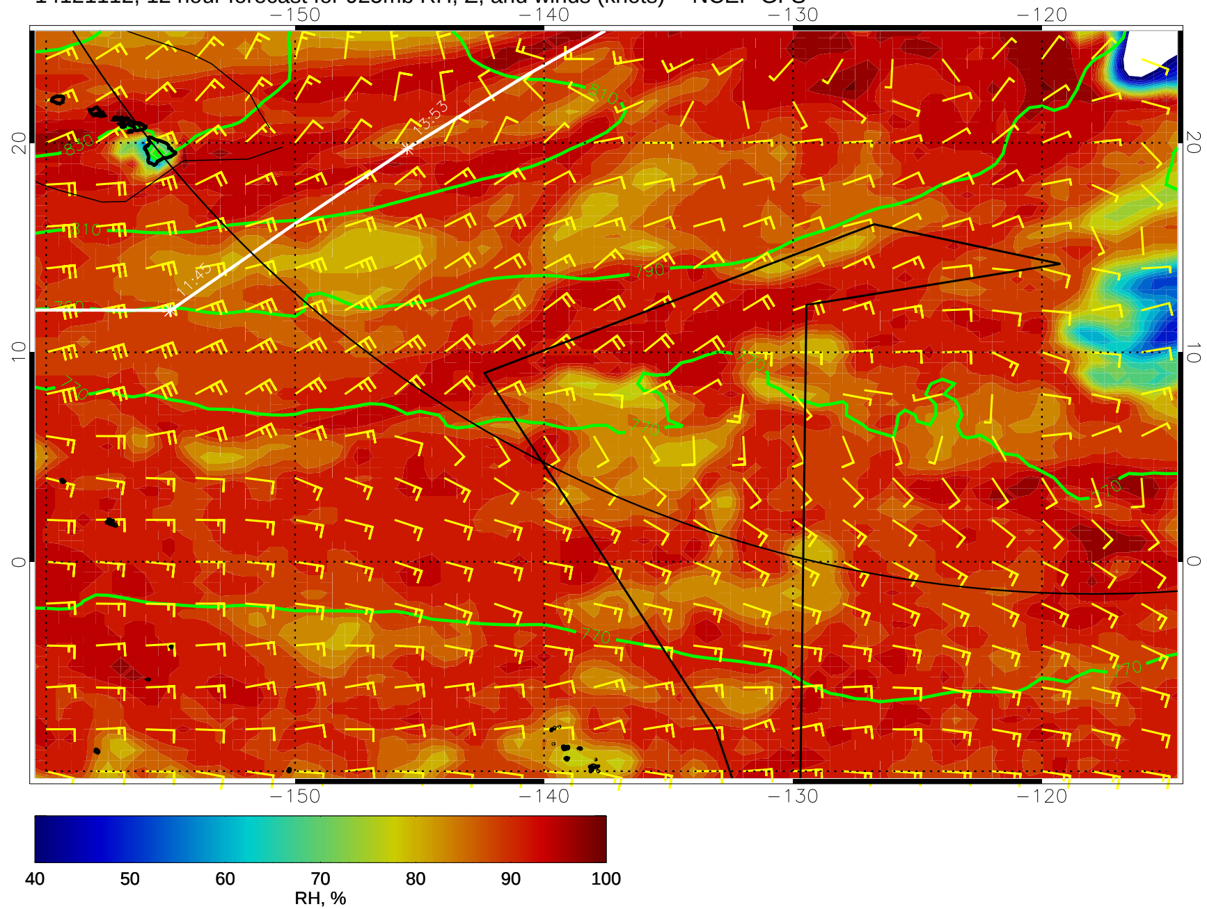
14121112, 12 hour forecast for 925mb RH, Z, and winds (knots) -- NCEP GFS
