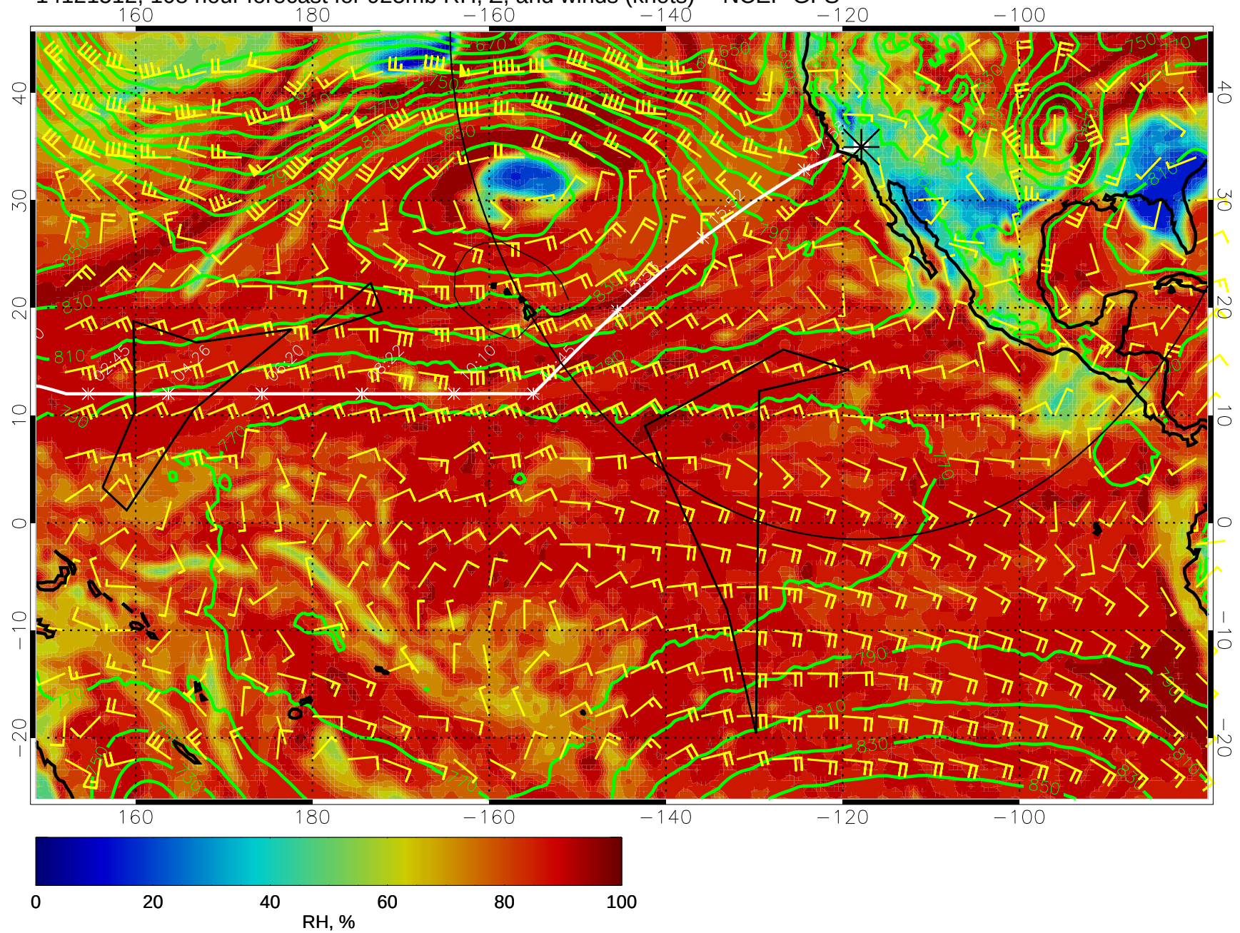
14121512, 108 hour forecast for 925mb RH, Z, and winds (knots) -- NCEP GFS
