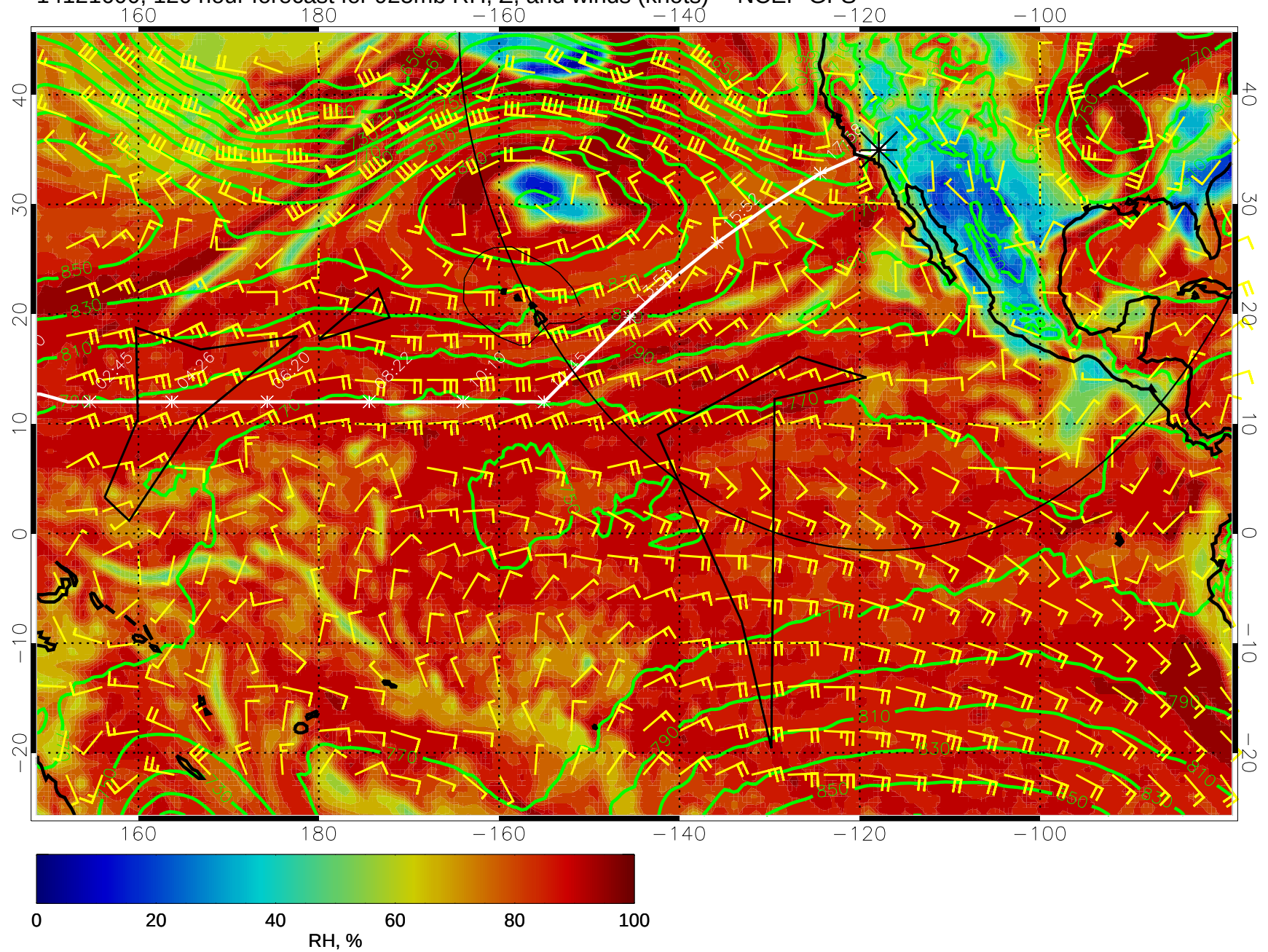
14121600, 120 hour forecast for 925mb RH, Z, and winds (knots) -- NCEP GFS
