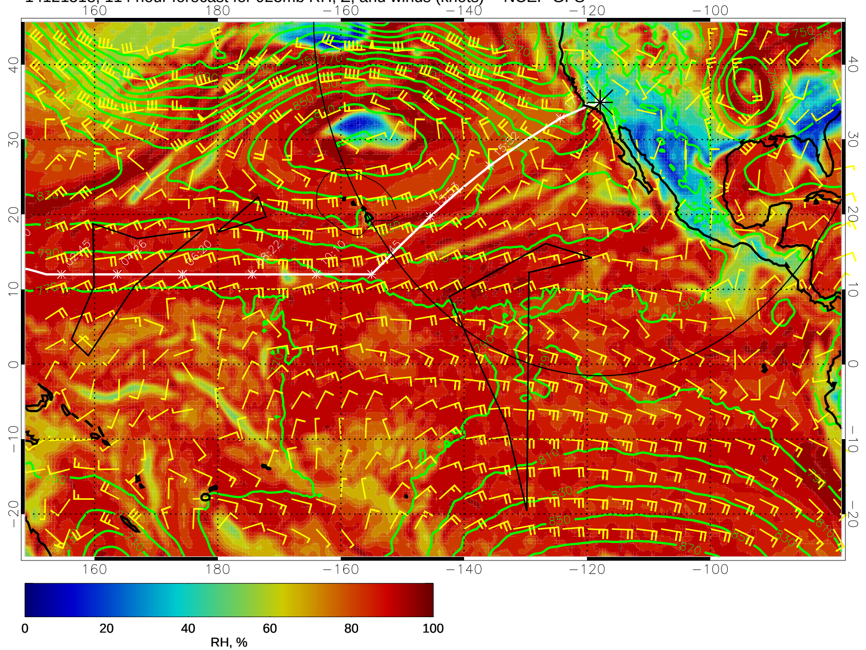
14121518, 114 hour forecast for 925mb RH, Z, and winds (knots) -- NCEP GFS
