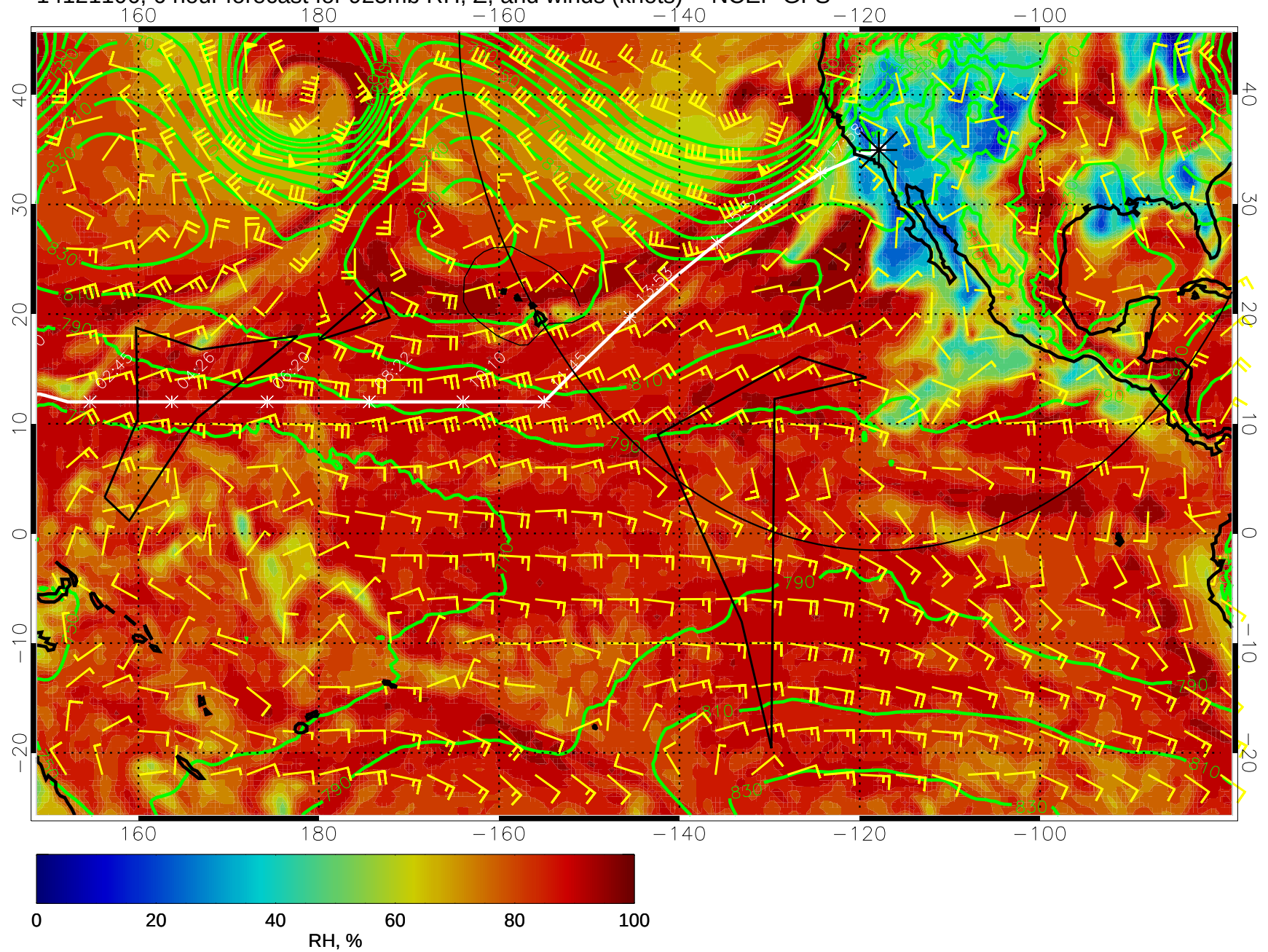
14121106, 6 hour forecast for 925mb RH, Z, and winds (knots) -- NCEP GFS
