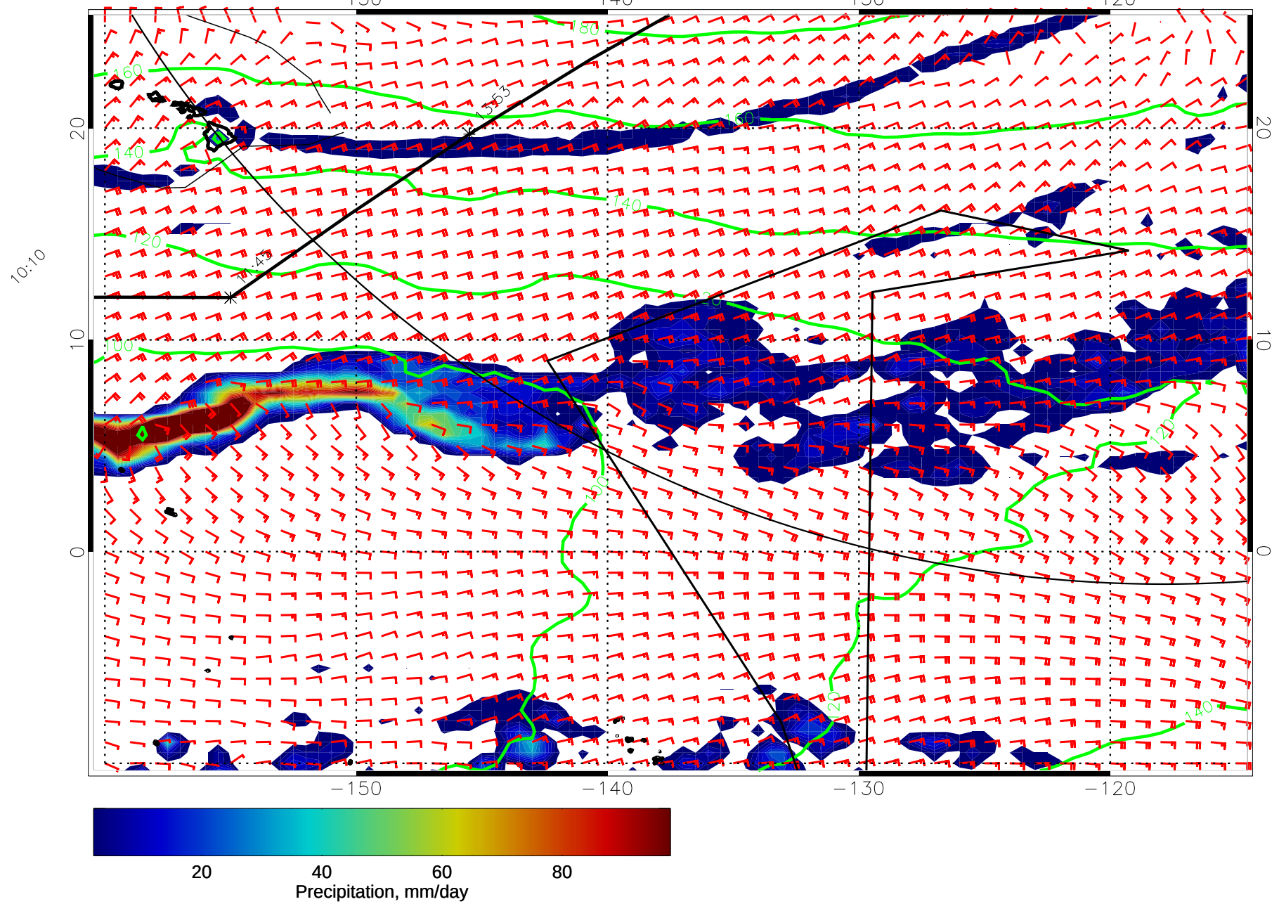
14121306, 54 hour forecast for precip, 1000mb Z, and winds (knots) -- NCEP GFS
