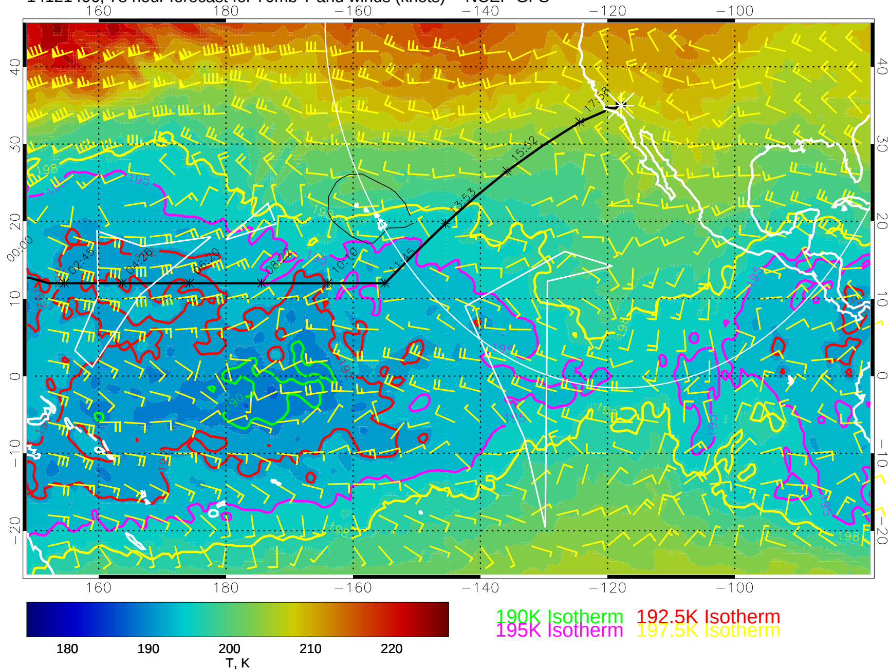
14121406, 78 hour forecast for 70mb T and winds (knots) -- NCEP GFS
