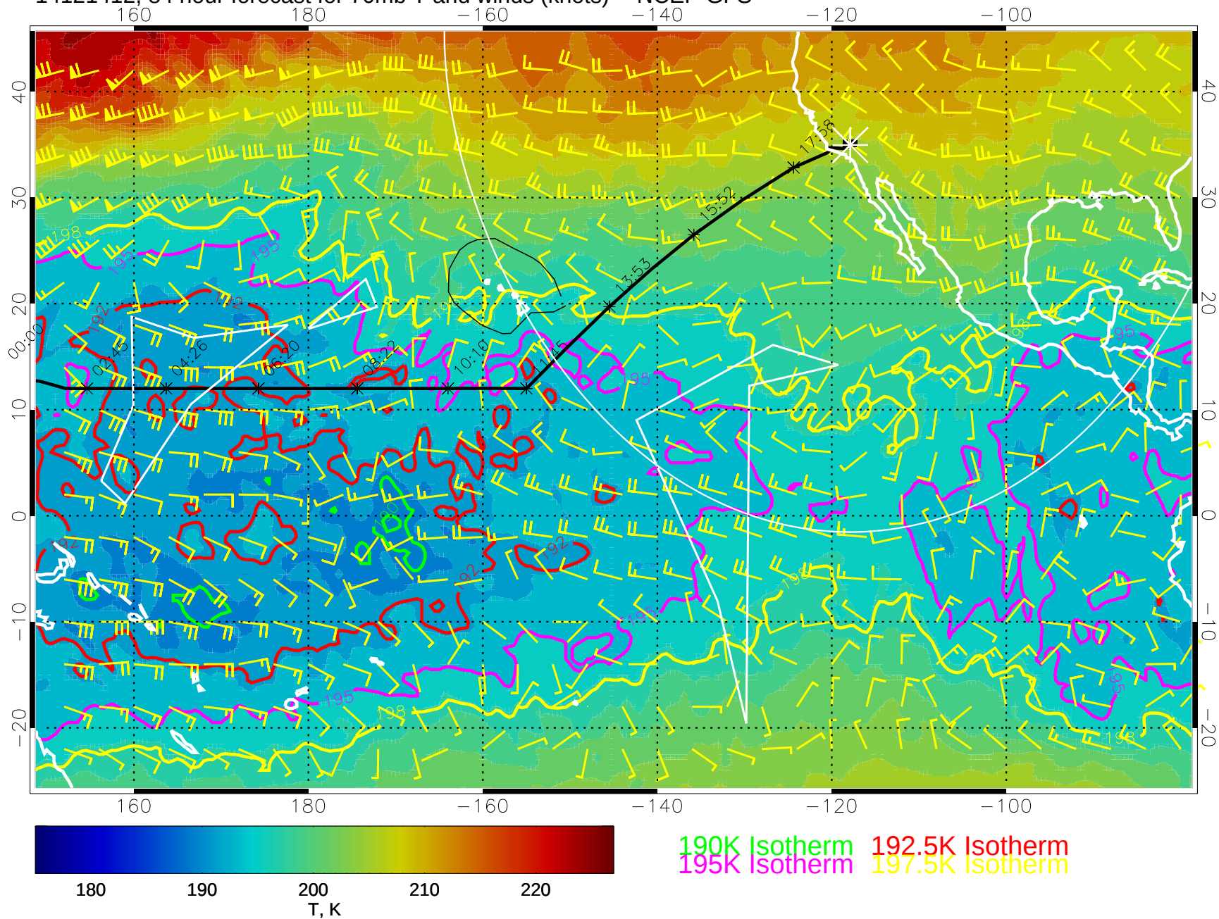
14121412, 84 hour forecast for 70mb T and winds (knots) -- NCEP GFS
