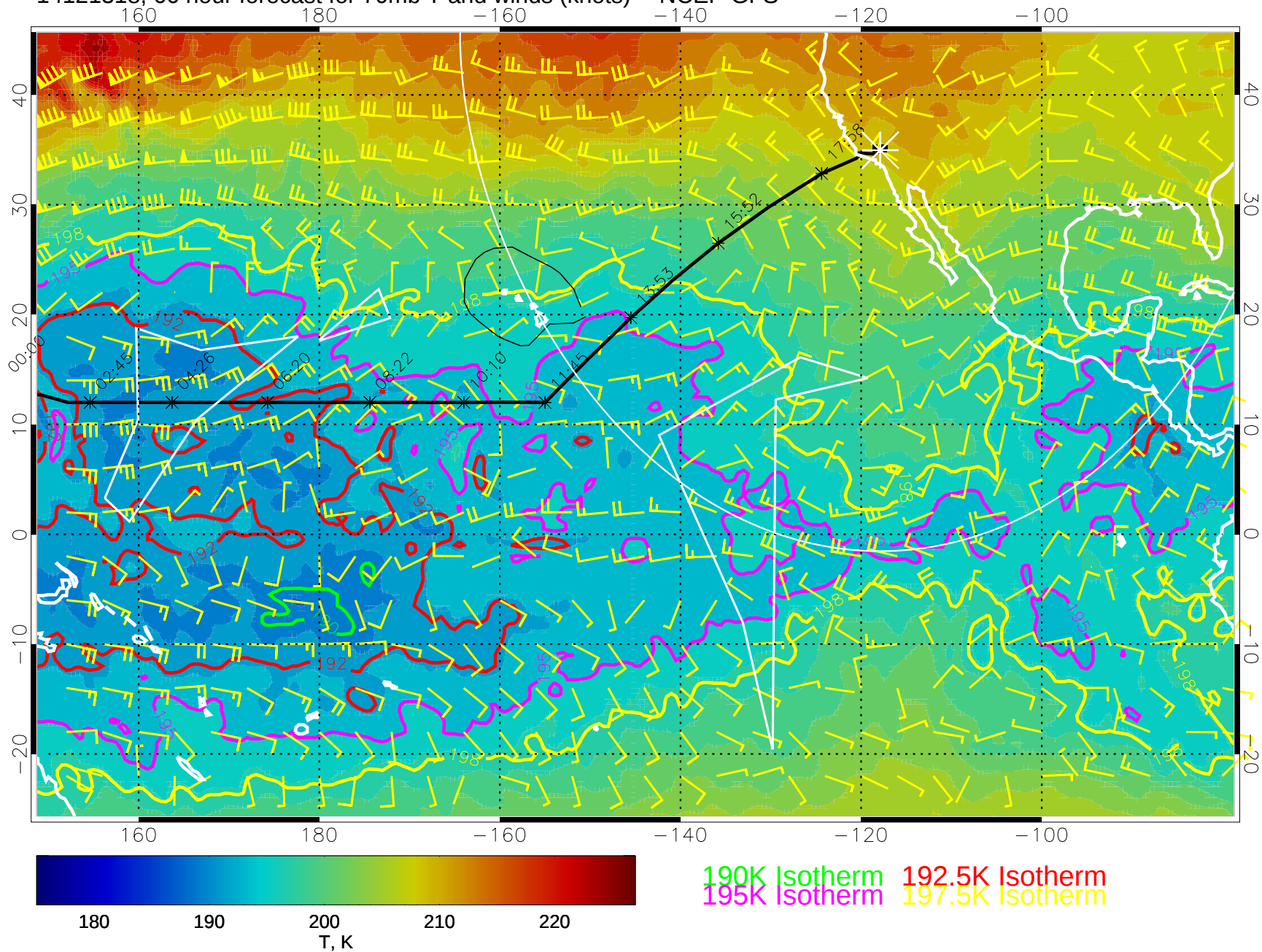
14121318, 66 hour forecast for 70mb T and winds (knots) -- NCEP GFS
