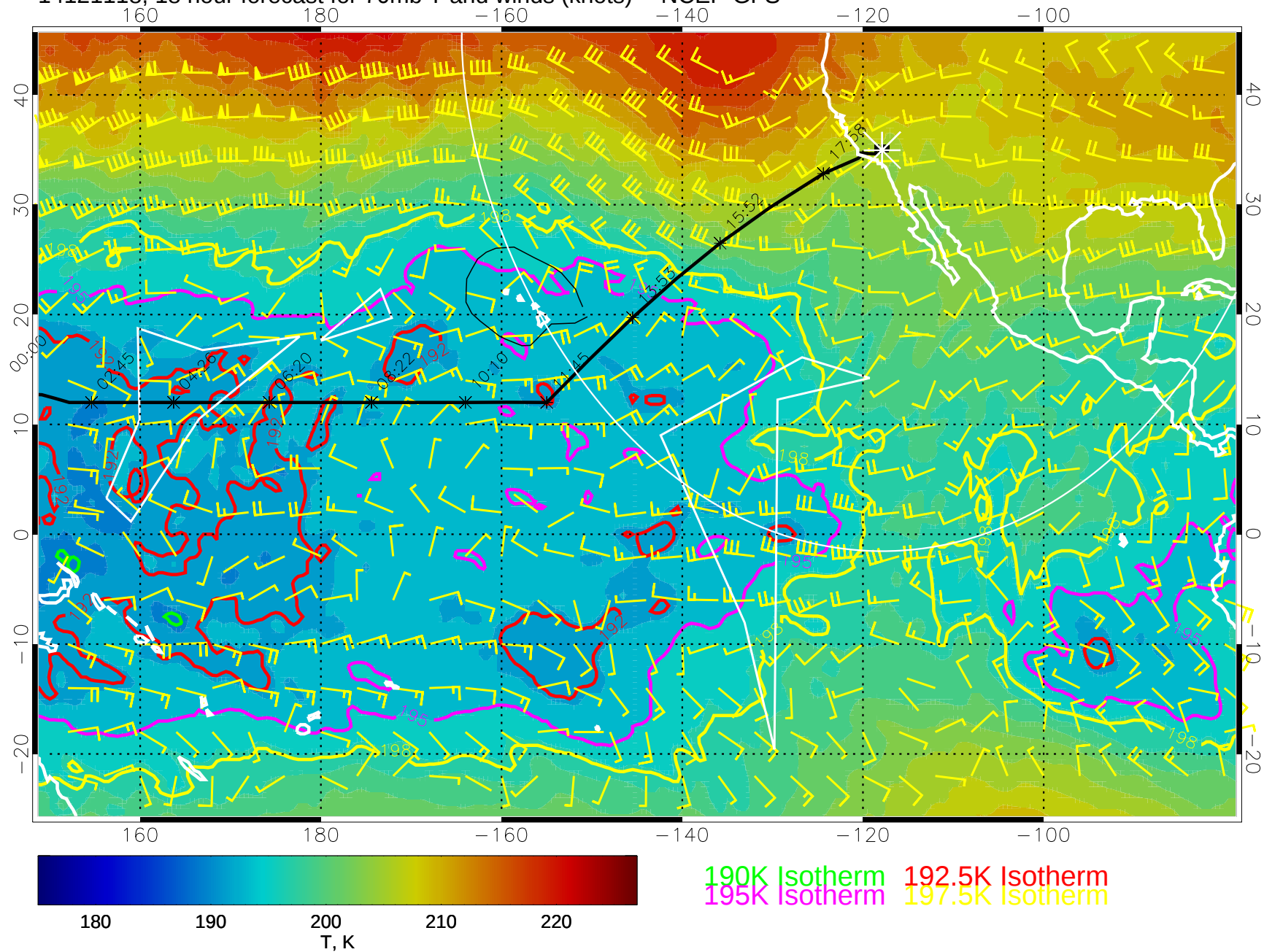
14121118, 18 hour forecast for 70mb T and winds (knots) -- NCEP GFS
