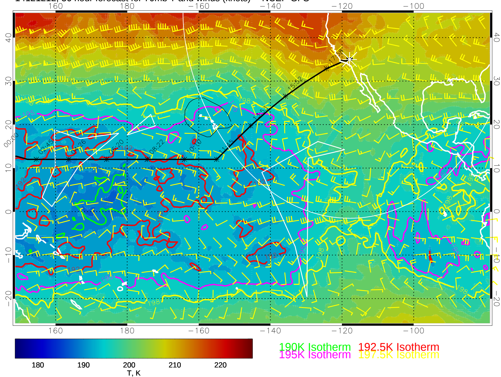
14121212, 36 hour forecast for 70mb T and winds (knots) -- NCEP GFS
