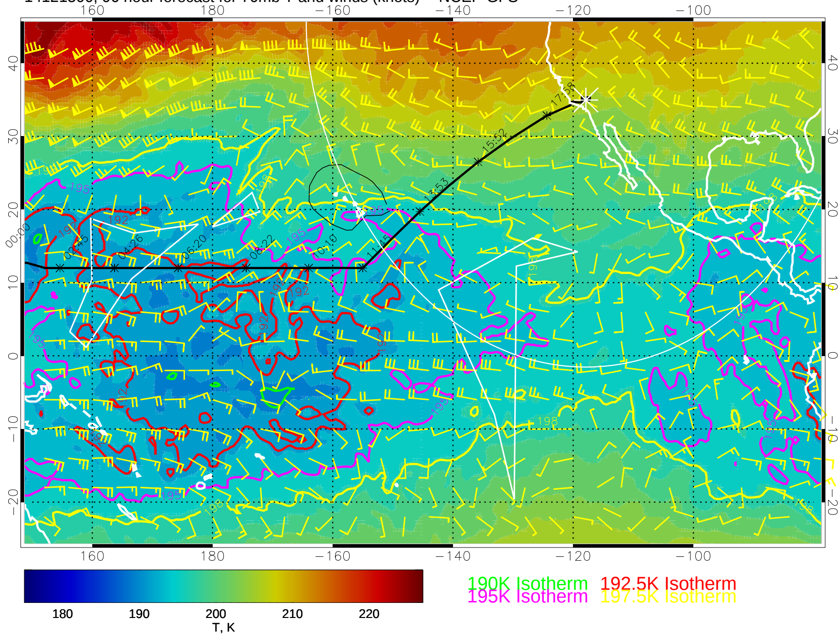
14121500, 96 hour forecast for 70mb T and winds (knots) -- NCEP GFS
