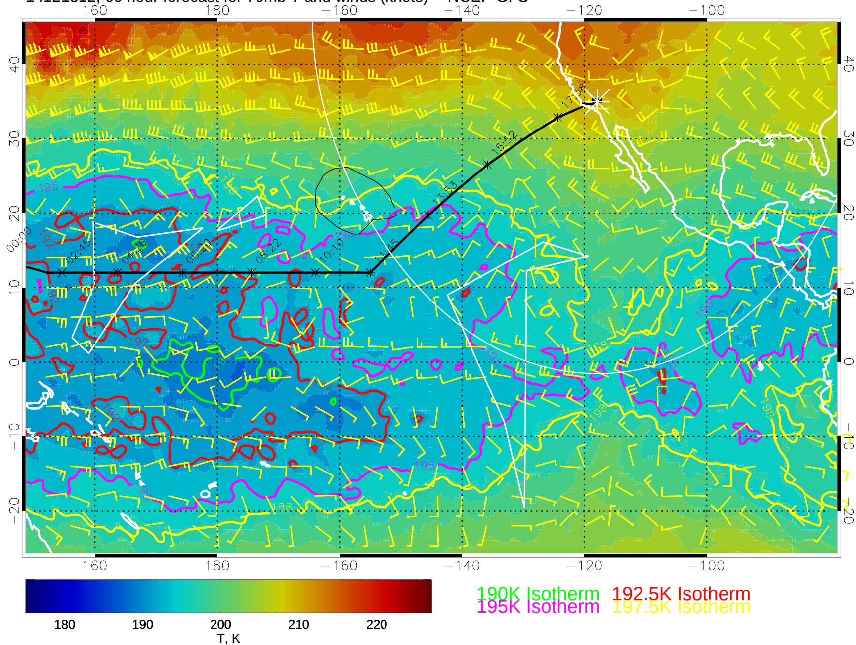
14121312, 60 hour forecast for 70mb T and winds (knots) -- NCEP GFS
