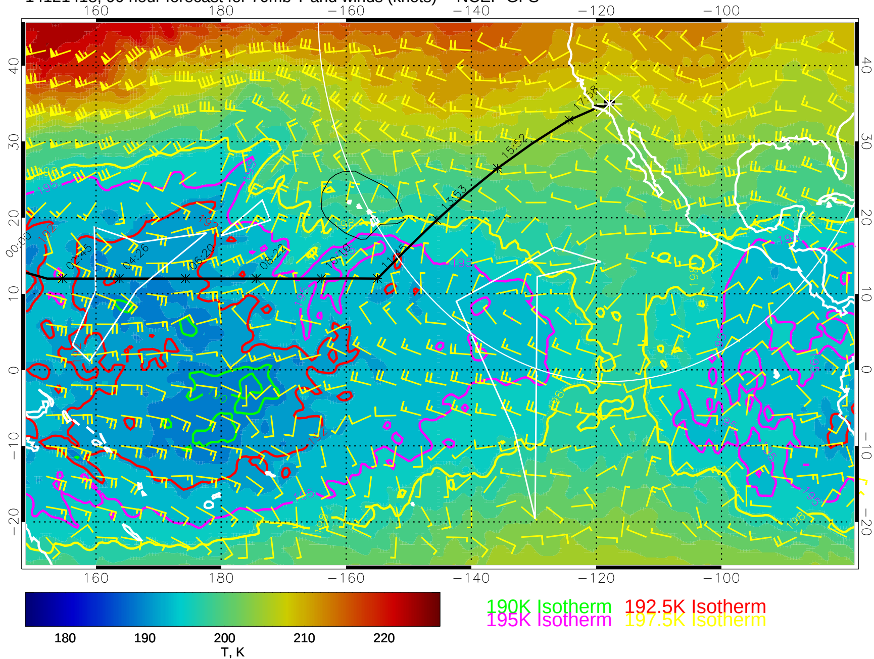
14121418, 90 hour forecast for 70mb T and winds (knots) -- NCEP GFS
