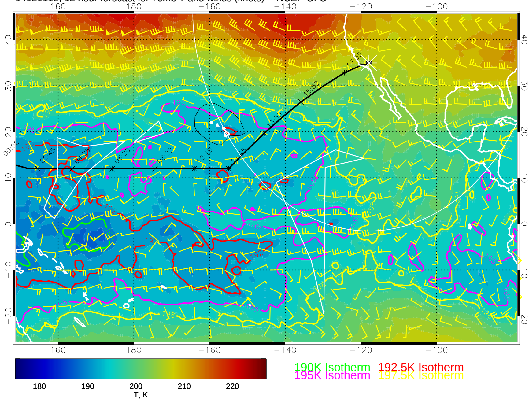
14121112, 12 hour forecast for 70mb T and winds (knots) -- NCEP GFS
