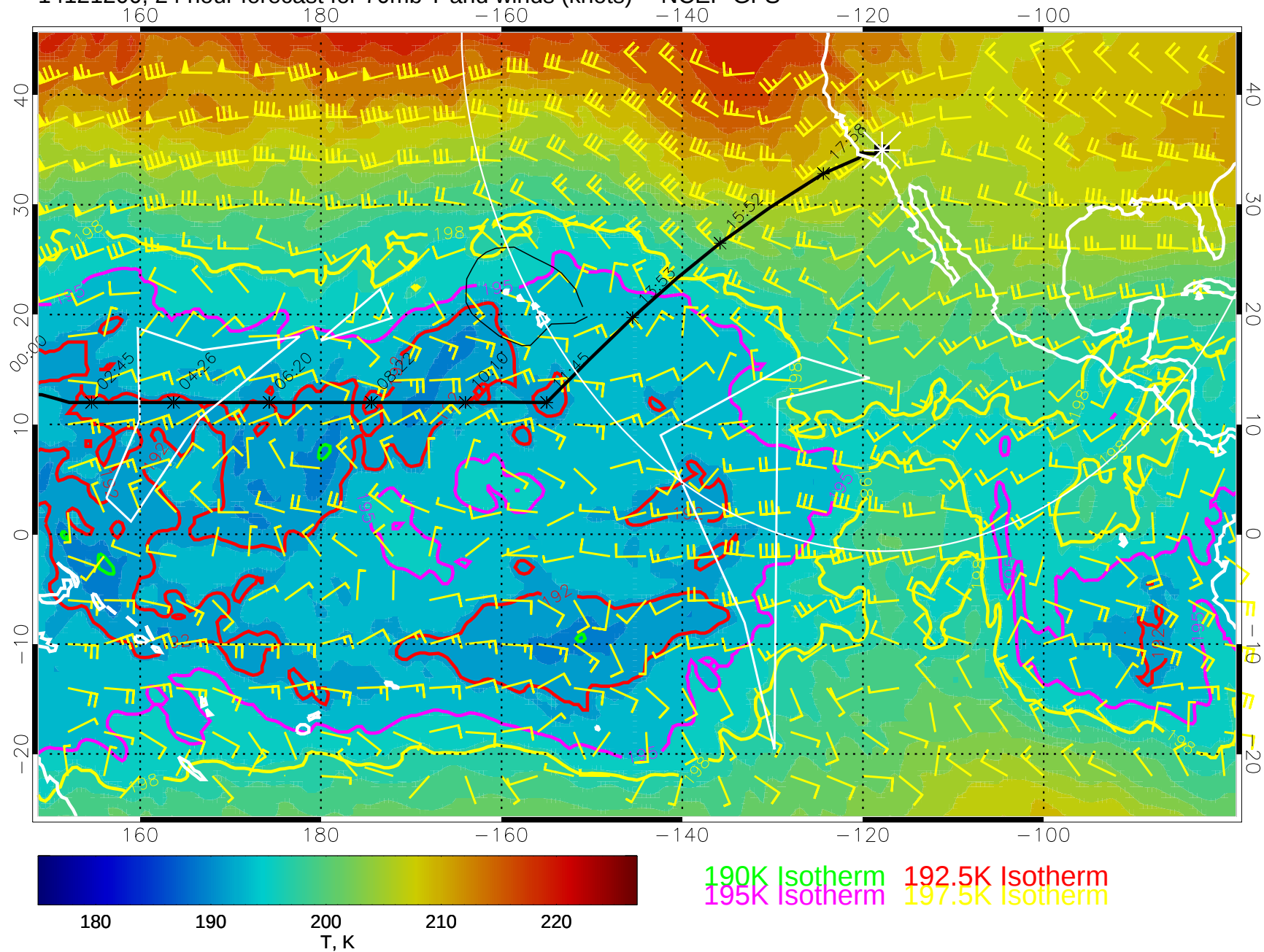
14121200, 24 hour forecast for 70mb T and winds (knots) -- NCEP GFS
