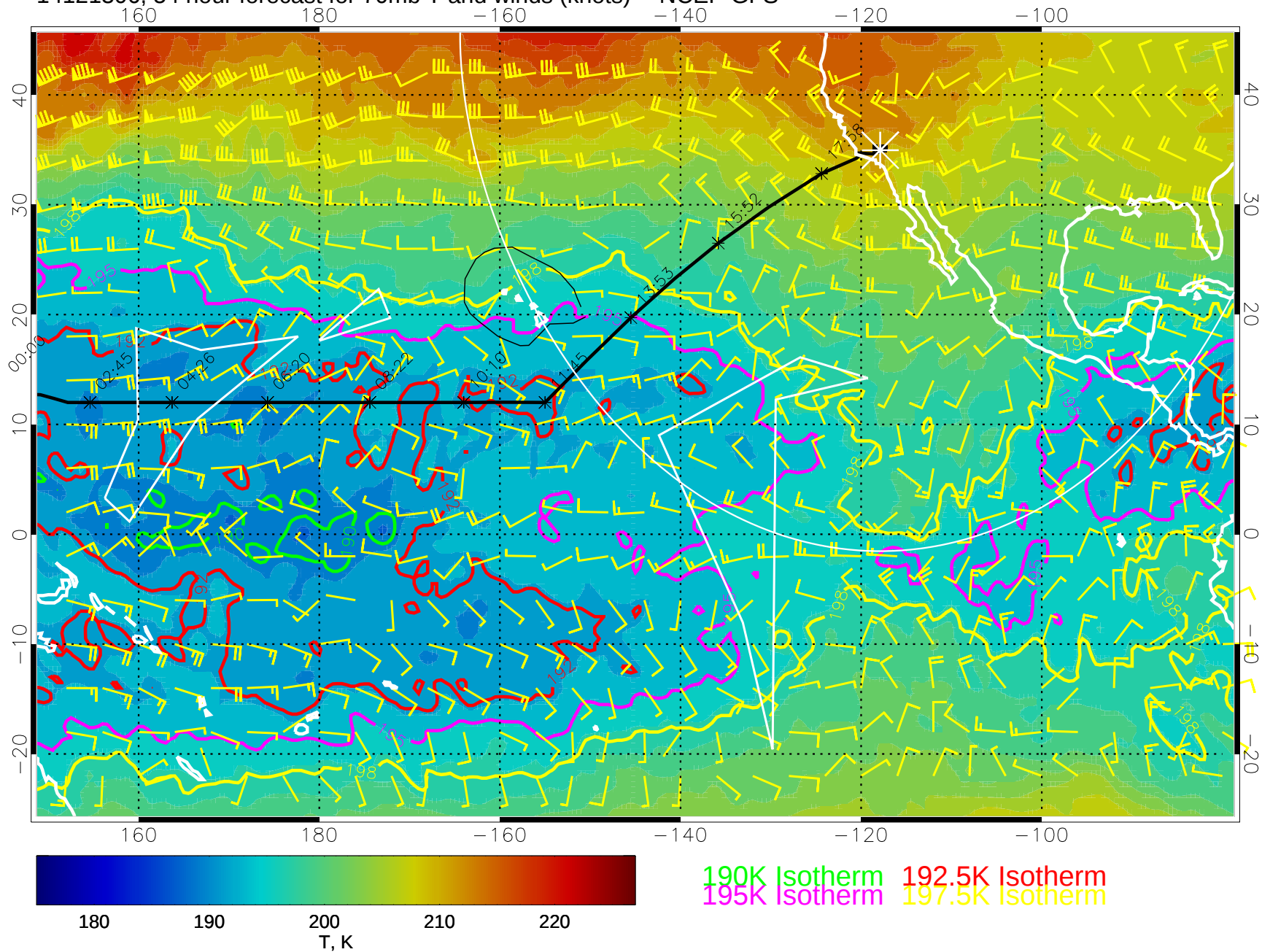
14121306, 54 hour forecast for 70mb T and winds (knots) -- NCEP GFS
