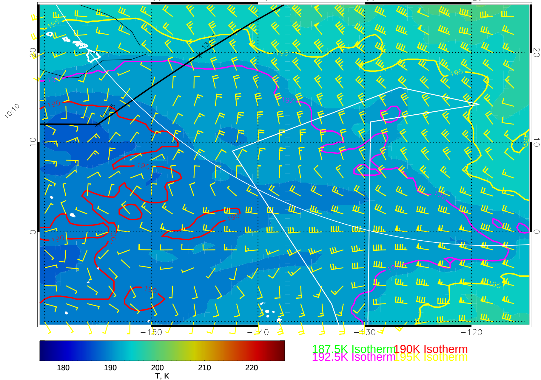
14121212, 36 hour forecast for 100mb T and winds (knots) -- NCEP GFS
