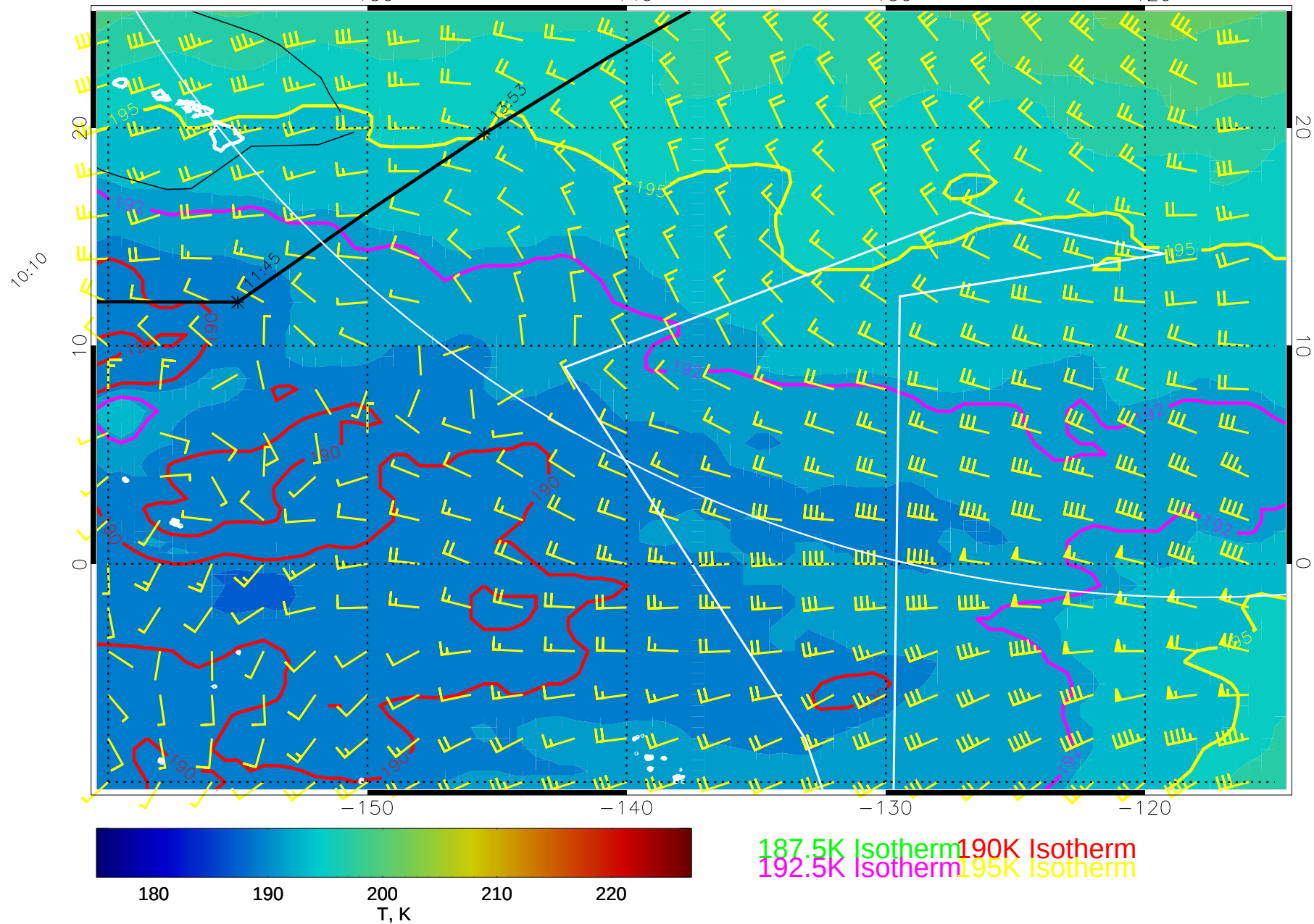
14121312, 60 hour forecast for 100mb T and winds (knots) -- NCEP GFS
