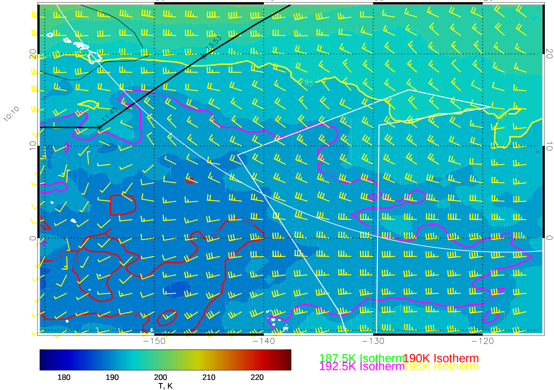
14121412, 84 hour forecast for 100mb T and winds (knots) -- NCEP GFS
