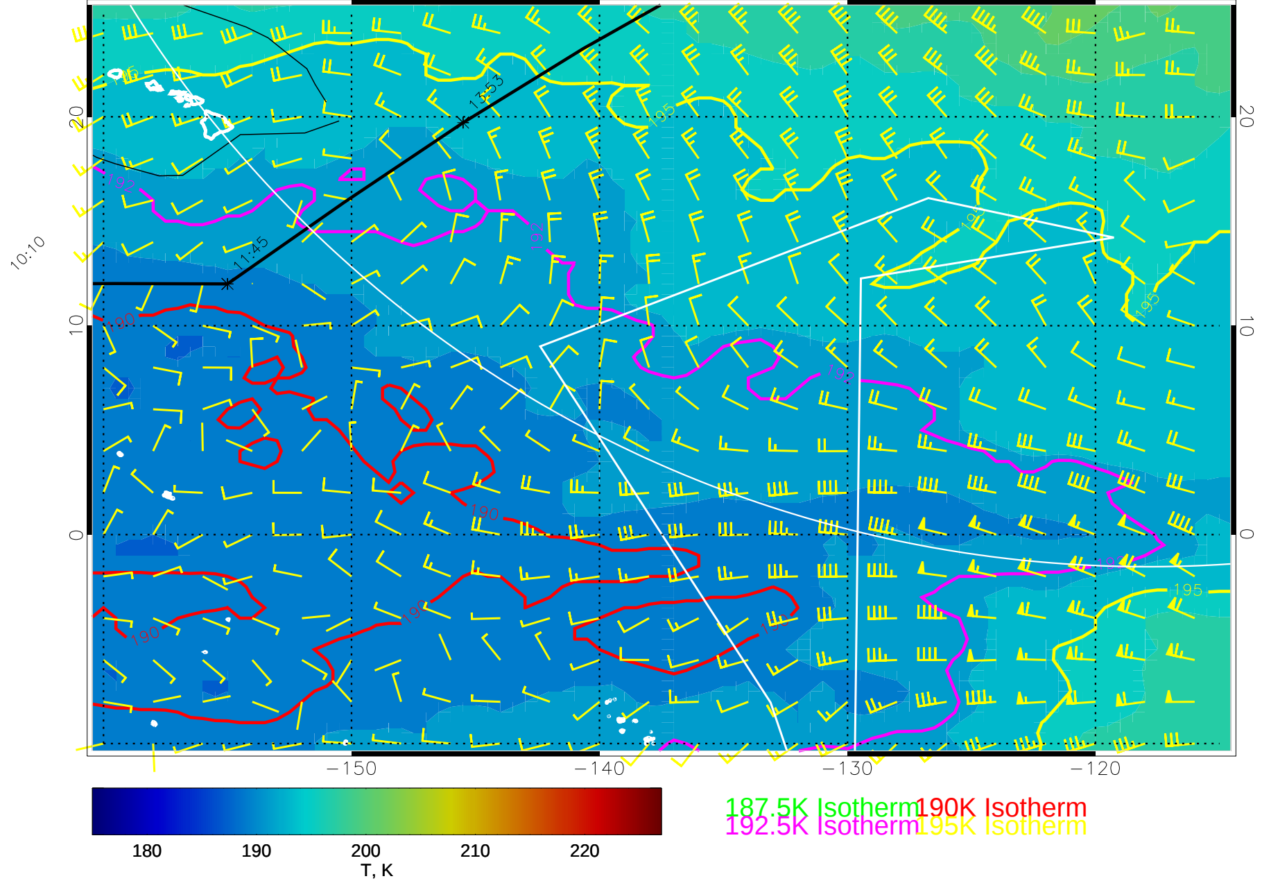
14121300, 48 hour forecast for 100mb T and winds (knots) -- NCEP GFS
