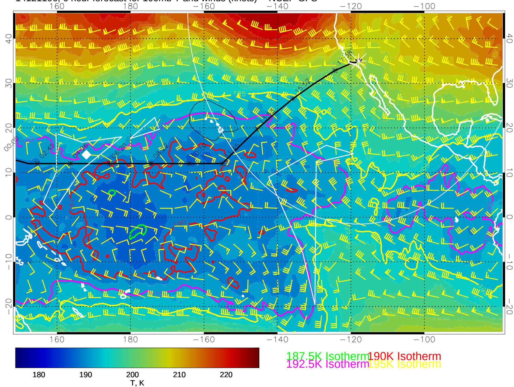
14121106, 6 hour forecast for 100mb T and winds (knots) -- NCEP GFS
