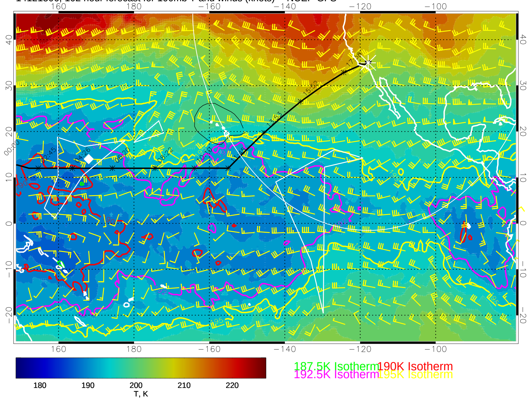
14121506, 102 hour forecast for 100mb T and winds (knots) -- NCEP GFS
