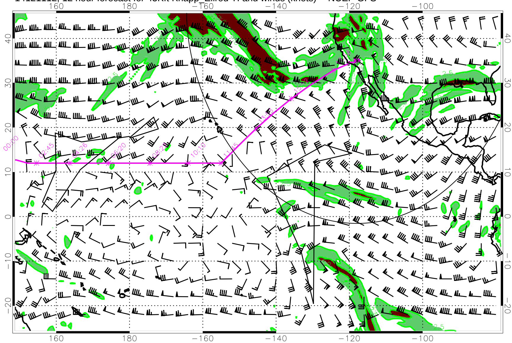
14121112, 12 hour forecast for 45Kft Knapp_Ellrod TI and winds (knots) -- NCEP GFS
