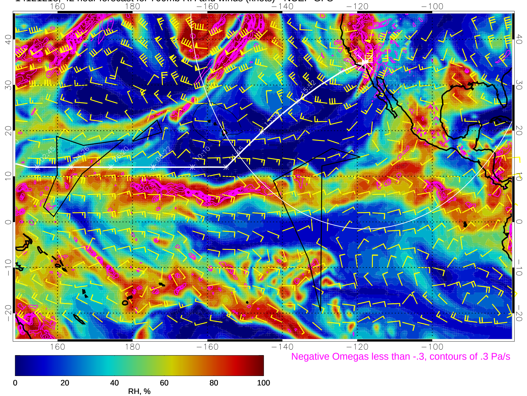
14121218, 42 hour forecast for 700mb RH and winds (knots) - NCEP GFS
