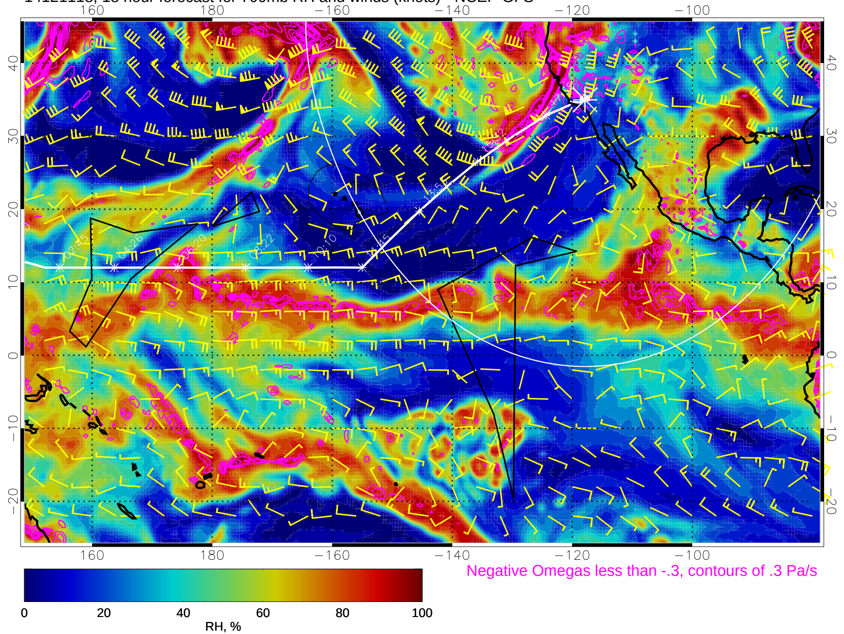
14121118, 18 hour forecast for 700mb RH and winds (knots) - NCEP GFS
