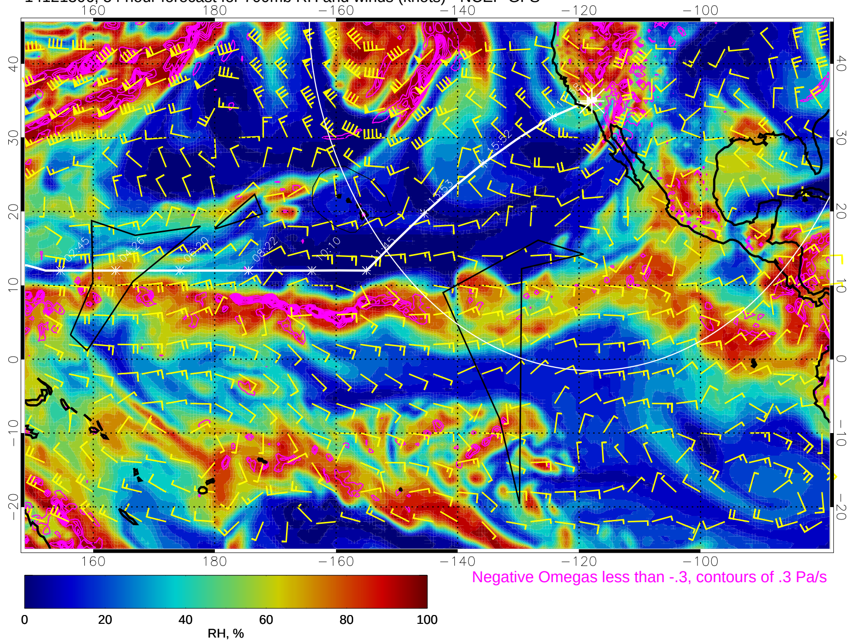
14121306, 54 hour forecast for 700mb RH and winds (knots) - NCEP GFS
