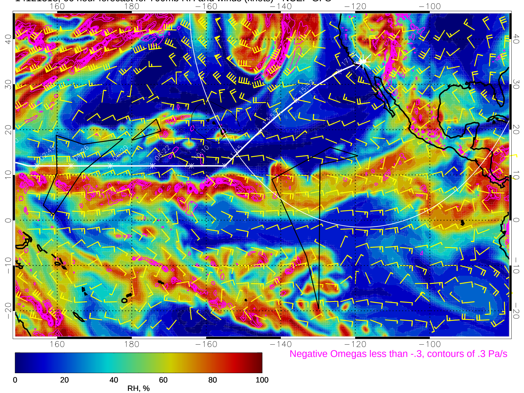
14121318, 66 hour forecast for 700mb RH and winds (knots) - NCEP GFS
