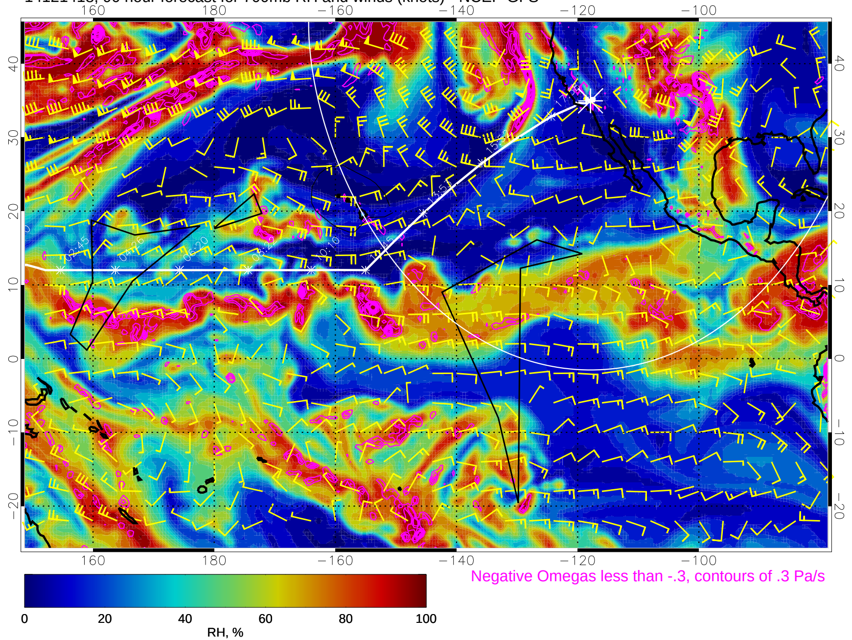
14121418, 90 hour forecast for 700mb RH and winds (knots) - NCEP GFS
