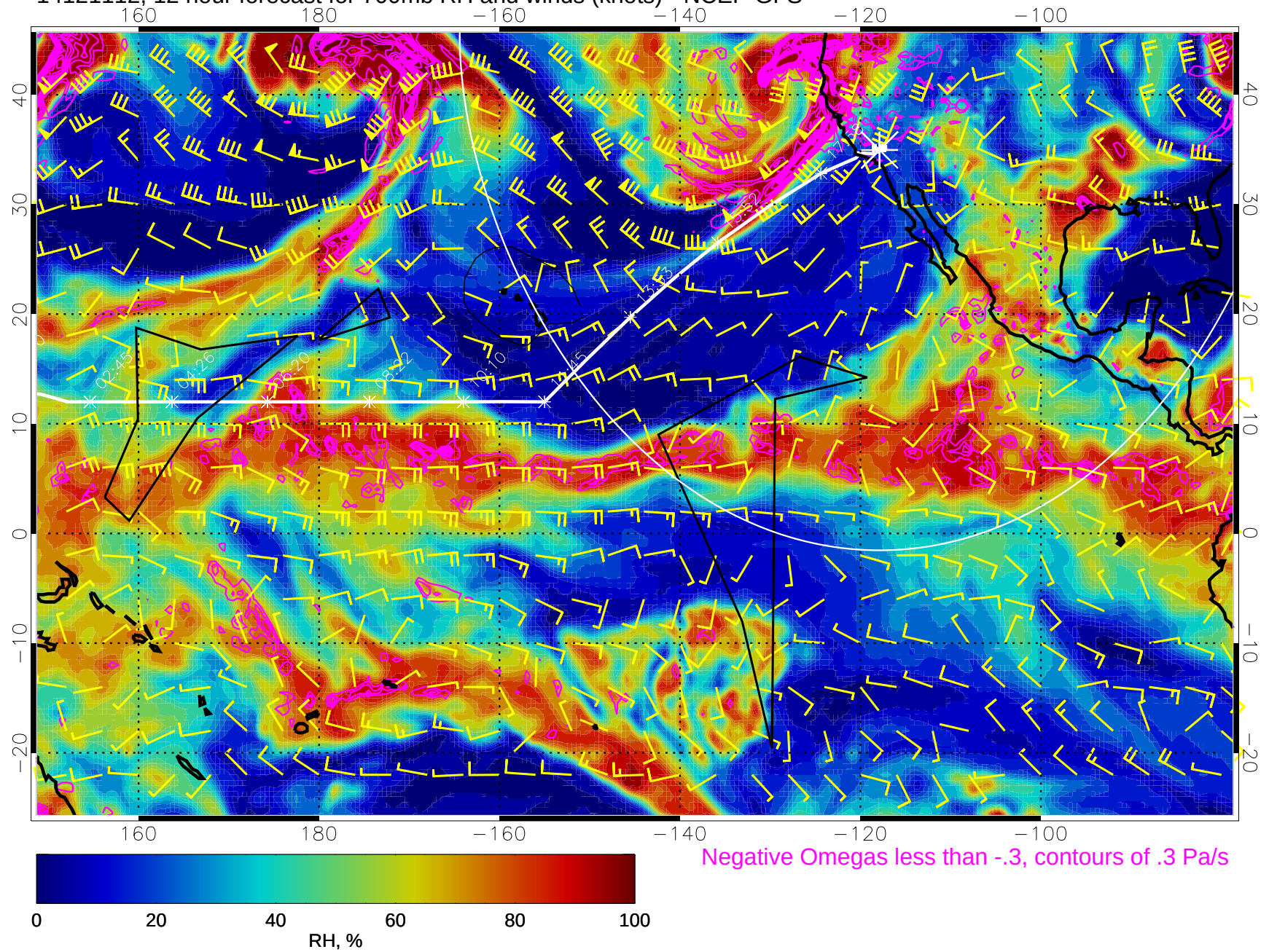
14121112, 12 hour forecast for 700mb RH and winds (knots) - NCEP GFS
