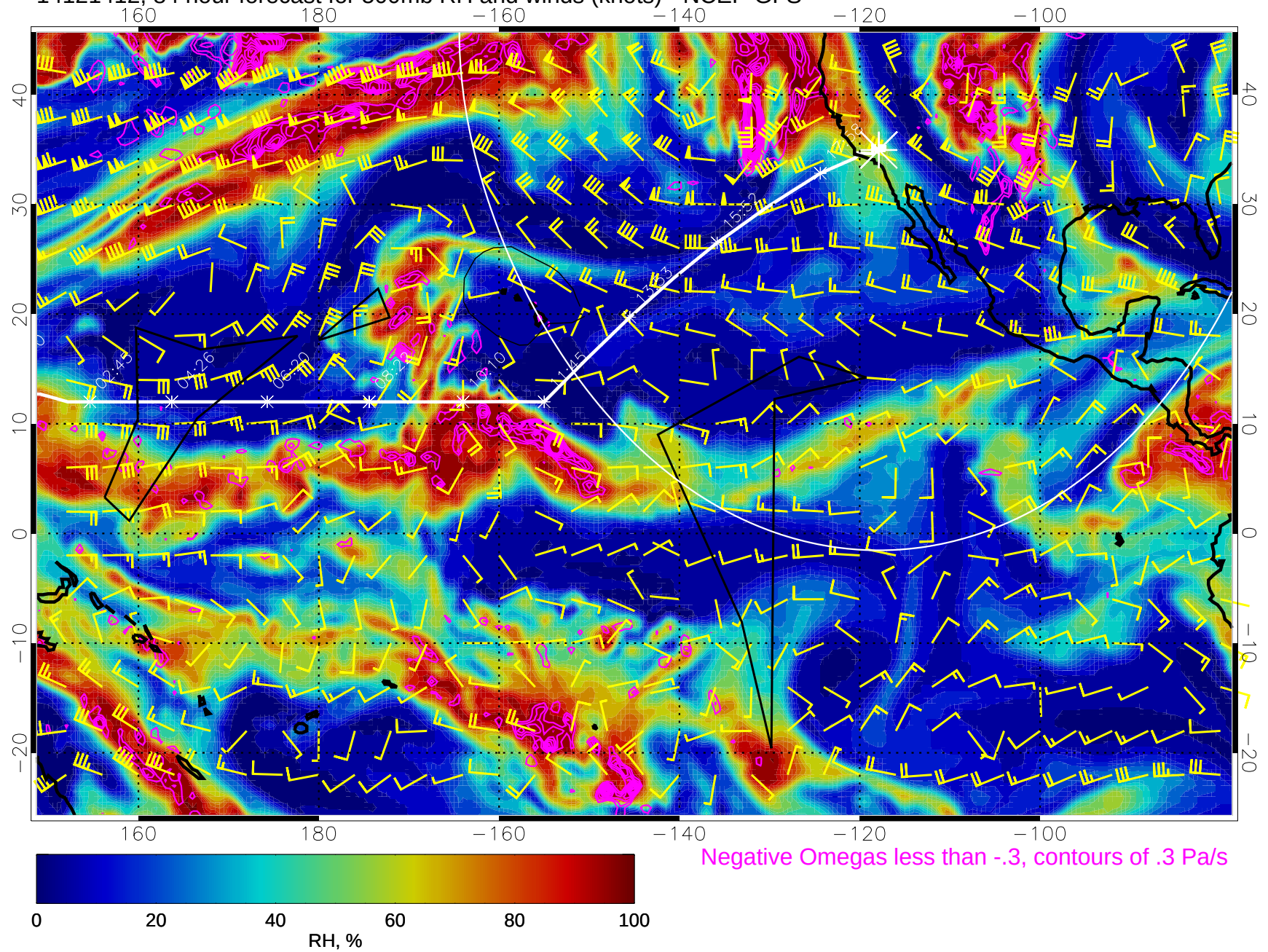
14121412, 84 hour forecast for 500mb RH and winds (knots) - NCEP GFS
