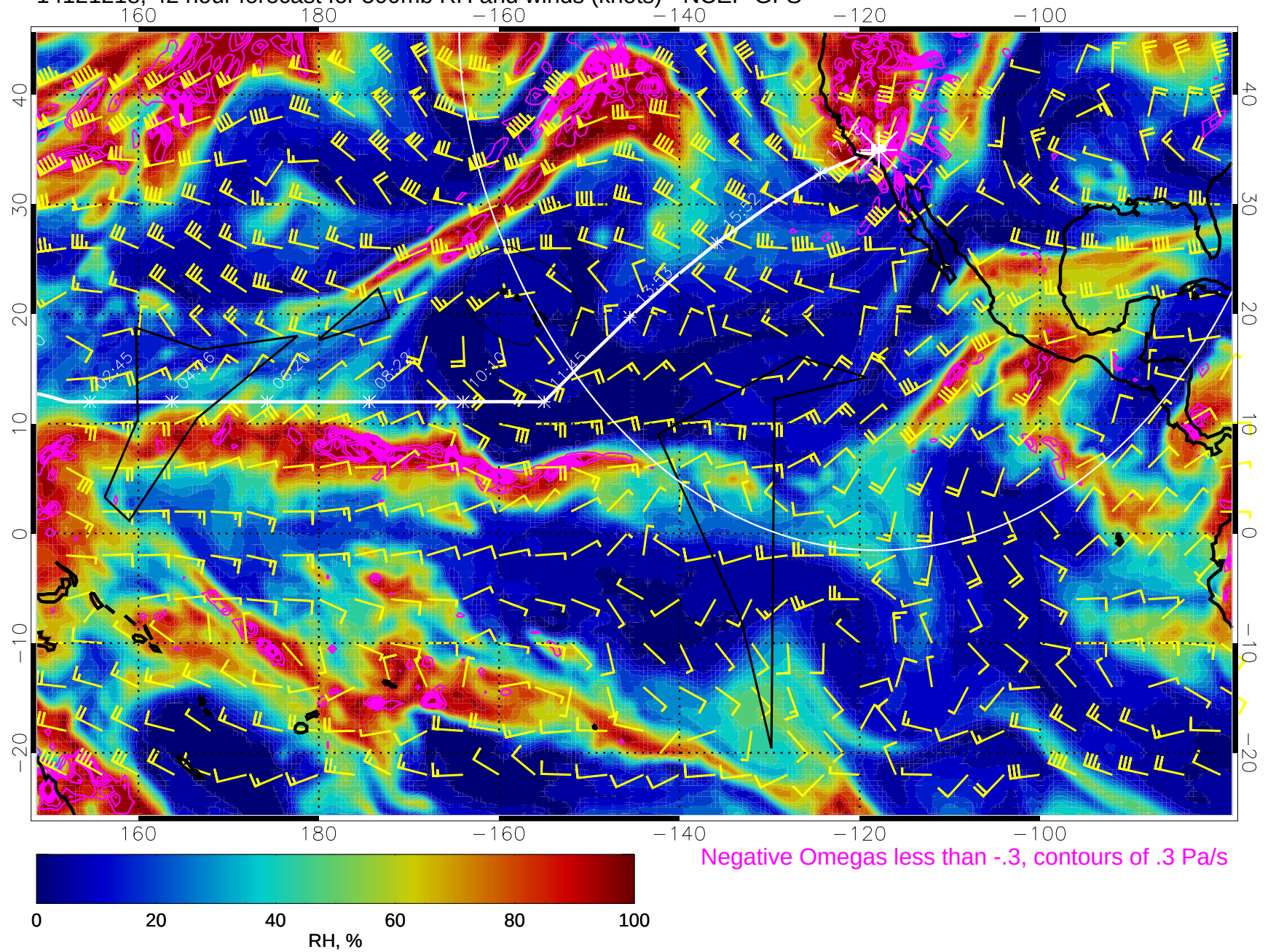
14121218, 42 hour forecast for 500mb RH and winds (knots) - NCEP GFS
