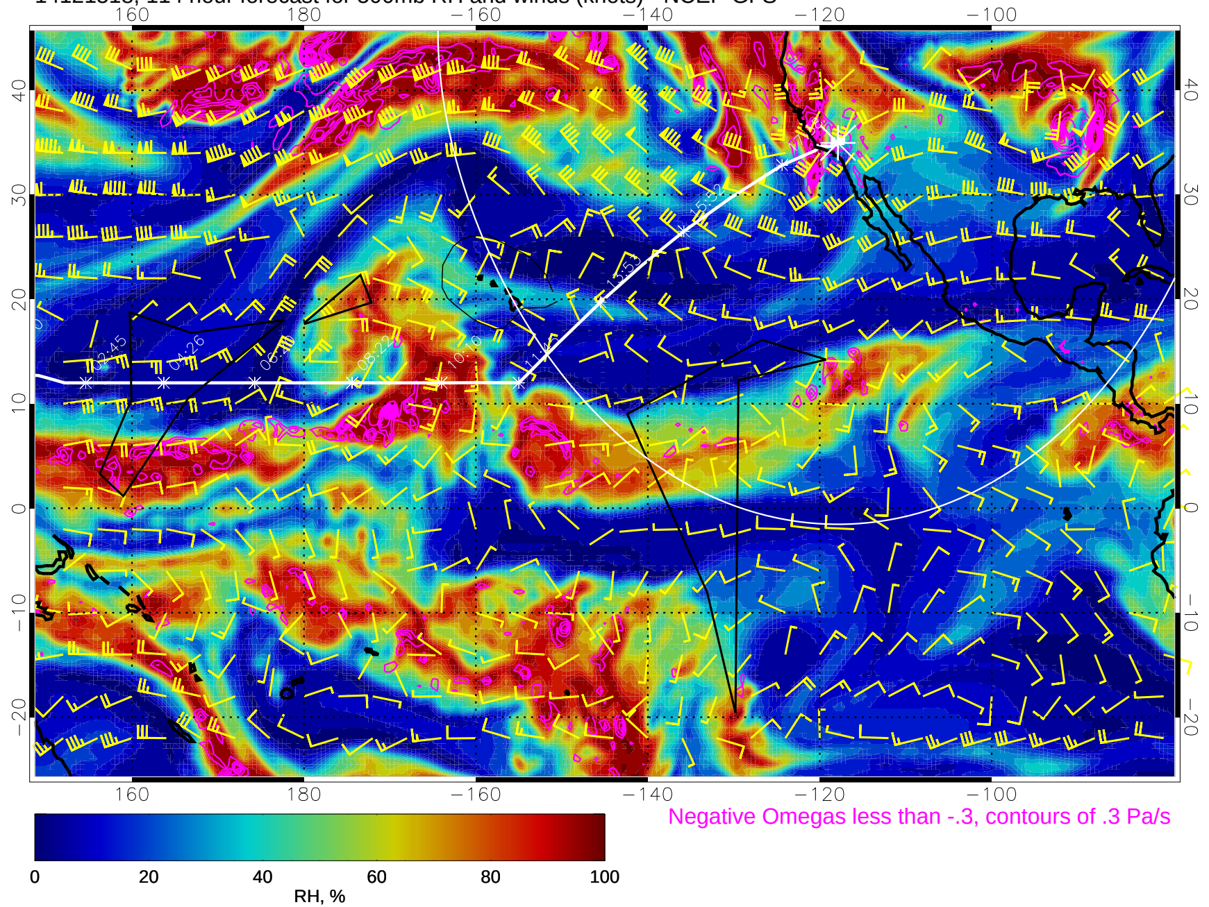
14121518, 114 hour forecast for 500mb RH and winds (knots) - NCEP GFS
