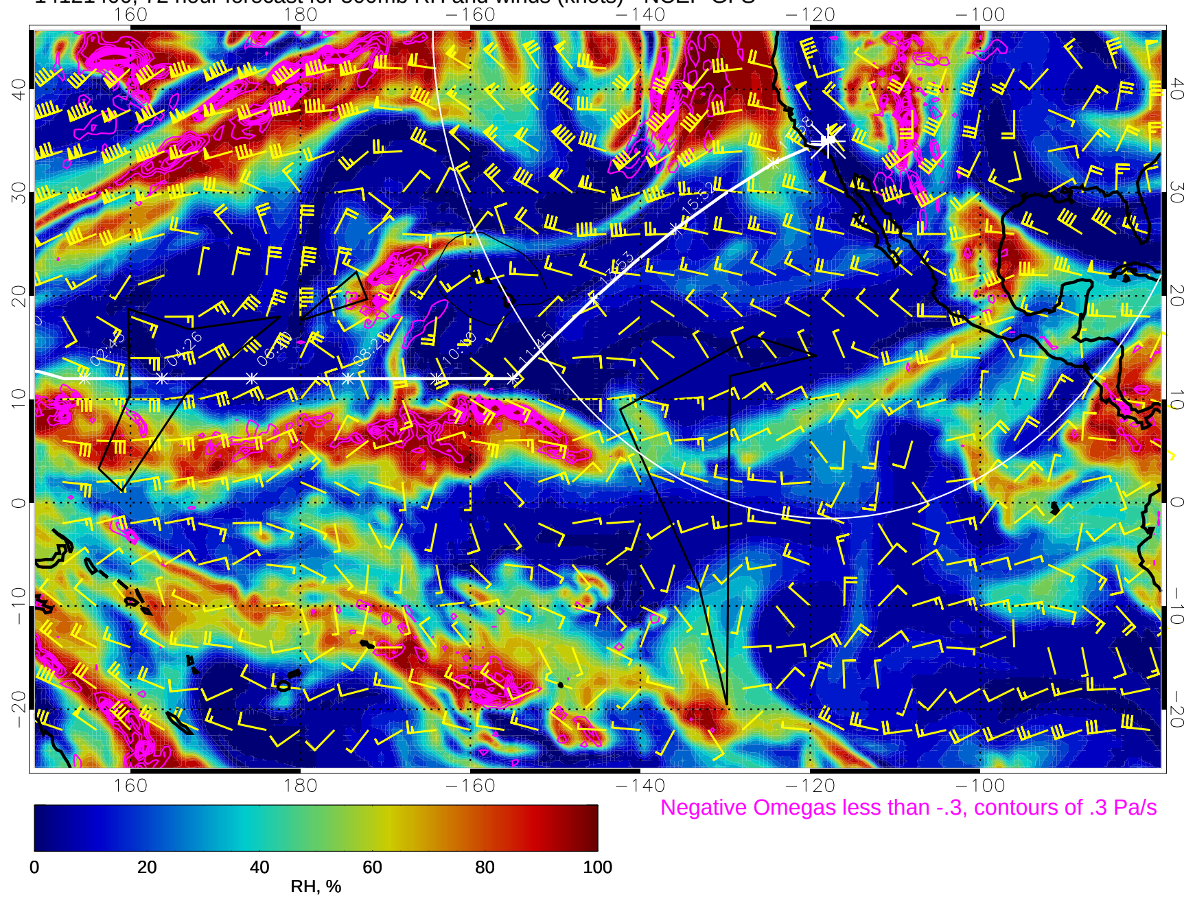
14121400, 72 hour forecast for 500mb RH and winds (knots) - NCEP GFS
