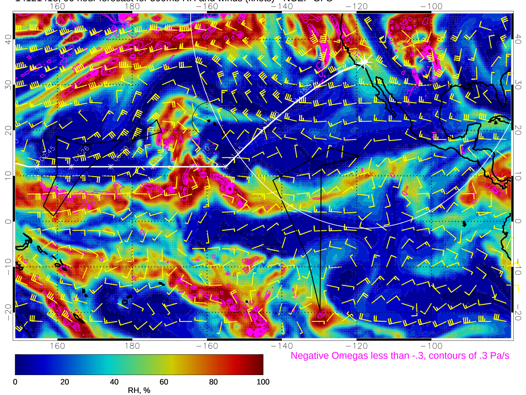
14121418, 90 hour forecast for 500mb RH and winds (knots) - NCEP GFS
