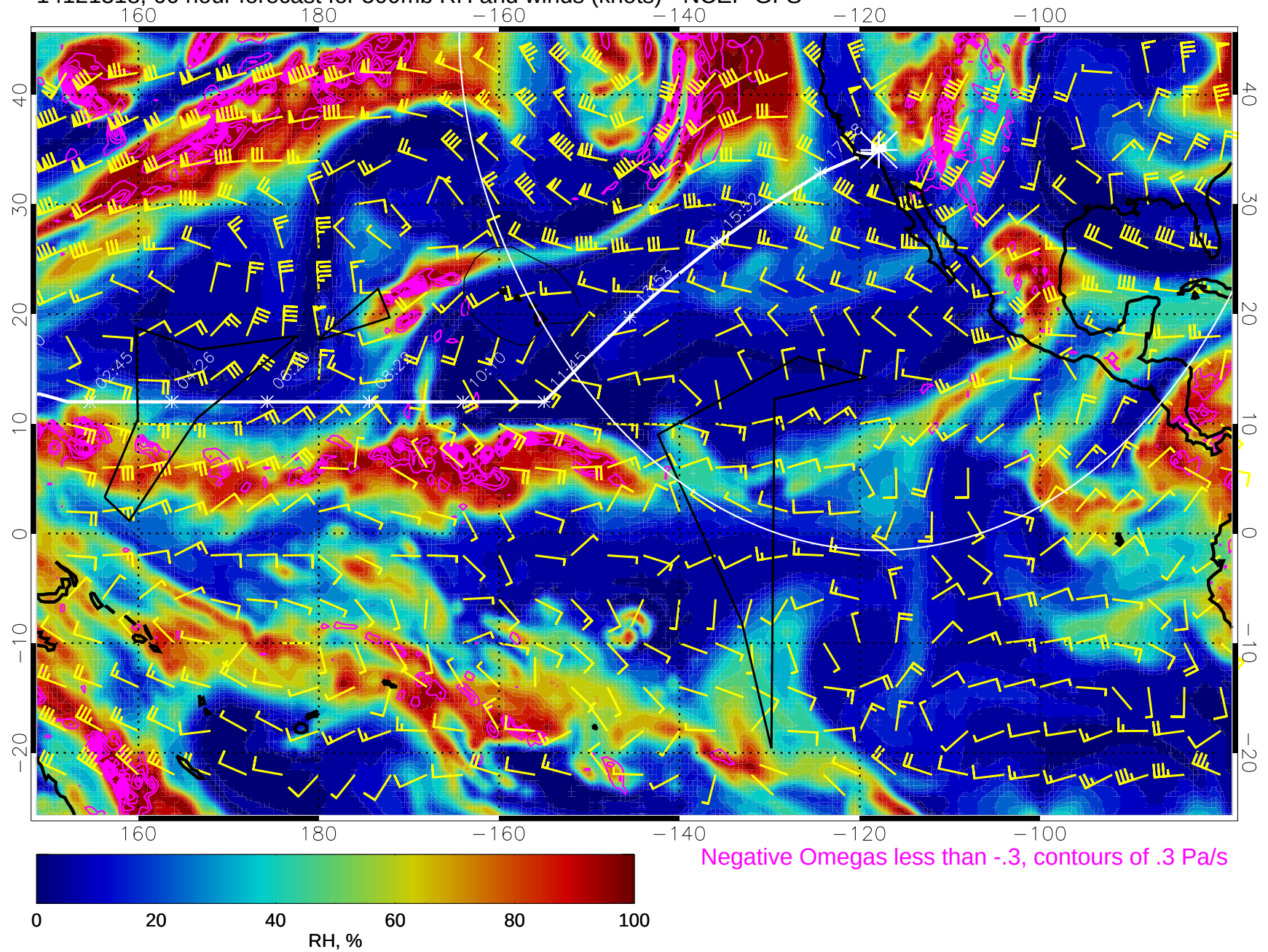
14121318, 66 hour forecast for 500mb RH and winds (knots) - NCEP GFS
