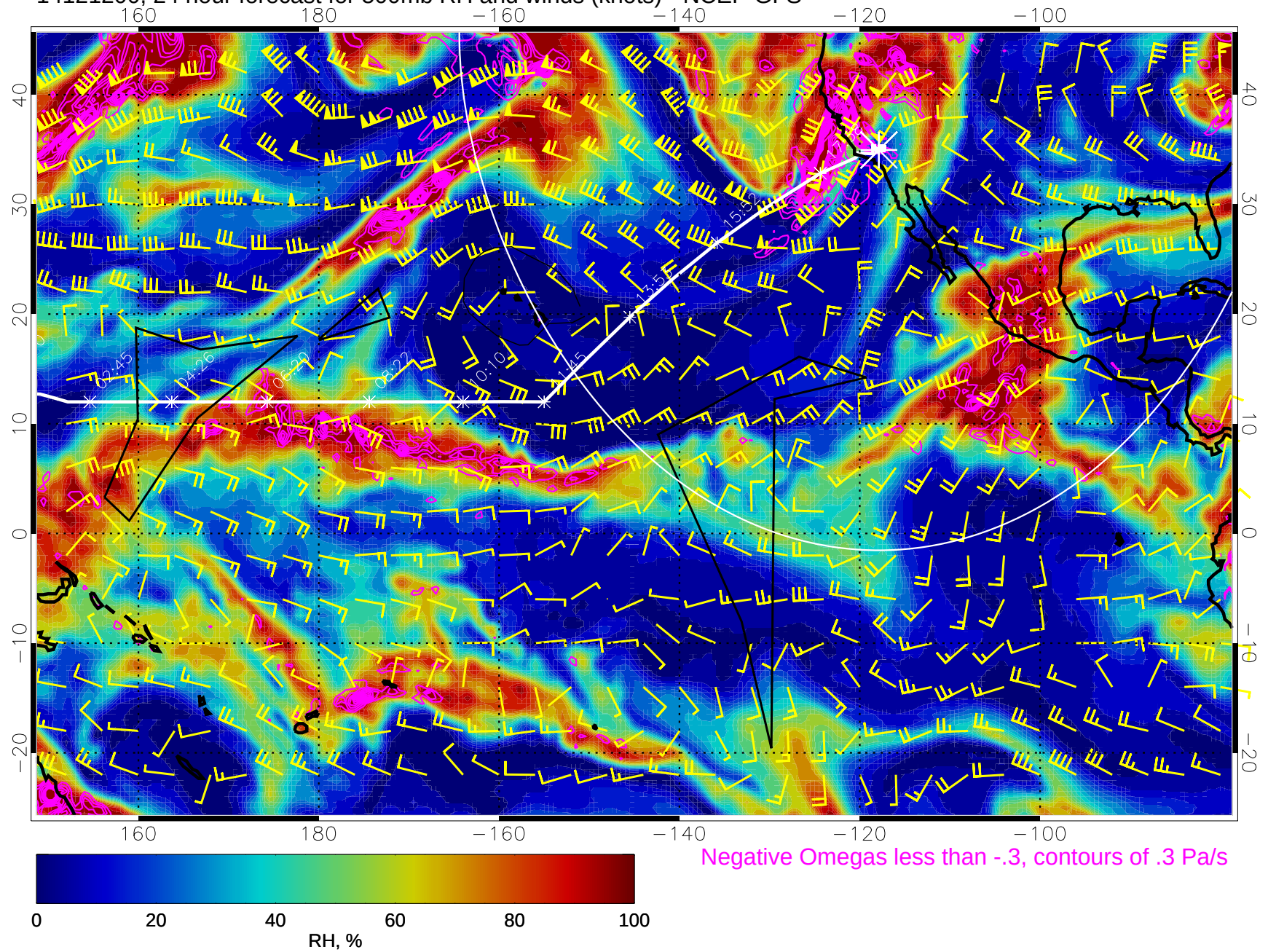
14121200, 24 hour forecast for 500mb RH and winds (knots) - NCEP GFS
