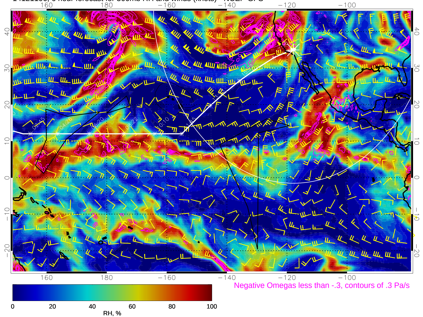
14121106, 6 hour forecast for 500mb RH and winds (knots) - NCEP GFS
