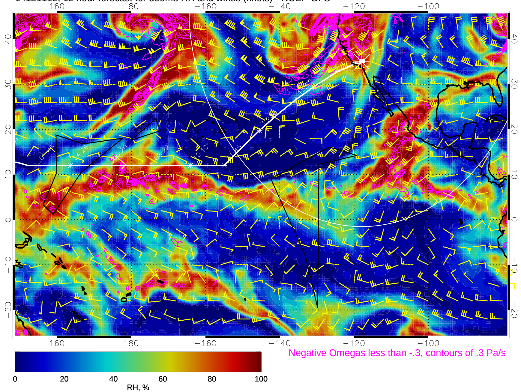
14121112, 12 hour forecast for 500mb RH and winds (knots) - NCEP GFS
