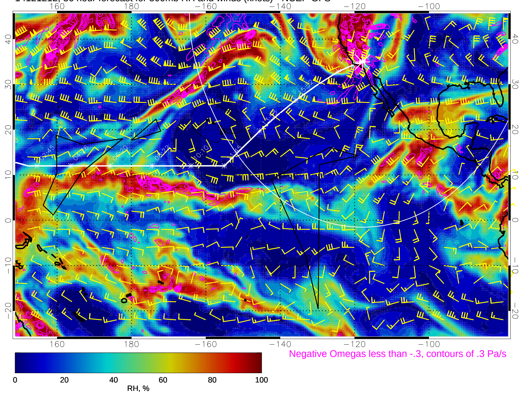
14121212, 36 hour forecast for 500mb RH and winds (knots) - NCEP GFS
