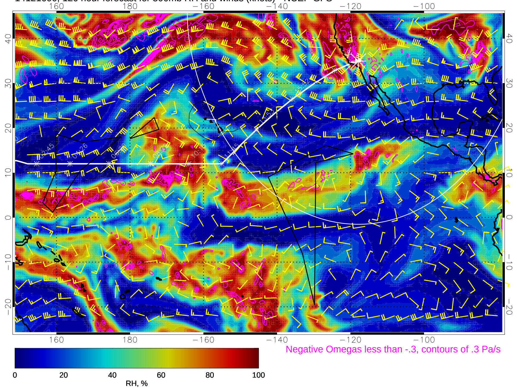
14121600, 120 hour forecast for 500mb RH and winds (knots) - NCEP GFS
