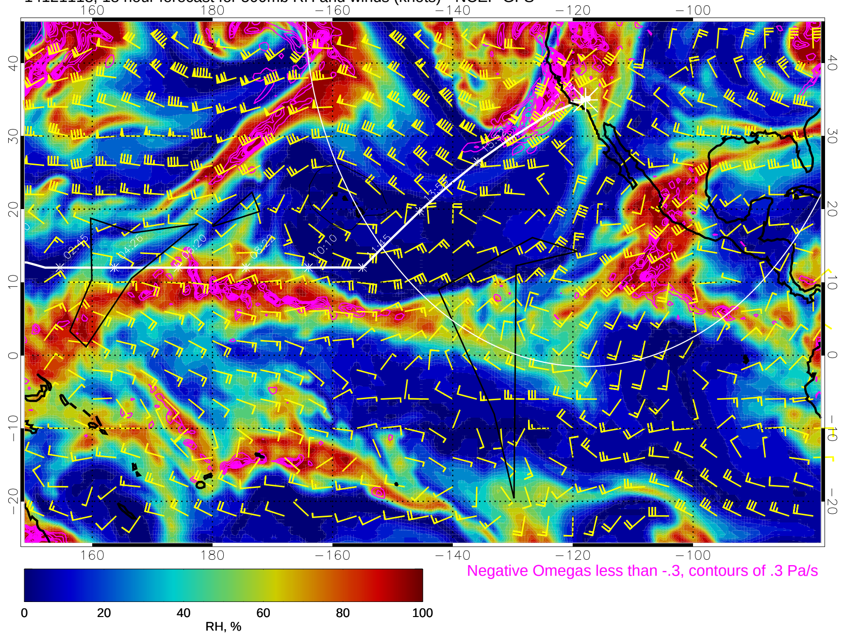
14121118, 18 hour forecast for 500mb RH and winds (knots) - NCEP GFS
