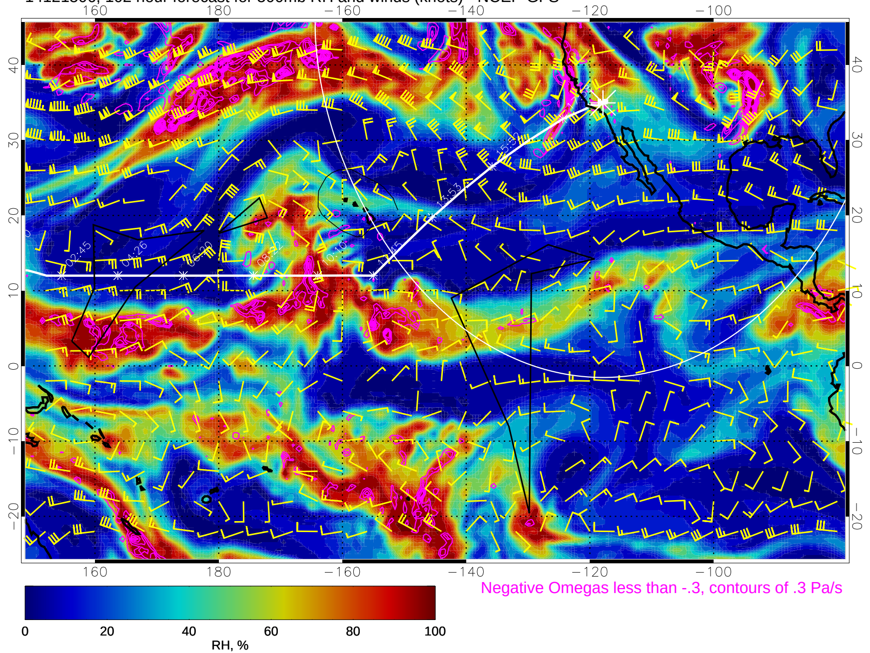
14121506, 102 hour forecast for 500mb RH and winds (knots) - NCEP GFS
