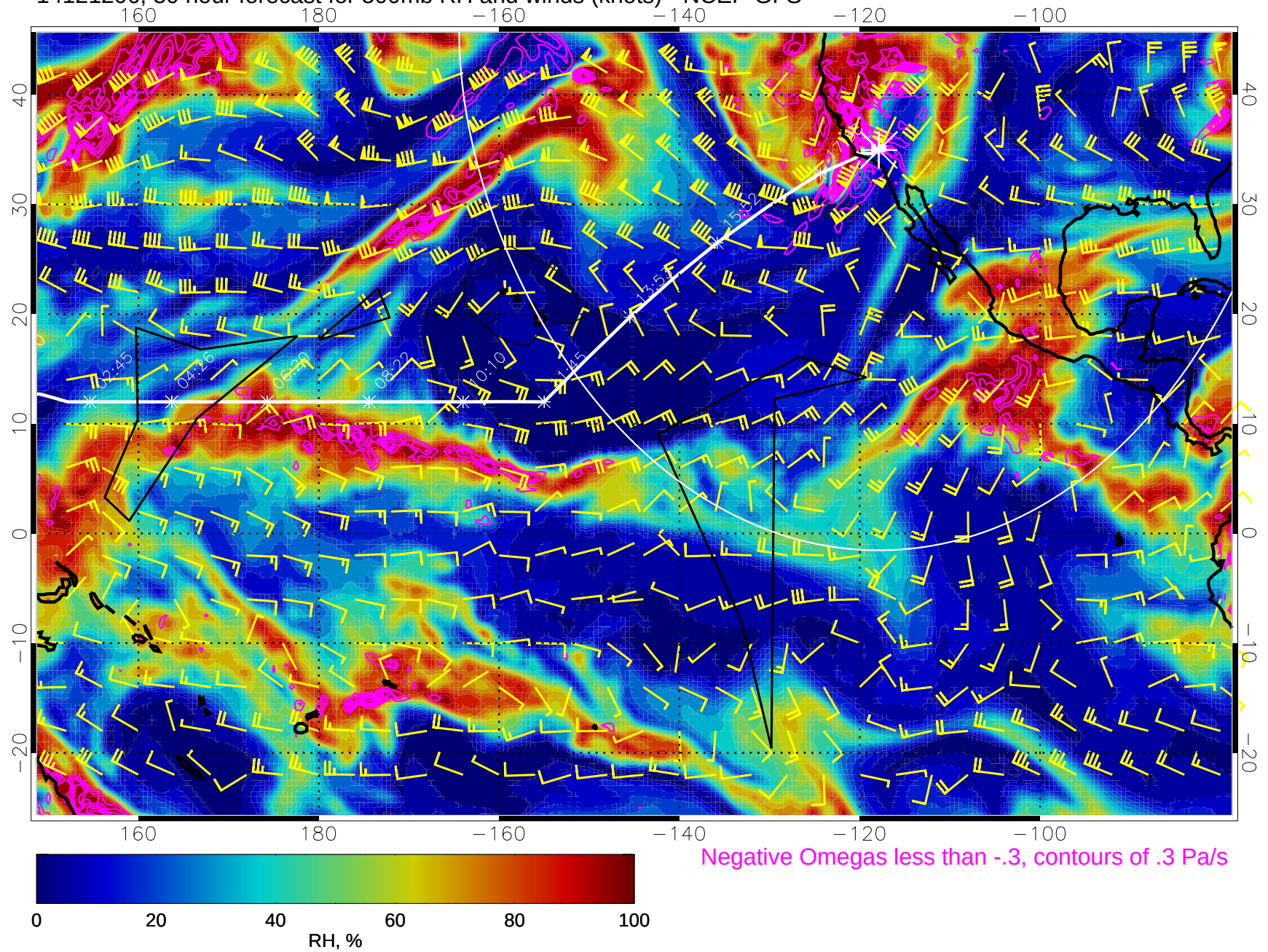
14121206, 30 hour forecast for 500mb RH and winds (knots) - NCEP GFS
