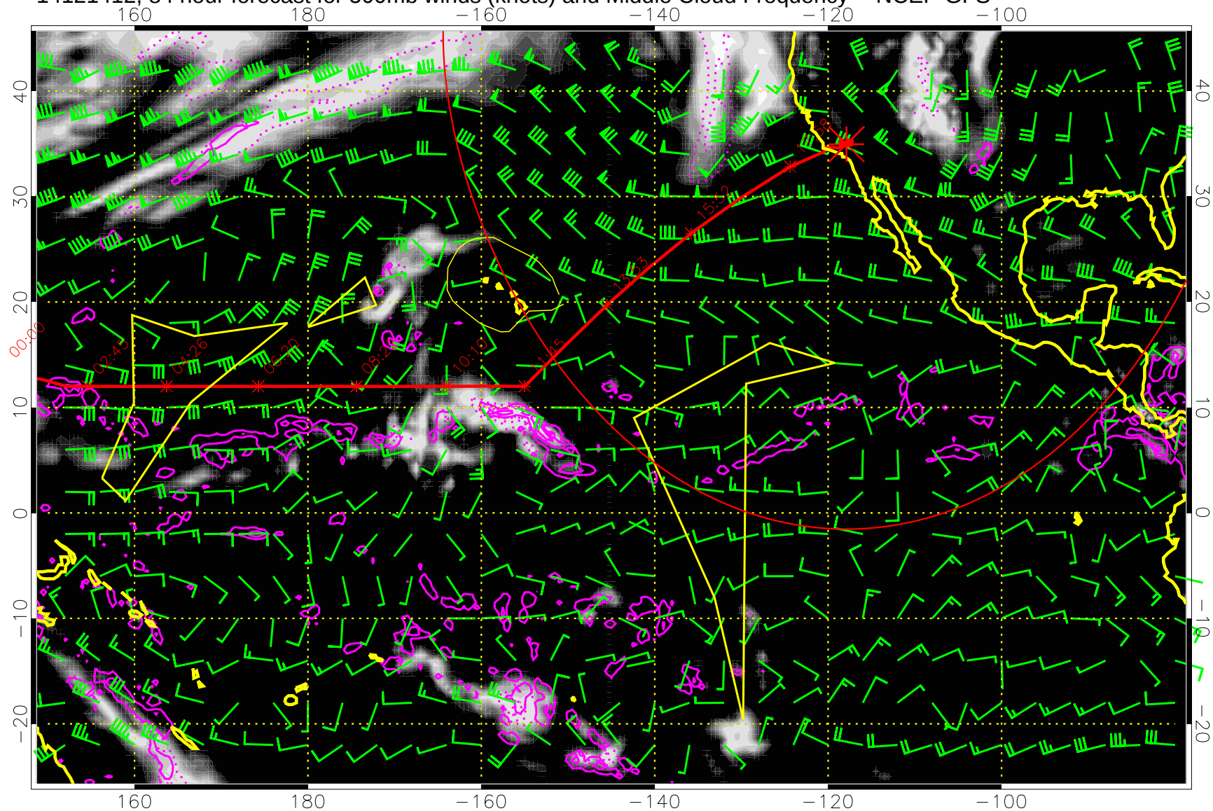
14121412, 84 hour forecast for 500mb winds (knots) and Middle Cloud Frequency -- NCEP GFS
