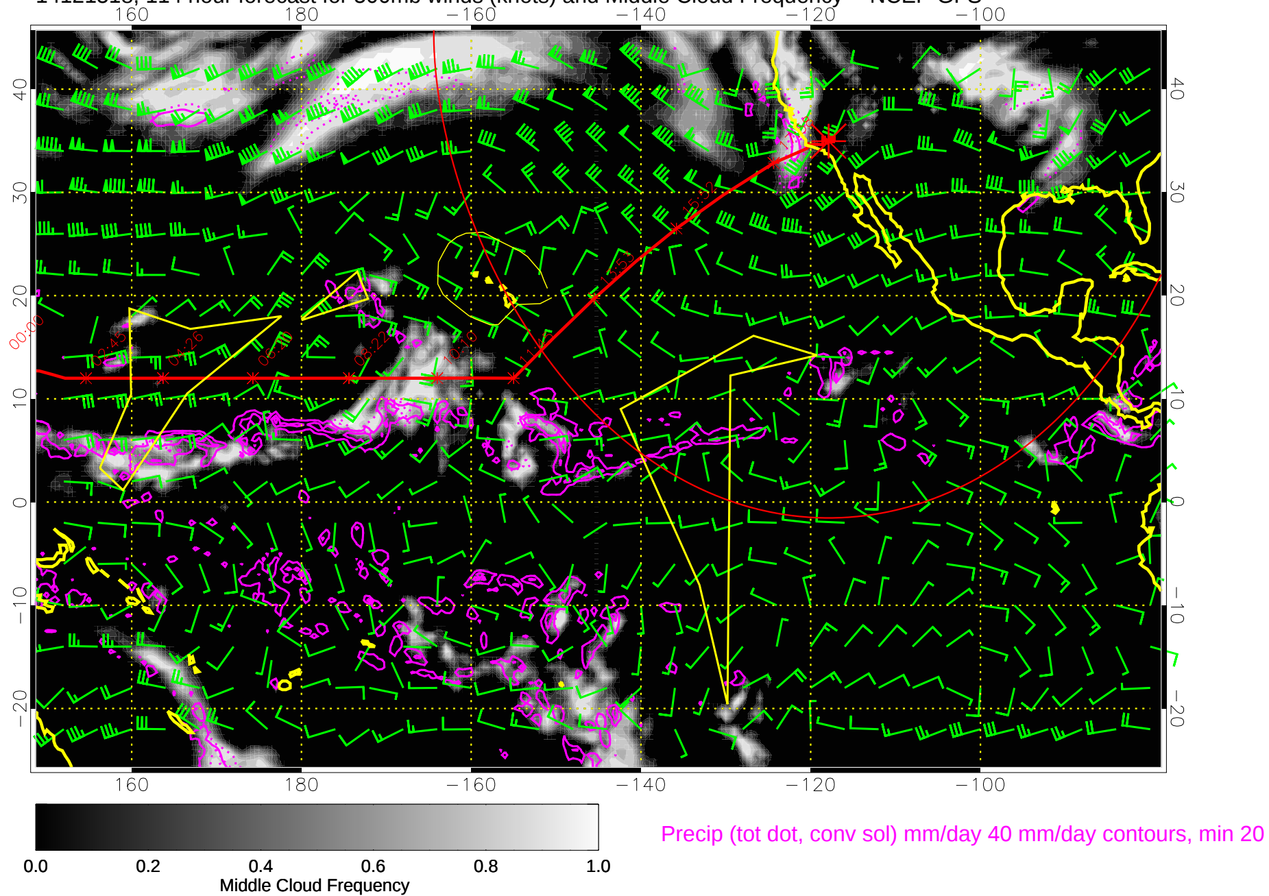
14121518, 114 hour forecast for 500mb winds (knots) and Middle Cloud Frequency -- NCEP GFS
