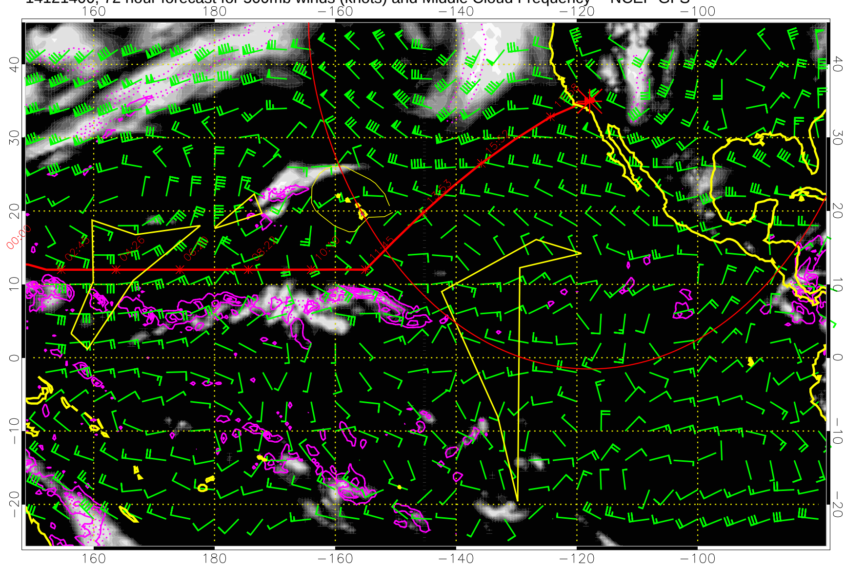
14121400, 72 hour forecast for 500mb winds (knots) and Middle Cloud Frequency -- NCEP GFS
