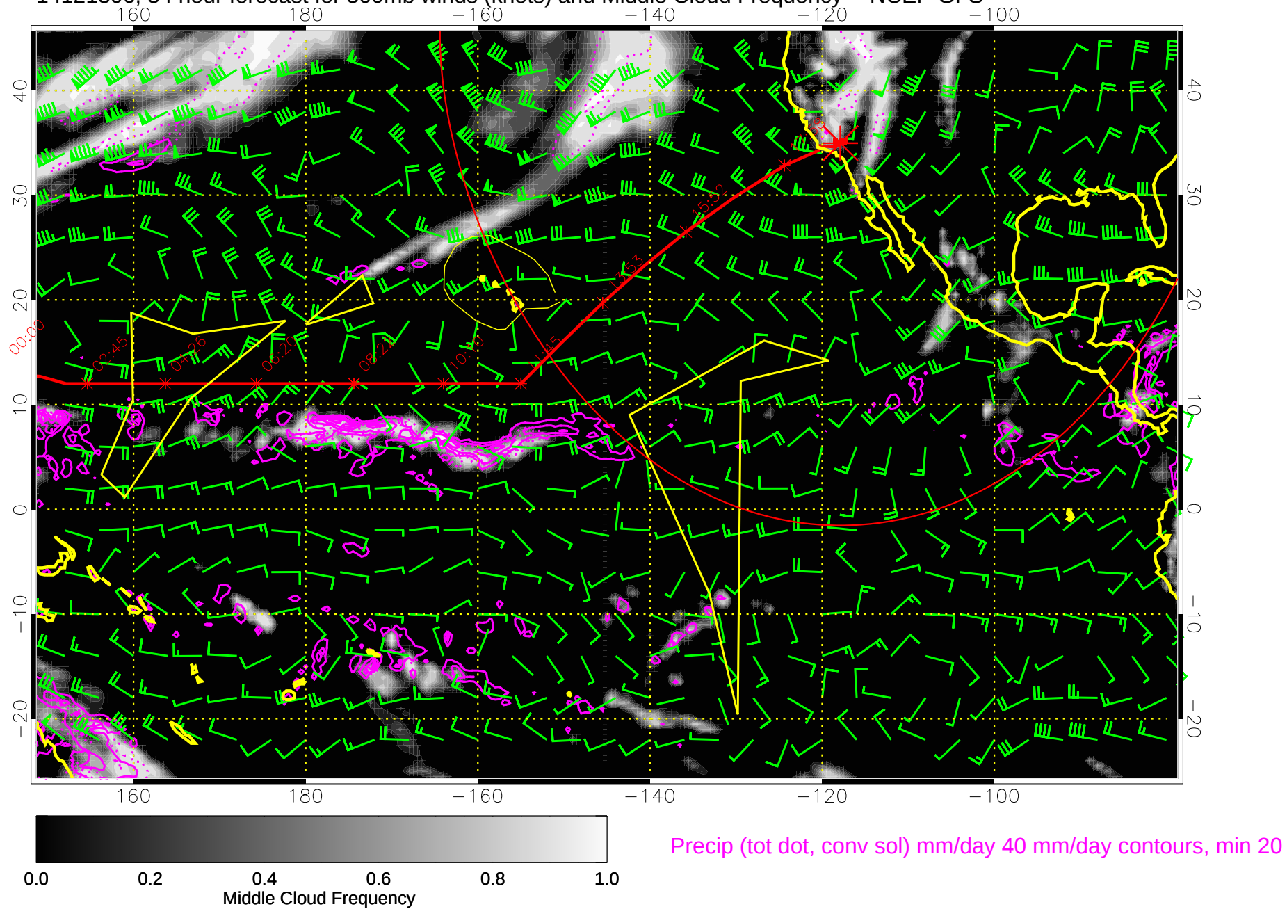
14121306, 54 hour forecast for 500mb winds (knots) and Middle Cloud Frequency -- NCEP GFS
