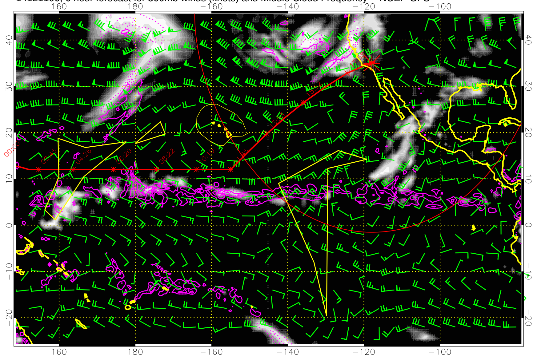
14121106, 6 hour forecast for 500mb winds (knots) and Middle Cloud Frequency -- NCEP GFS
