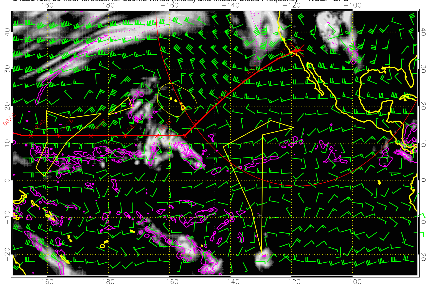
14121418, 90 hour forecast for 500mb winds (knots) and Middle Cloud Frequency -- NCEP GFS
