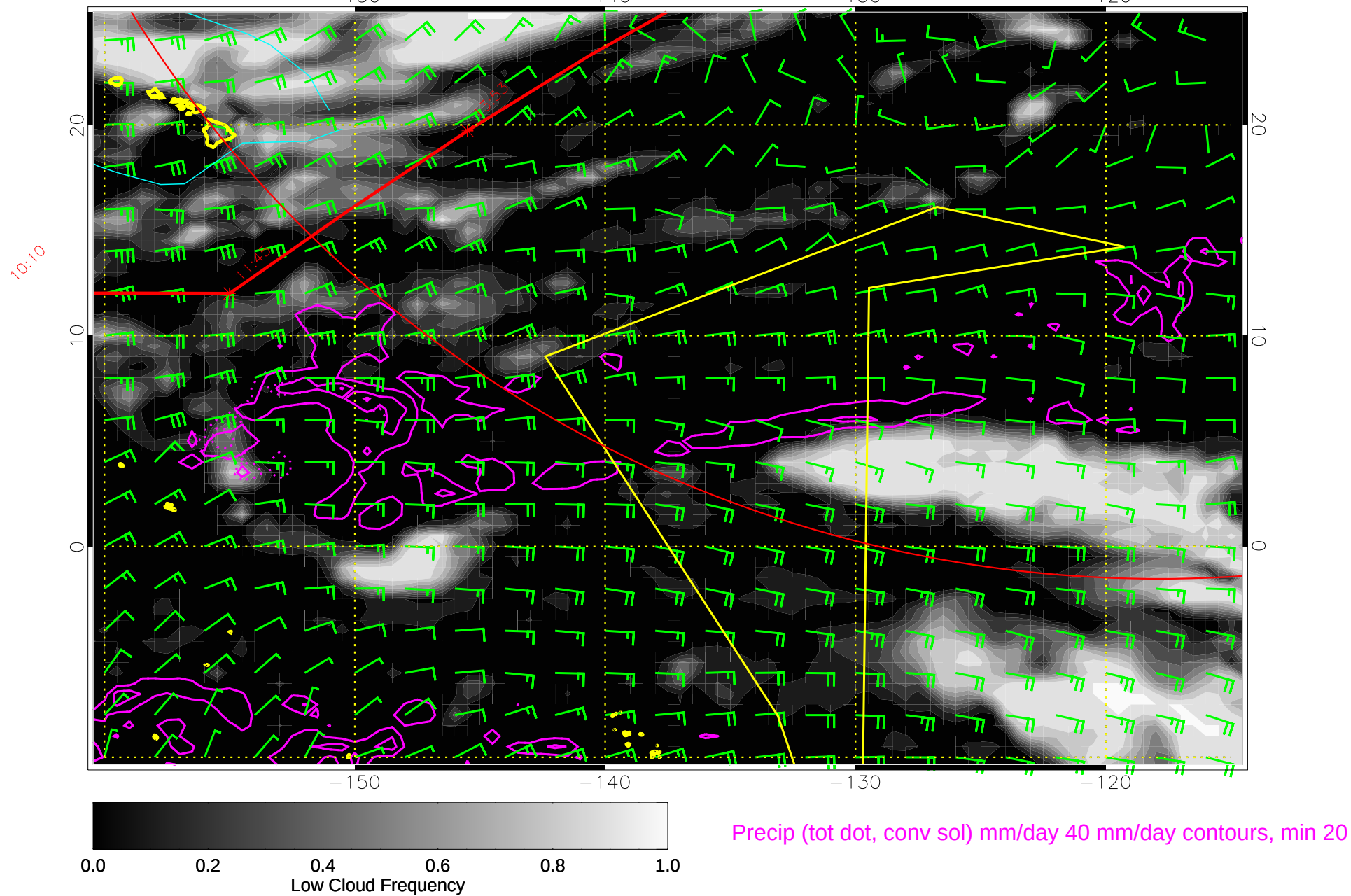
14121512, 108 hour forecast for 850mb winds (knots) and Low Cloud Frequency -- NCEP GFS
