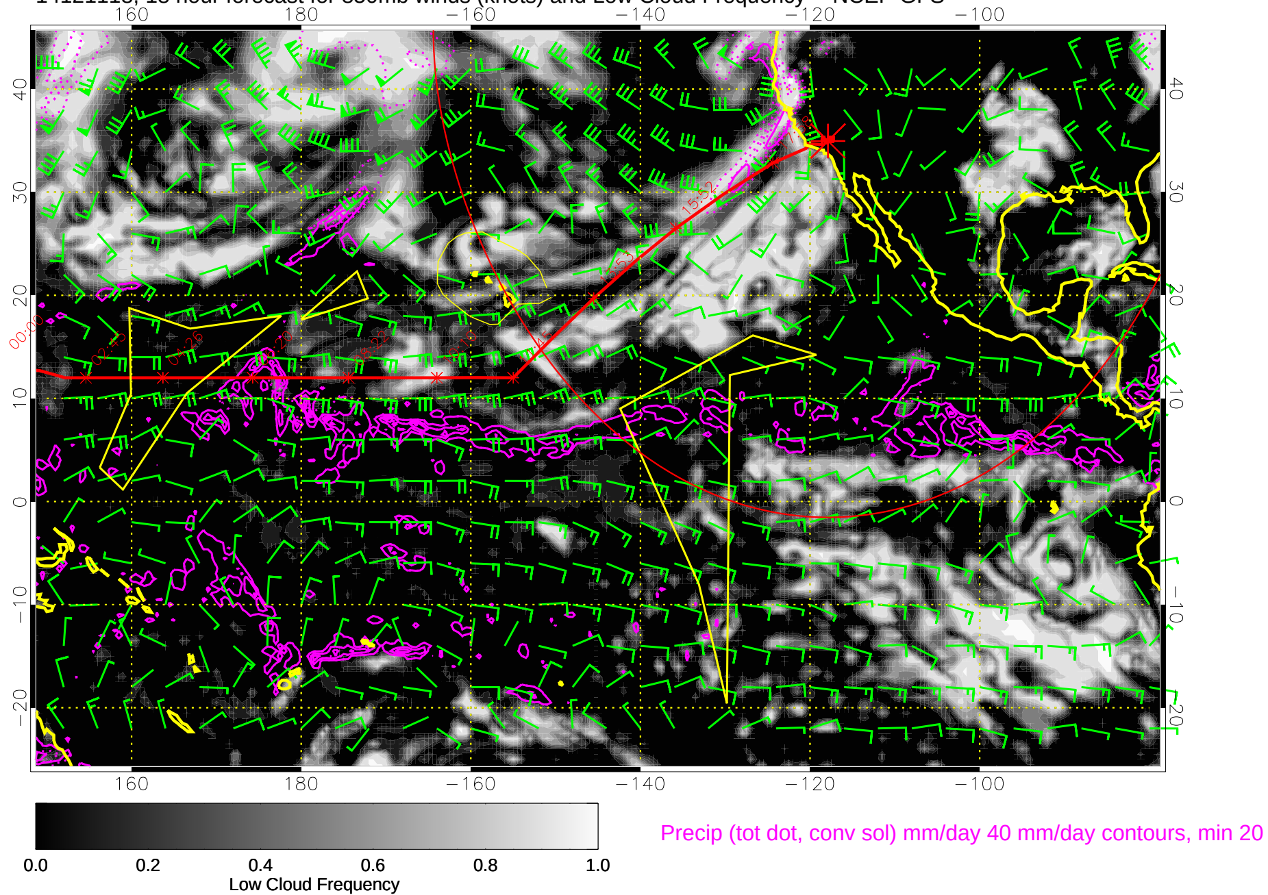
14121118, 18 hour forecast for 850mb winds (knots) and Low Cloud Frequency -- NCEP GFS
