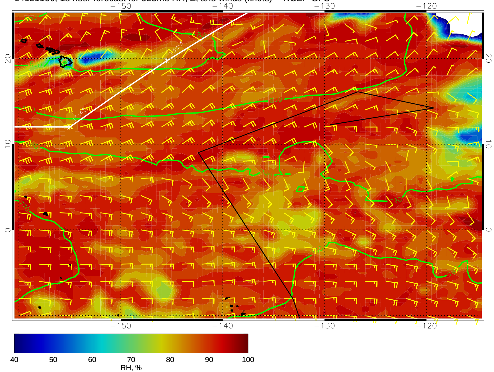
14121106, 18 hour forecast for 925mb RH, Z, and winds (knots) -- NCEP GFS
