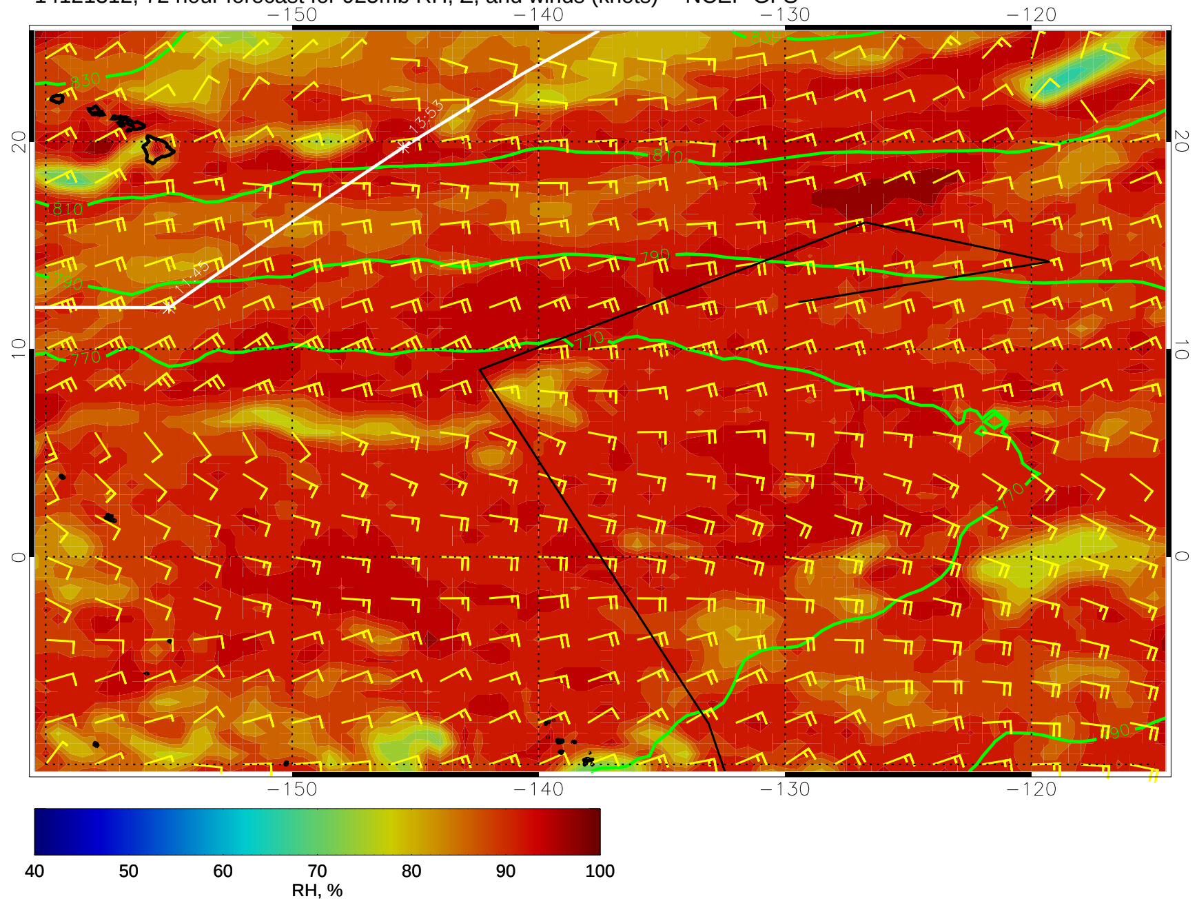
14121312, 72 hour forecast for 925mb RH, Z, and winds (knots) -- NCEP GFS
