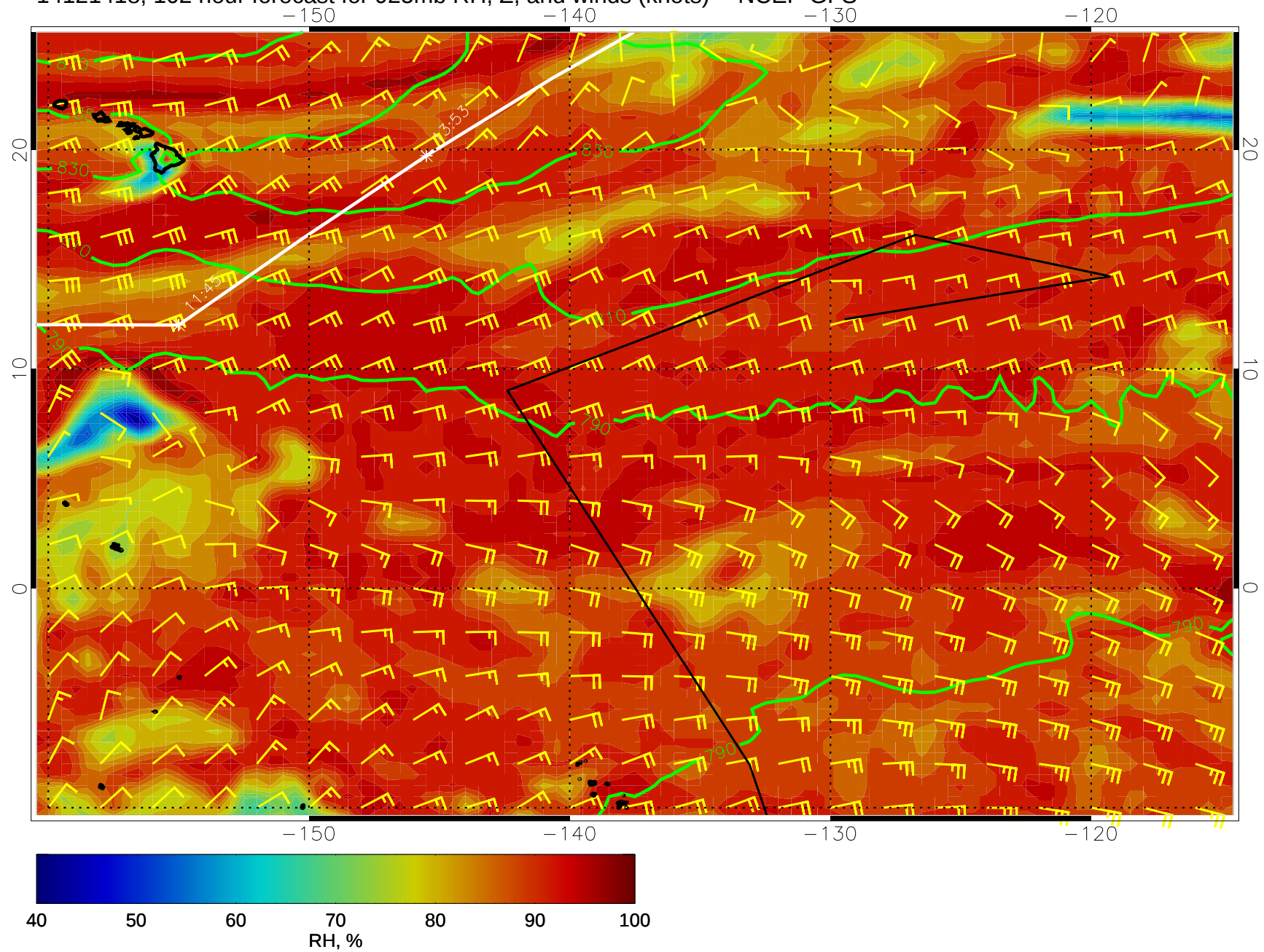
14121418, 102 hour forecast for 925mb RH, Z, and winds (knots) -- NCEP GFS
