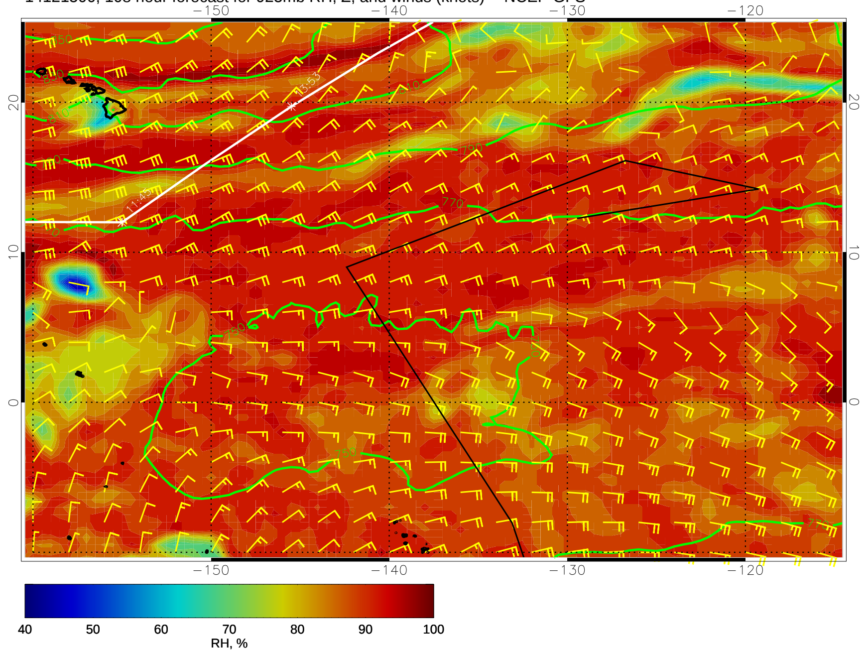
14121500, 108 hour forecast for 925mb RH, Z, and winds (knots) -- NCEP GFS
