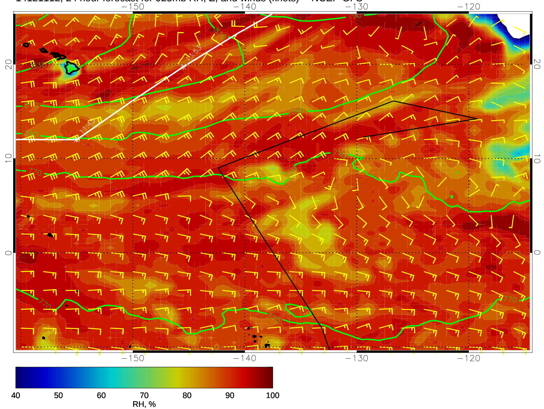
14121112, 24 hour forecast for 925mb RH, Z, and winds (knots) -- NCEP GFS
