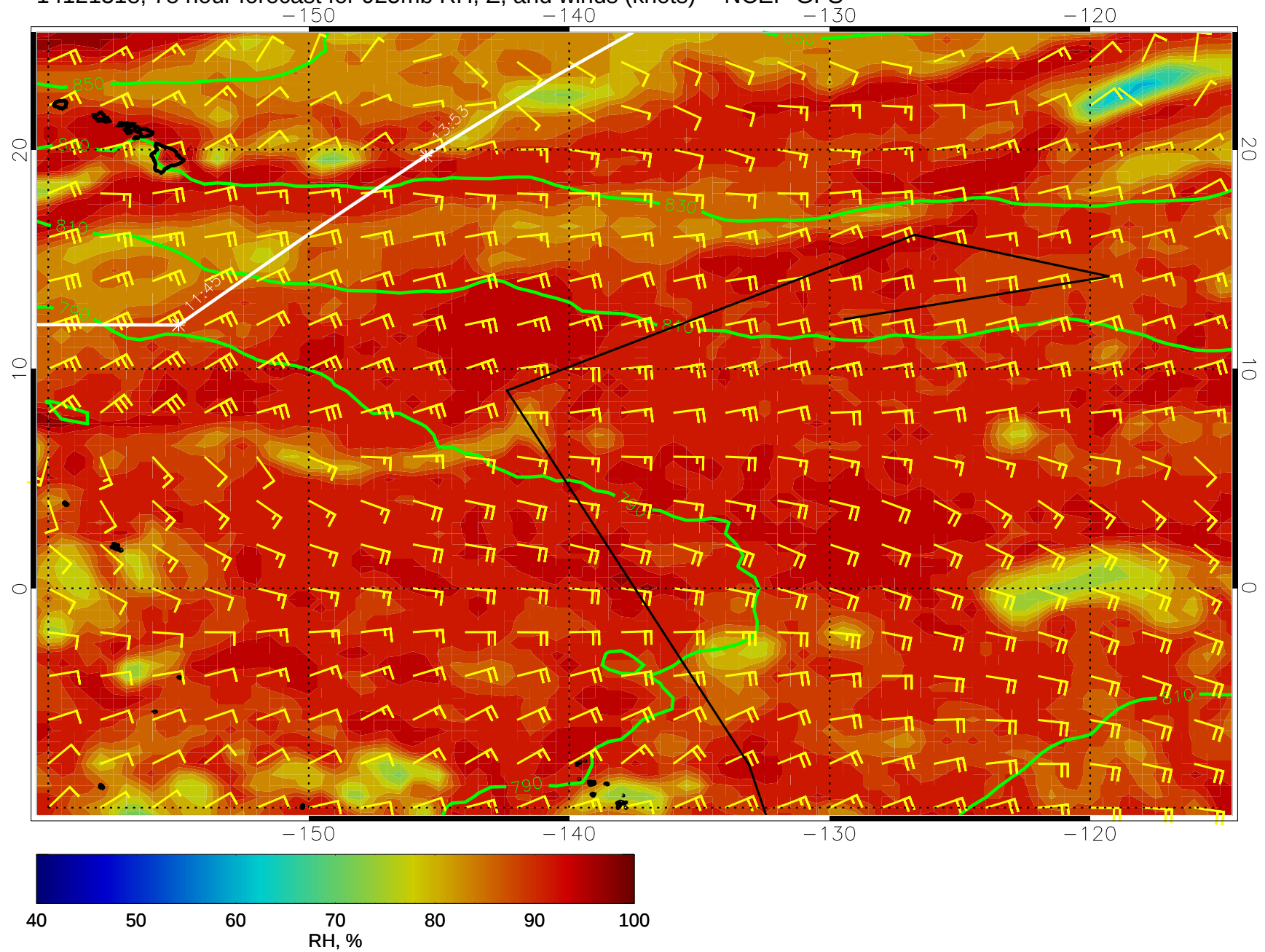
14121318, 78 hour forecast for 925mb RH, Z, and winds (knots) -- NCEP GFS
