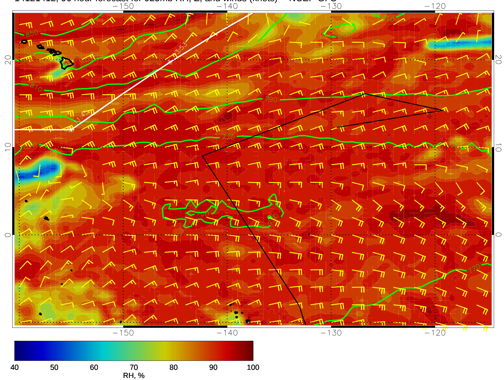
14121412, 96 hour forecast for 925mb RH, Z, and winds (knots) -- NCEP GFS
