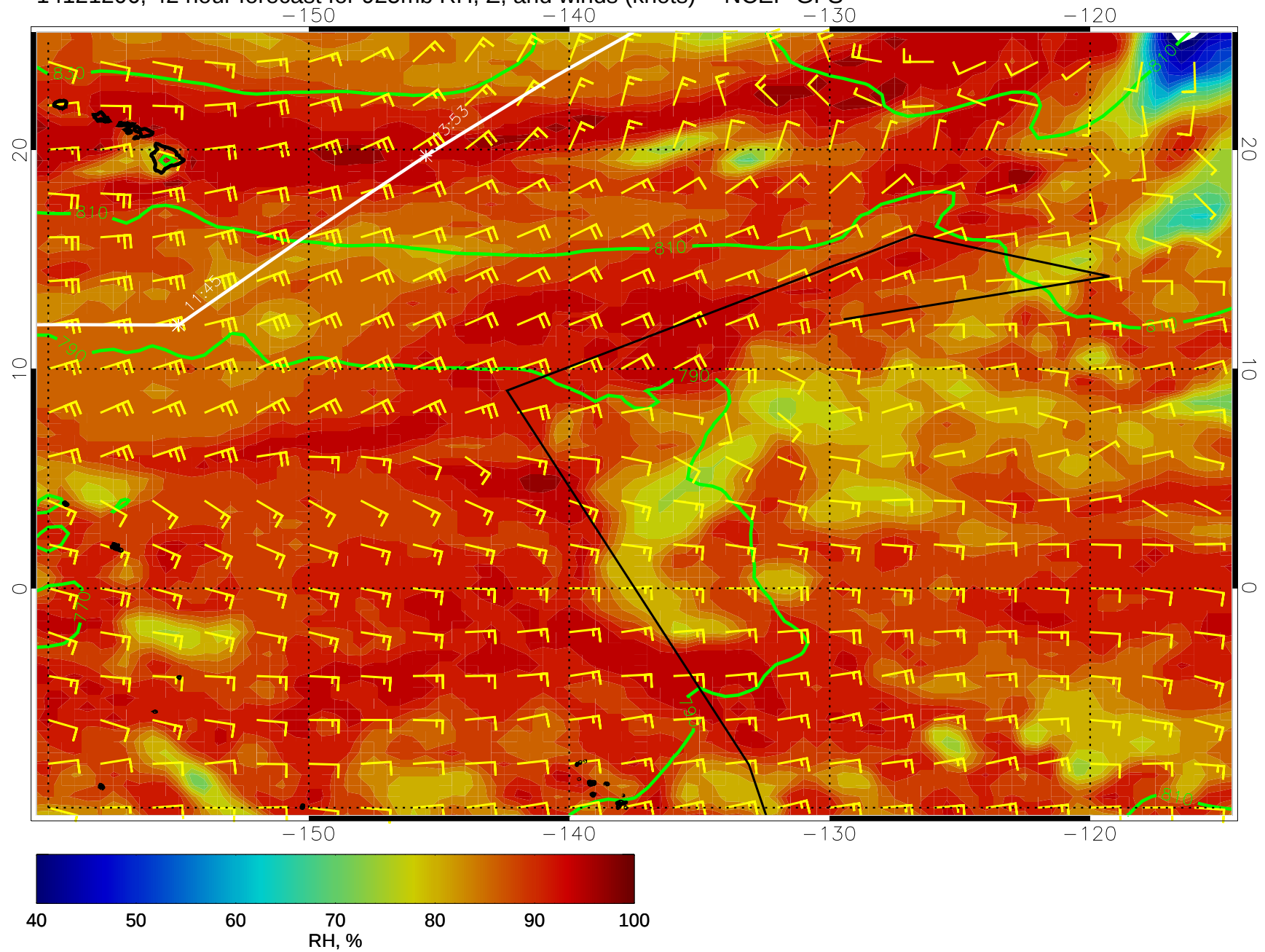
14121206, 42 hour forecast for 925mb RH, Z, and winds (knots) -- NCEP GFS
