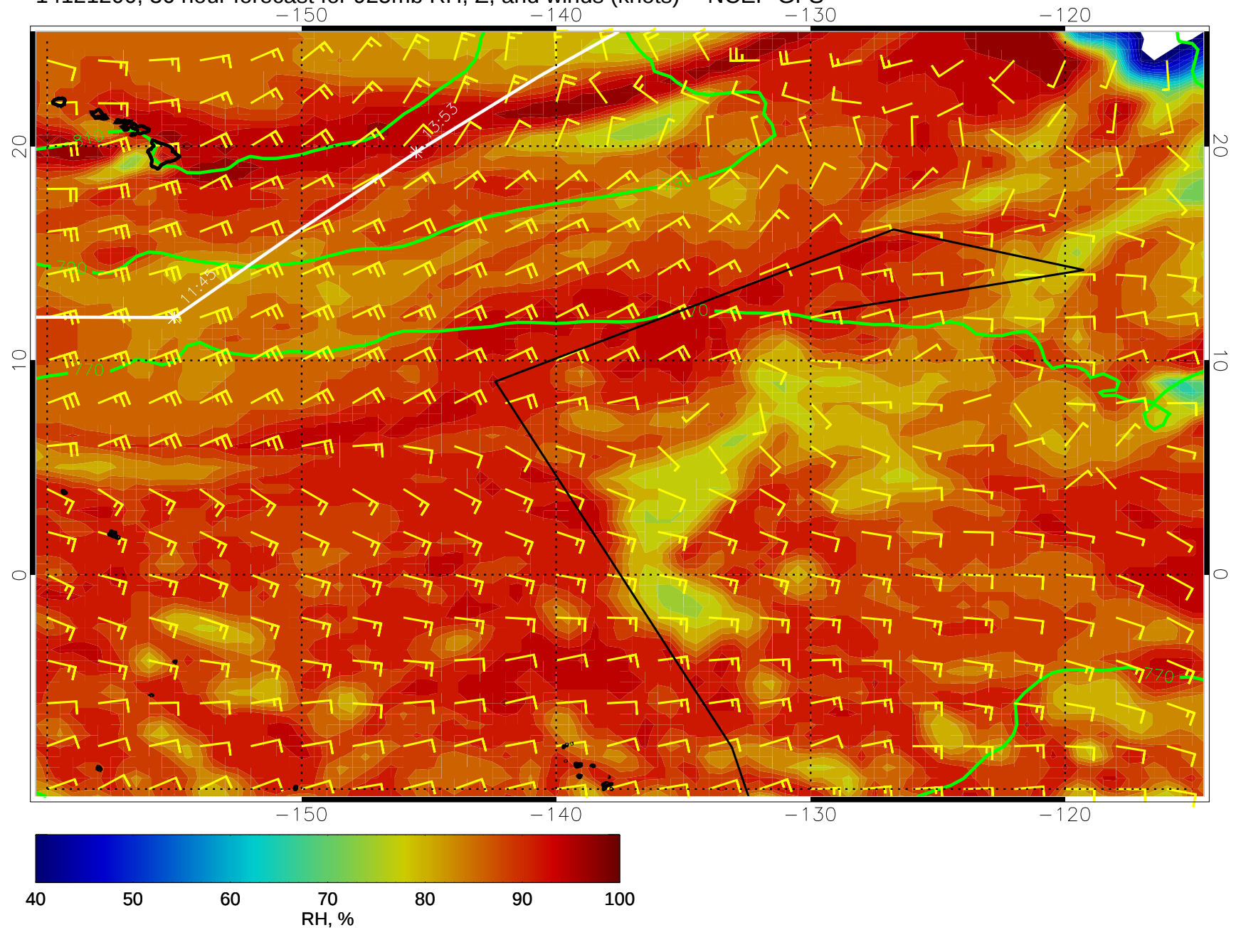
14121200, 36 hour forecast for 925mb RH, Z, and winds (knots) -- NCEP GFS
