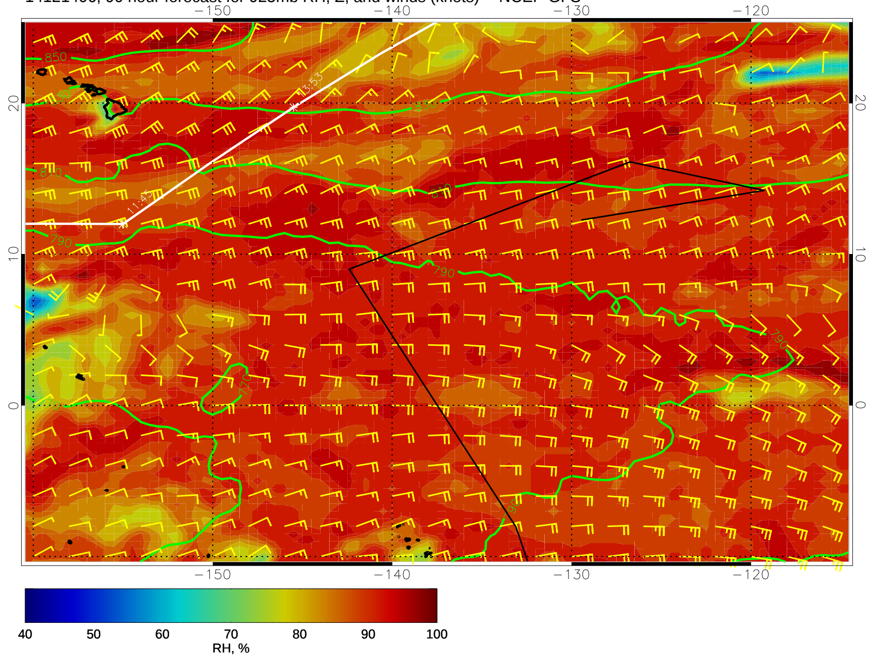
14121406, 90 hour forecast for 925mb RH, Z, and winds (knots) -- NCEP GFS
