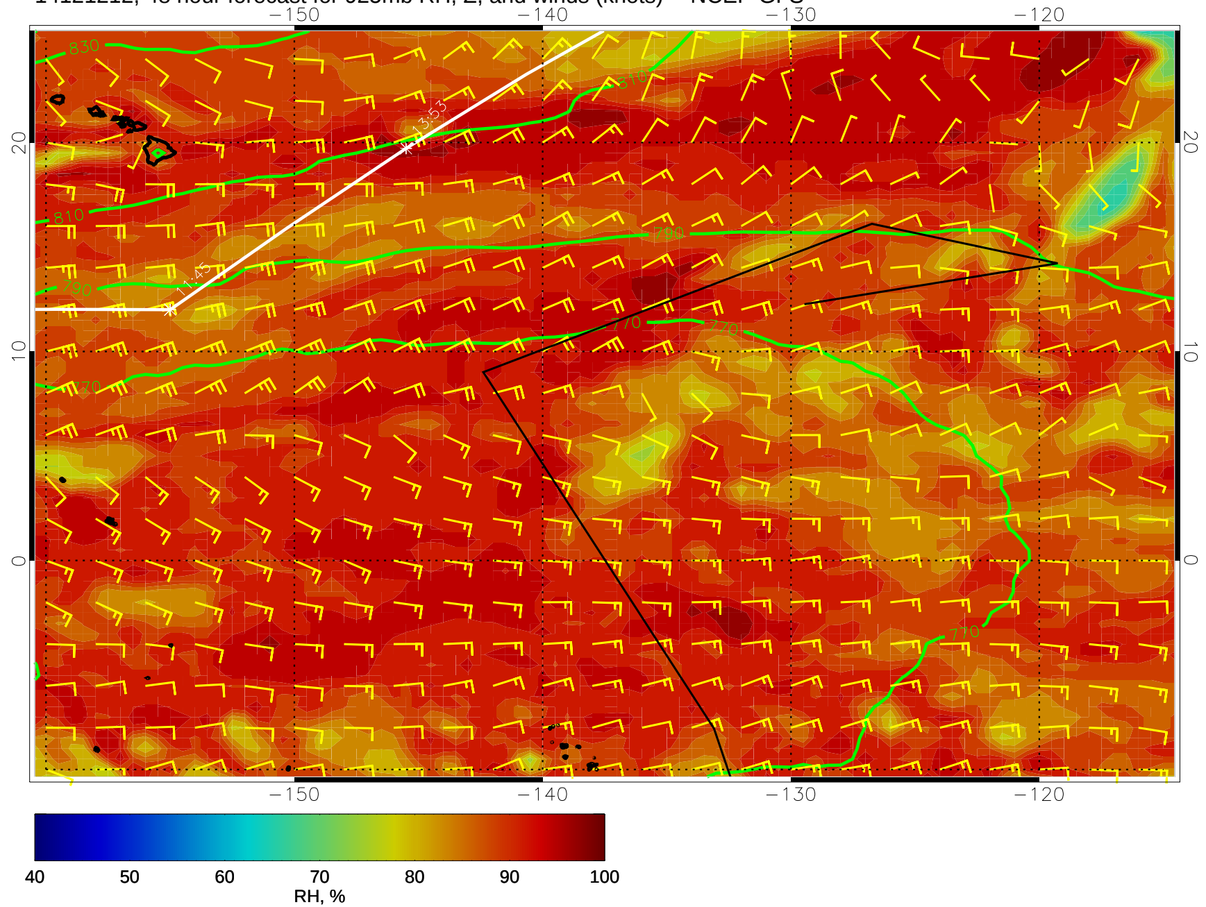
14121212, 48 hour forecast for 925mb RH, Z, and winds (knots) -- NCEP GFS
