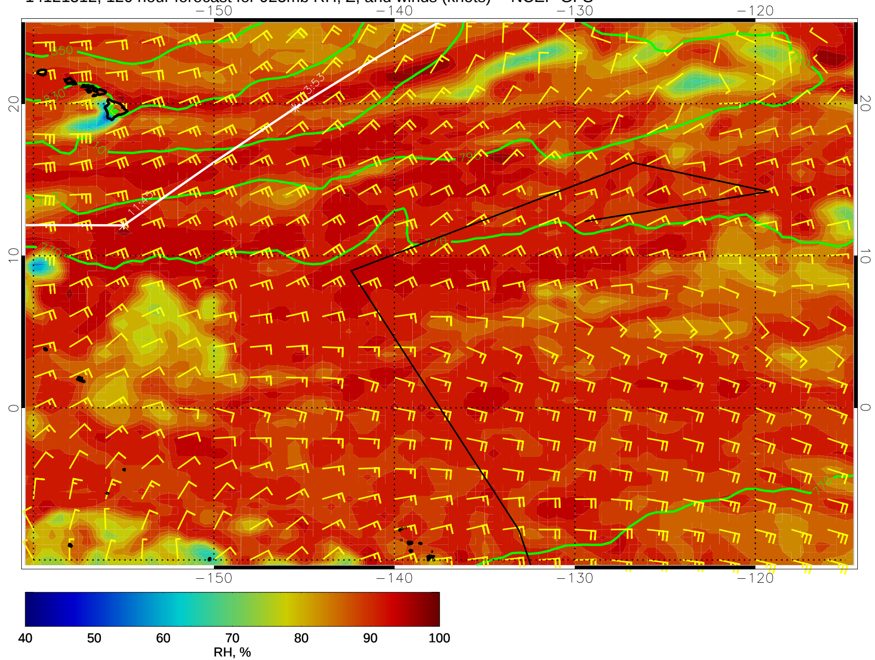
14121512, 120 hour forecast for 925mb RH, Z, and winds (knots) -- NCEP GFS
