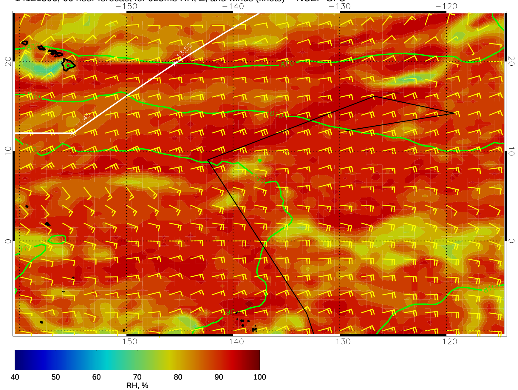
14121306, 66 hour forecast for 925mb RH, Z, and winds (knots) -- NCEP GFS
