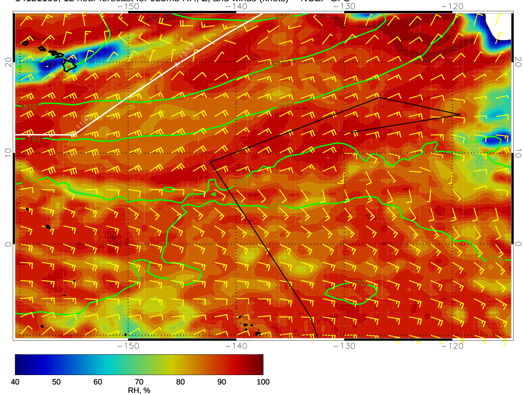
14121100, 12 hour forecast for 925mb RH, Z, and winds (knots) -- NCEP GFS
