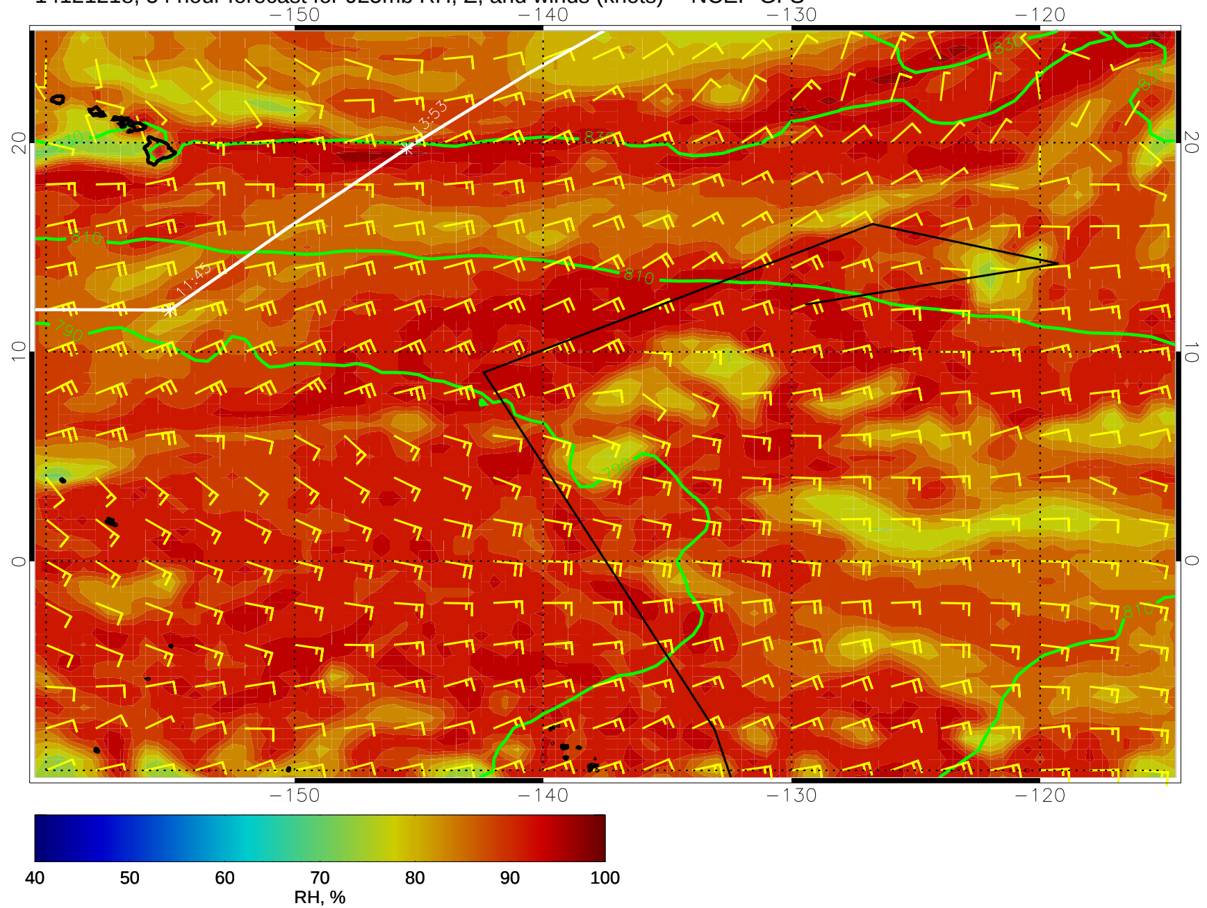
14121218, 54 hour forecast for 925mb RH, Z, and winds (knots) -- NCEP GFS
