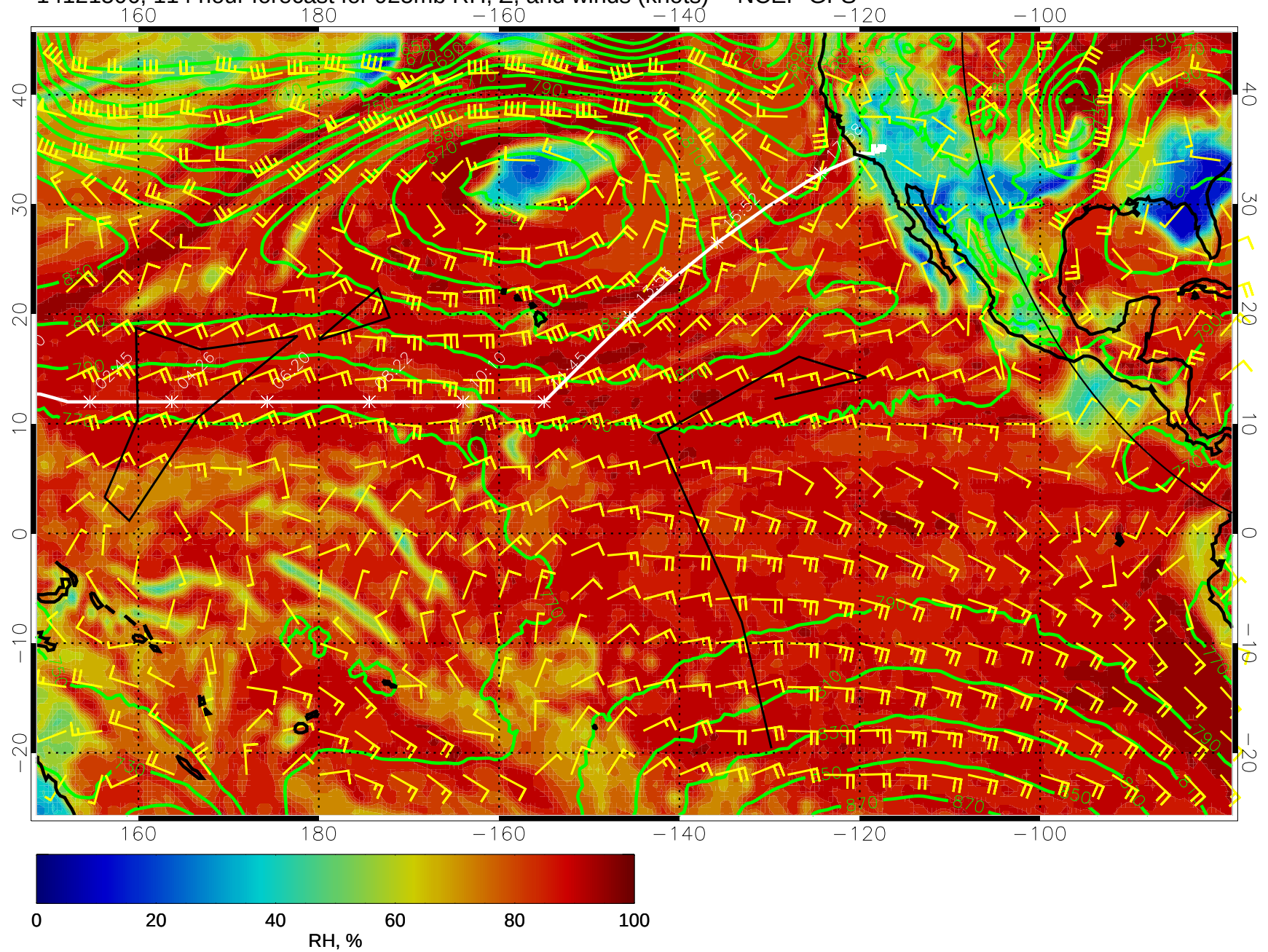
14121506, 114 hour forecast for 925mb RH, Z, and winds (knots) -- NCEP GFS
