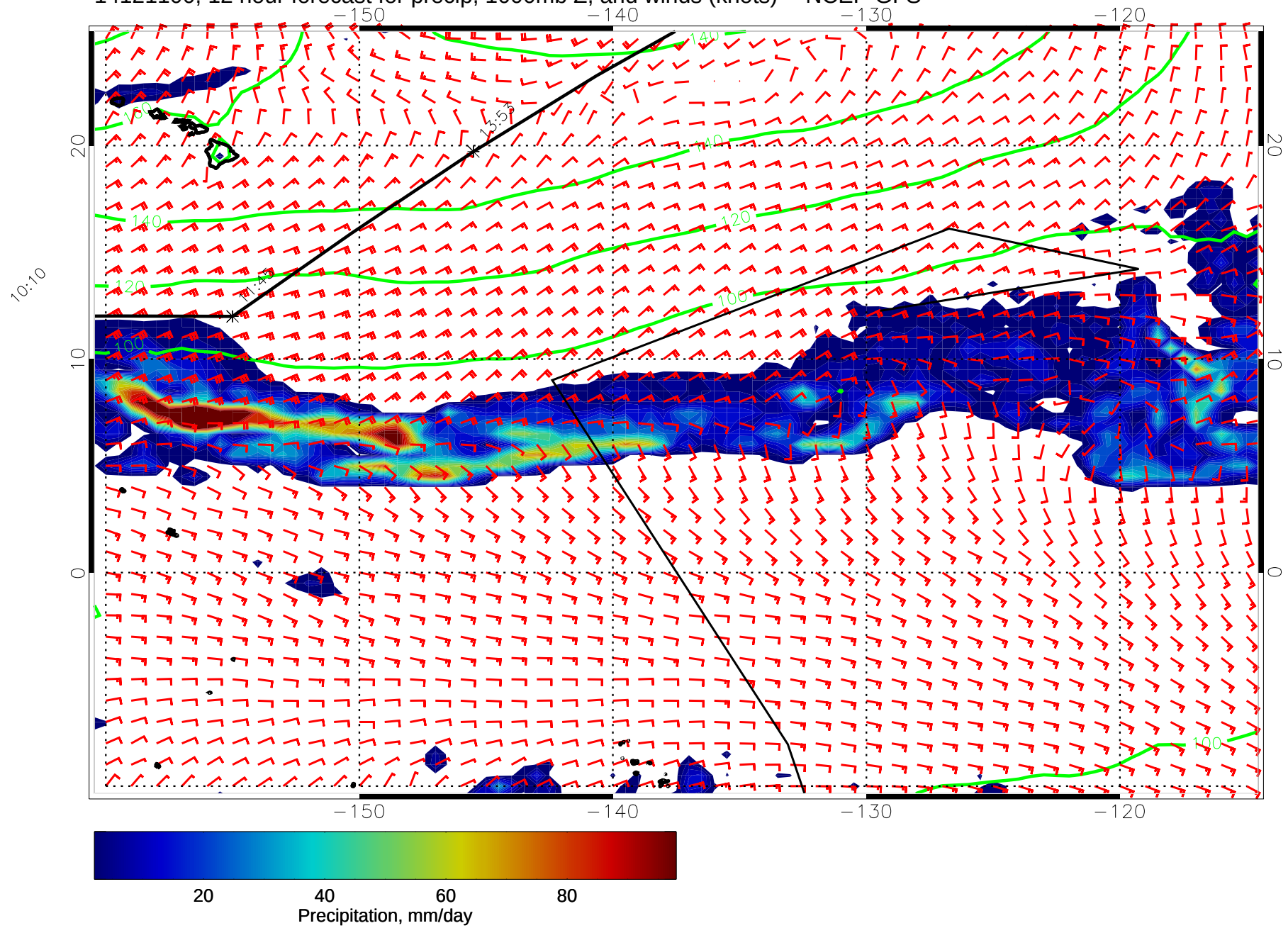
14121100, 12 hour forecast for precip, 1000mb Z, and winds (knots) -- NCEP GFS
