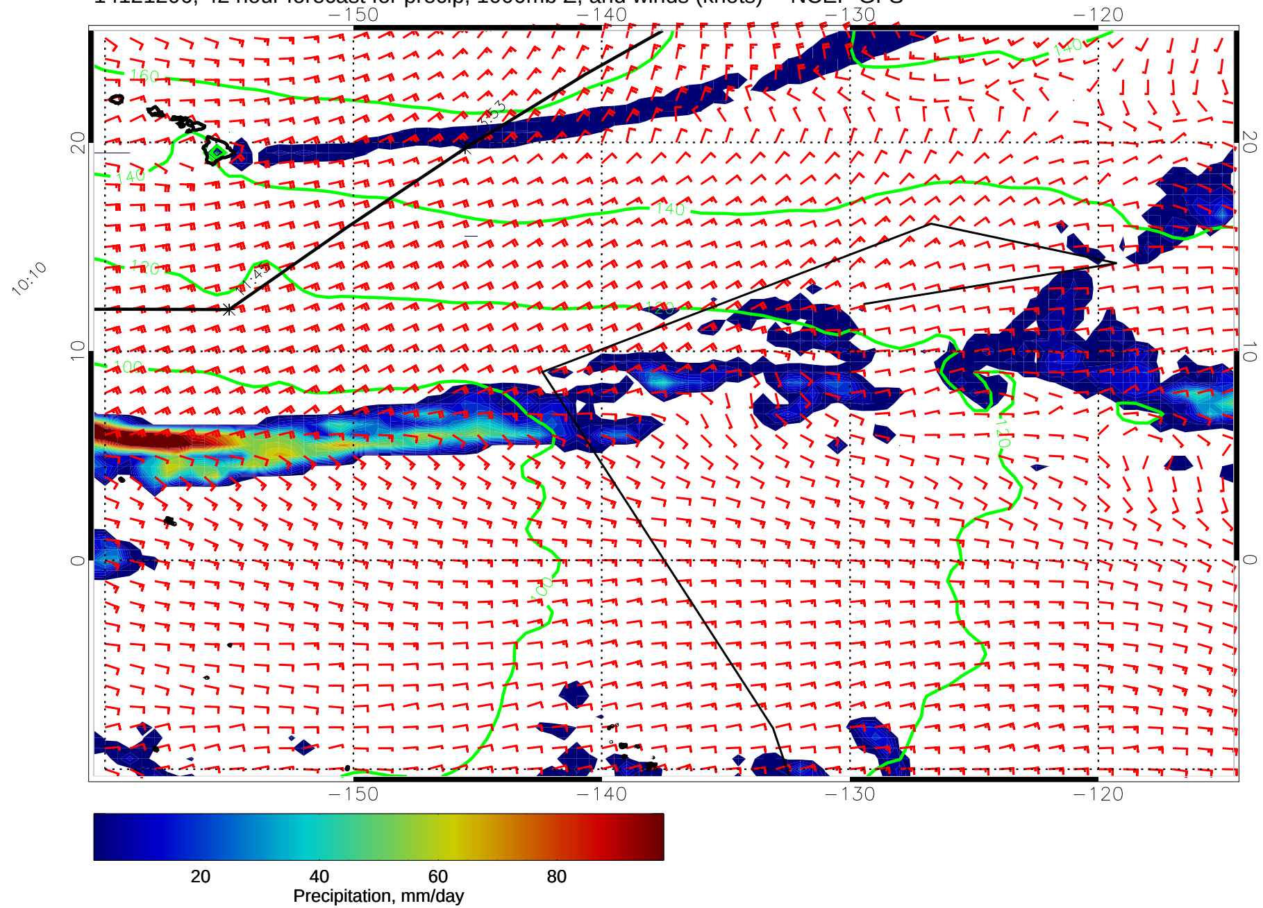
14121206, 42 hour forecast for precip, 1000mb Z, and winds (knots) -- NCEP GFS
