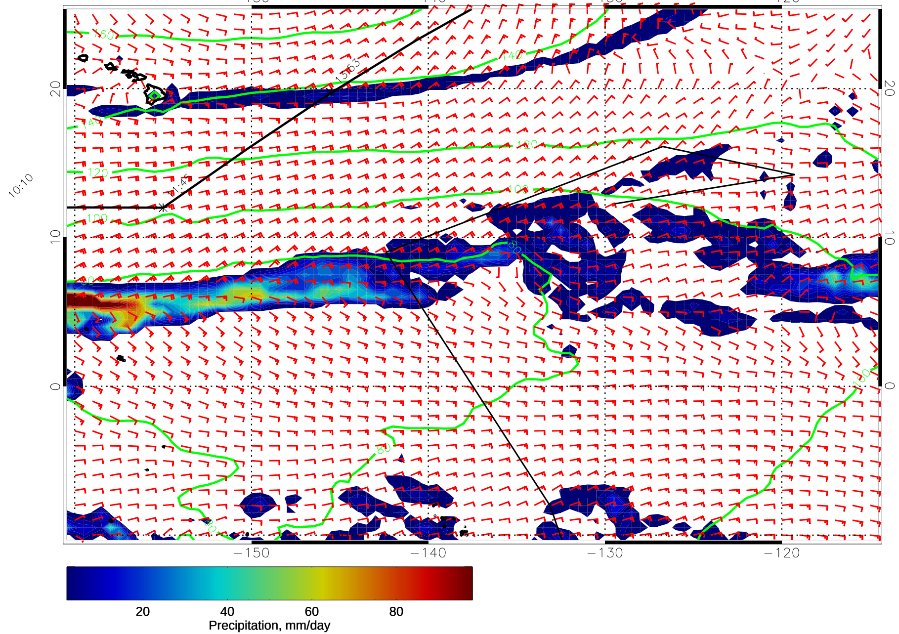
14121212, 48 hour forecast for precip, 1000mb Z, and winds (knots) -- NCEP GFS
