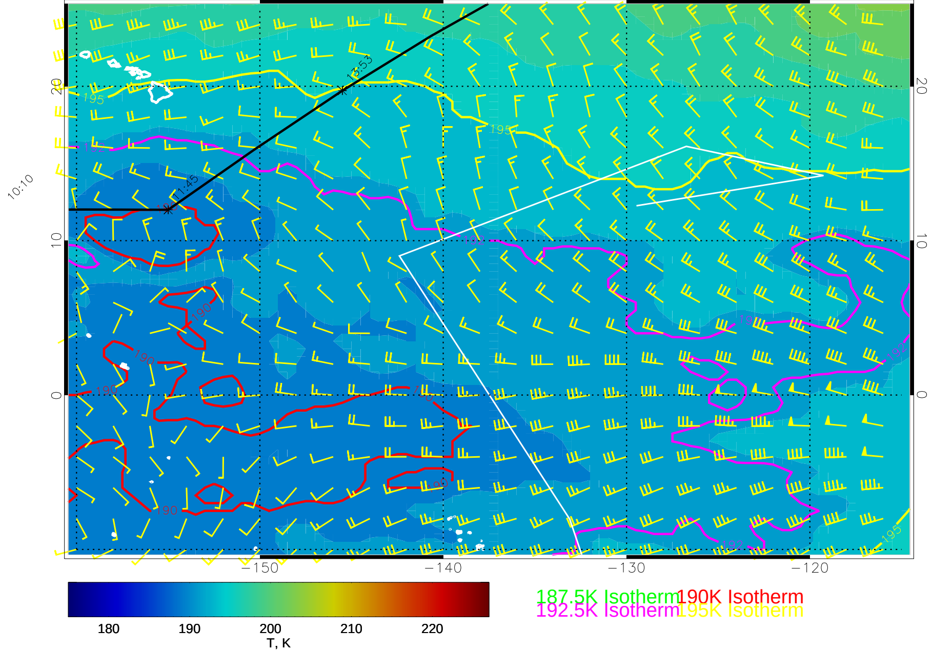
14121318, 78 hour forecast for 100mb T and winds (knots) -- NCEP GFS
