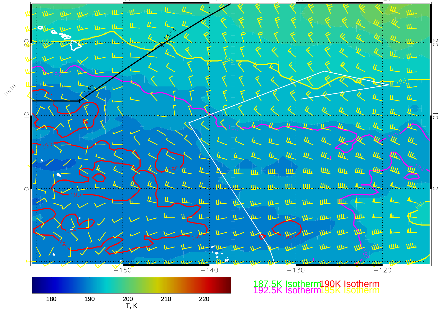
14121312, 72 hour forecast for 100mb T and winds (knots) -- NCEP GFS
