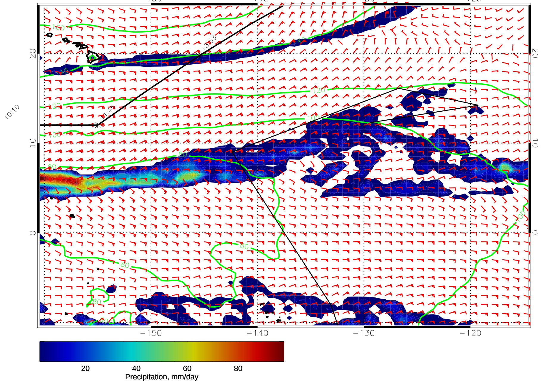
14121212, 60 hour forecast for precip, 1000mb Z, and winds (knots) -- NCEP GFS
