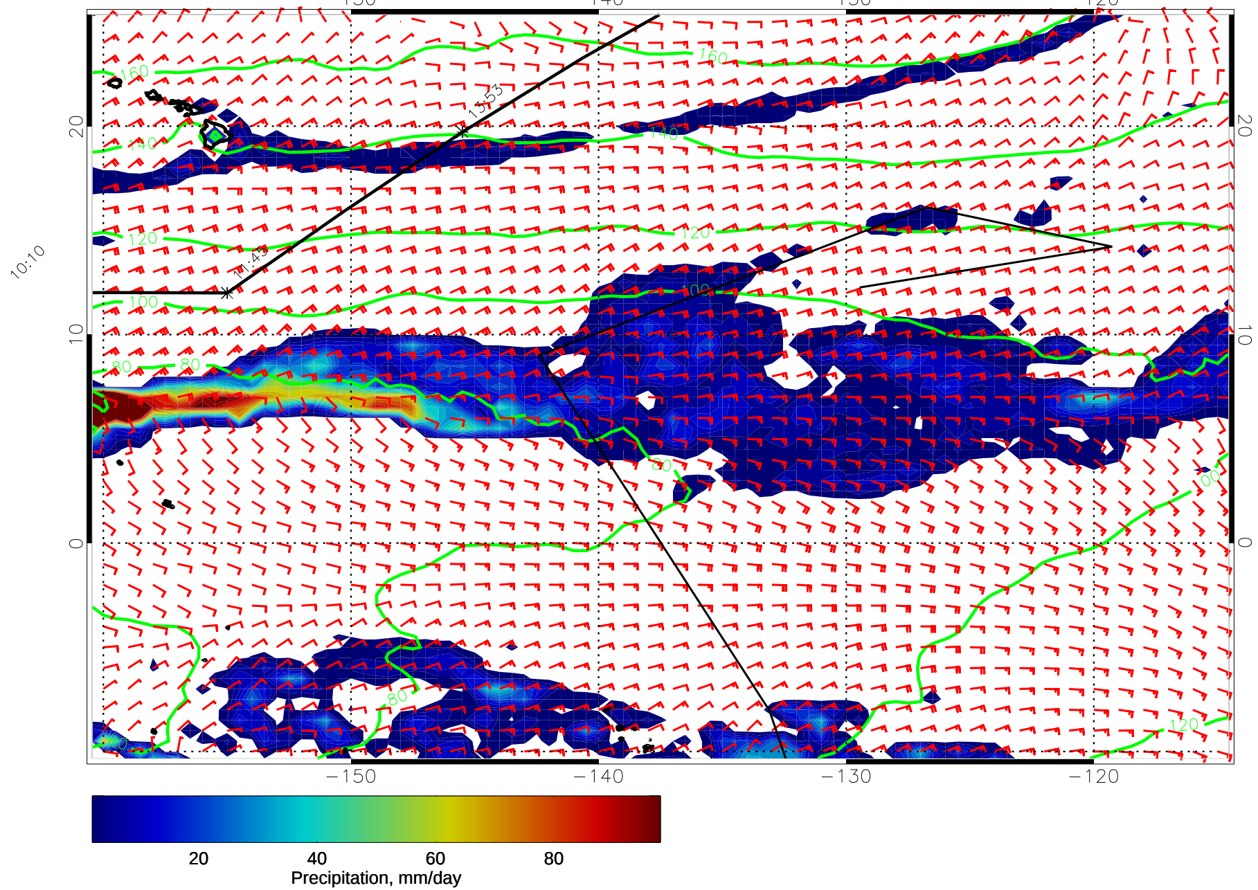
14121312, 84 hour forecast for precip, 1000mb Z, and winds (knots) -- NCEP GFS
