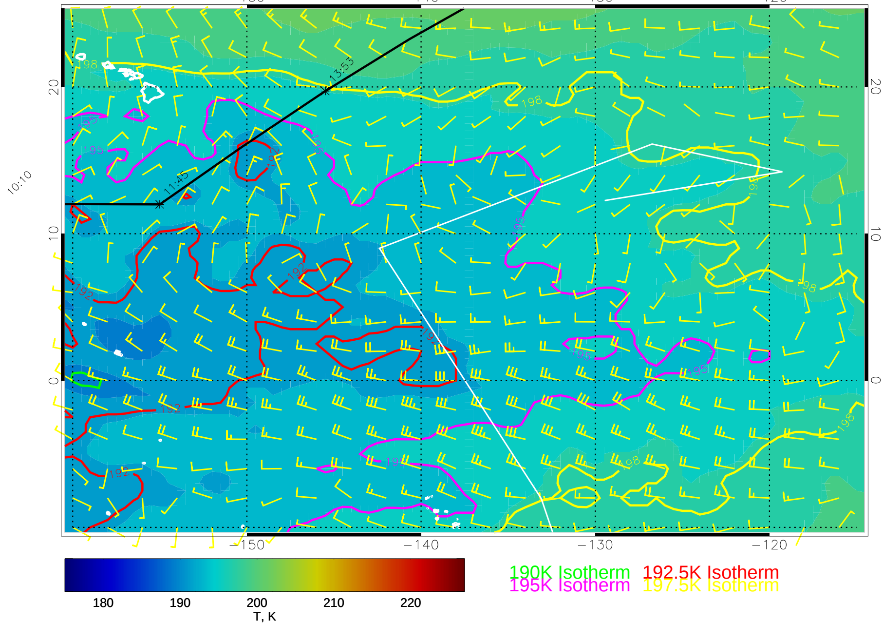
14121500, 120 hour forecast for 70mb T and winds (knots) -- NCEP GFS
