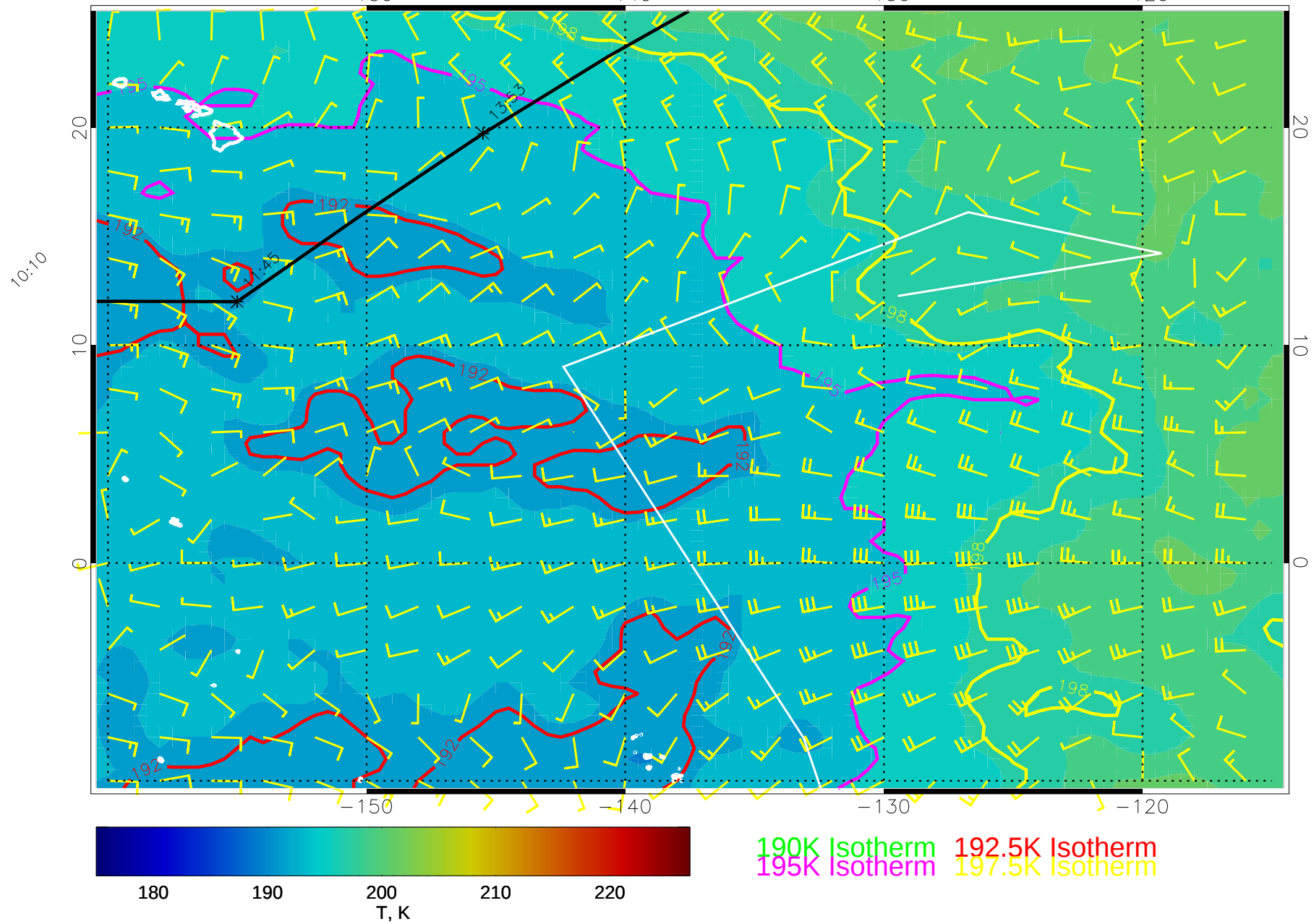
14121206, 54 hour forecast for 70mb T and winds (knots) -- NCEP GFS
