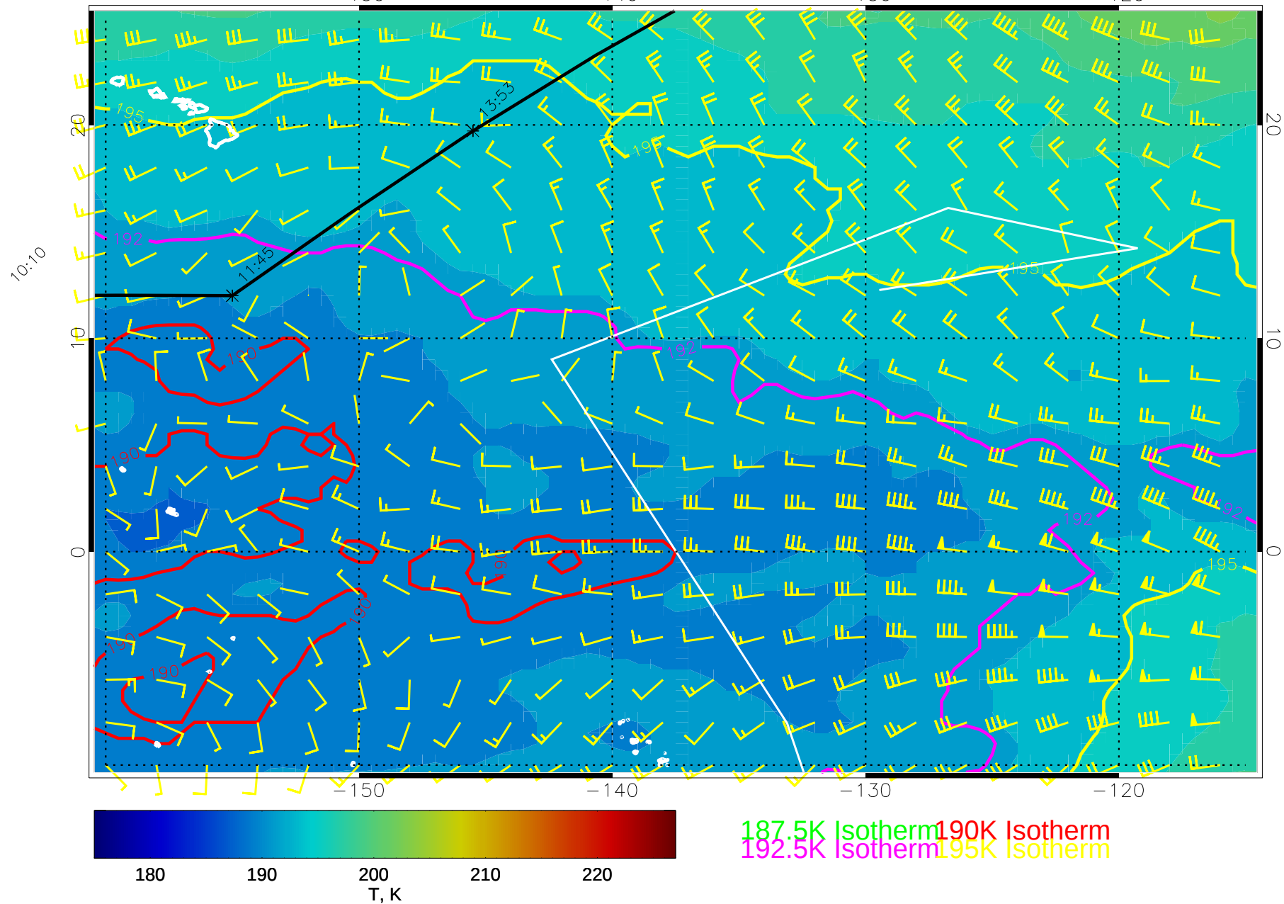
14121306, 78 hour forecast for 100mb T and winds (knots) -- NCEP GFS
