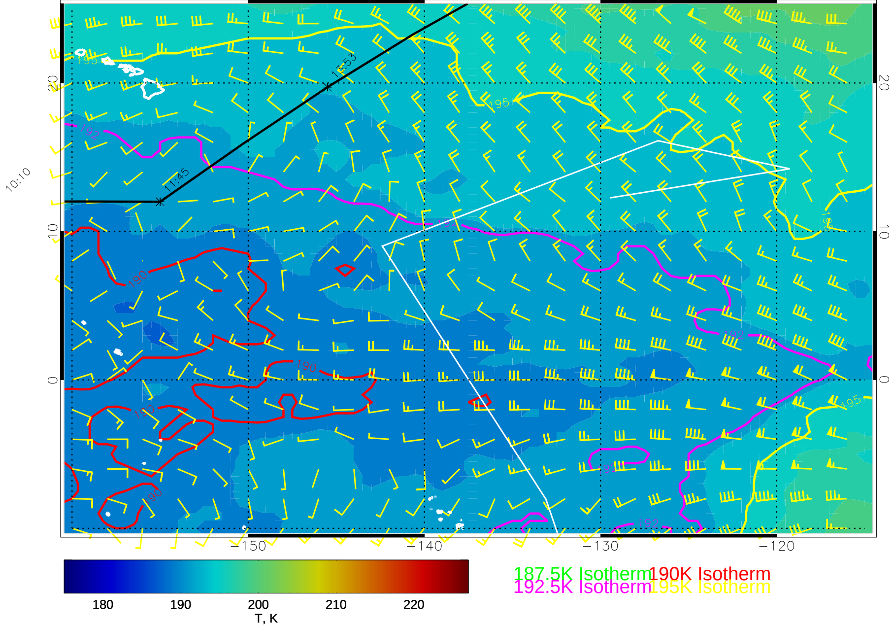
14121300, 72 hour forecast for 100mb T and winds (knots) -- NCEP GFS
