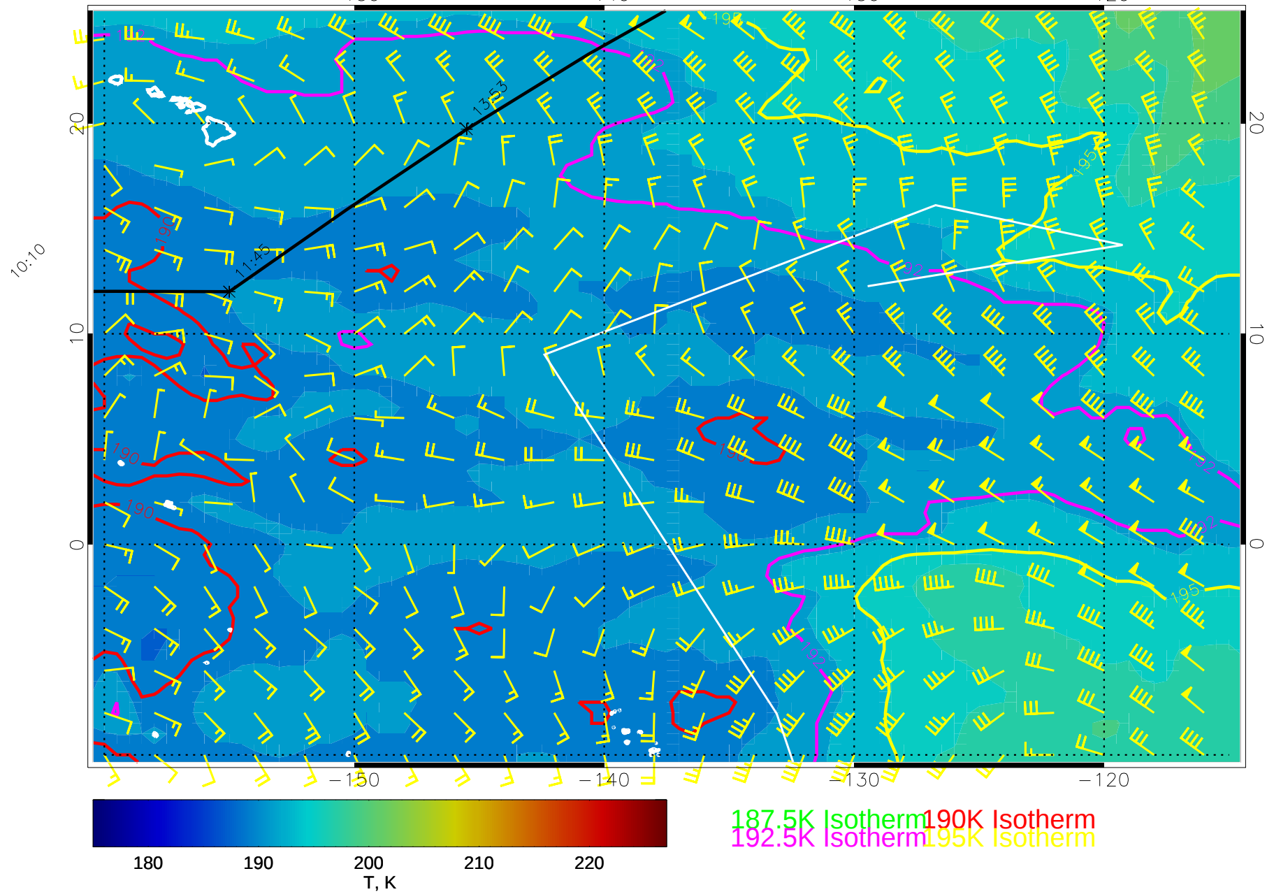
14121100, 24 hour forecast for 100mb T and winds (knots) -- NCEP GFS
