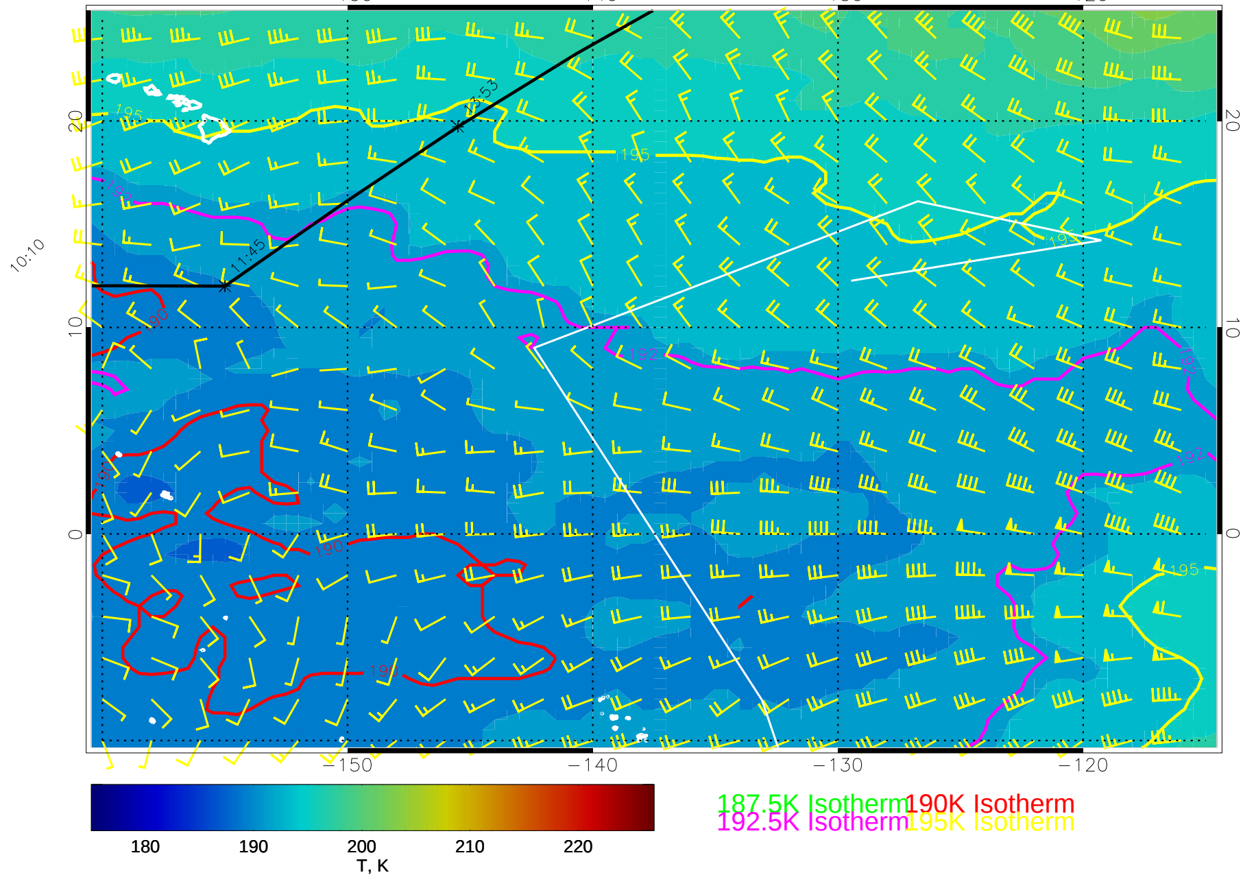
14121312, 84 hour forecast for 100mb T and winds (knots) -- NCEP GFS
