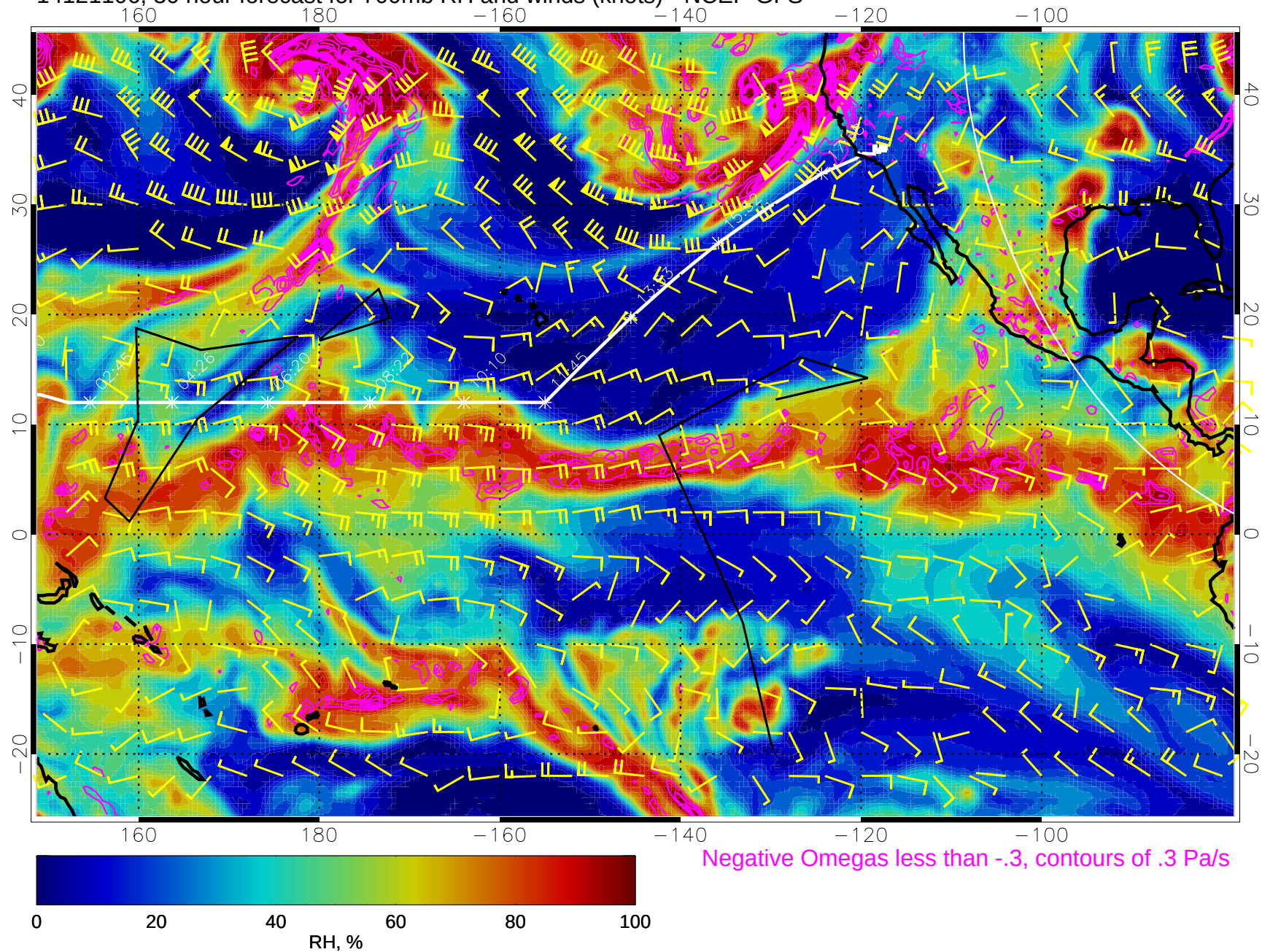
14121106, 30 hour forecast for 700mb RH and winds (knots) - NCEP GFS
