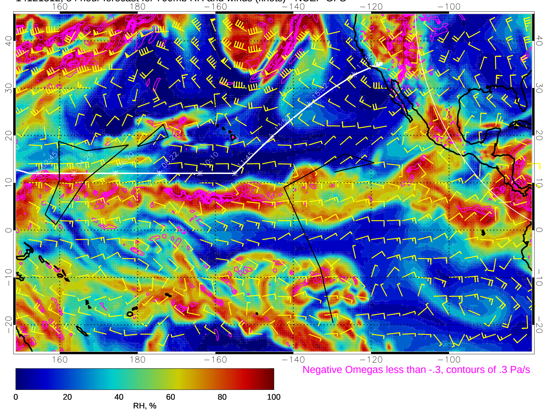
14121312, 84 hour forecast for 700mb RH and winds (knots) - NCEP GFS
