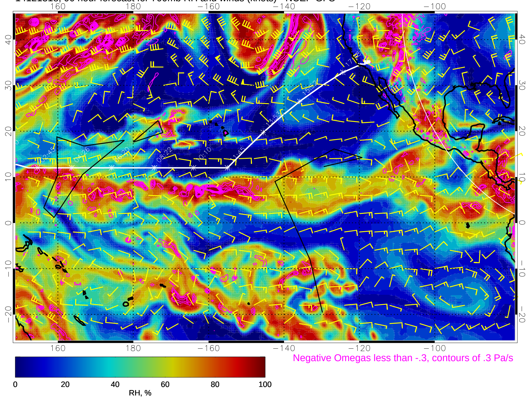
14121318, 90 hour forecast for 700mb RH and winds (knots) - NCEP GFS
