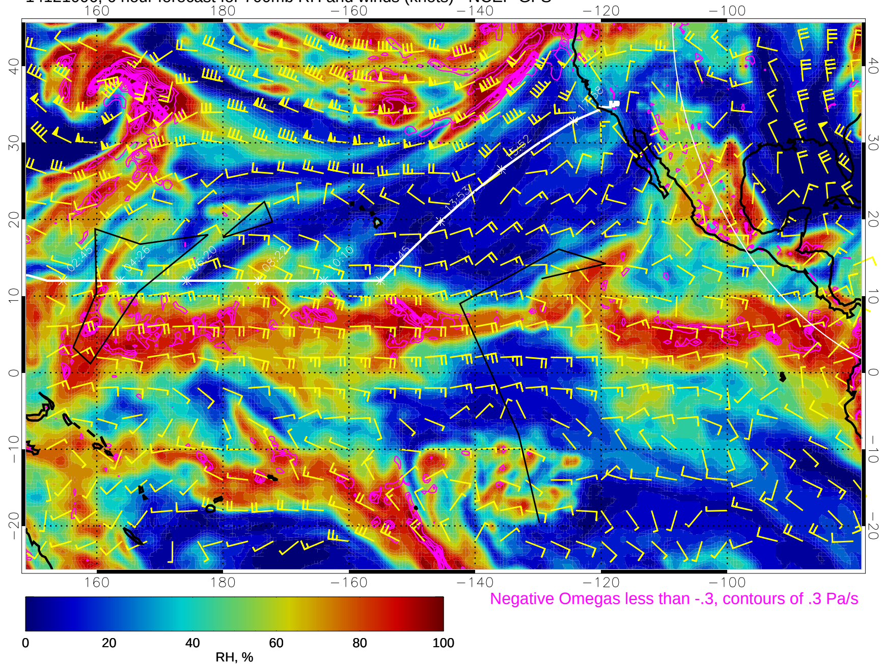
14121006, 6 hour forecast for 700mb RH and winds (knots) - NCEP GFS
