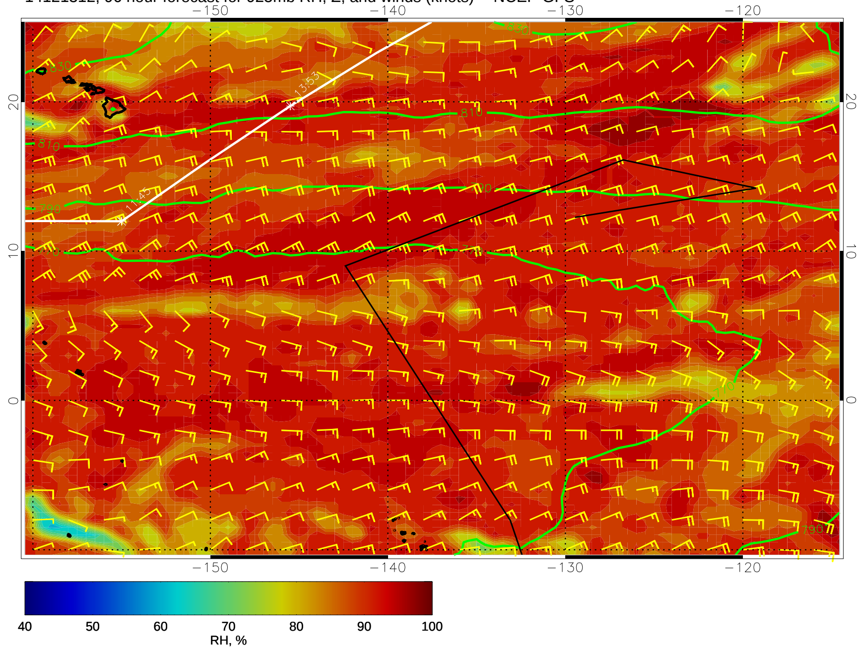
14121312, 96 hour forecast for 925mb RH, Z, and winds (knots) -- NCEP GFS
