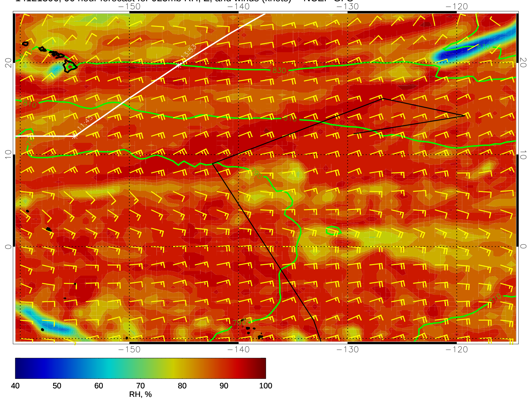
14121306, 90 hour forecast for 925mb RH, Z, and winds (knots) -- NCEP GFS
