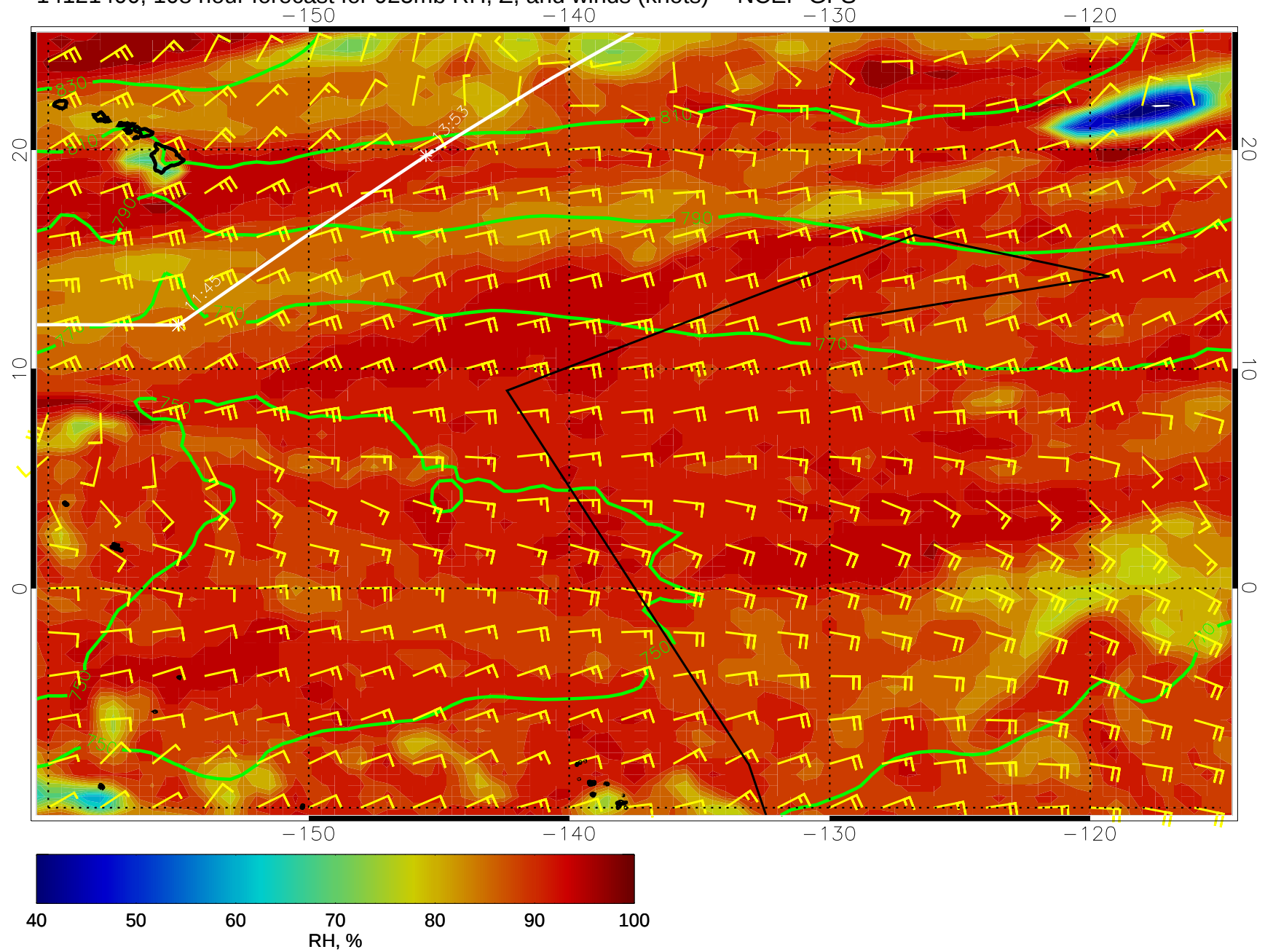
14121400, 108 hour forecast for 925mb RH, Z, and winds (knots) -- NCEP GFS
