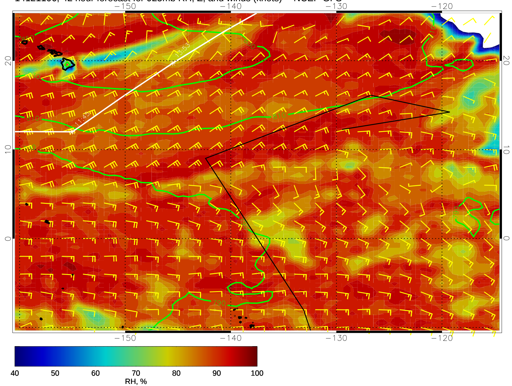
14121106, 42 hour forecast for 925mb RH, Z, and winds (knots) -- NCEP GFS
