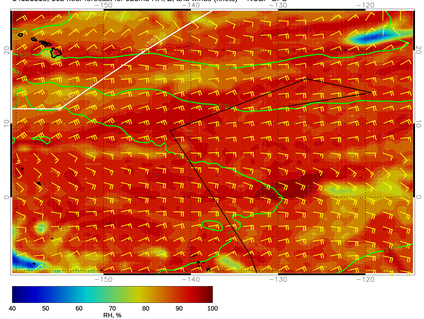
14121318, 102 hour forecast for 925mb RH, Z, and winds (knots) -- NCEP GFS
