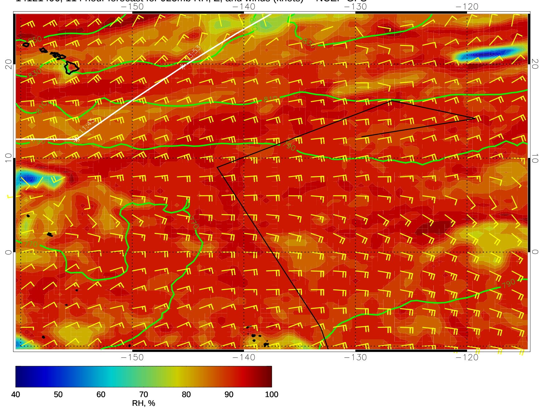
14121406, 114 hour forecast for 925mb RH, Z, and winds (knots) -- NCEP GFS
