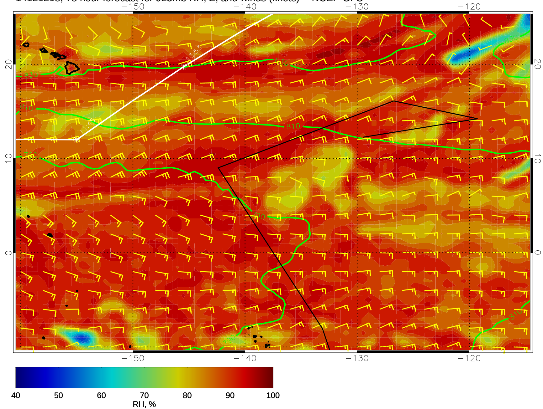
14121218, 78 hour forecast for 925mb RH, Z, and winds (knots) -- NCEP GFS
