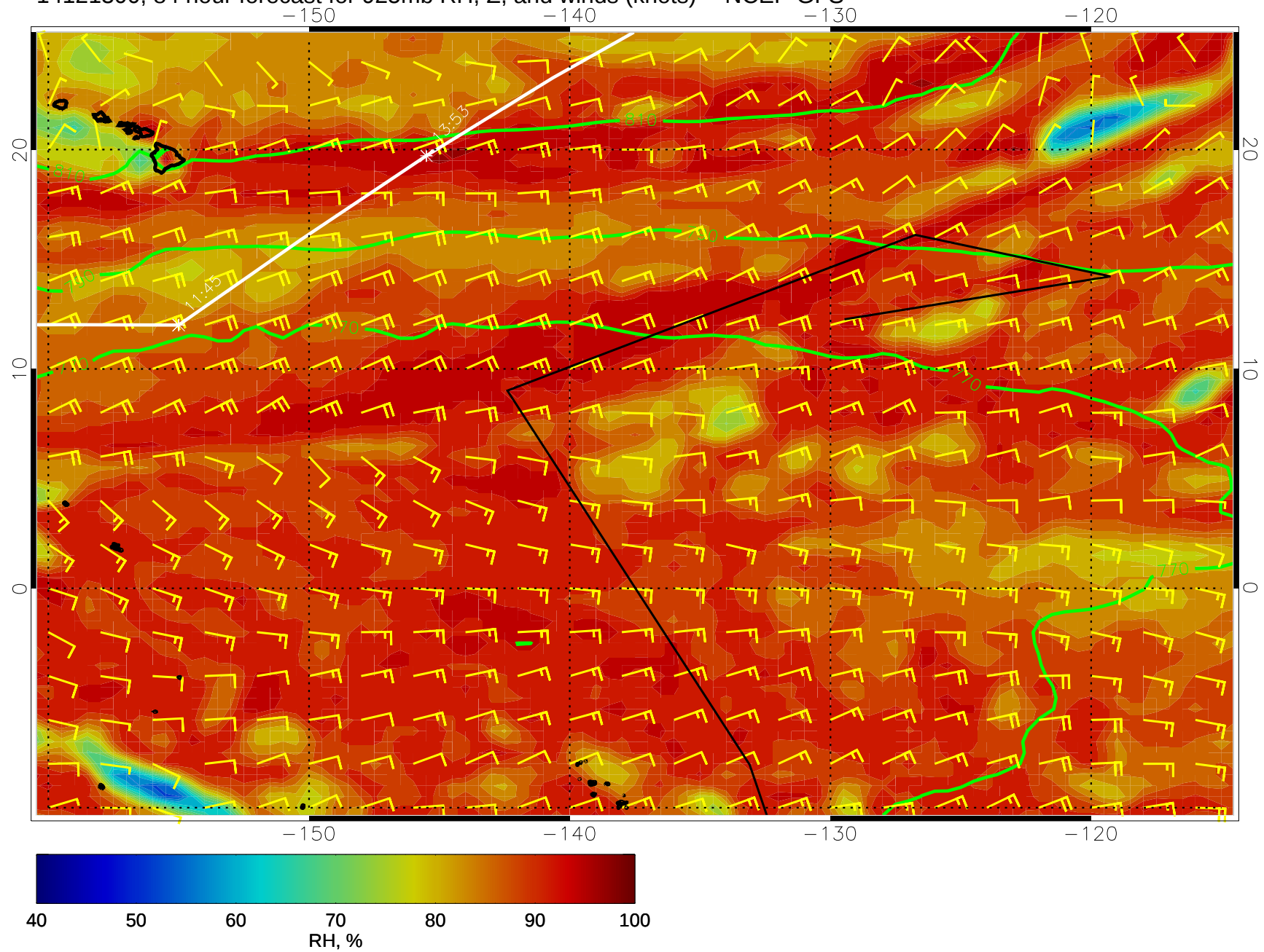
14121300, 84 hour forecast for 925mb RH, Z, and winds (knots) -- NCEP GFS
