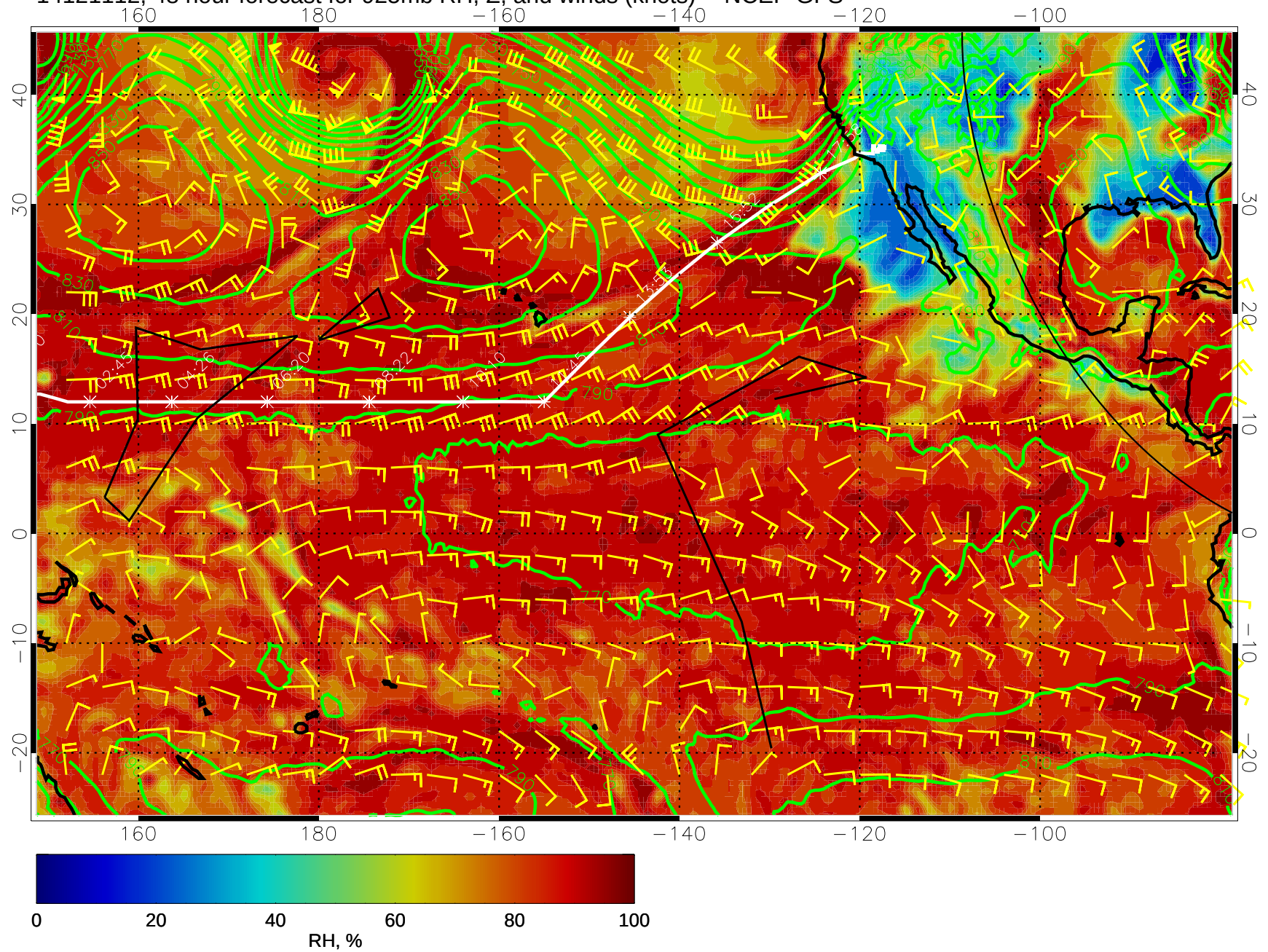
14121112, 48 hour forecast for 925mb RH, Z, and winds (knots) -- NCEP GFS
