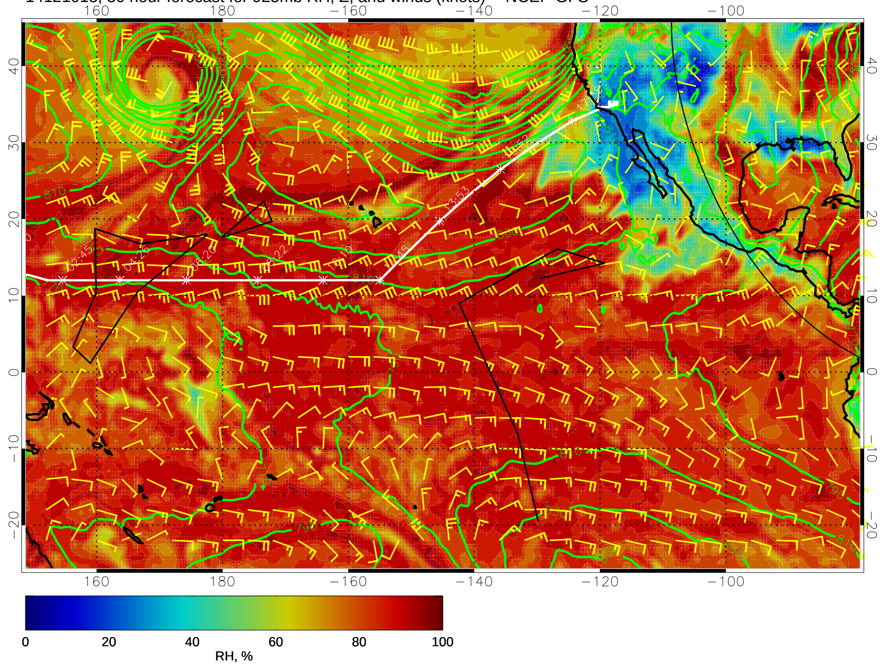
14121018, 30 hour forecast for 925mb RH, Z, and winds (knots) -- NCEP GFS
