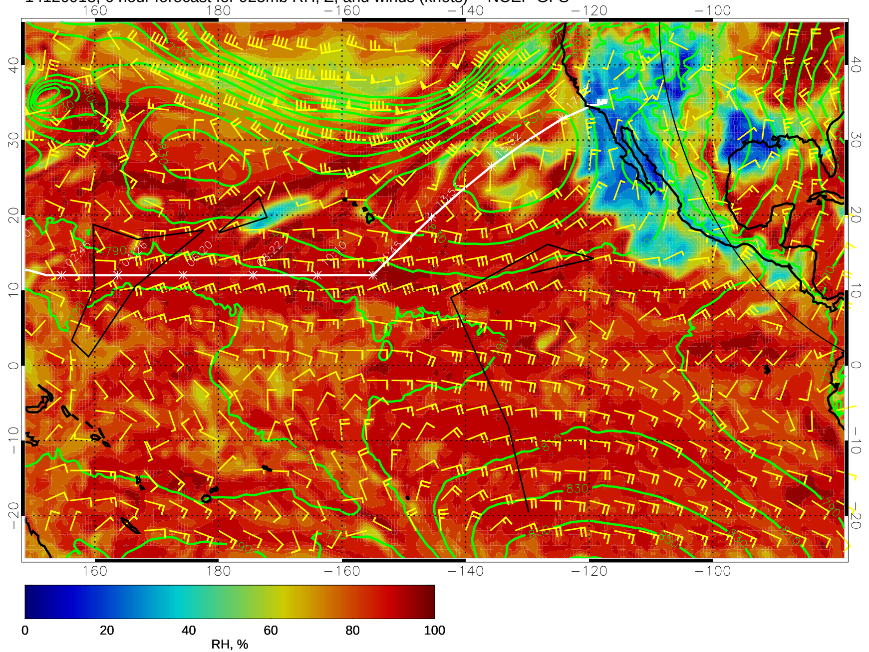
14120918, 6 hour forecast for 925mb RH, Z, and winds (knots) -- NCEP GFS
