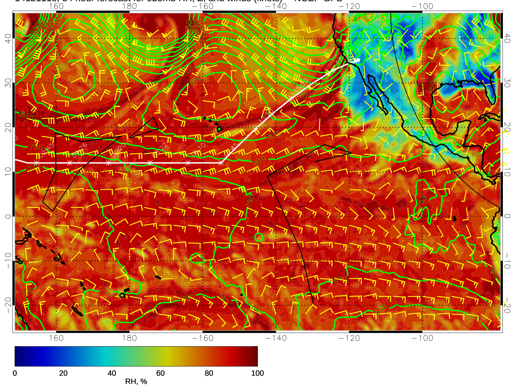
14121118, 54 hour forecast for 925mb RH, Z, and winds (knots) -- NCEP GFS
