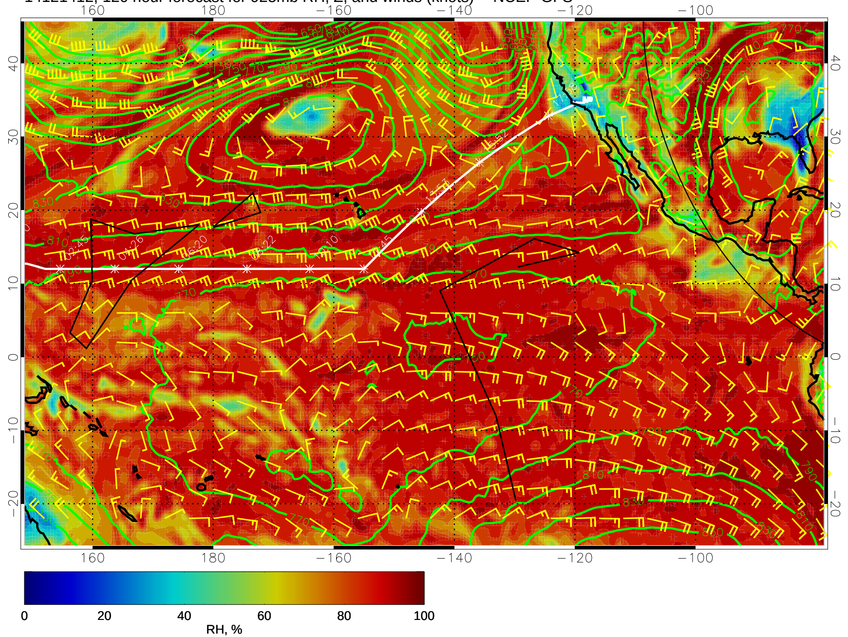
14121412, 120 hour forecast for 925mb RH, Z, and winds (knots) -- NCEP GFS
