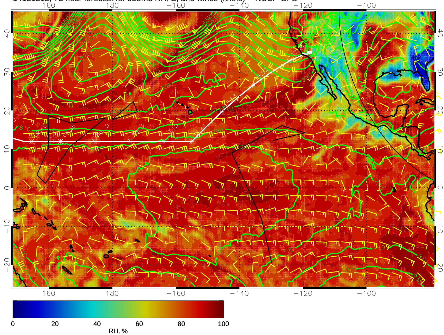
14121212, 72 hour forecast for 925mb RH, Z, and winds (knots) -- NCEP GFS
