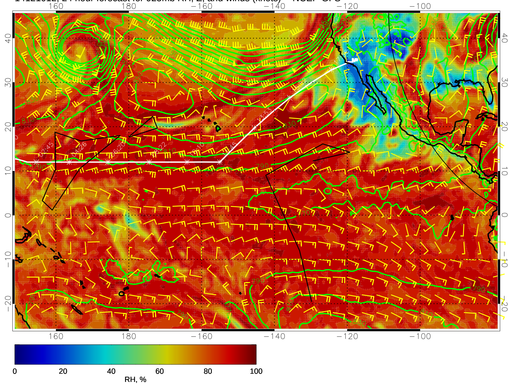
14121012, 24 hour forecast for 925mb RH, Z, and winds (knots) -- NCEP GFS
