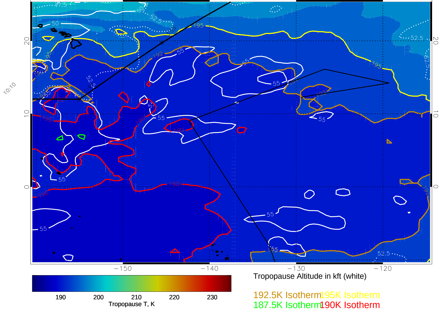
14121412, 120 hour forecast for Tropopause T and Alt(kft) -- NCEP GFS
