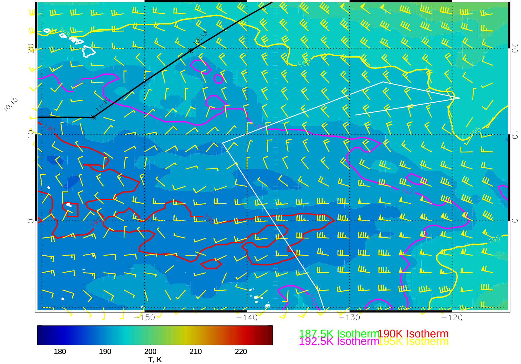
14121300, 84 hour forecast for 100mb T and winds (knots) -- NCEP GFS
