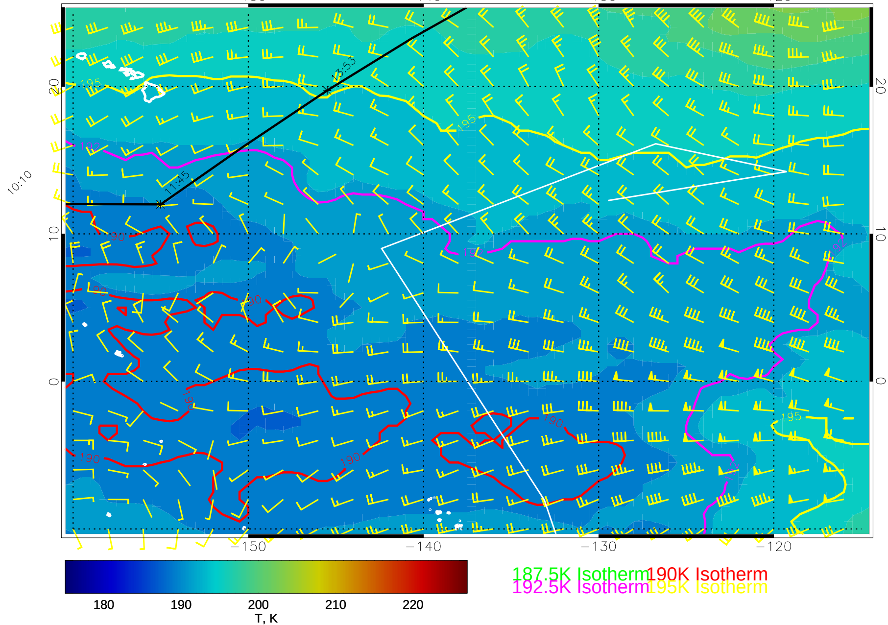
14121312, 96 hour forecast for 100mb T and winds (knots) -- NCEP GFS
