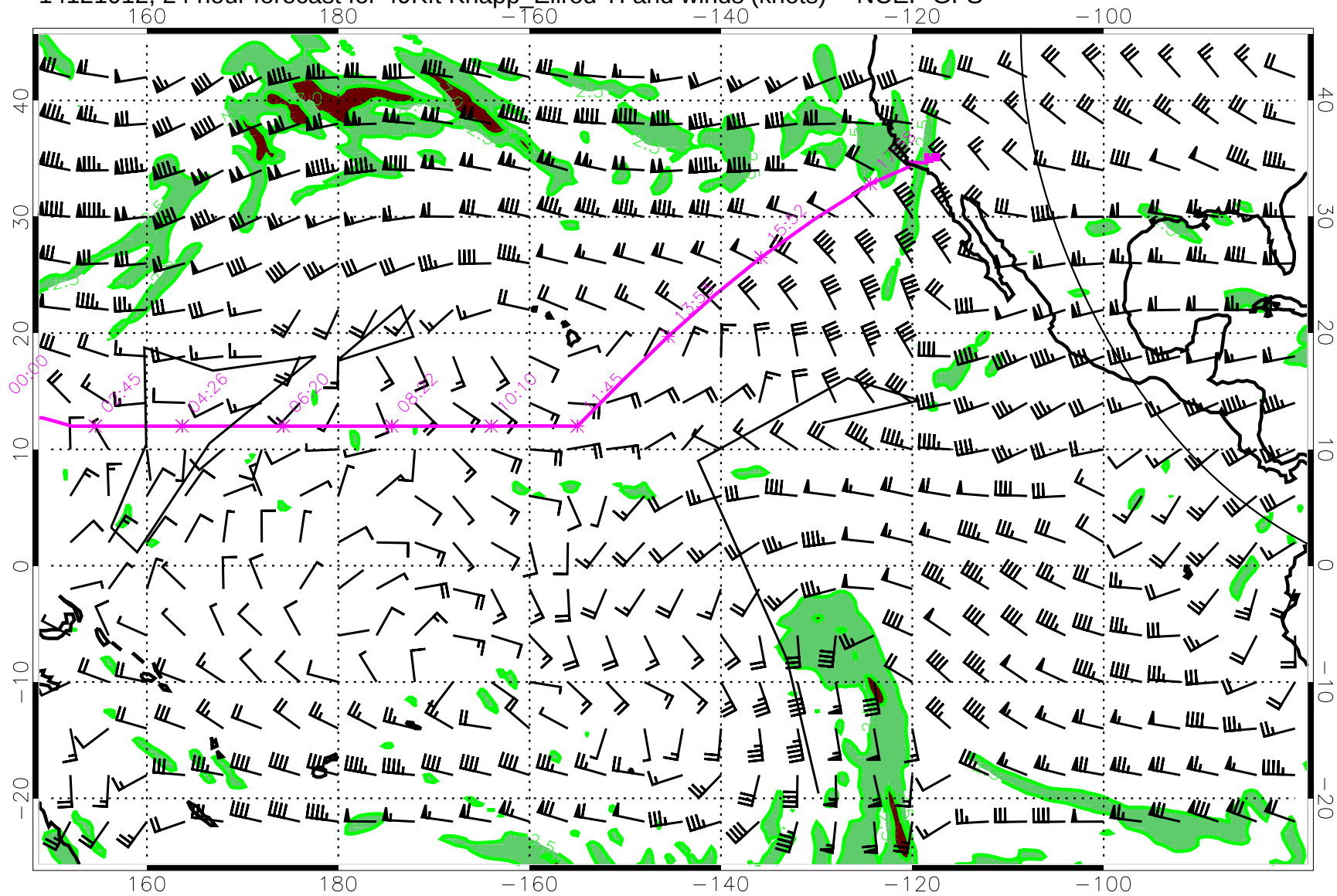
14121012, 24 hour forecast for 49Kft Knapp_Ellrod TI and winds (knots) -- NCEP GFS
